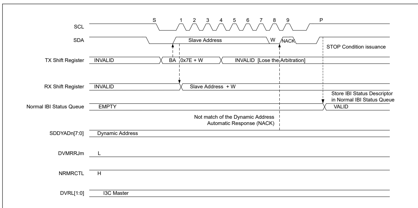
Figure 28.83 Mastership request : NACK (not match the DVDYAD[7:0] of DAT) and NRMRCTL = 1
