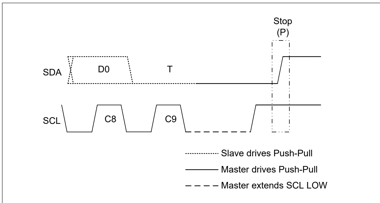
Figure 28.74 Master clock stalling in T-bit before STOP
