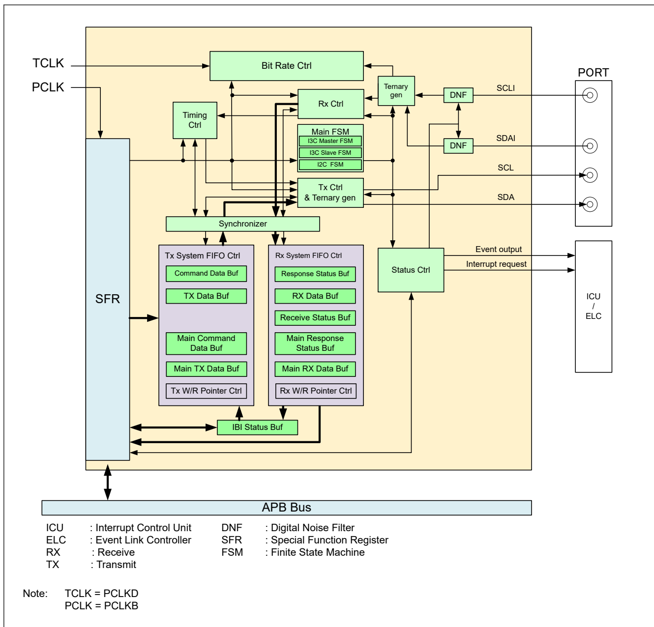
Figure 28.1 I3C block diagram
