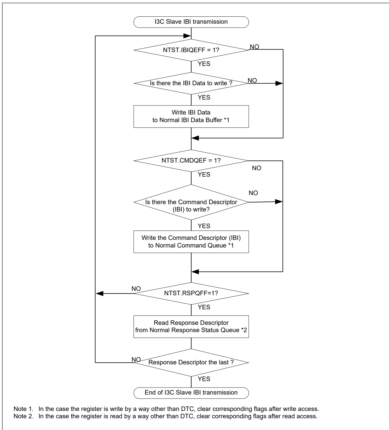
Figure 28.114 Example of I3C slave IBI transmission flowchart
