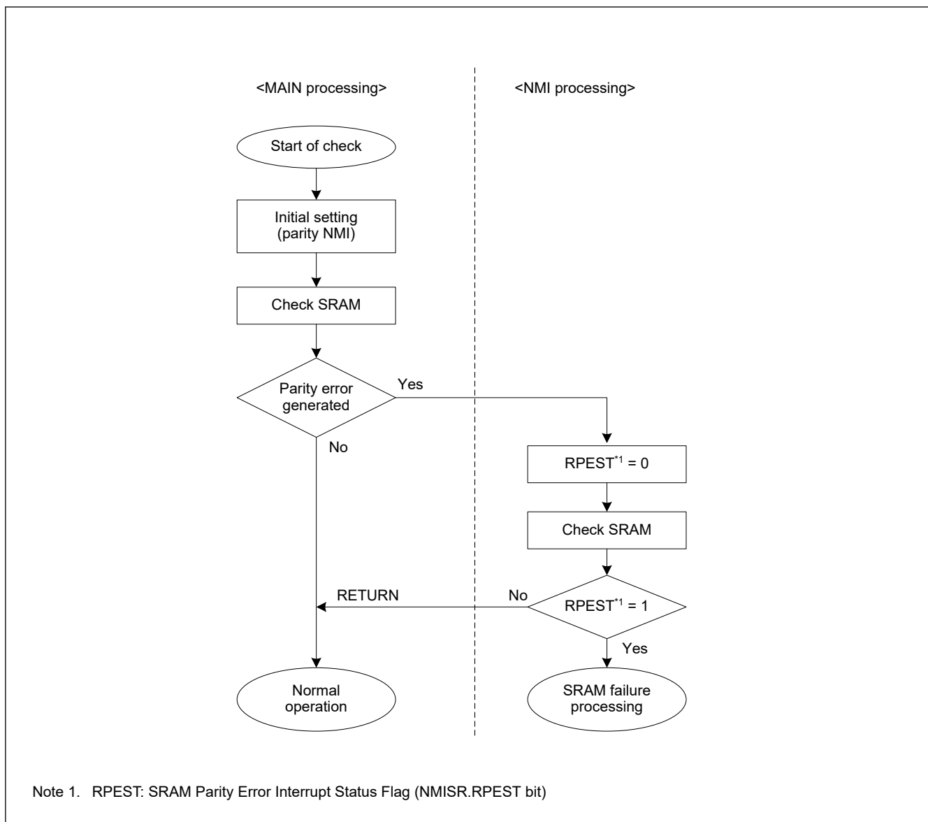
Figure 37.2 Flow of SRAM parity check when SRAM parity interrupt is enabled
