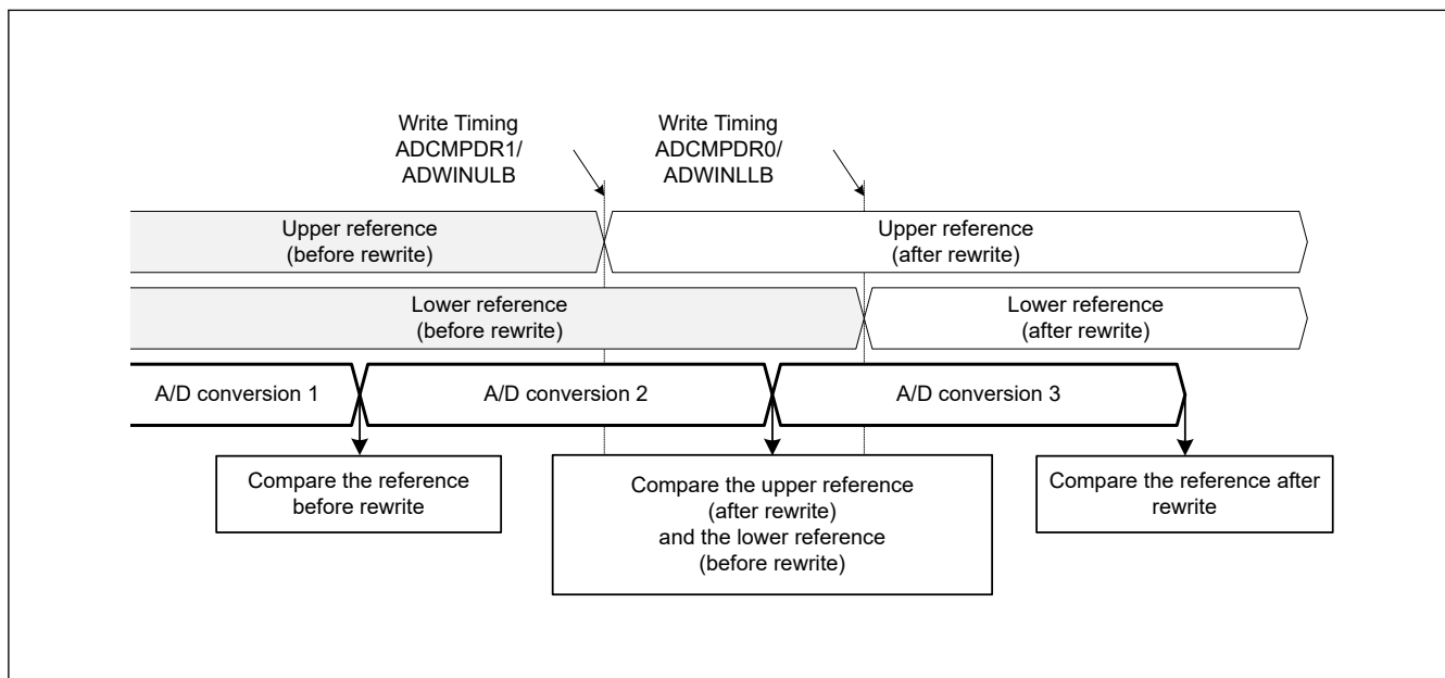
Figure 34.4 Comparison between upper and lower references before and after a rewrite
