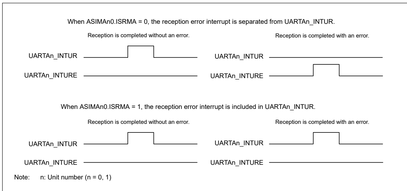
Figure 31.8 Various interrupt output waveforms depending on ASIMAn0.ISRMA setting
