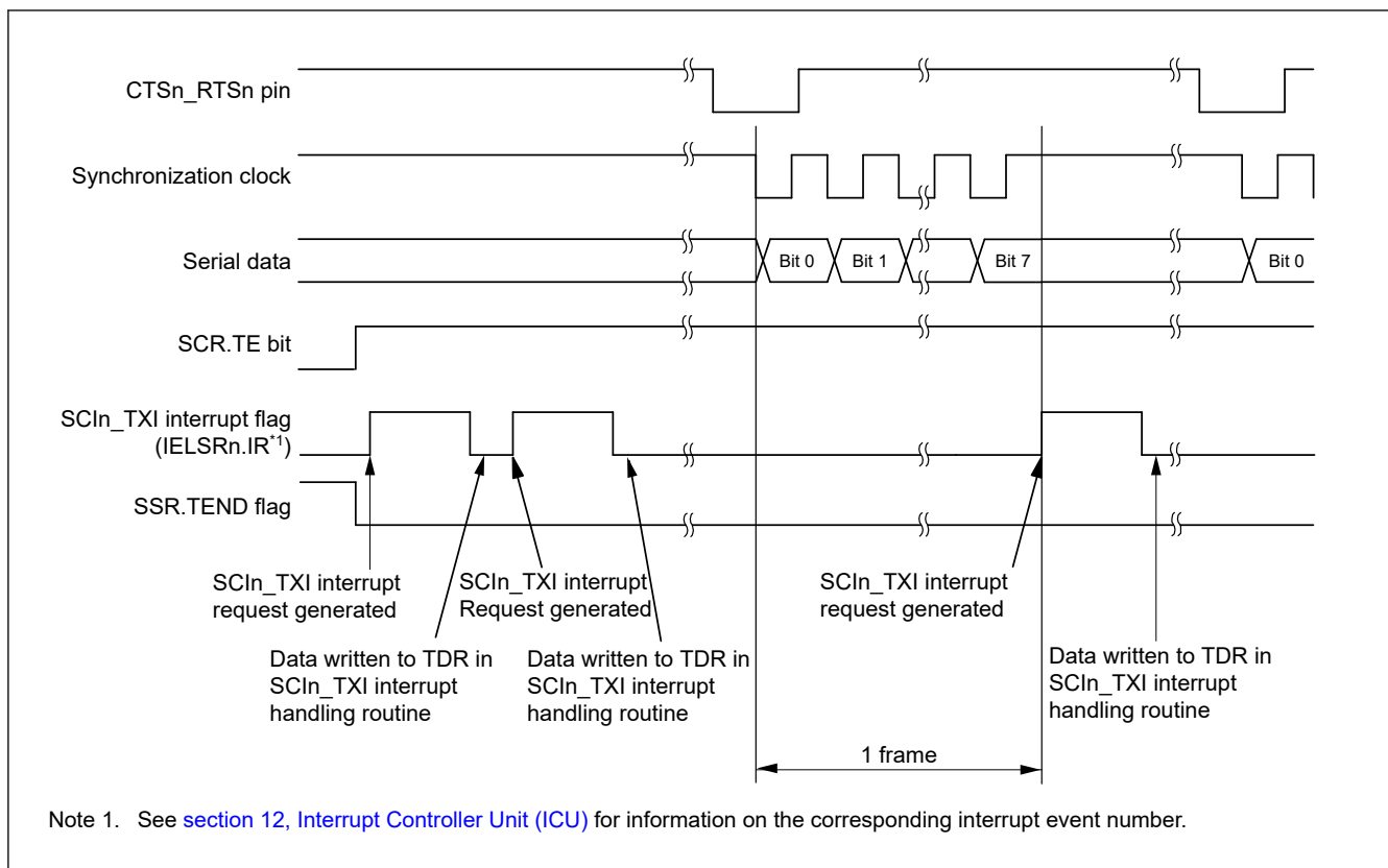
Figure 27.37 Example of serial data transmission in clock synchronous mode when the CTS function is used at the beginning of transmission
