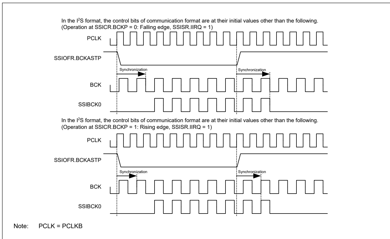
Figure 32.45 Example of stopping SSIBCK0 with SSIOFR.BCKASTP
