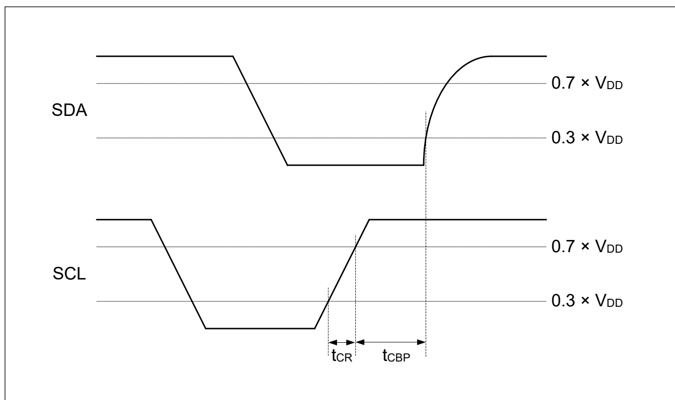
Figure 41.39 I3C STOP condition Timing
