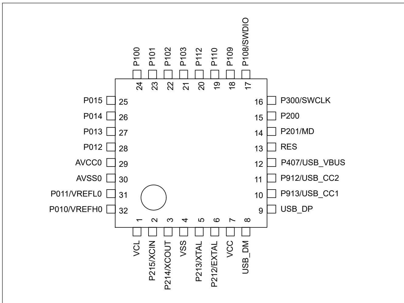
Figure 1.5 Pin assignment for LQFP/QFN 32-pin (top view)
