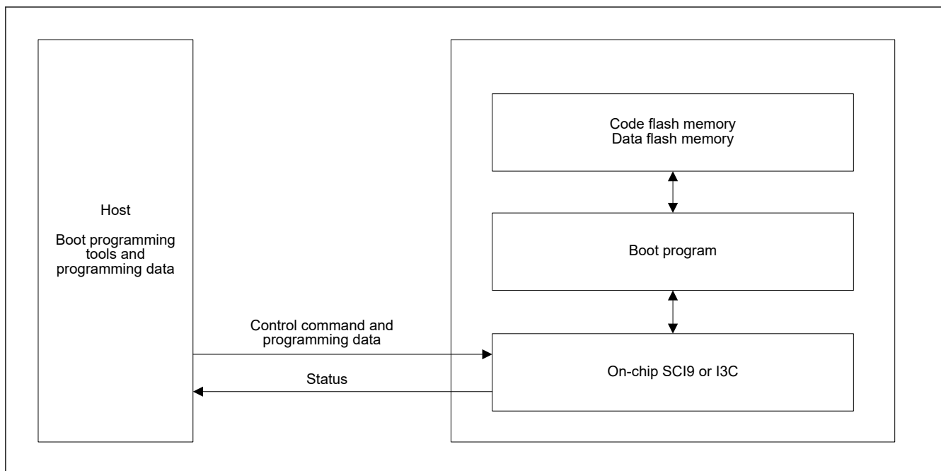
Figure 38.10 System configuration in SCI boot mode or IIC boot mode
