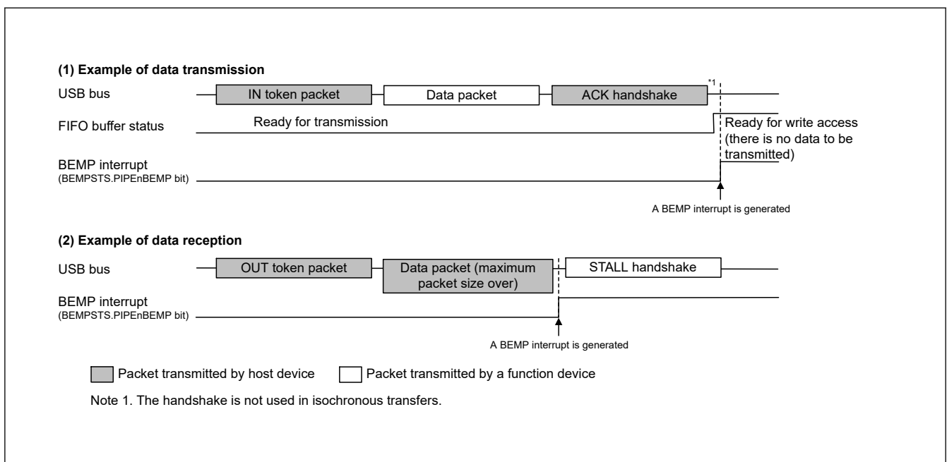
Figure 25.7 Timing of BEMP interrupt generation in device controller mode
