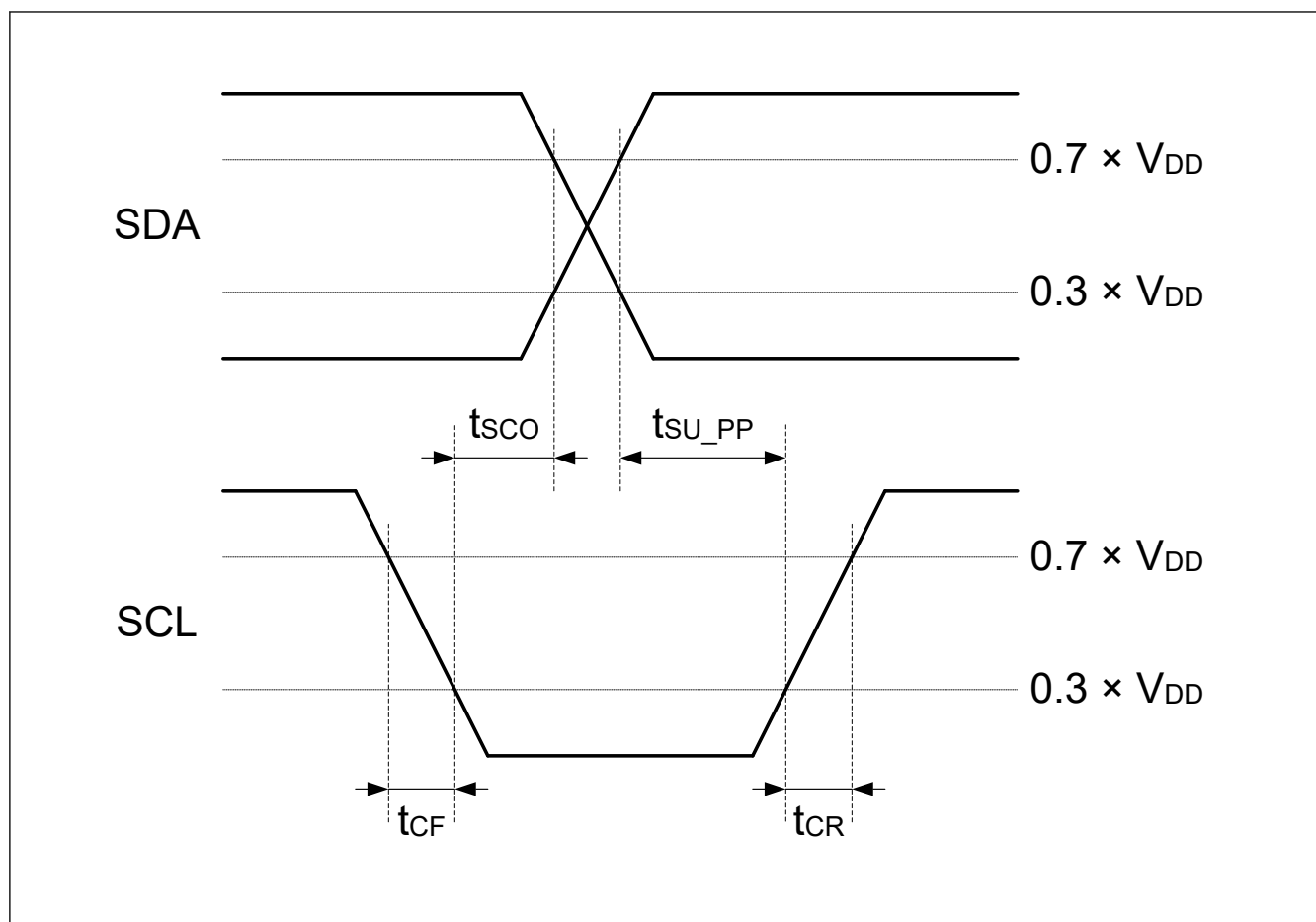
Figure 41.41 I3C Slave Out Timing
