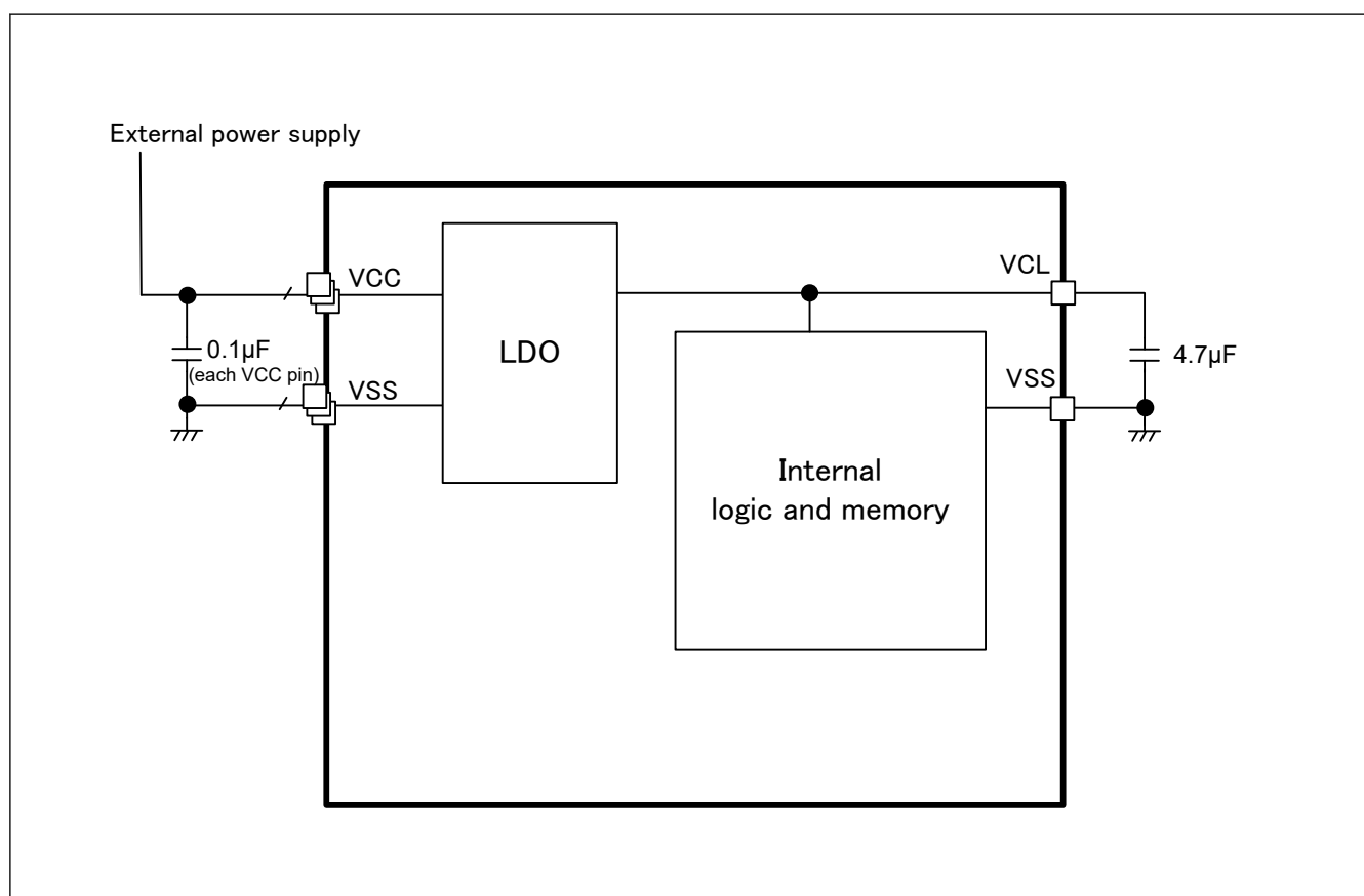
Figure 40.1 LDO settings
