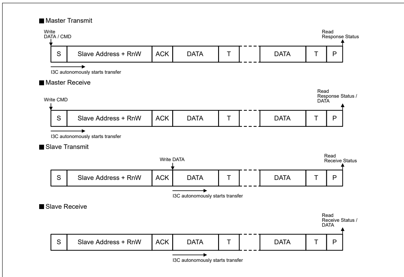
Figure 28.47 Data handler with normal FIFO buffer transfer
