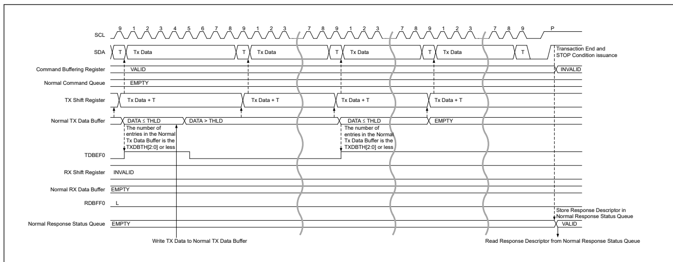
Figure 28.17 SDR data write transfer timing (2/2)
