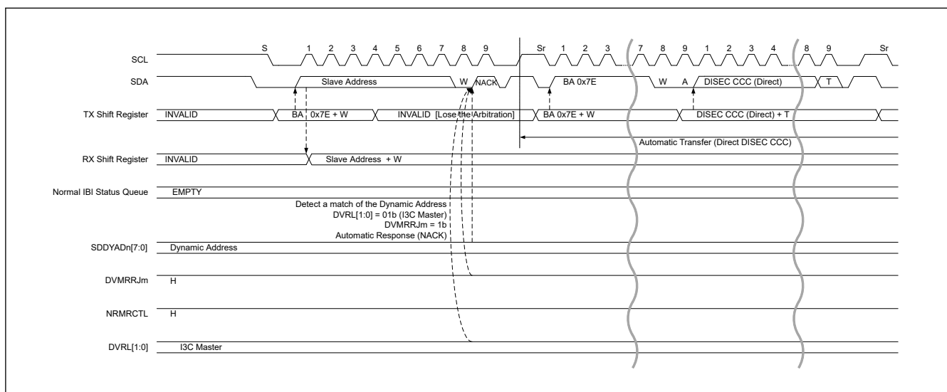
Figure 28.85 Mastership request : NACK (DVMRRJ = 1) and NRMRCTL = 1 (1/2)
