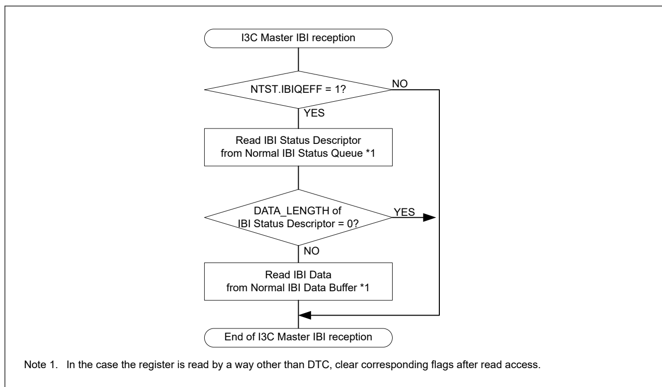
Figure 28.108 Example of I3C master IBI reception flowchart
