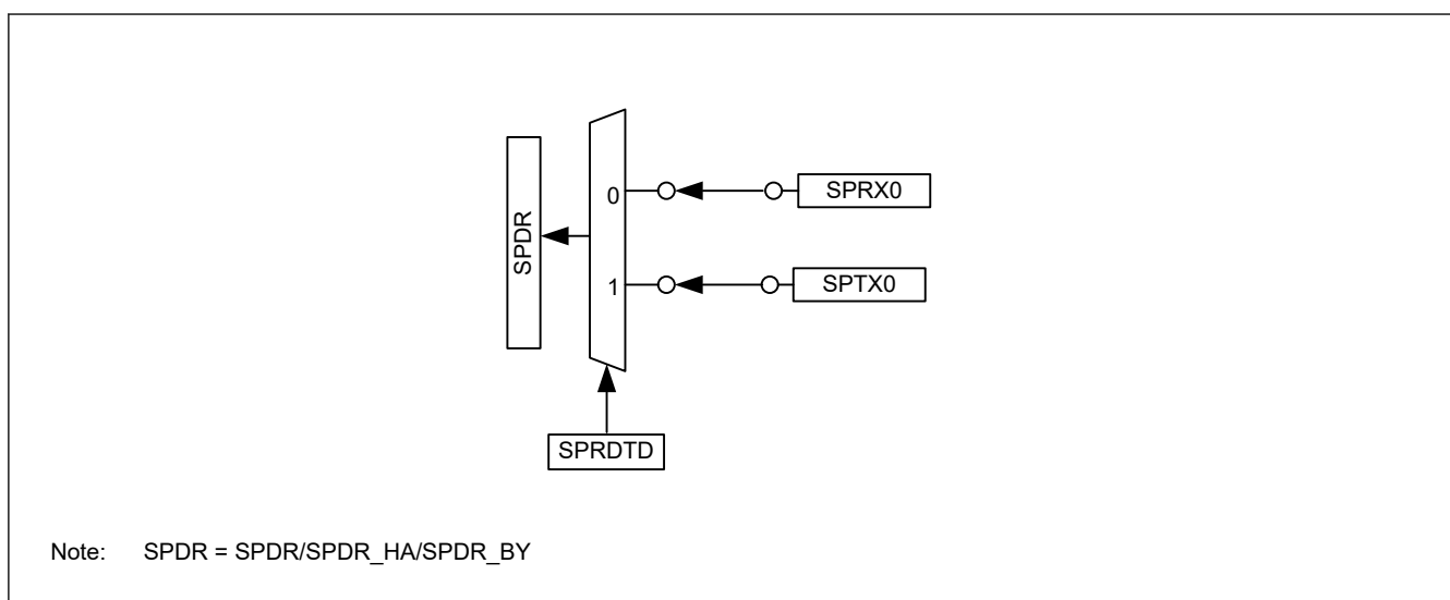
Figure 30.4 Configuration of SPDR/SPDR_HA/SPDR_BY for read access
