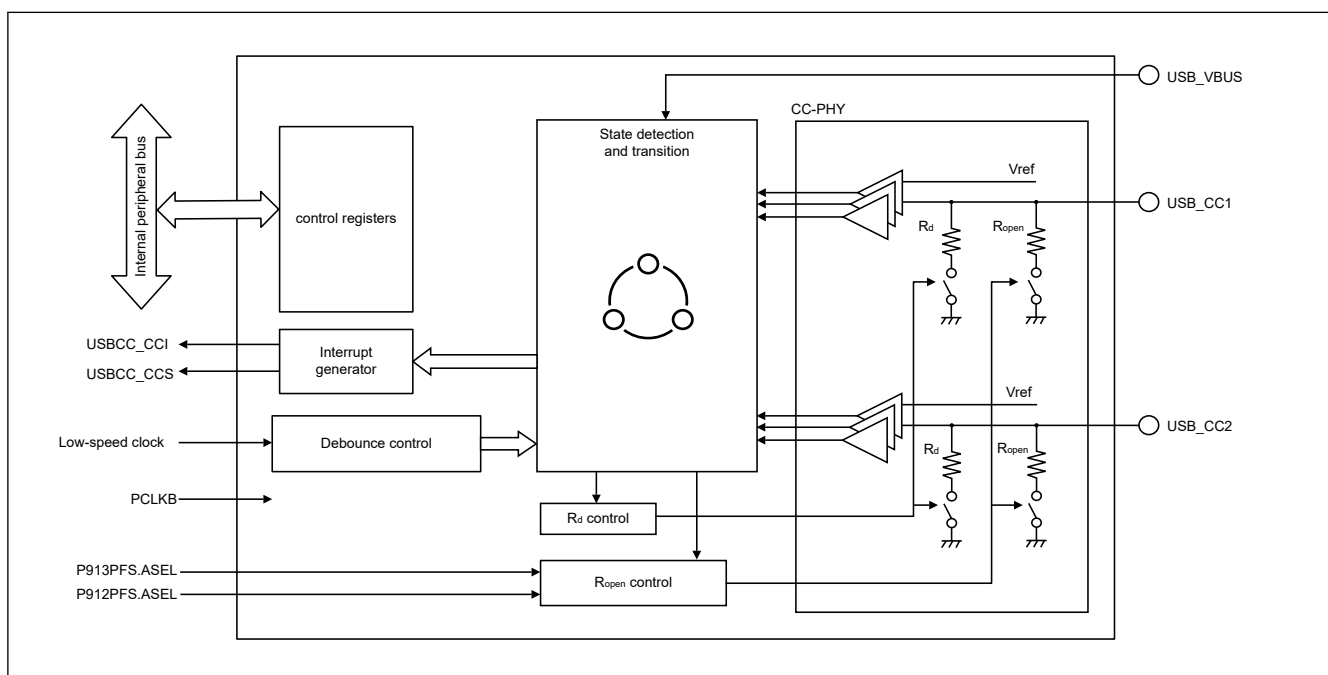
Figure 26.1 Block diagram for USB Type-C interface
