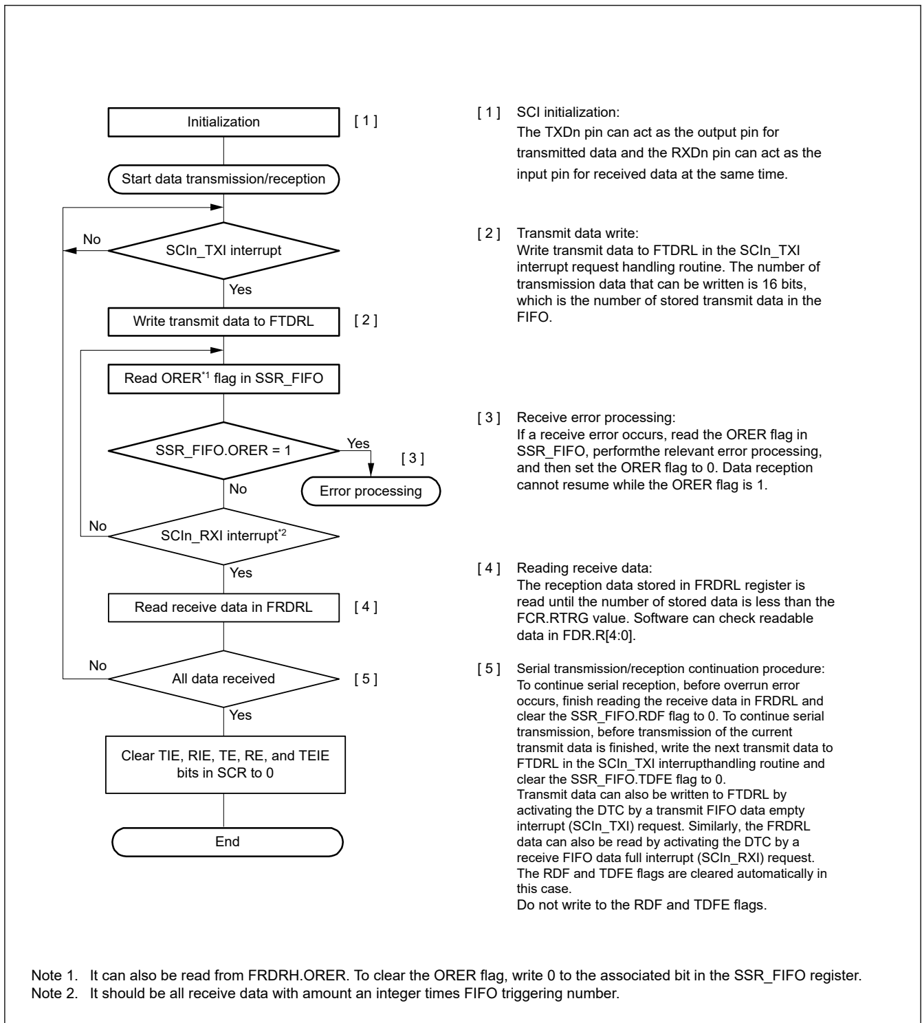
Figure 27.46 Example flow of simultaneous serial transmission and reception in clock synchronous mode with FIFO selected
