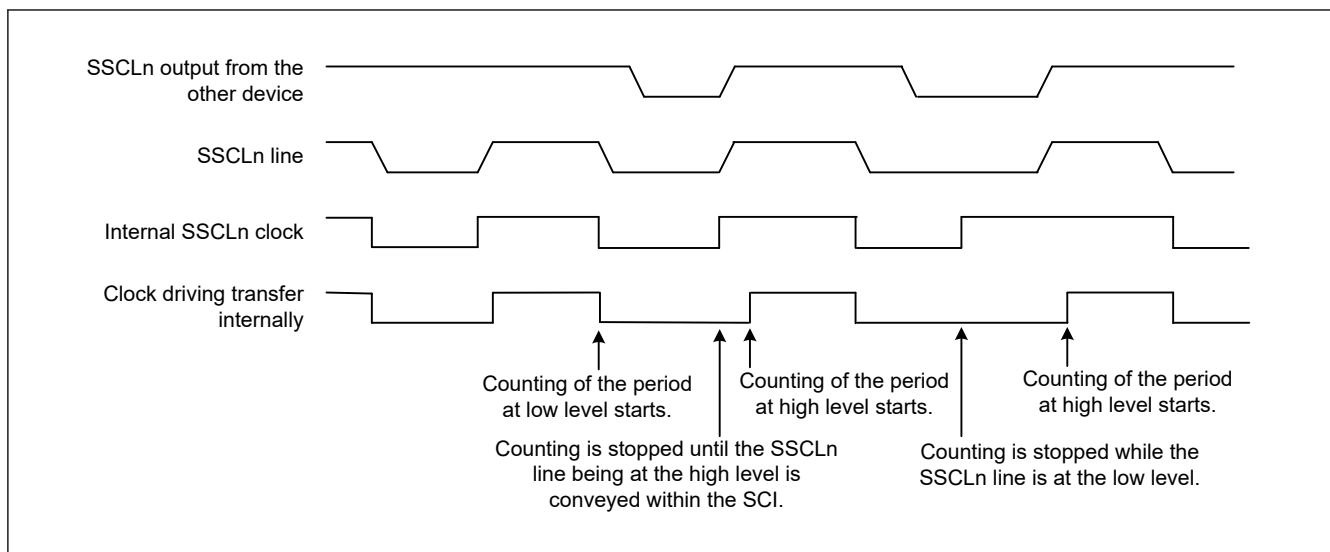
Figure 27.61 Example operations for clock synchronization
