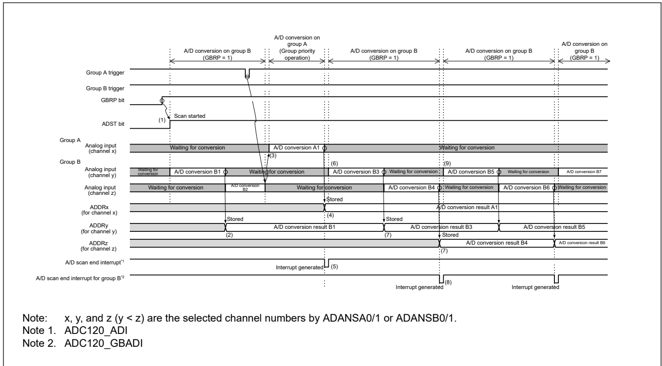
Figure 34.21 Group priority operation example 1-5: Continuously activating single scan for group B (when \text{ADGSPCR.GBRP} = 1 )
