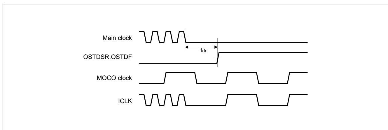
Figure 41.56 Oscillation stop detection timing
