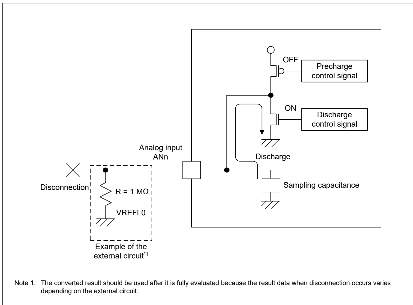
Figure 34.29 Example of disconnection detection when discharge is selected
