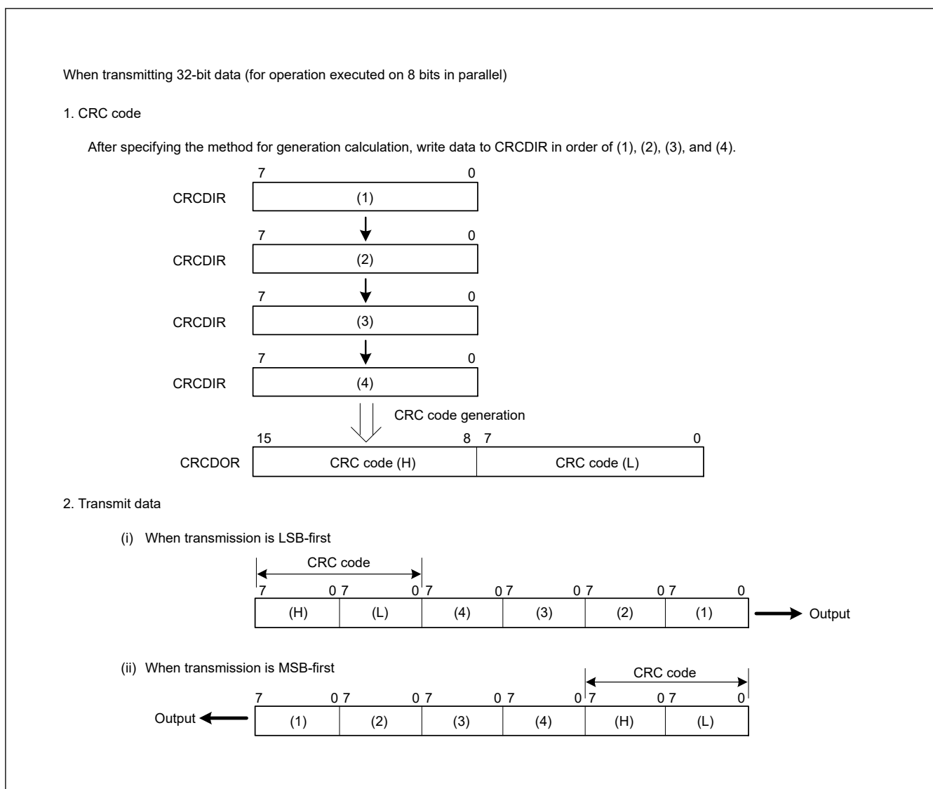
Figure 33.6 LSB-first and MSB-first data transmission
