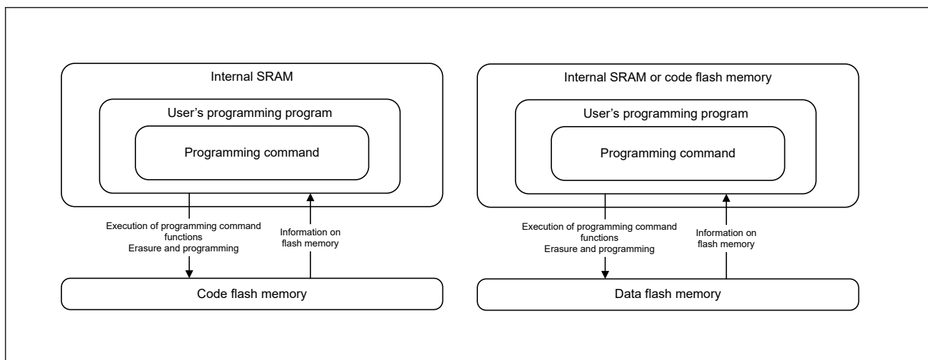
Figure 38.12 Schematic view of self-programming
