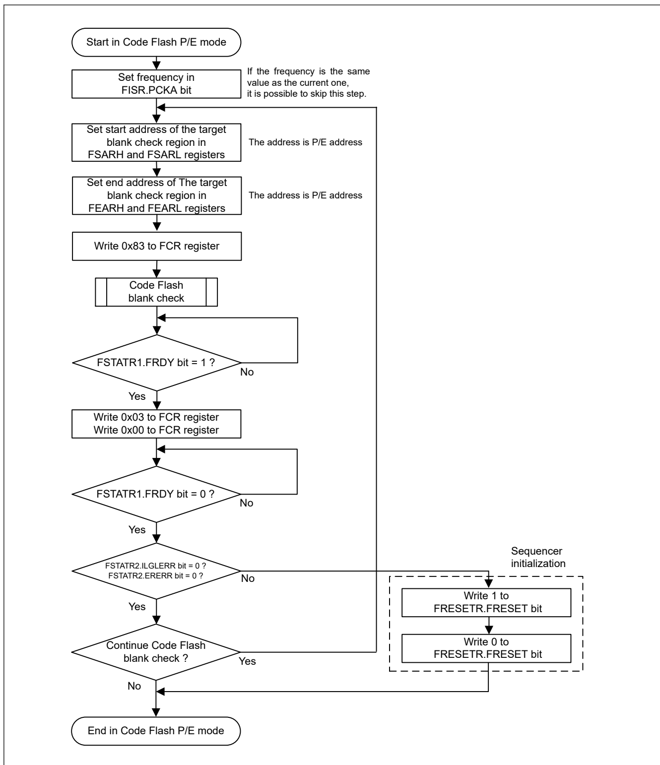
Figure 38.27 Flowchart for the code flash blank check procedure
