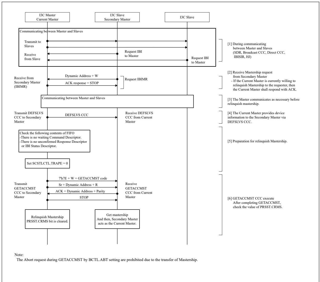
Figure 28.26 I3C Master Mastership processing flow
