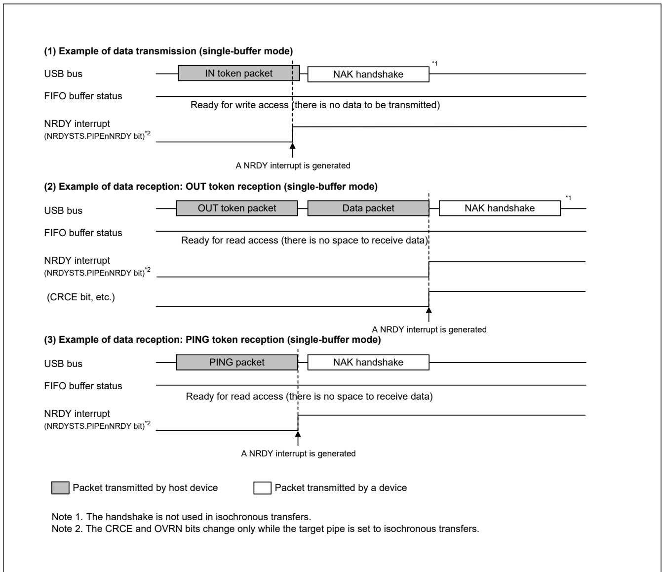
Figure 25.6 Timing of NRDY interrupt generation in device controller mode
