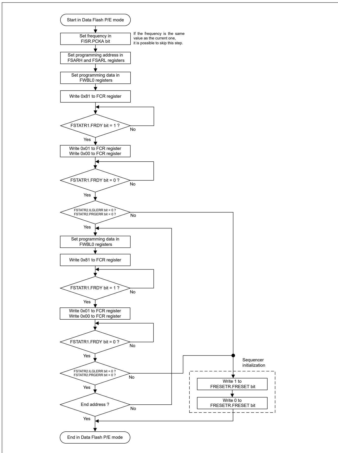
Figure 38.22 Flowchart for consecutive programming of the data flash
