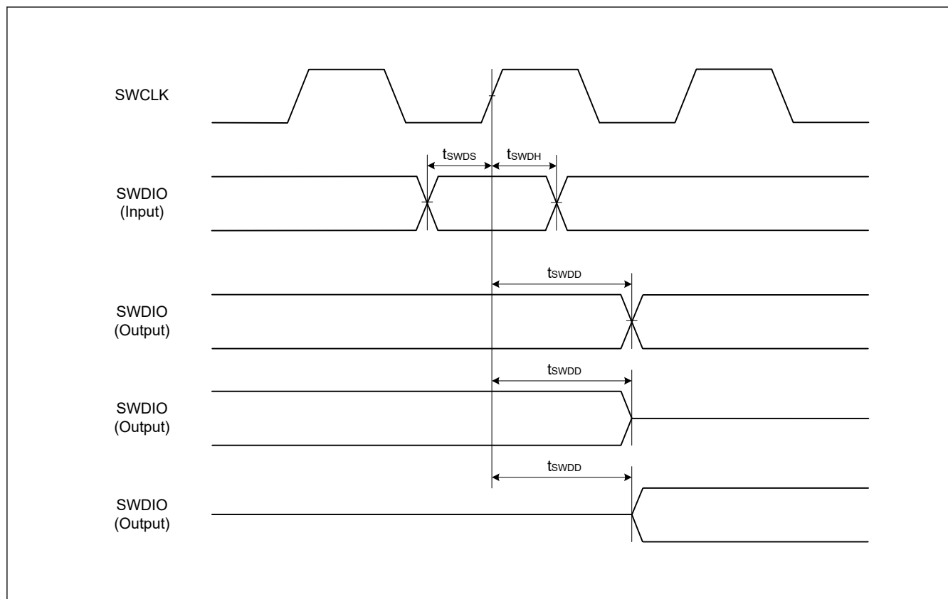
Figure 41.63 SWD input/output timing
