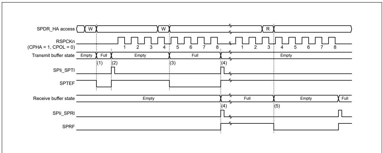
Figure 30.27 Operation example of the SPI_SPTI and SPI_SPRI interrupts when CPHA = 1 and CPOL = 0 in master mode
