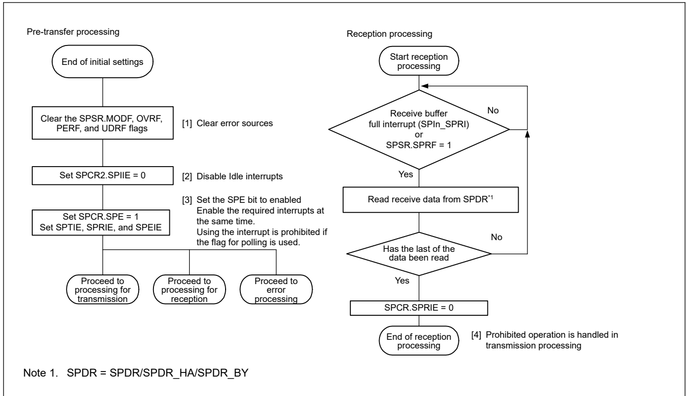
Figure 30.34 Reception flow in master mode
