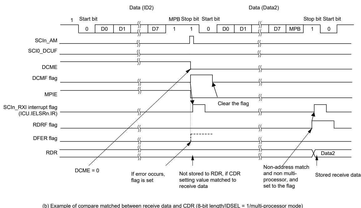
Figure 27.6 Example of address match (2) multi-processor mode
