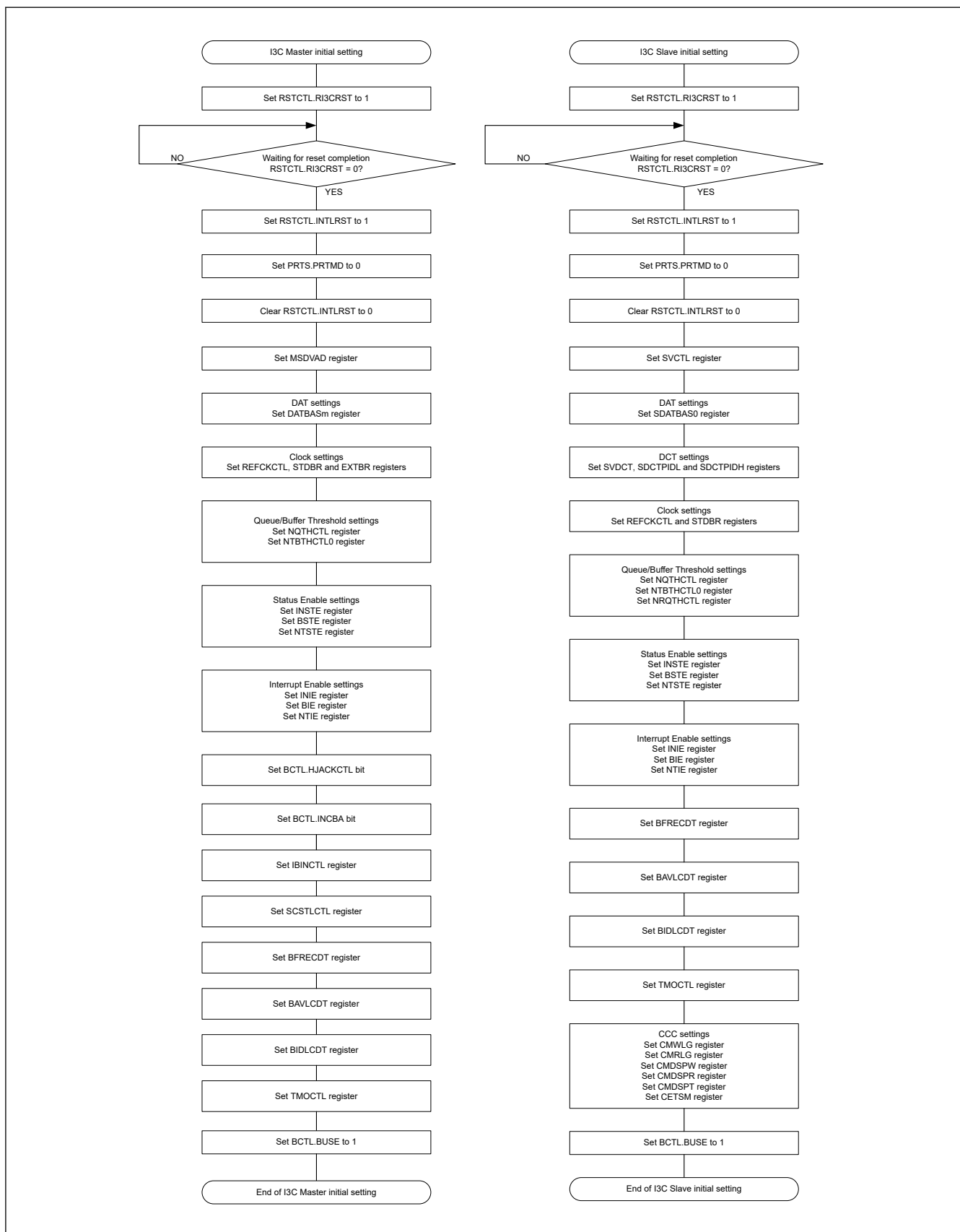
Figure 28.101 Example of I3C initialization flowchart
