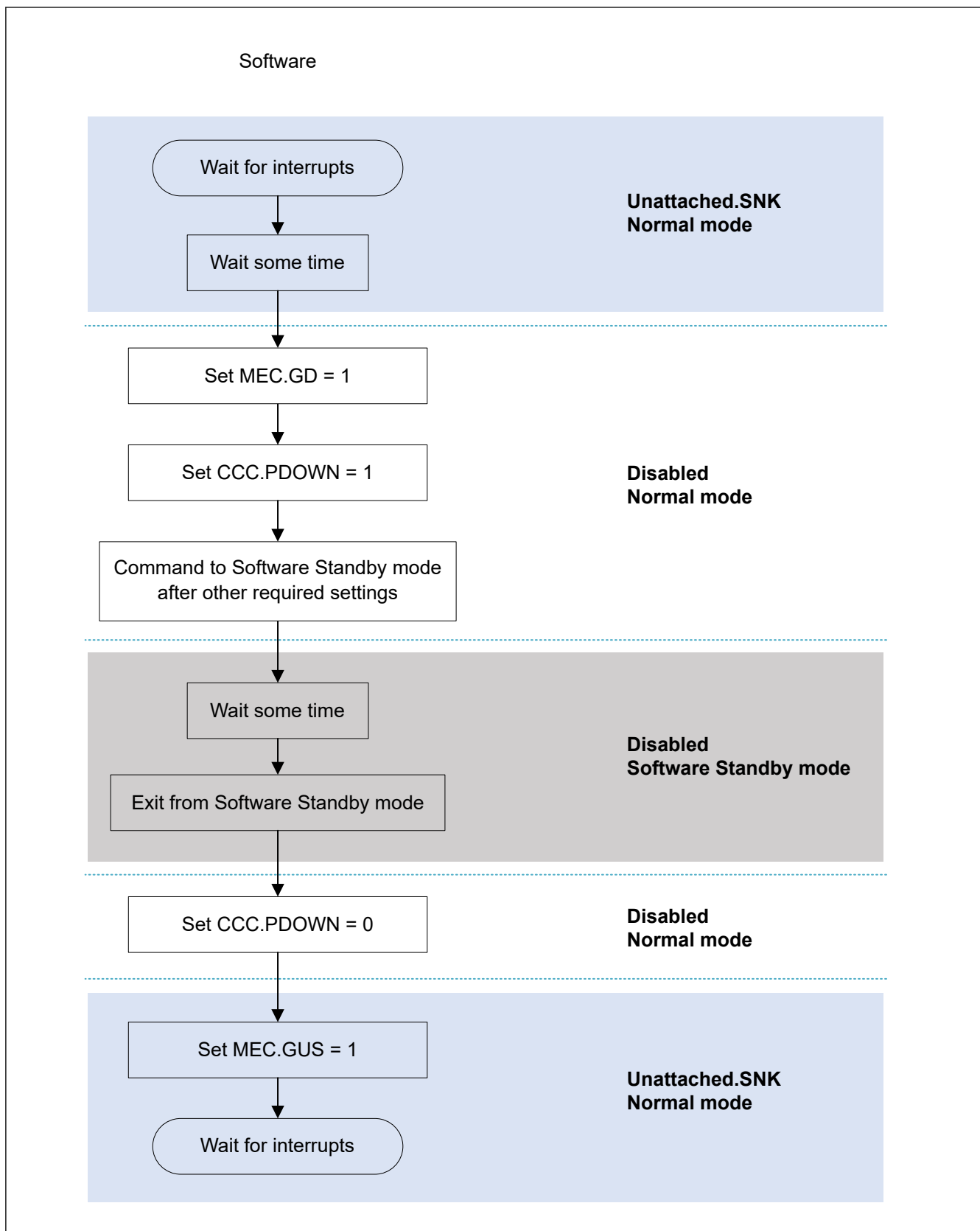
Figure 26.6 Sink-only mode Software Standby mode entry and exit flow
