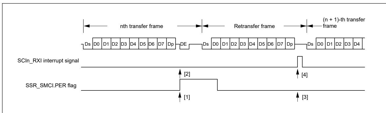
Figure 27.55 Data re-transfer operation in smart card interface reception mode
