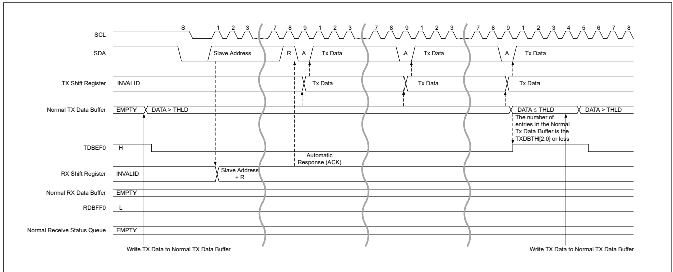
Figure 28.41 Legacy I 2 C message data read transfer timing (1/2)
