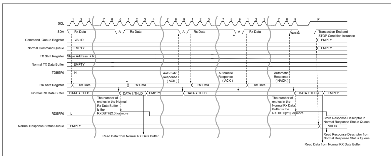
Figure 28.21 SDR data read transfer timing (2/2)
