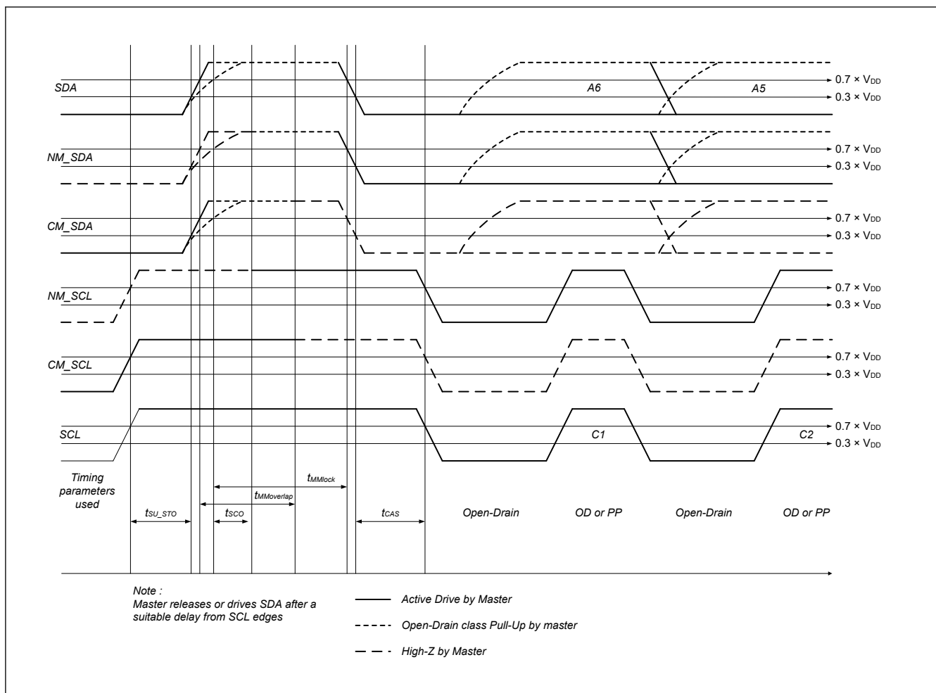
Figure 41.44 I3C Timing
