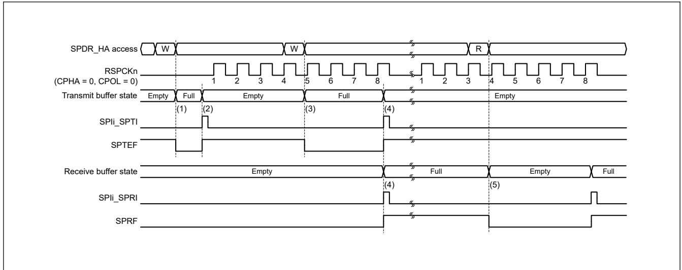
Figure 30.26 Operation example of the SPli_SPTI and SPli_SPRI interrupts when CPHA = 0 and CPOL = 0 in master mode
