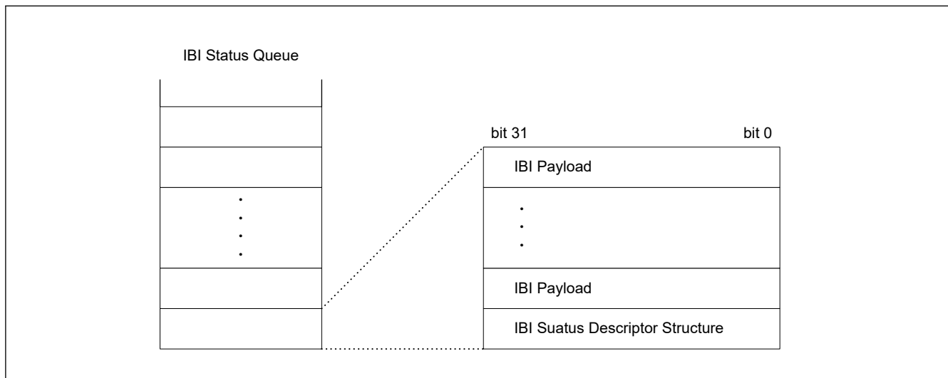
Figure 28.4 IBI status descriptor data structure
