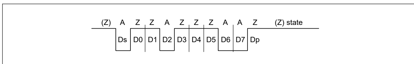
Figure 27.49 Direct convention with SDIR in SCMR = 0, SINV in SCMR = 0, and PM in SMR_SMCI = 0
