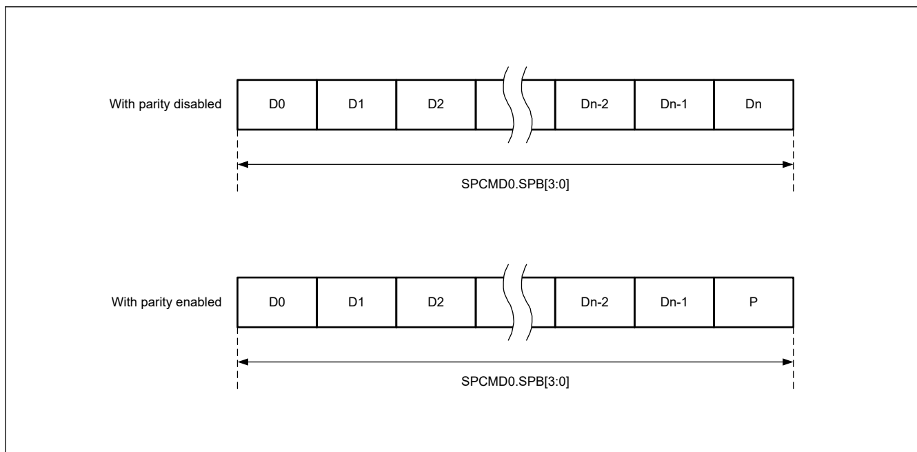
Figure 30.13 Data format with parity disabled and enabled
