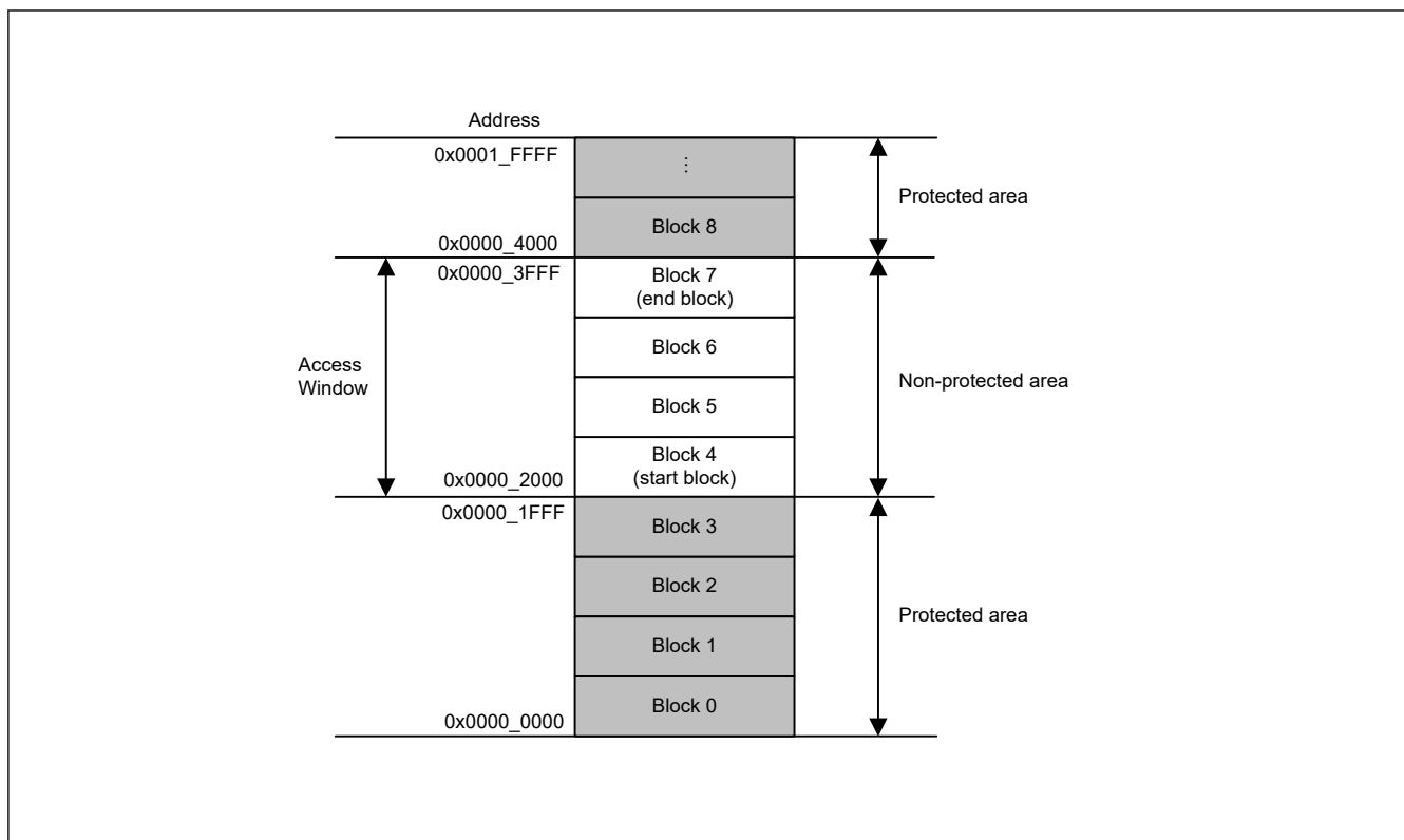
Figure 38.7 Flash area protection overview
