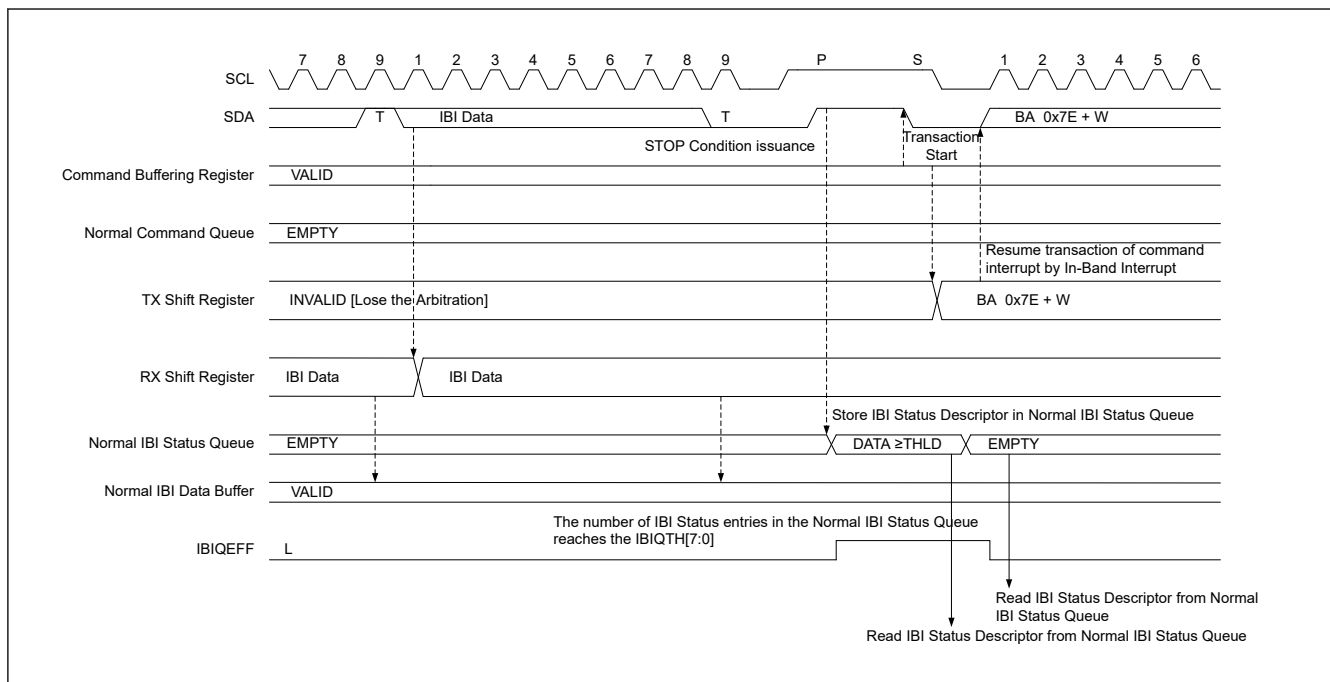
Figure 28.25 I3C master IBI transfer timing (2/2)
