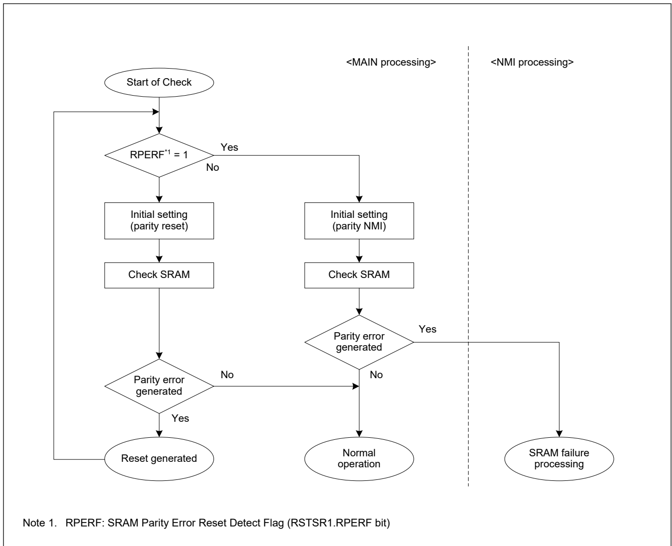
Figure 37.1 Flow of SRAM parity check when SRAM parity reset is enabled
