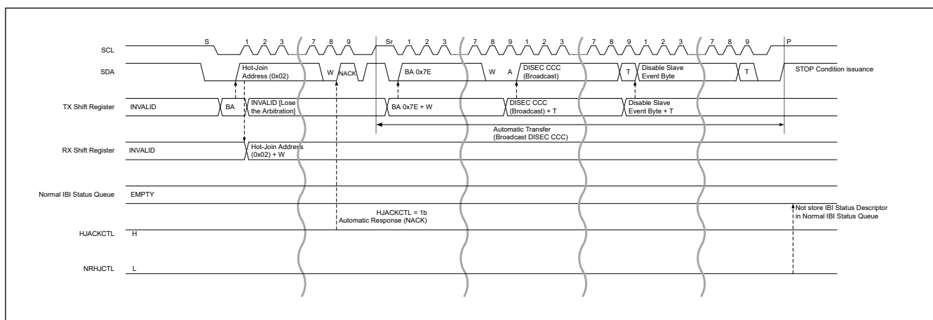
Figure 28.88 Hot-join event : NACK (HJACKCTL = 1) and NRHJCTL = 0
