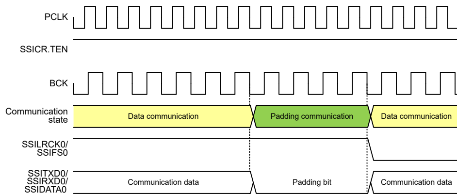
Figure 32.49 Transition from data communication to padding communication
