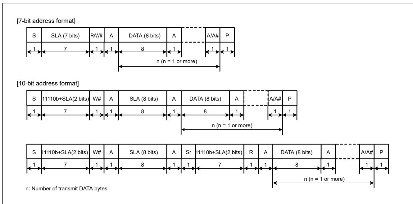
Figure 28.48 I 2 C bus format
