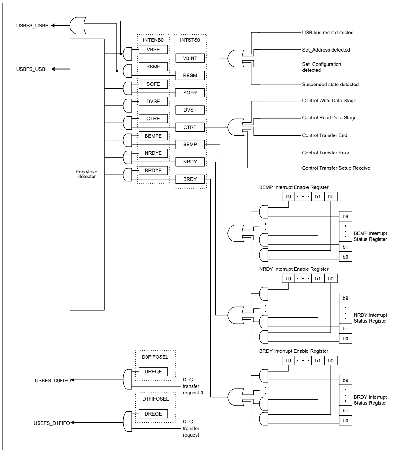
Figure 25.4 USBFS interrupt-related circuits
