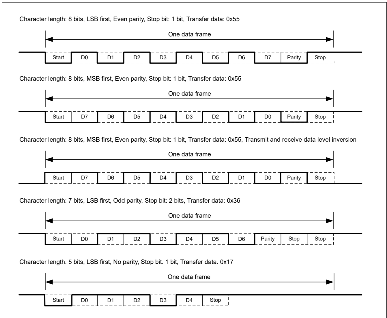
Figure 31.3 Example of transmit and receive data waveform
