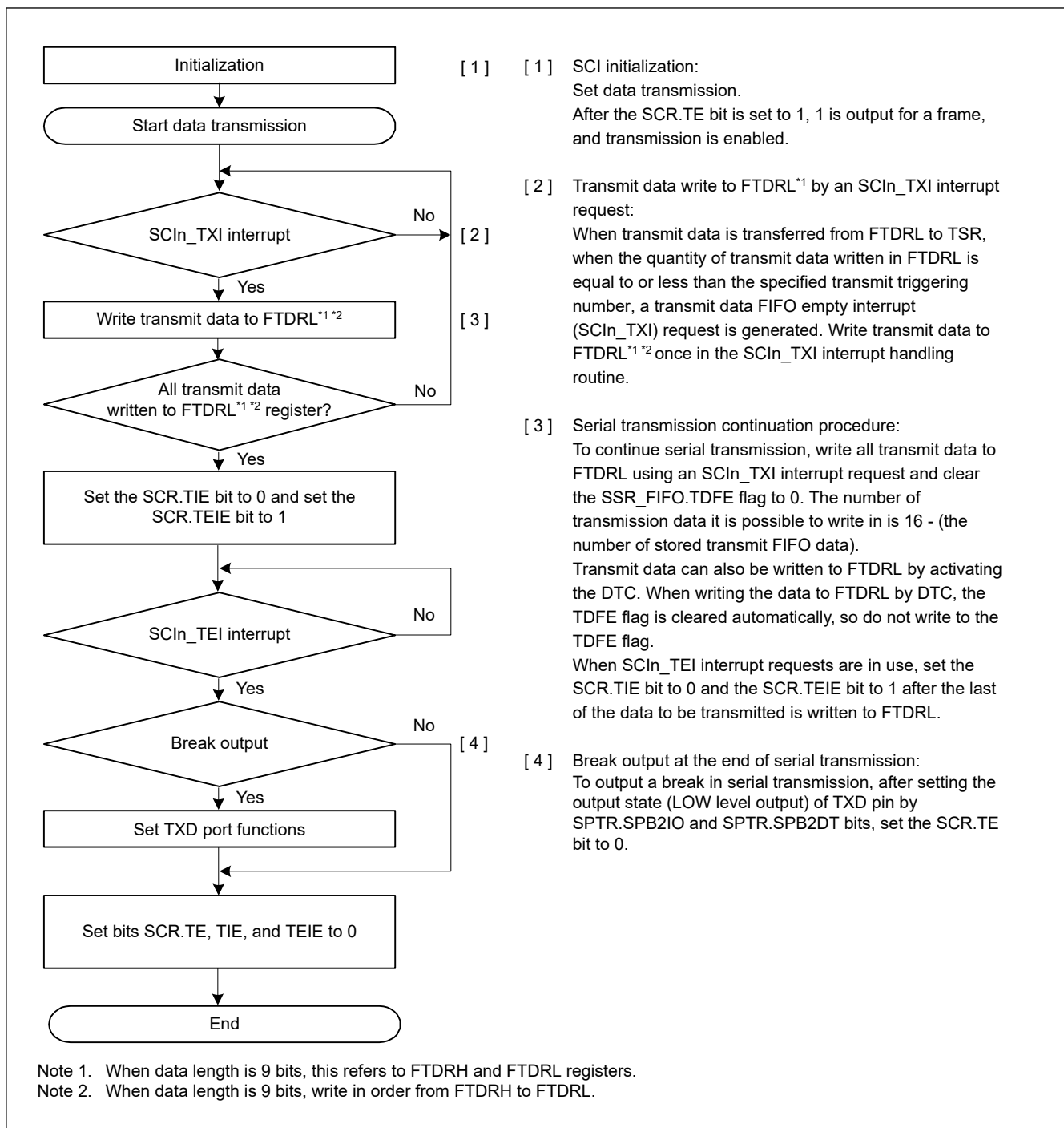
Figure 27.12 Example flow of serial transmission in asynchronous mode with FIFO selected
