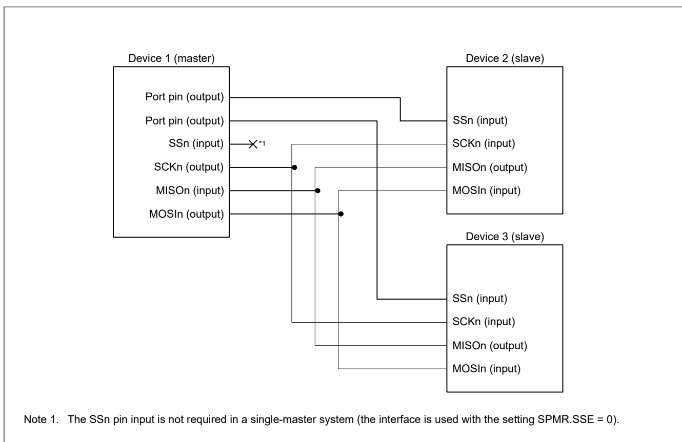
Figure 27.68 Example connections using simple SPI mode in single master mode with SPMR.SSE bit = 0
