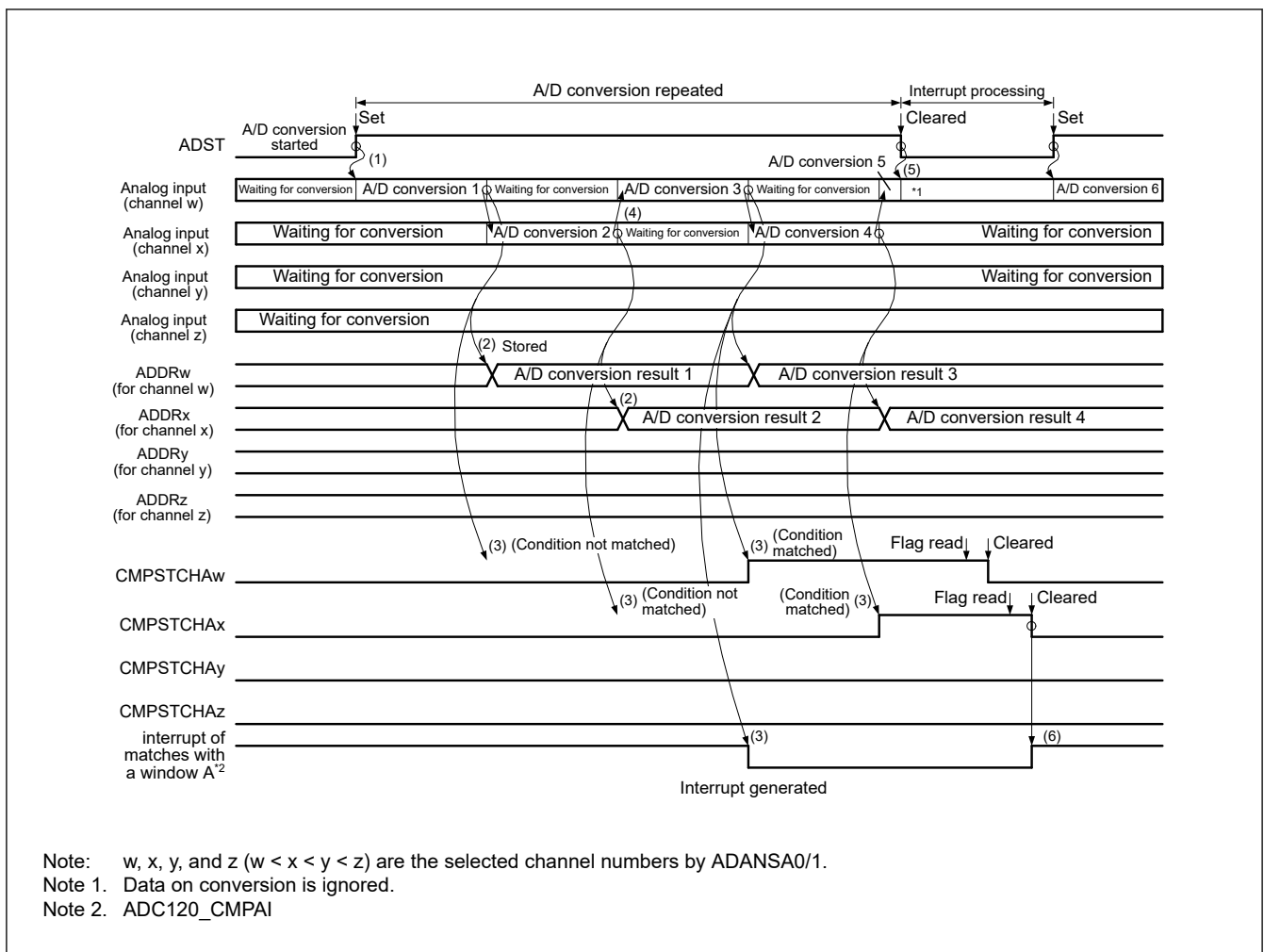
Figure 34.22 Example of compare function operation, when the analog inputs (channel w to z) are compared
