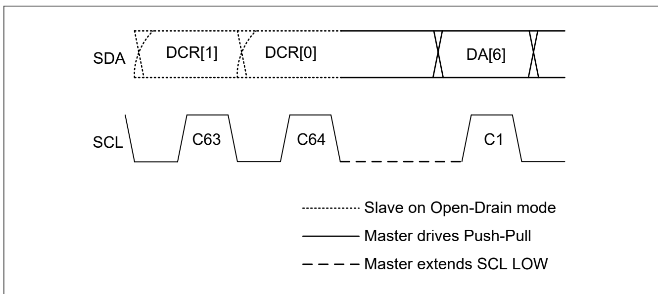
Figure 28.76 Master clock stalling in dynamic address first bit
