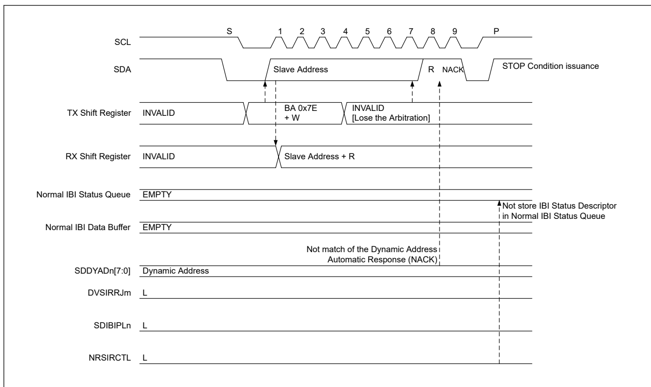
Figure 28.79 Slave interrupt request : NACK (not match the SDDYAD[7:0] of DAT) and NRSIRCTL = 0
