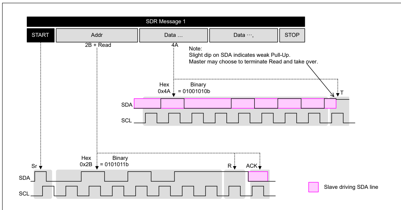
Figure 28.51 Example communication using I3C coding SDR without broadcast (0x7E)
