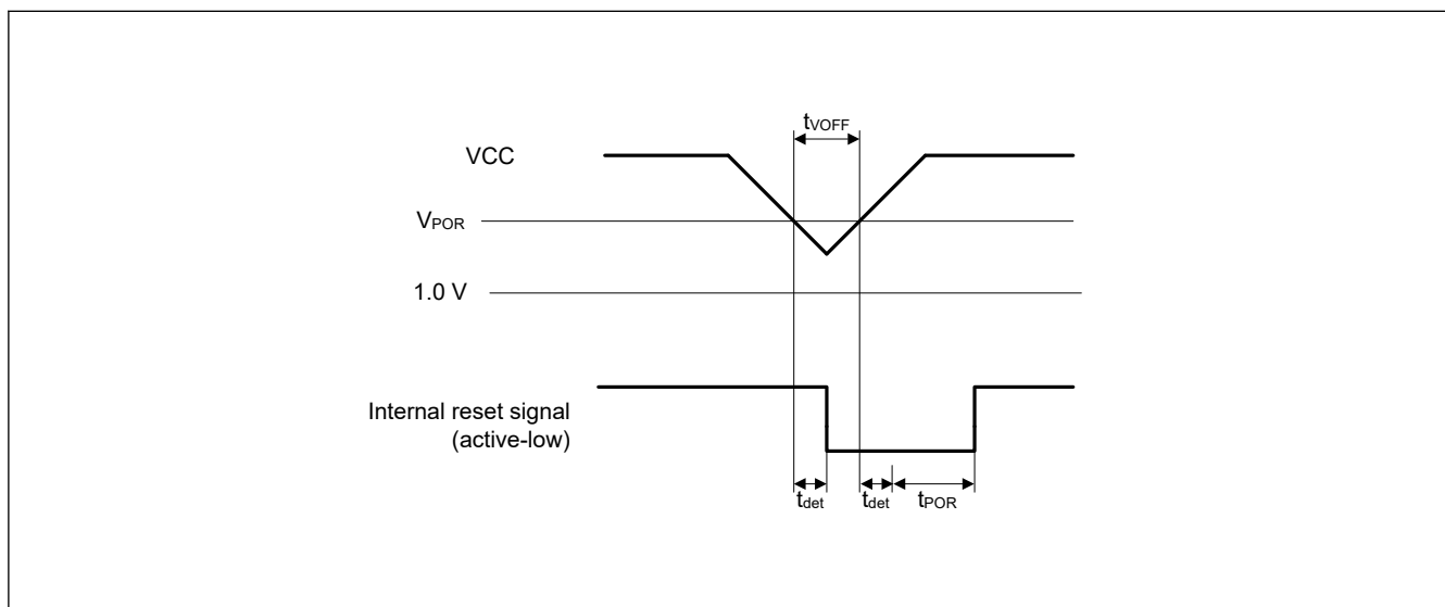
Figure 41.57 Voltage detection reset timing
