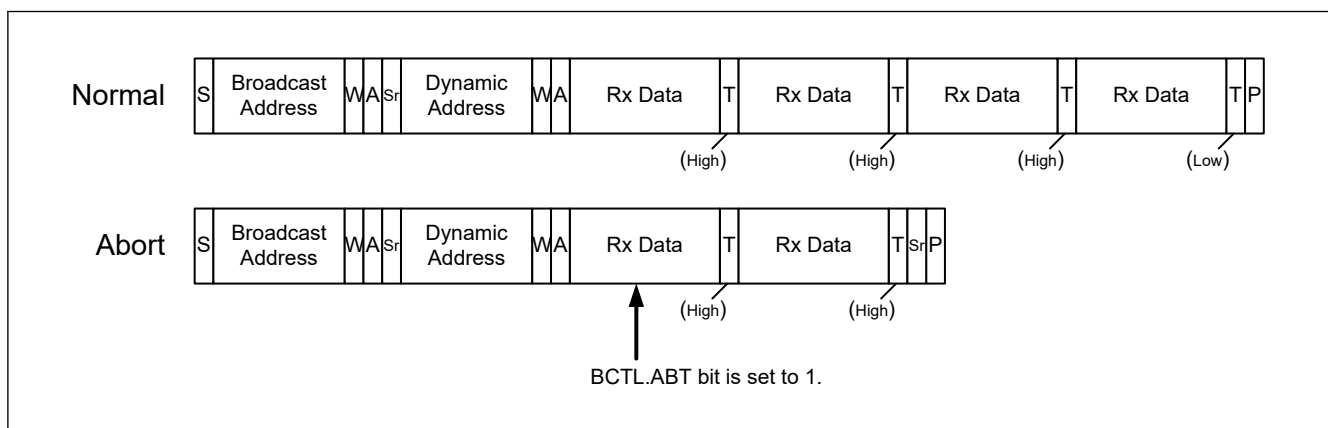
Figure 28.94 Abort operation of SDR read transfer
