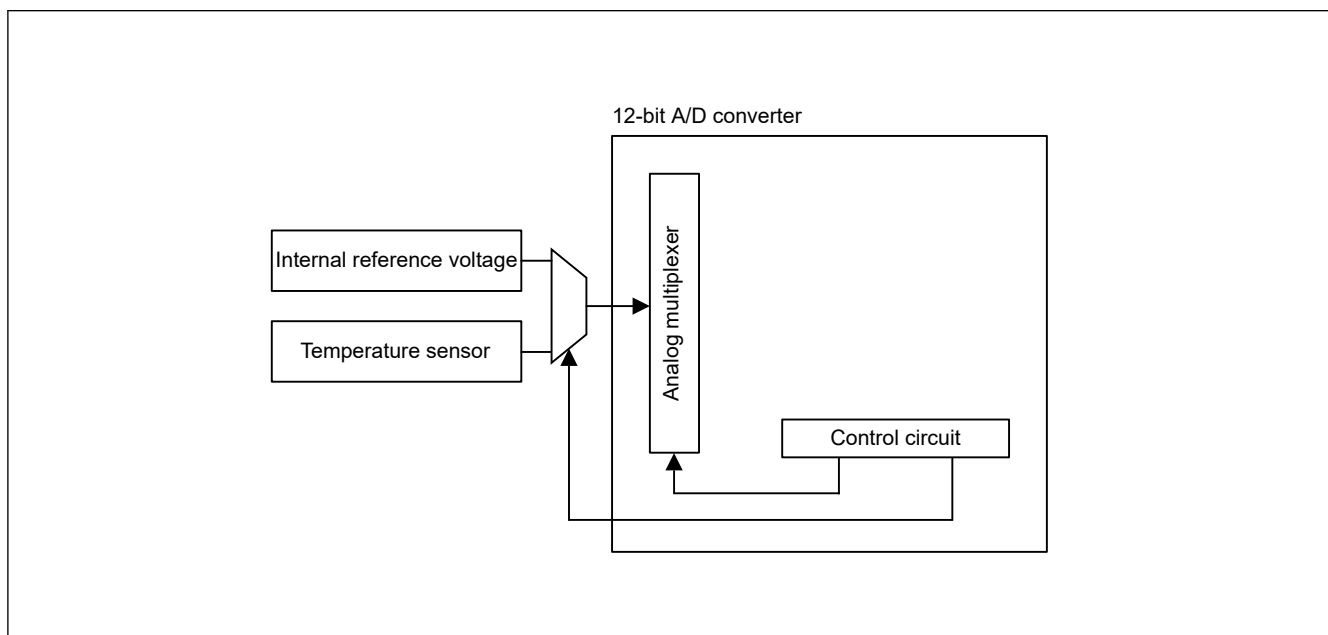
Figure 35.1 TSN block diagram
