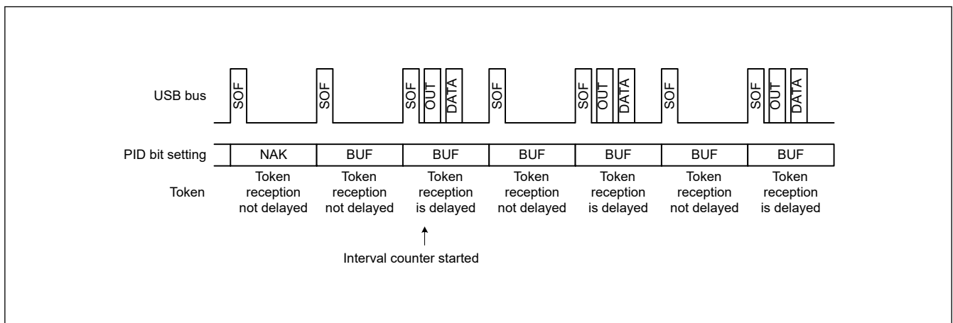
Figure 25.11 Relationship between frames and expected token reception when IITV[2:0] \neq 0
