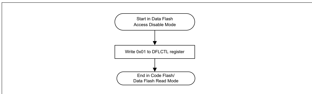
Figure 38.14 Mode transitions to read mode from data flash access disable mode
