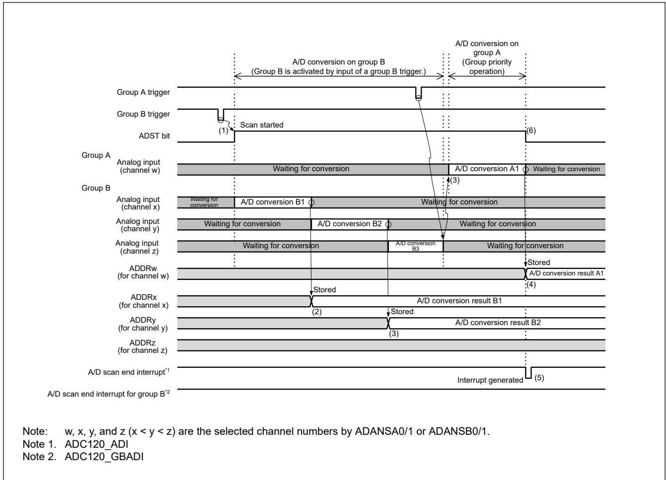
Figure 34.20 Group priority operation example 1-4: “Group A trigger is input during group B scan” when rescanning is disabled (when ADGSPCR.GBRSCN = 0, ADGSPCR.GBRP = 0)
