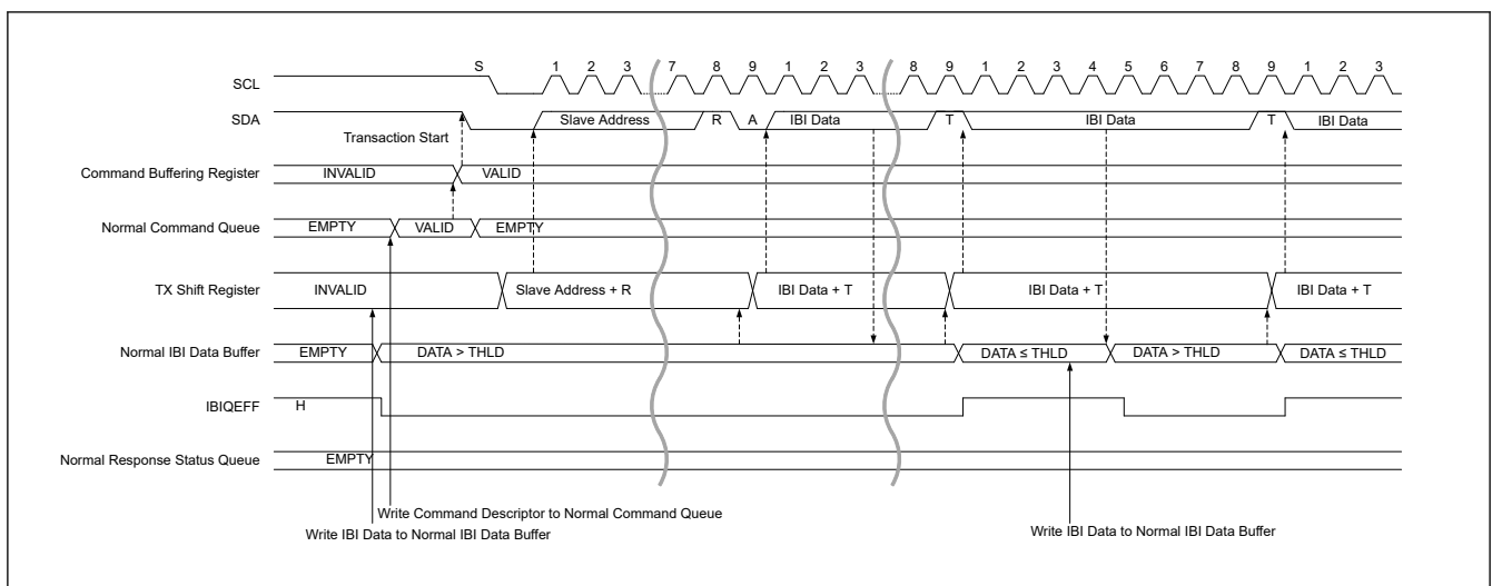
Figure 28.43 I3C slave IBI transfer timing (1/2)
