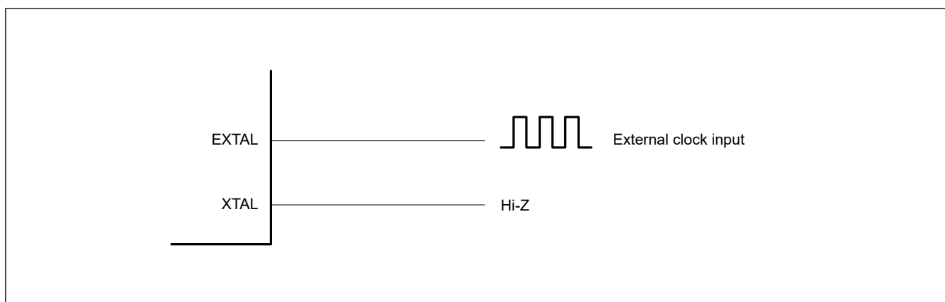
Figure 8.7 Equivalent circuit for external clock
