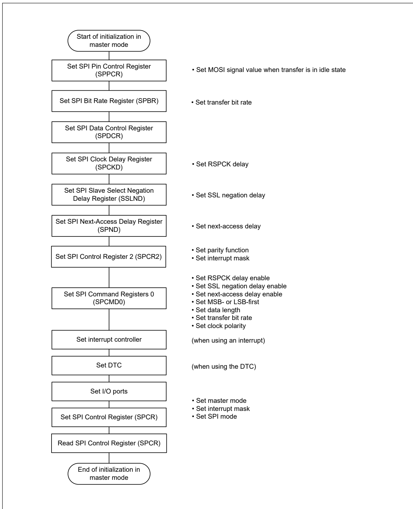
Figure 30.40 Example of initialization flow in master mode for clock synchronous operation
