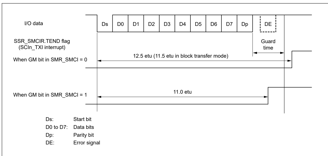
Figure 27.53 SSR.TEND flag generation timing during transmission
