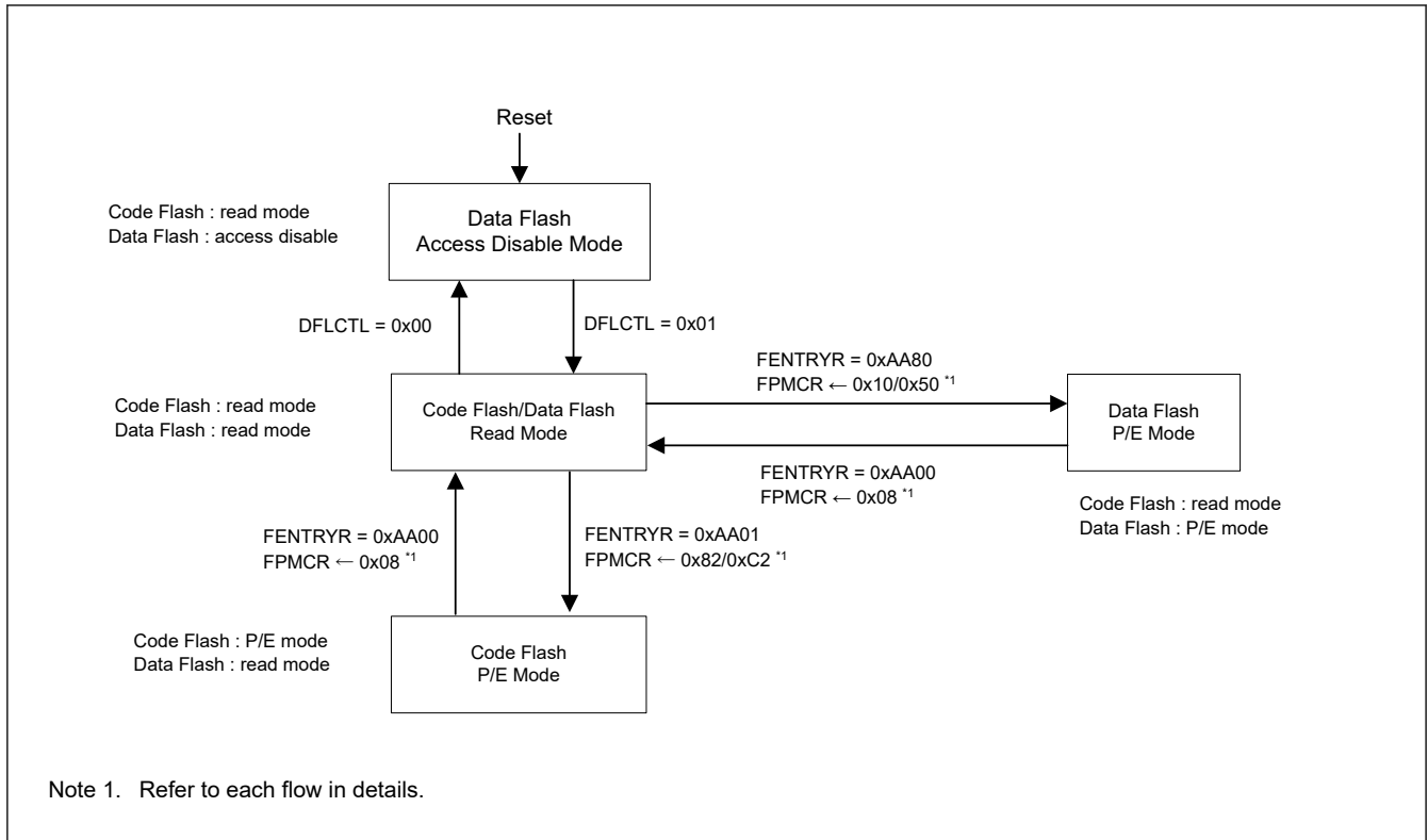
Figure 38.13 Mode transitions of the flash memory
