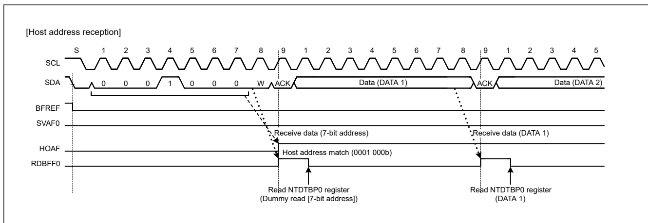
Figure 28.62 HOAF flag set timing during reception of host address
