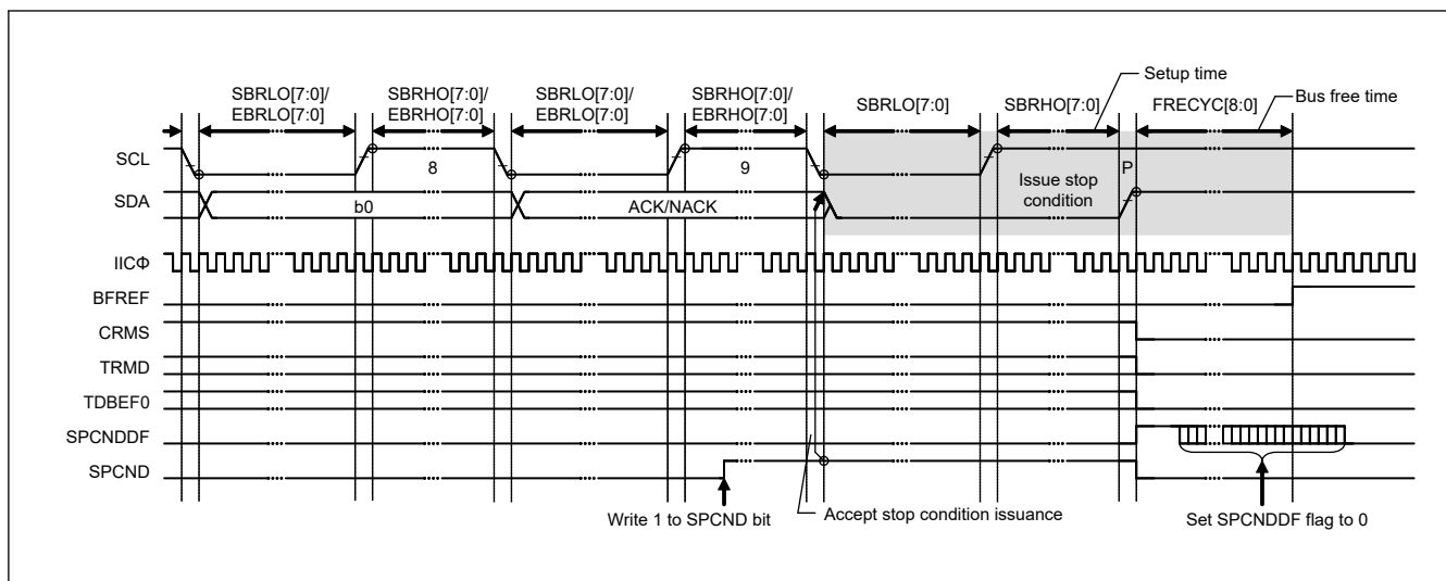
Figure 28.57 STOP condition issue timing (SPCND bit)
