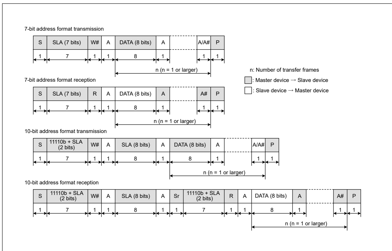
Figure 27.58 I 2 C bus format
