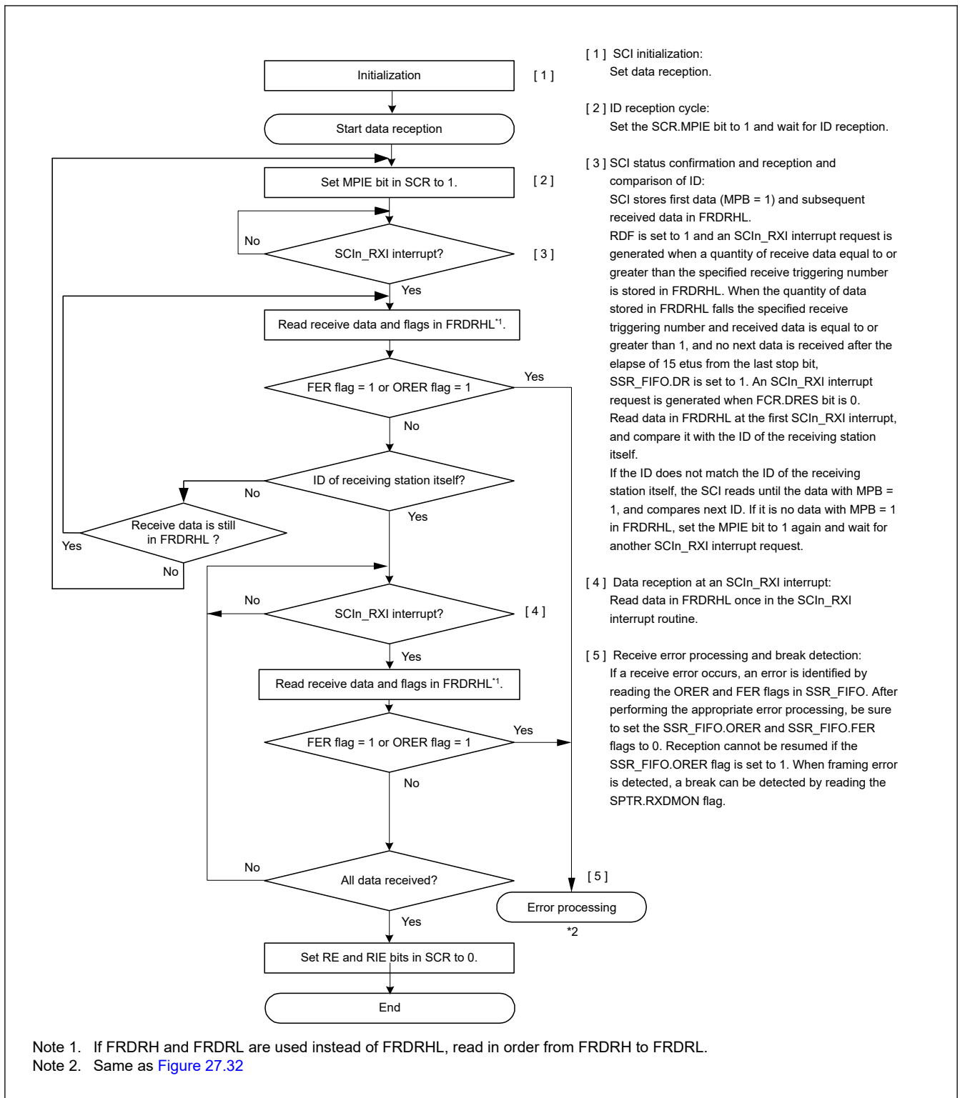
Figure 27.34 Example flow of serial reception in multi-processor mode with FIFO selected
