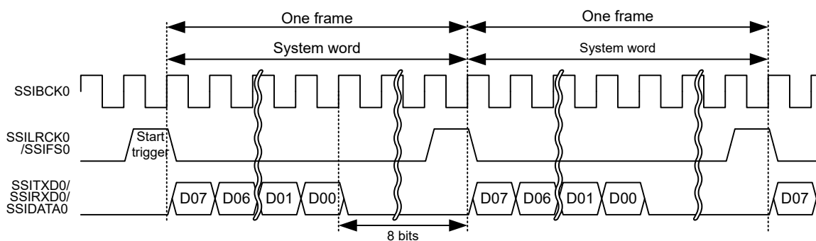
Figure 32.39 Short frame in monaural format (with padding: system word length > data word length)
