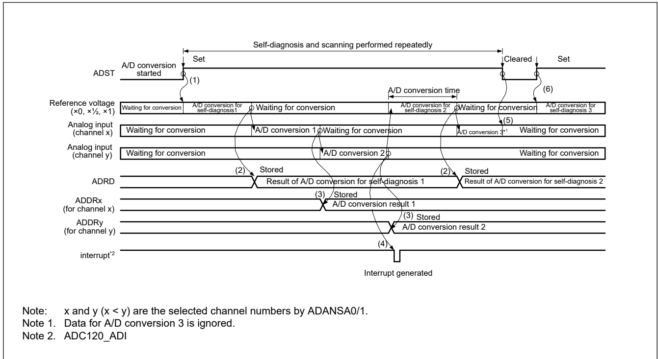
Figure 34.13 Example basic operation in continuous scan mode when the analog inputs (channel x and y) are selected with self-diagnosis
