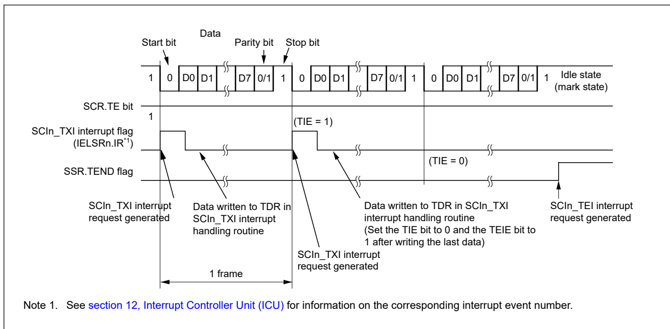
Figure 27.9 Example operation for serial transmission in asynchronous mode (3) with 8-bit data, parity bit, one stop bit, CTS function not used, and from the middle of transmission until transmission completion
