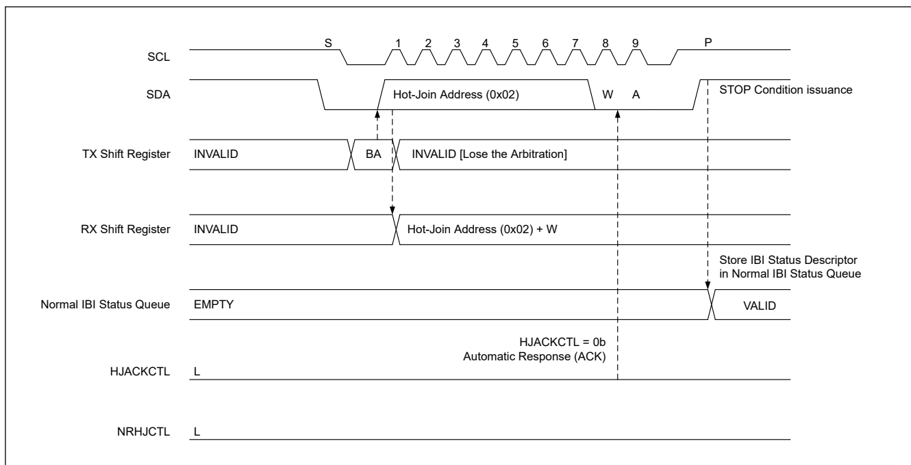
Figure 28.87 Hot-join event : ACK
