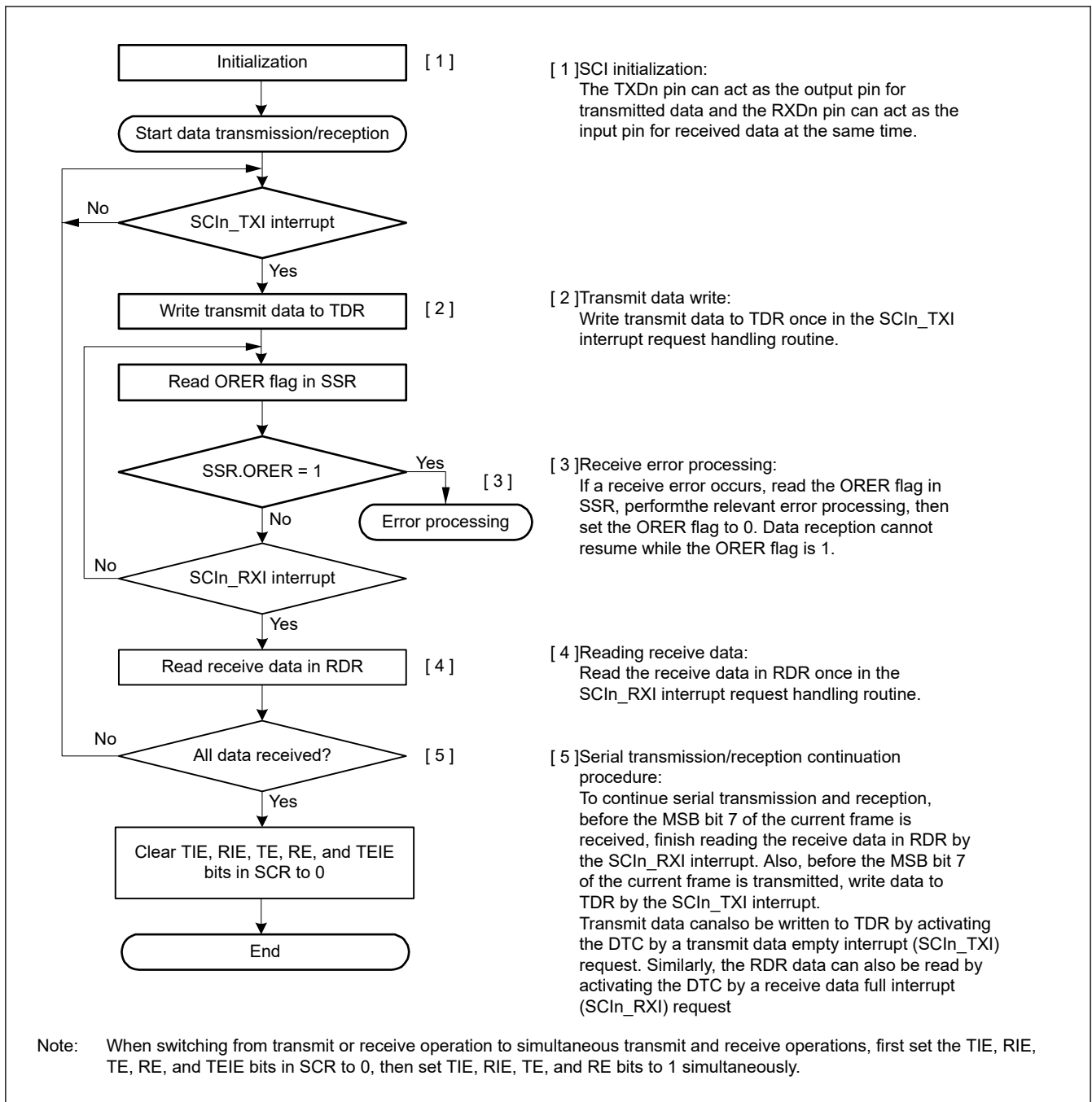
Figure 27.45 Example flow of simultaneous serial transmission and reception in clock synchronous mode with non-FIFO selected
