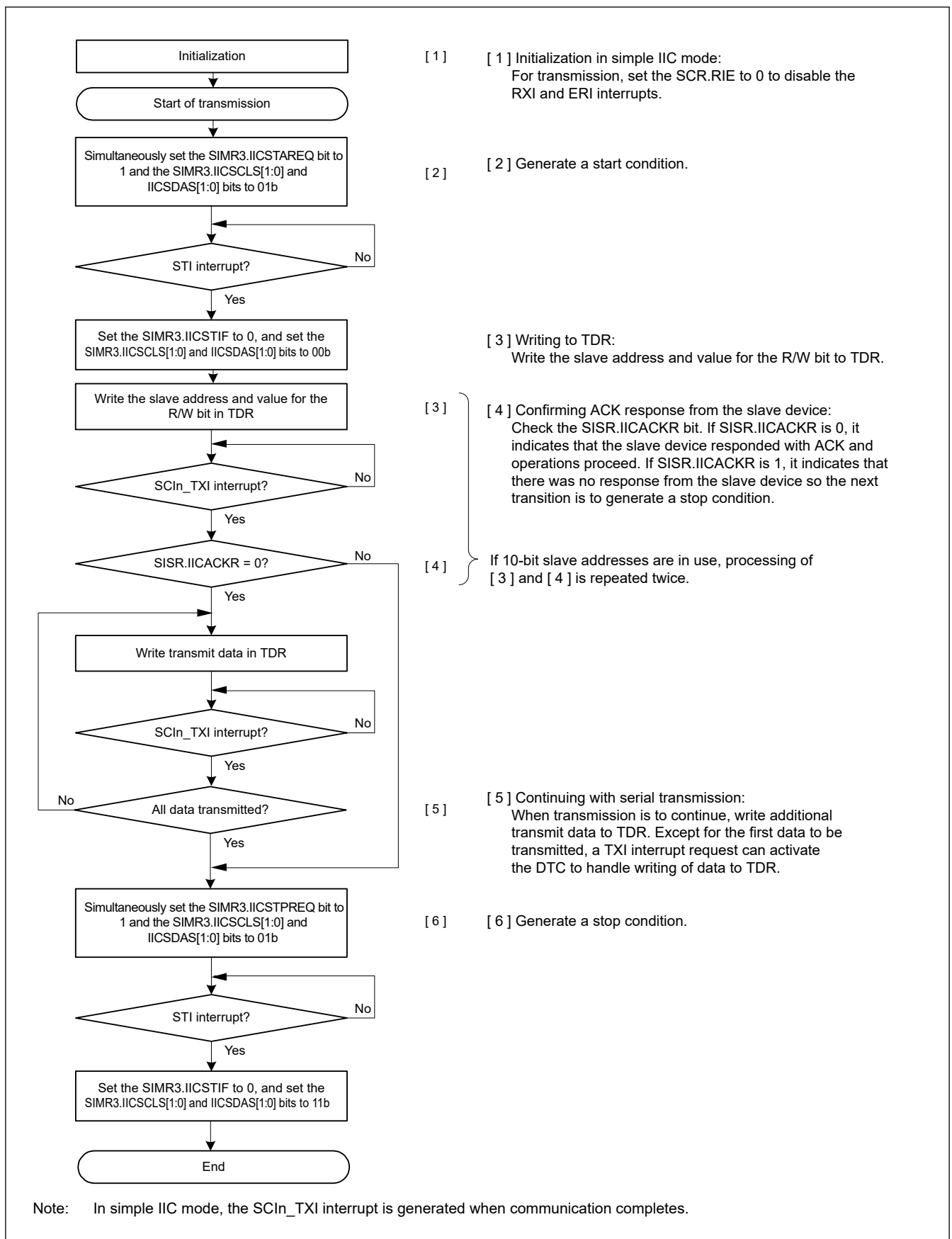
Figure 27.65 Example flow of master transmission in simple IIC mode with transmission interrupts and reception interrupts
