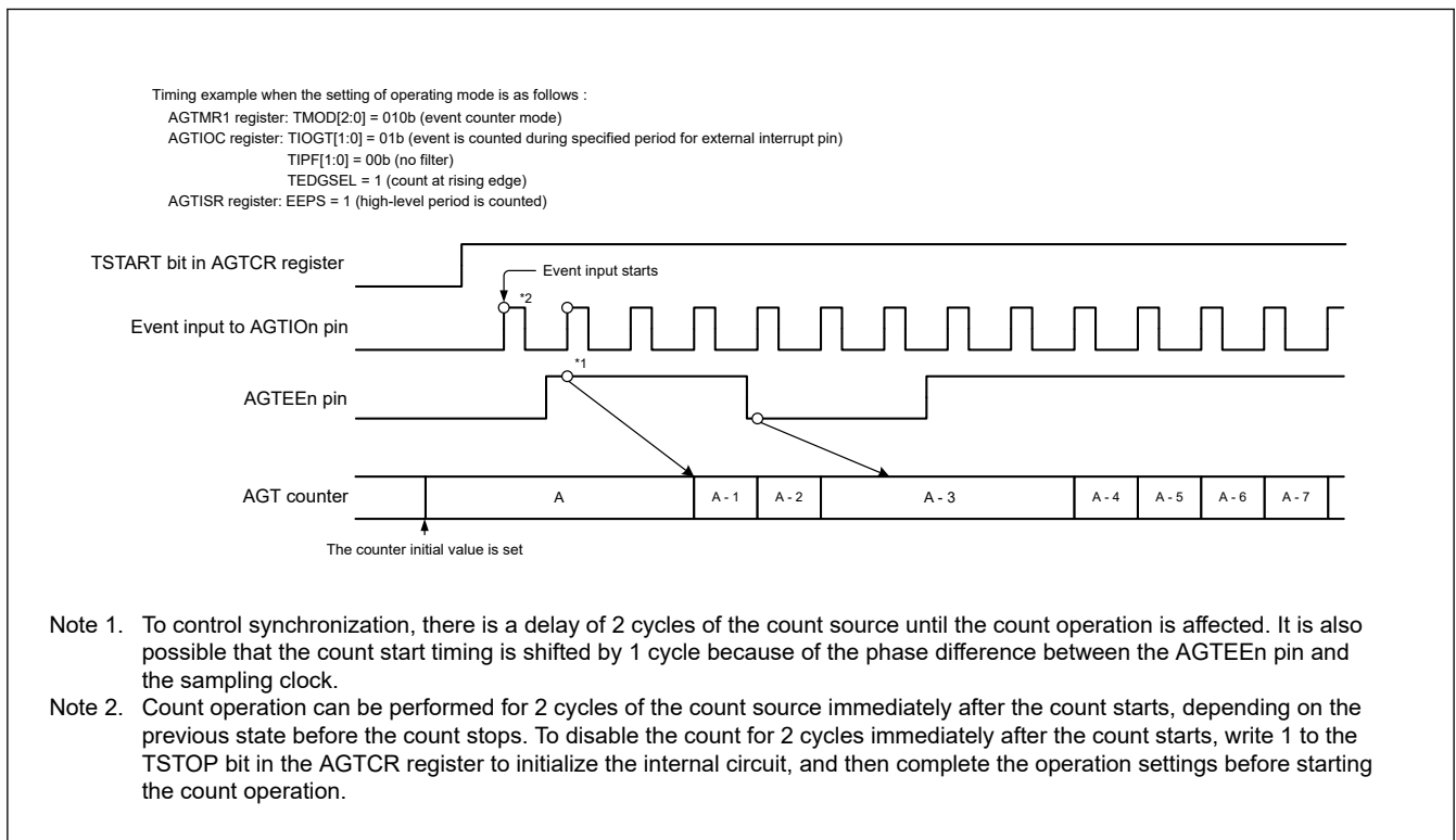
Figure 21.9 Operation in event counter mode example 2
