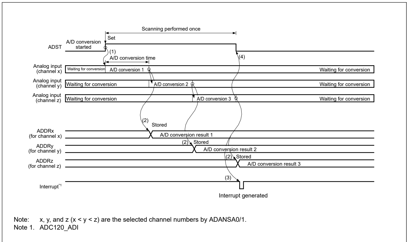
Figure 34.7 Example basic operation in single scan mode when the analog inputs (channel x to z) are selected
