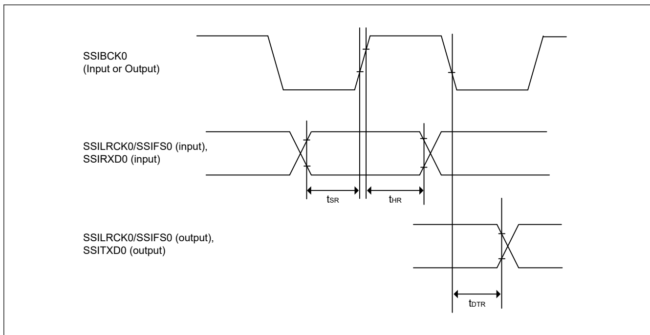
Figure 41.47 SSIE data transmit and receive timing when SSICR.BCKP = 0
