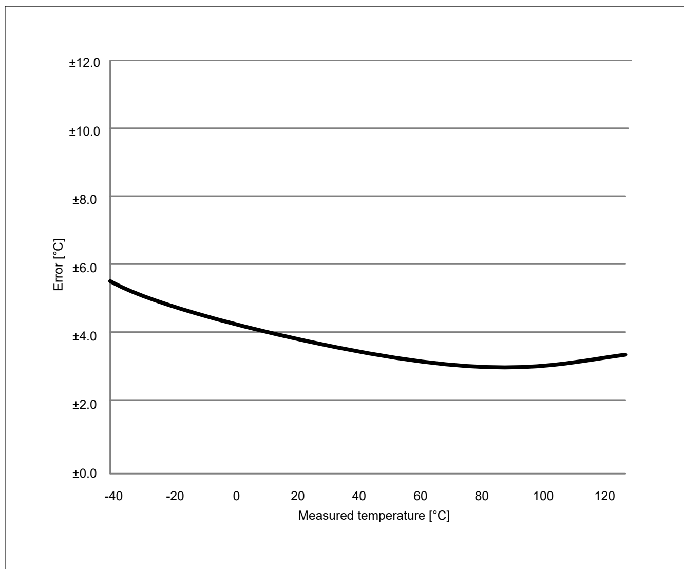
Figure 35.2 Error in the measured temperature (designed values)
