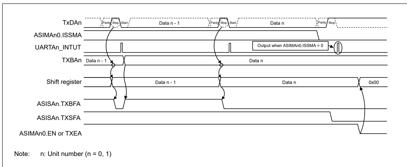
Figure 31.6 Timing when continuous transmission is completed
