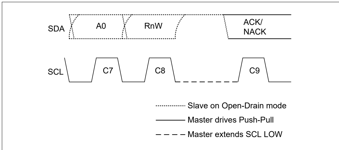
Figure 28.71 Master clock stalling in ACK phase
