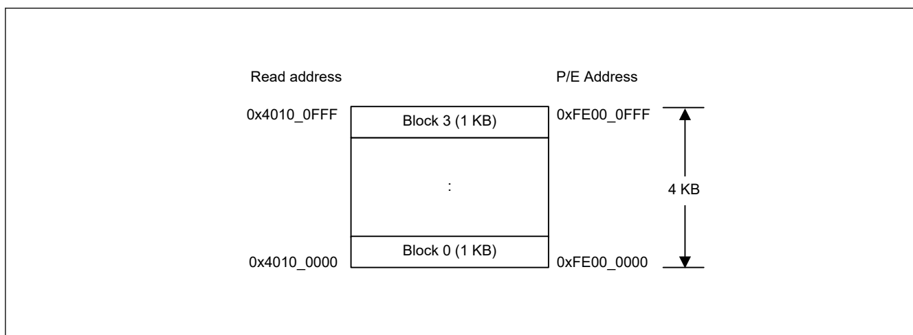
Figure 38.3 Mapping of the data flash memory
