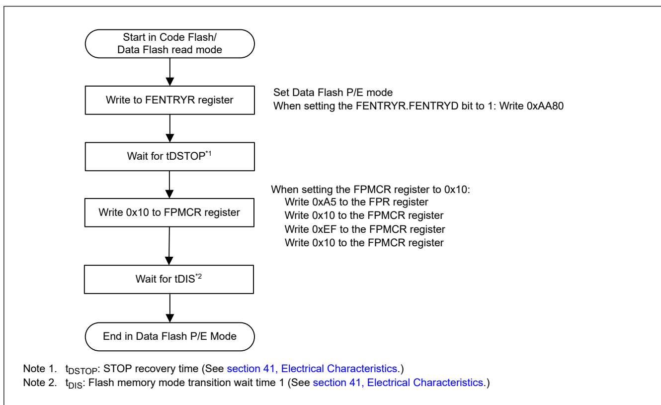
Figure 38.16 Procedure for changing from read mode to data flash P/E mode
