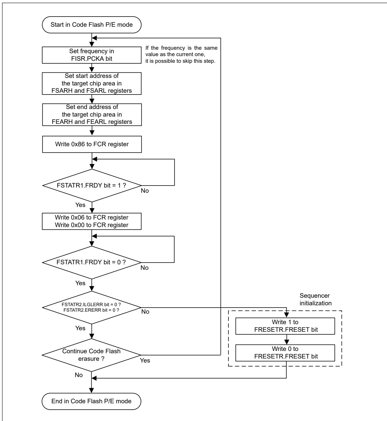
Figure 38.25 Flowchart for the code flash chip erase procedure
