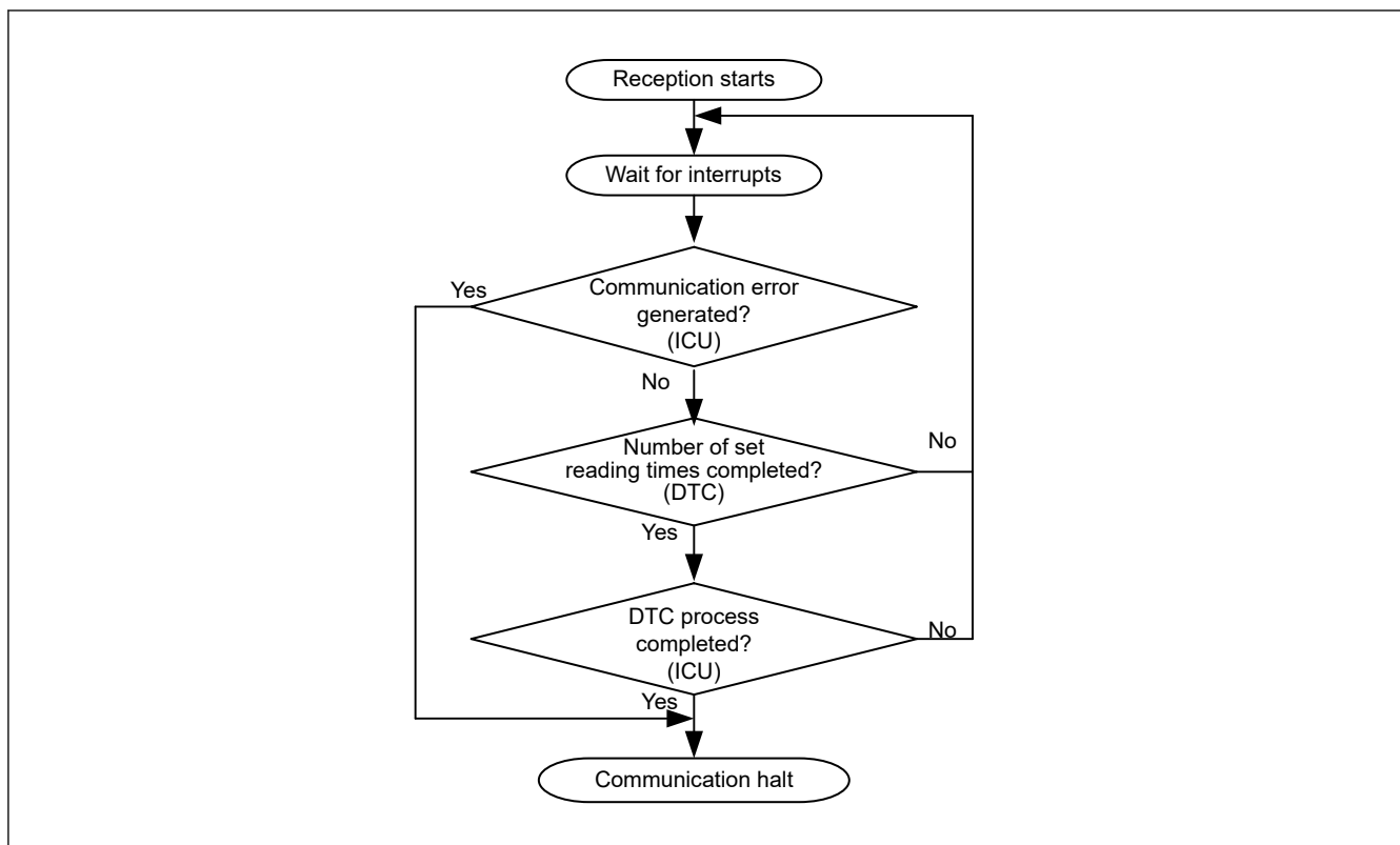
Figure 32.55 Reception procedure
