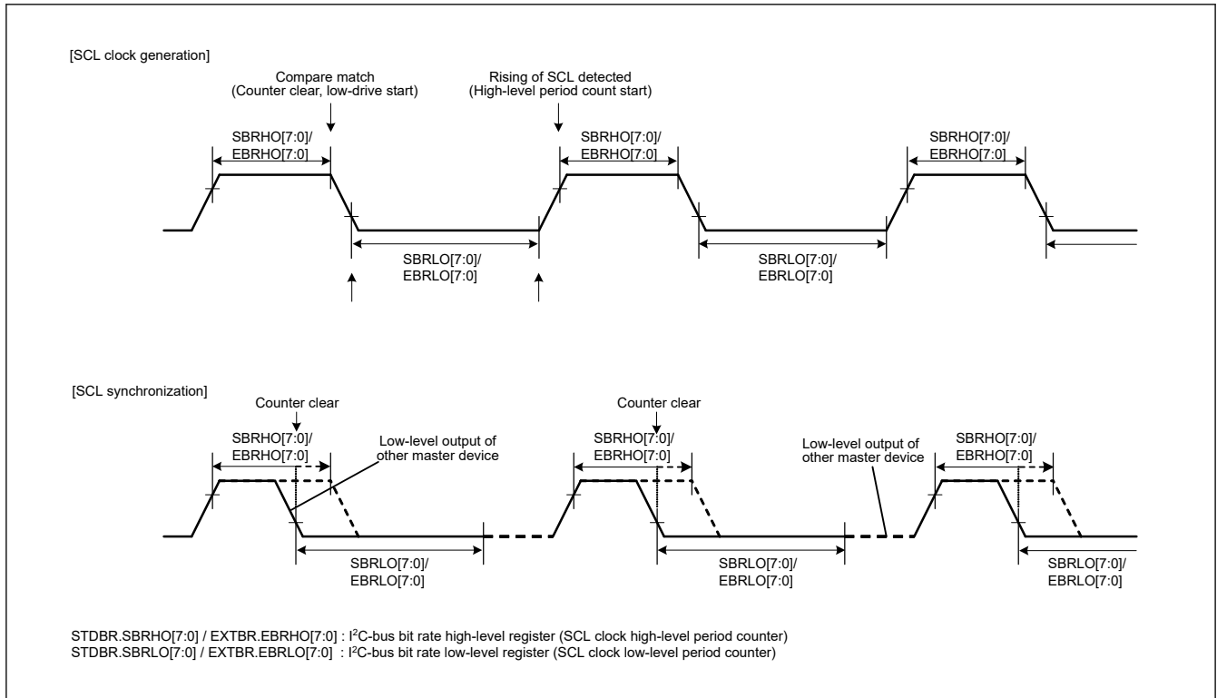
Figure 28.97 Generation and synchronization of the SCL signal
