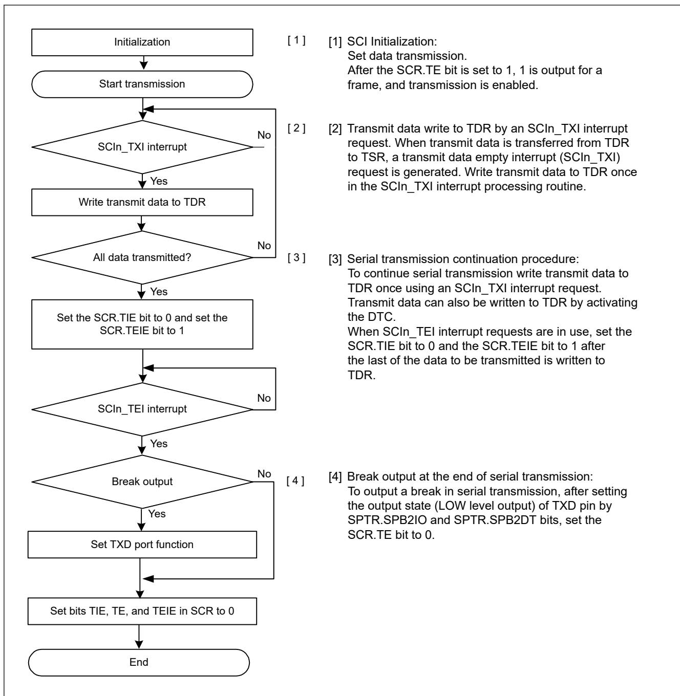
Figure 27.10 Example flow of serial transmission in asynchronous mode with non-FIFO selected
