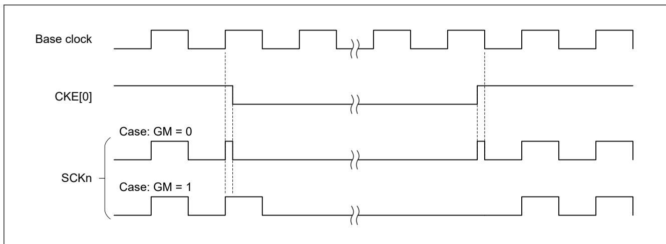
Figure 27.57 Clock Output timing
