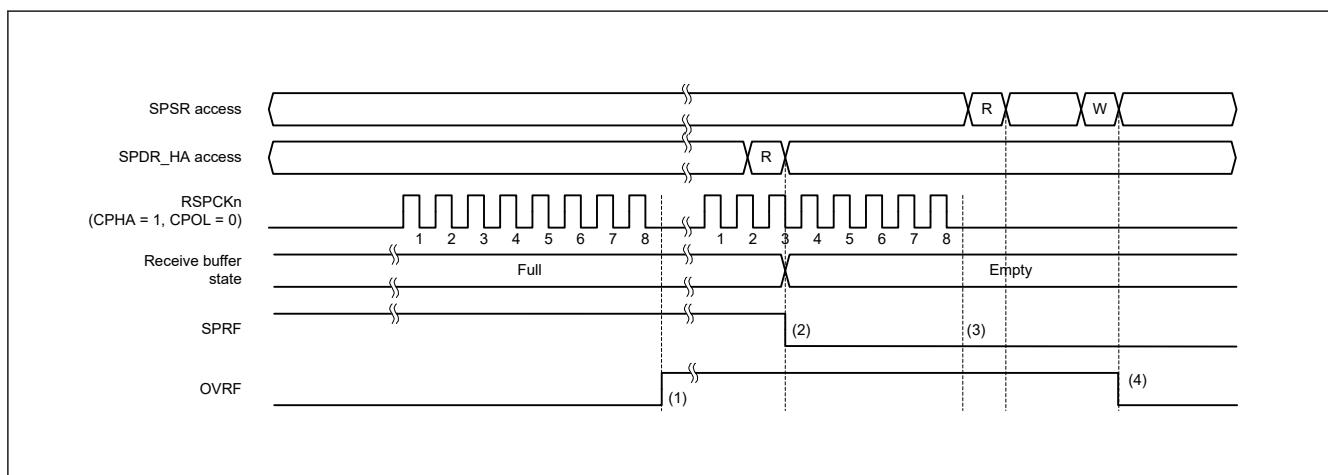
Figure 30.28 Operation example of the OVRF and SPRF flags
