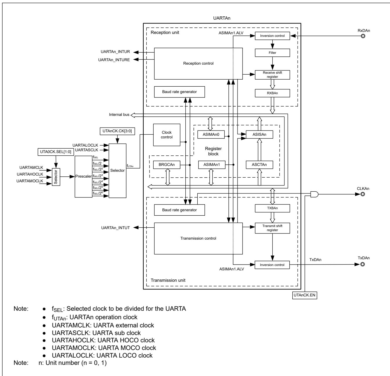
Figure 31.1 Block diagram of UARTAn
