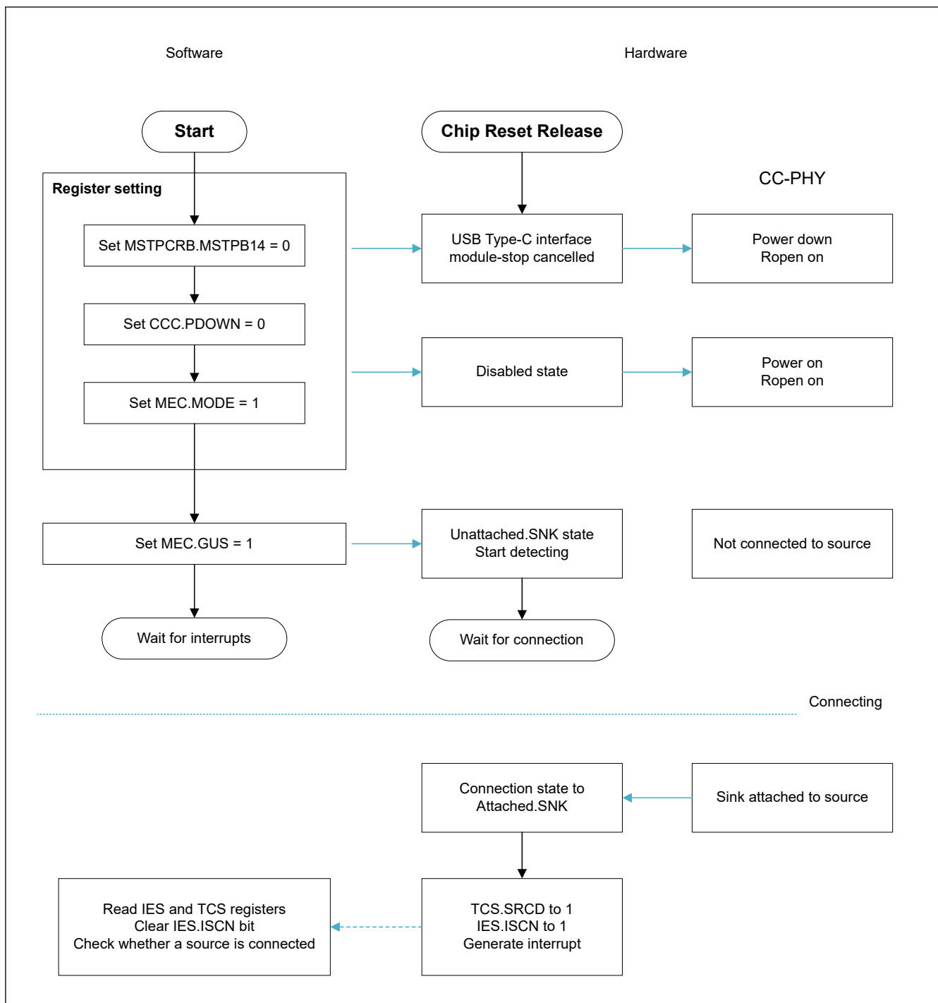
Figure 26.7 USB 2.0-only Sink mode initialization and connection detection flow
