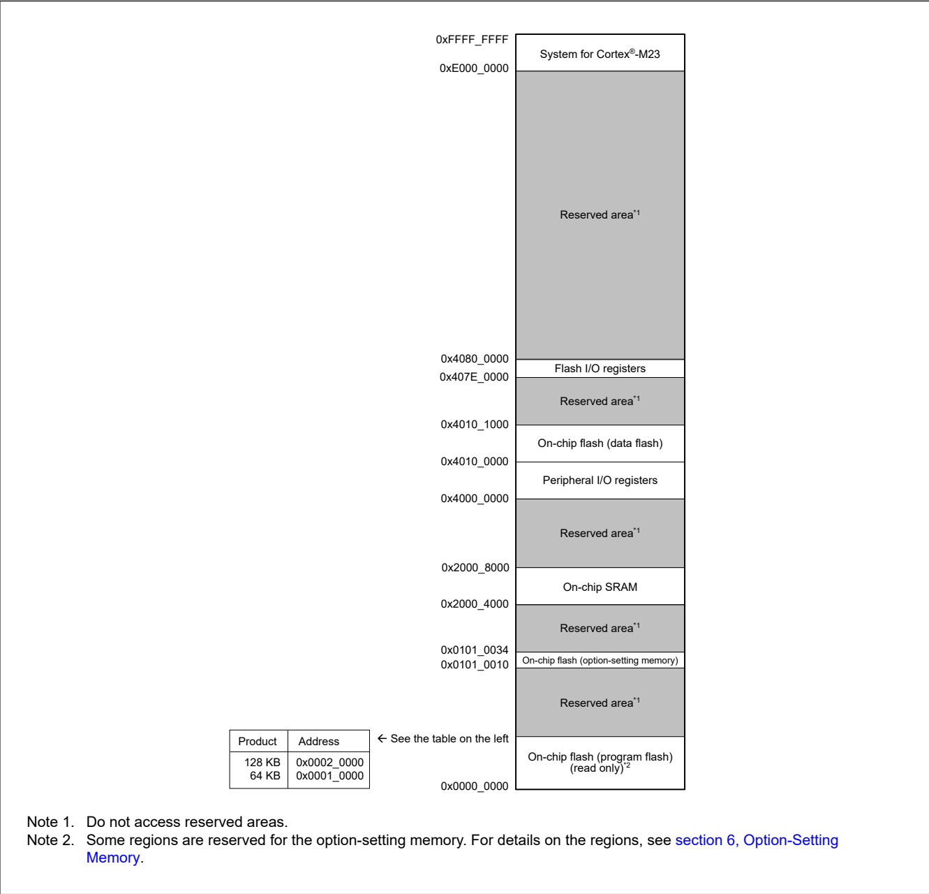
Figure 4.1 Memory map
