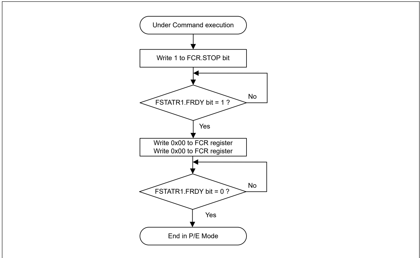
Figure 38.31 Simple flowchart for the forced stop procedure
