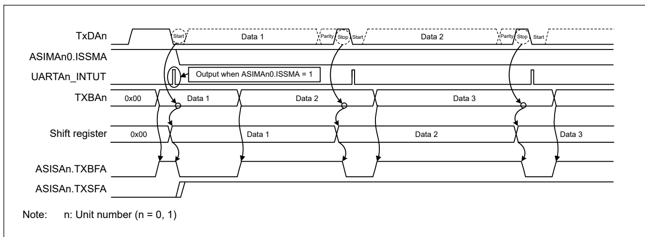
Figure 31.5 Timing when continuous transmission is started
