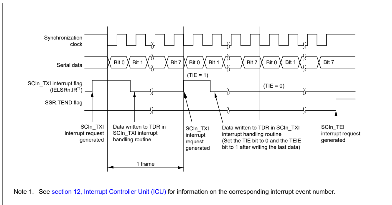
Figure 27.38 Example of serial data transmission in clock synchronous mode from the middle of transmission until transmission completion
