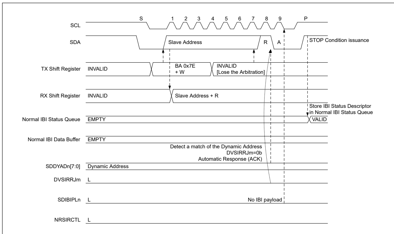
Figure 28.78 Slave interrupt request : ACK and DVIBIPL = 0
