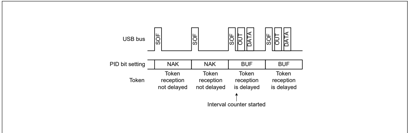
Figure 25.10 Relationship between frames and expected token reception when IITV[2:0] = 0
