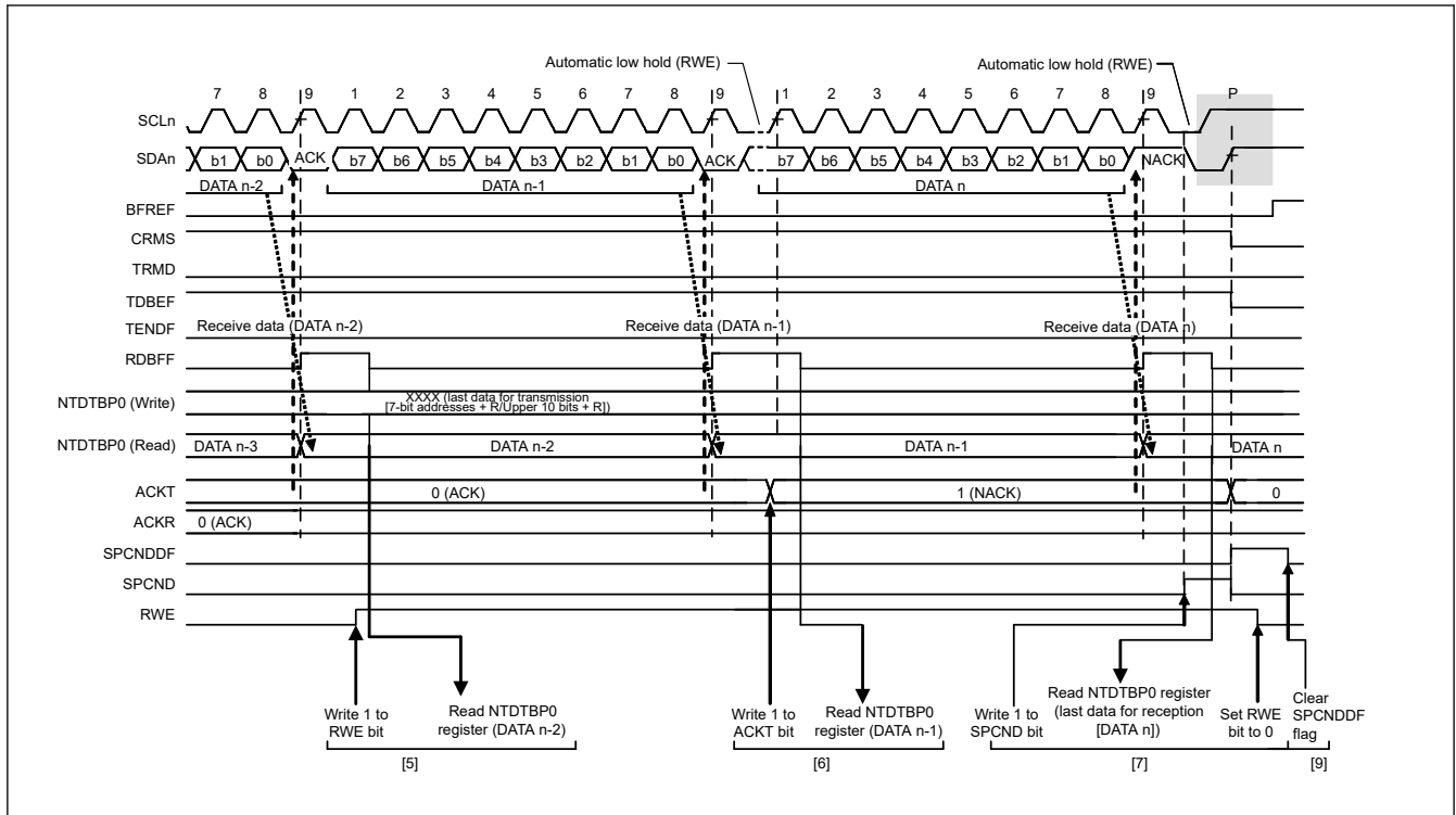
Figure 28.11 Master receive operation timing (3) (when ACKTWE = 0)
