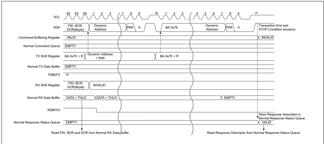
Figure 28.14 Dynamic address assign procedure (ENTDAA CCC) timing (3/3)
