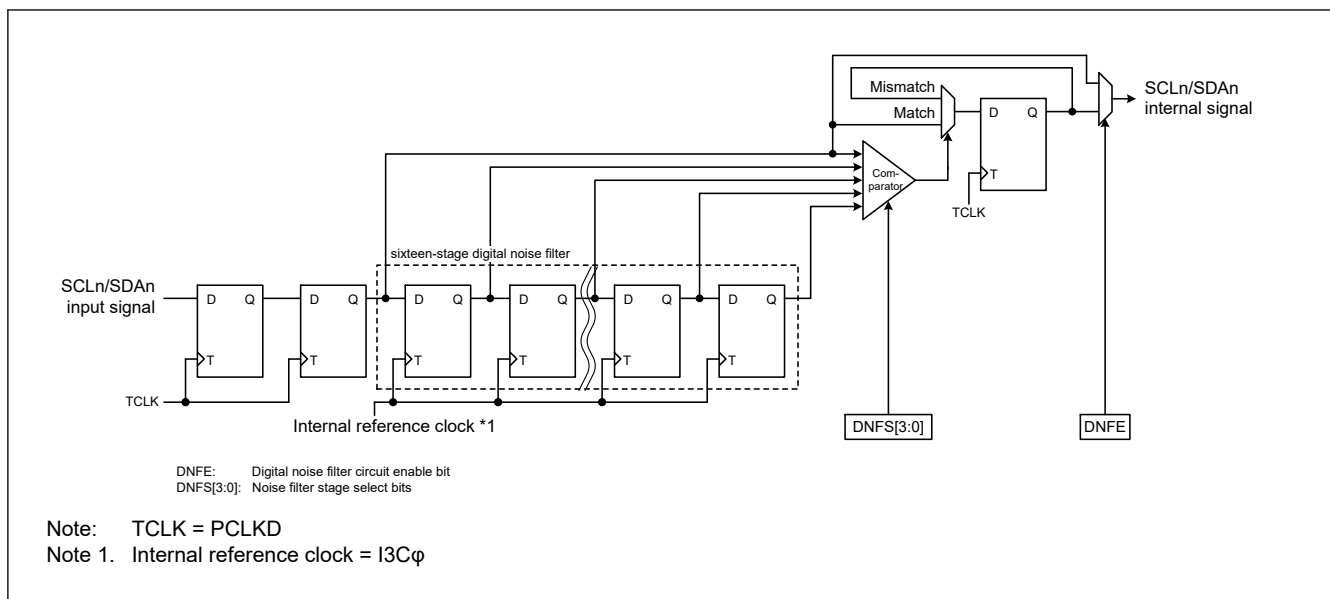
Figure 28.99 Block diagram of digital noise filter circuit
