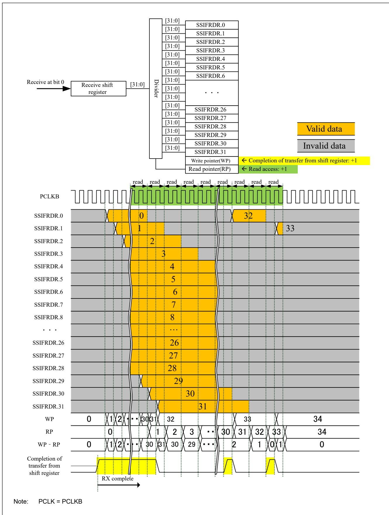
Figure 32.32 Configuration of the receive FIFO data register and receive shift register, and FIFO operation example
