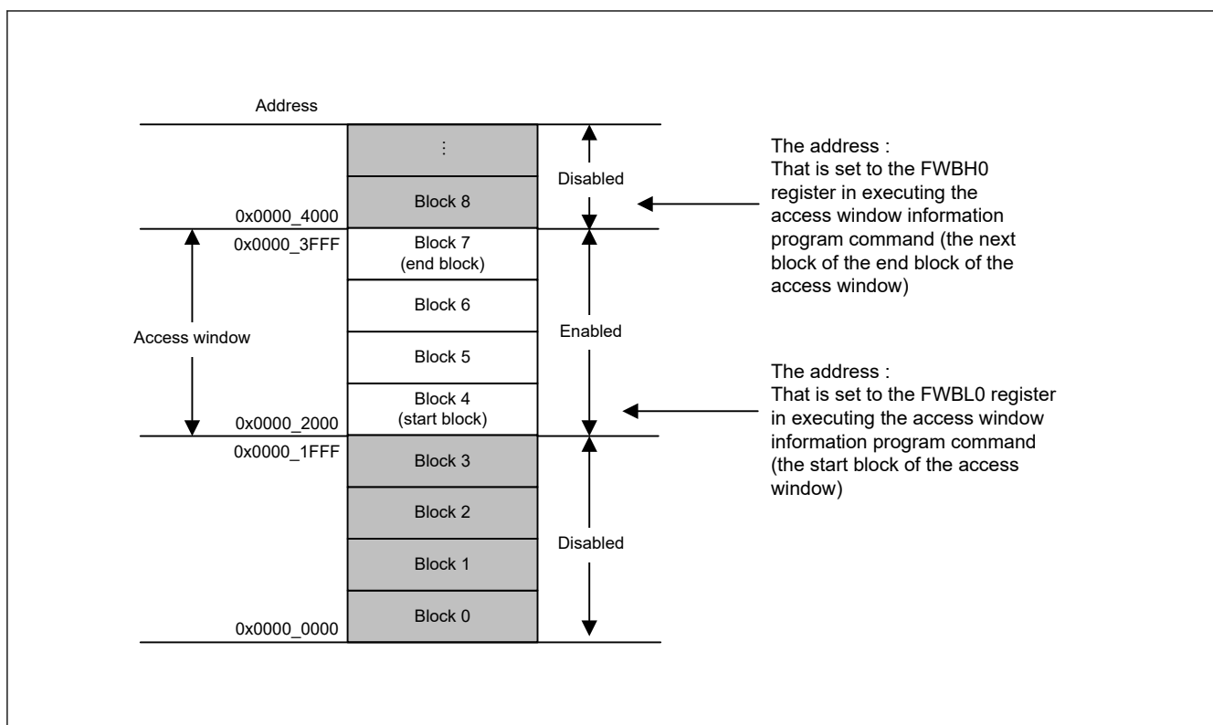
Figure 38.9 Area Protection Overview
