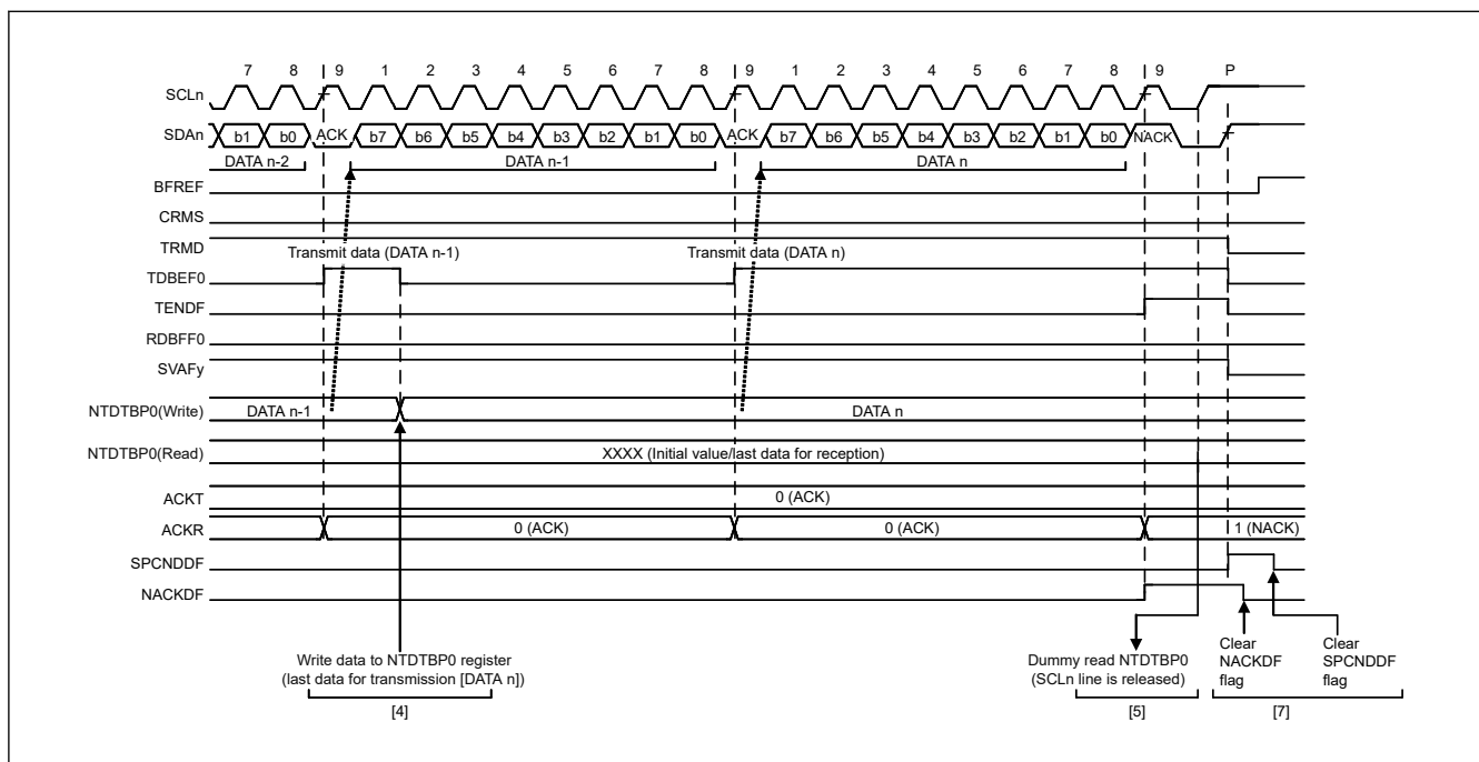
Figure 28.30 Slave transmit operation timing (2)
