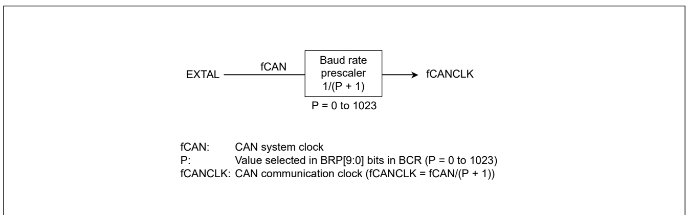
Figure 29.11 Block diagram of CAN clock generator
