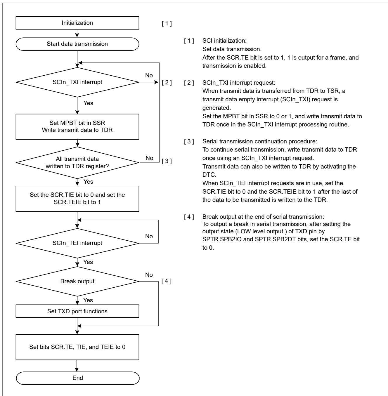
Figure 27.27 Example flow of multi-processor serial transmission with non-FIFO selected
