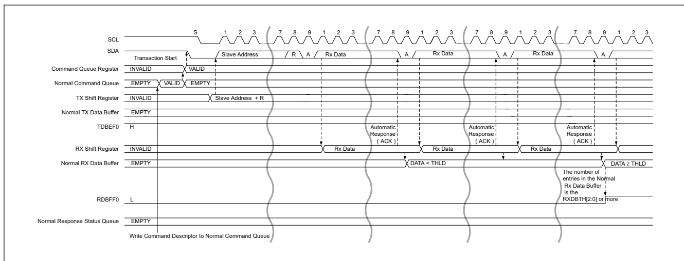
Figure 28.20 SDR data read transfer timing (1/2)
