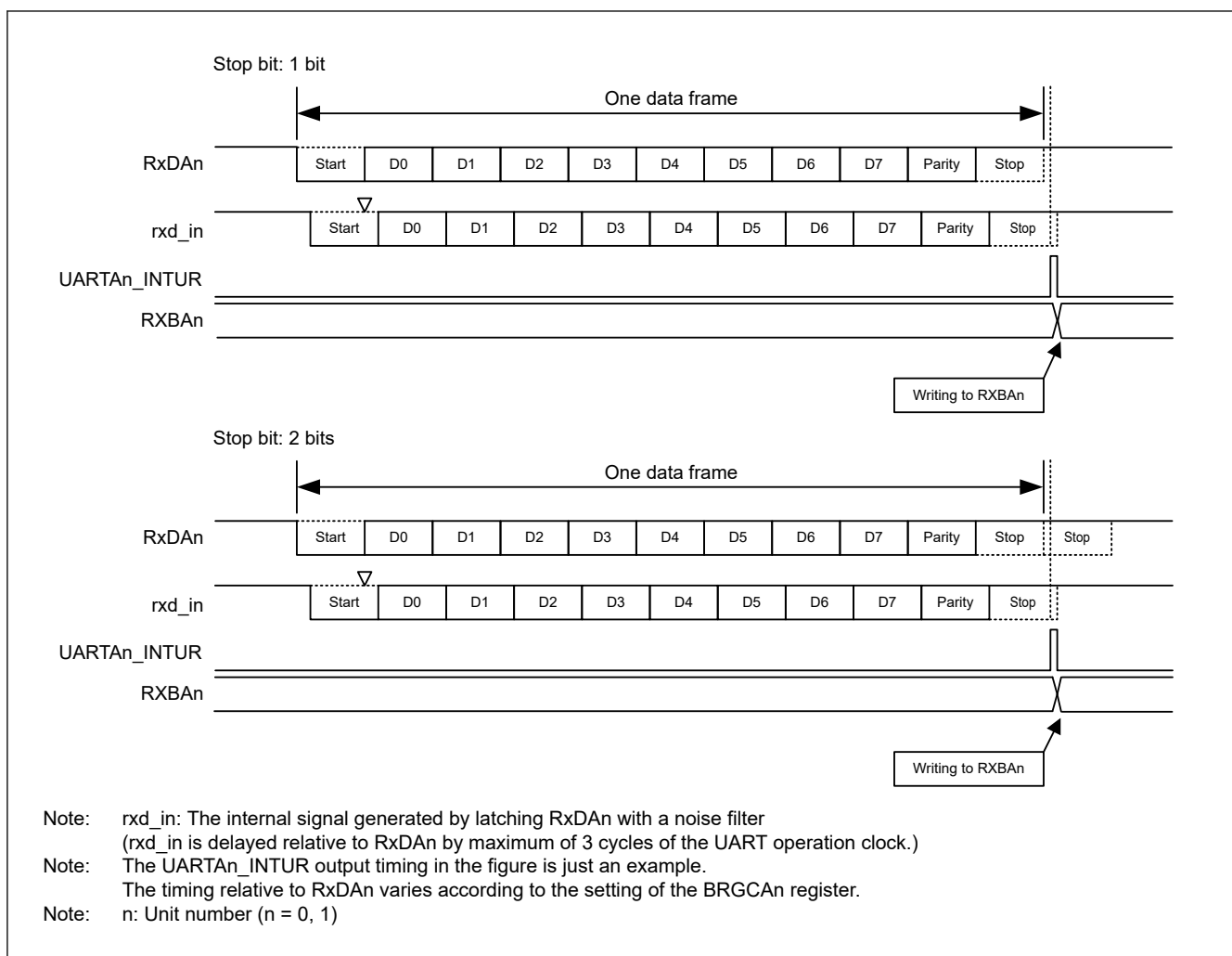
Figure 31.7 Timing of UART receive operation
