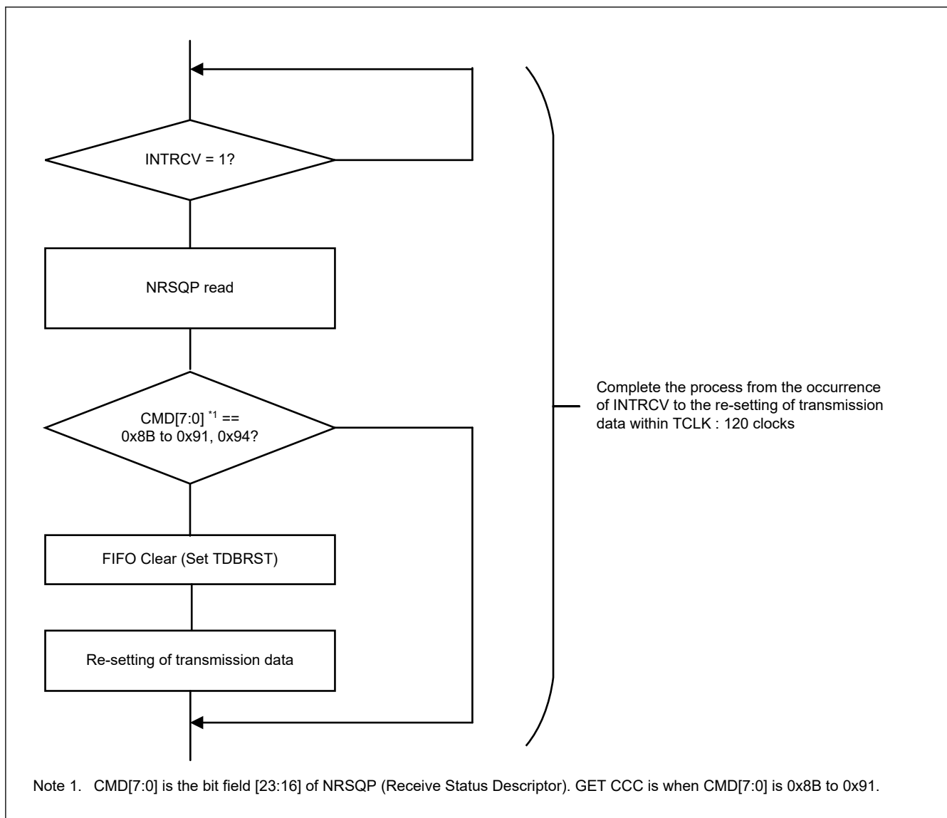
Figure 28.112 I3C slave receives GET CCC while data exists by writing from the NTDTBP0 register to the transmission buffer
