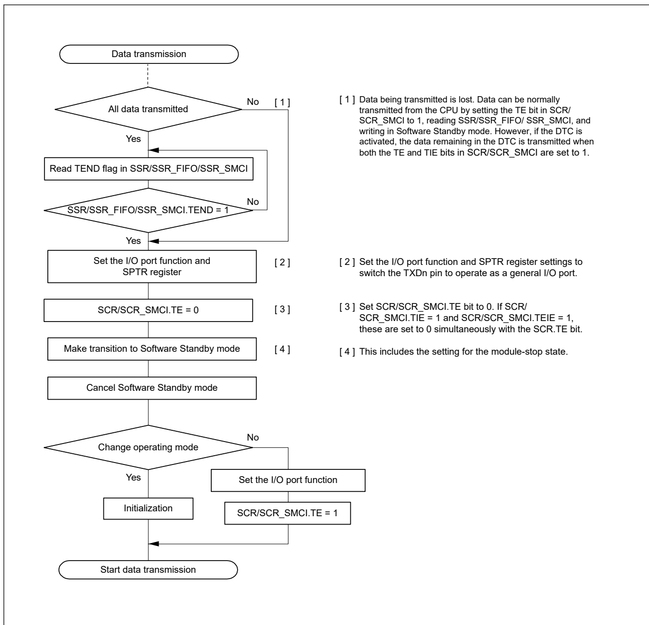
Figure 27.72 Example flow of transition to Software Standby mode during transmission
