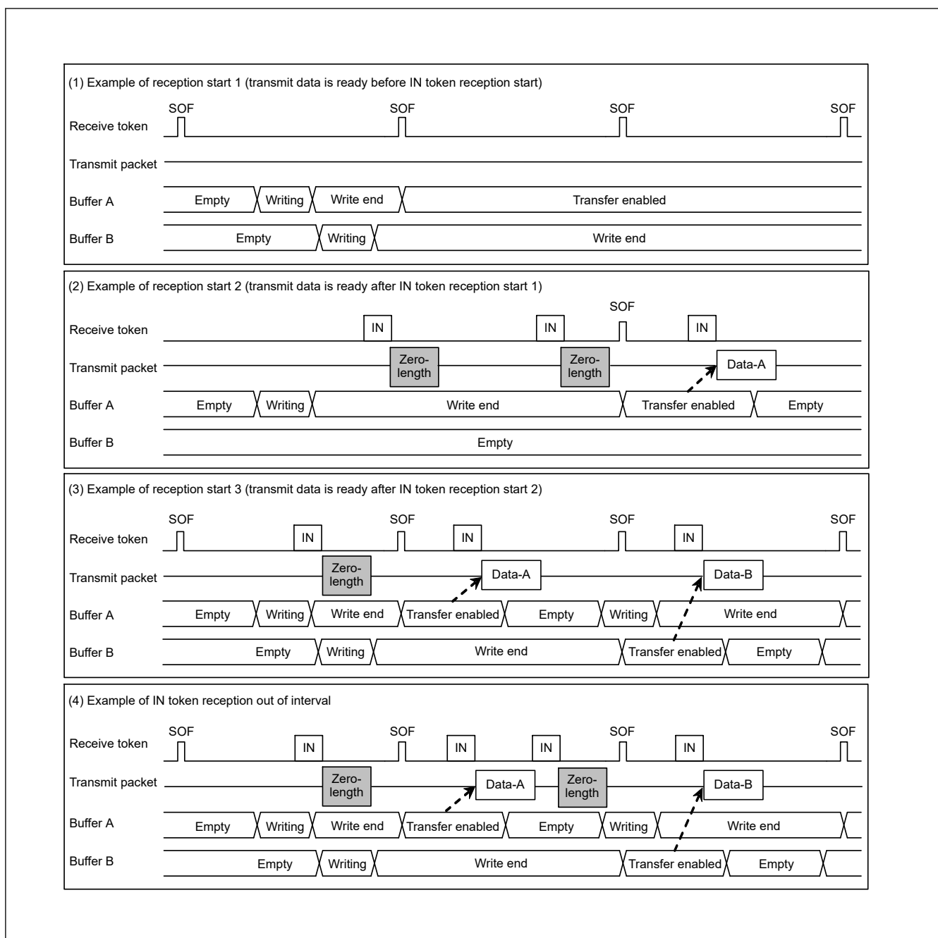
Figure 25.12 Example data setup operation
