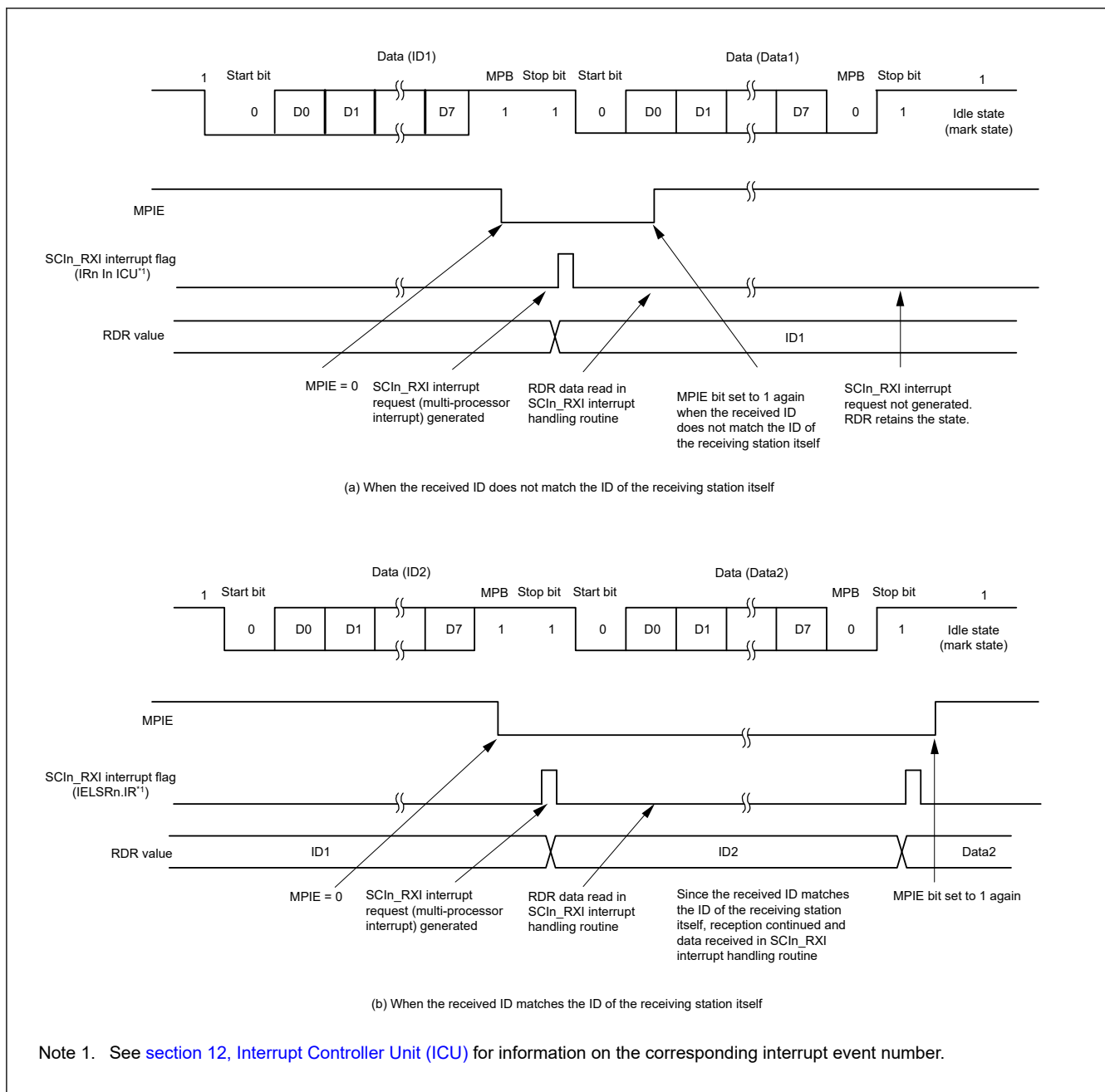
Figure 27.30 Example of SCI reception with 8-bit data, multi-processor bit, and 1 stop bit
