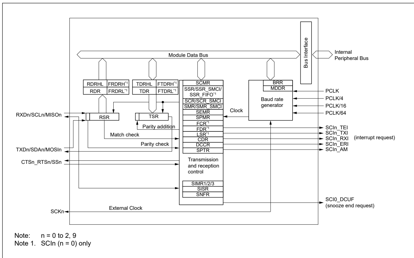
Figure 27.1 SCI block diagram
