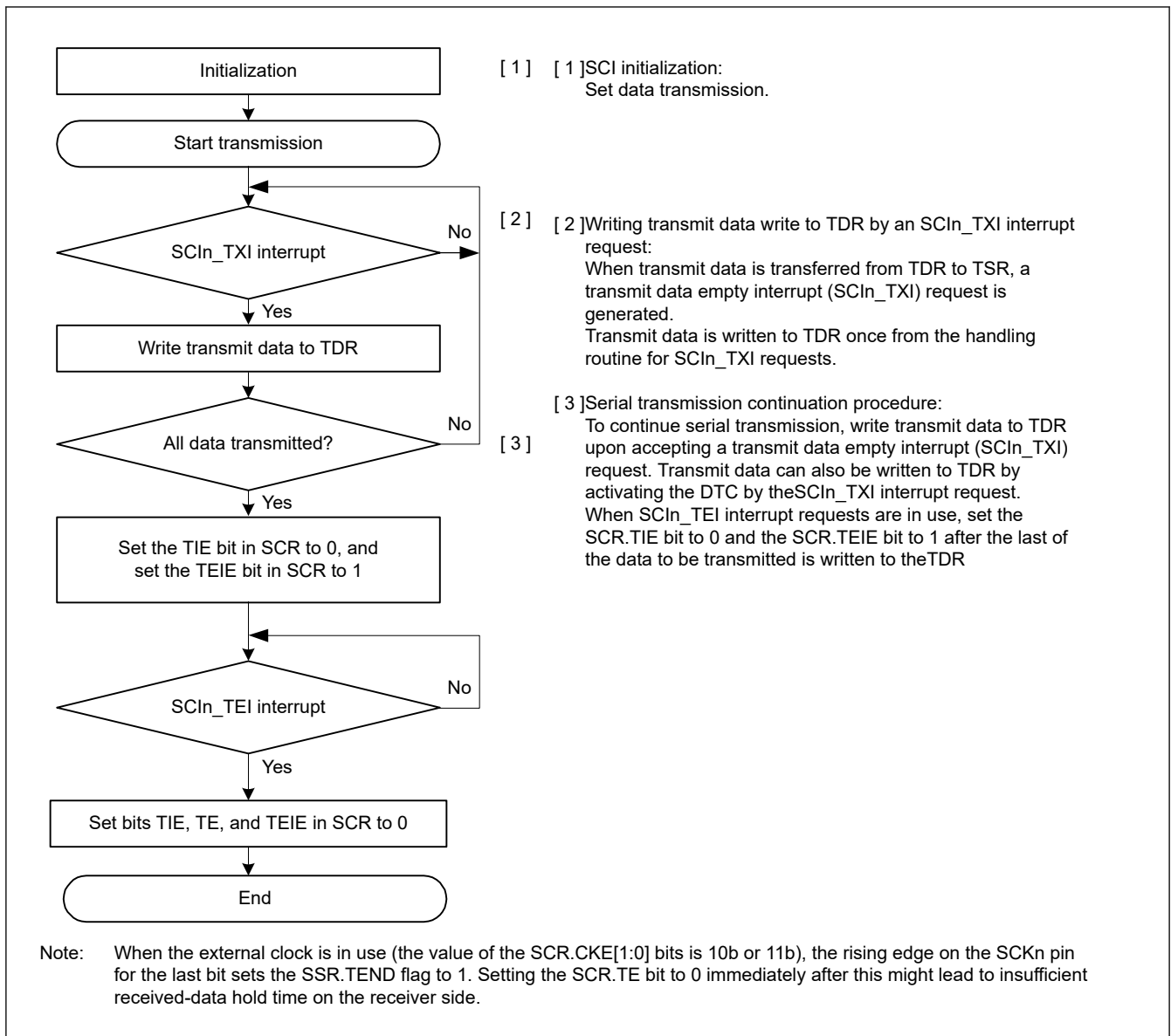
Figure 27.39 Example flow of serial transmission in clock synchronous mode with non-FIFO selected
