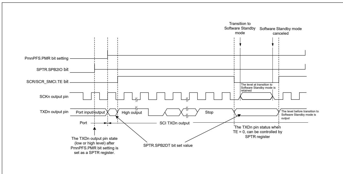
Figure 27.73 Port pin states during transition to Software Standby mode with internal clock and asynchronous transmission
