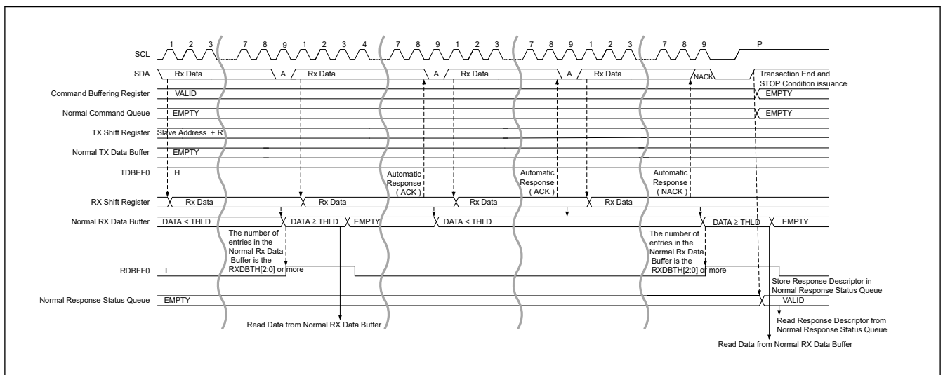
Figure 28.23 Legacy I 2 C message data read transfer timing (2/2)
