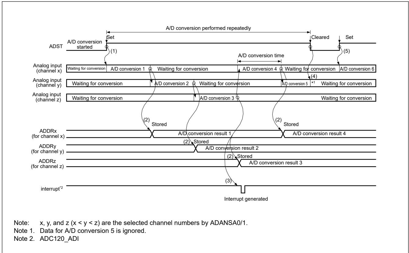
Figure 34.12 Example basic operation in continuous scan mode when the analog inputs (channel x to z) are selected
