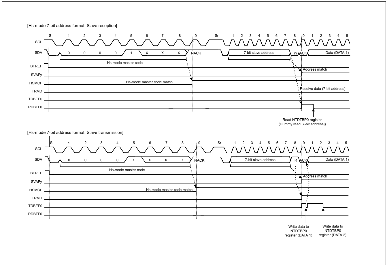
Figure 28.63 SVAFy/HSMCF Flag Set Timing during Reception of Hs-mode master code
