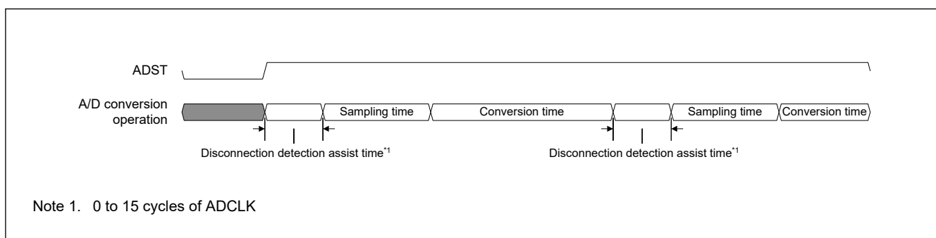
Figure 34.27 Operation of A/D conversion when disconnection detection assist function is used
