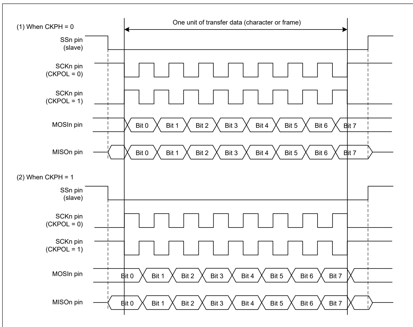
Figure 27.69 Relation between clock signal and transmit or receive data in simple SPI mode
