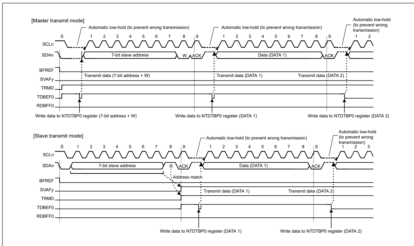
Figure 28.68 Automatic low-hold operation in transmit mode
