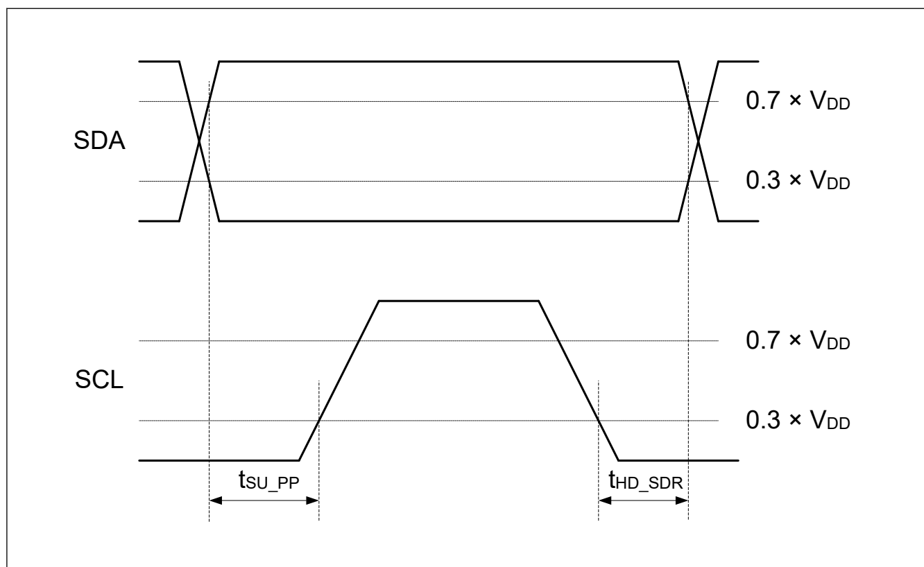
Figure 41.42 Master SDR Timing
