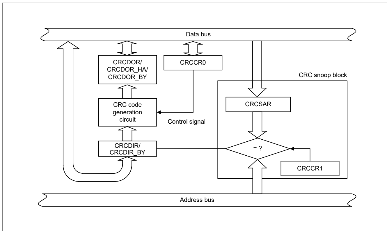
Figure 33.1 CRC calculator block diagram
