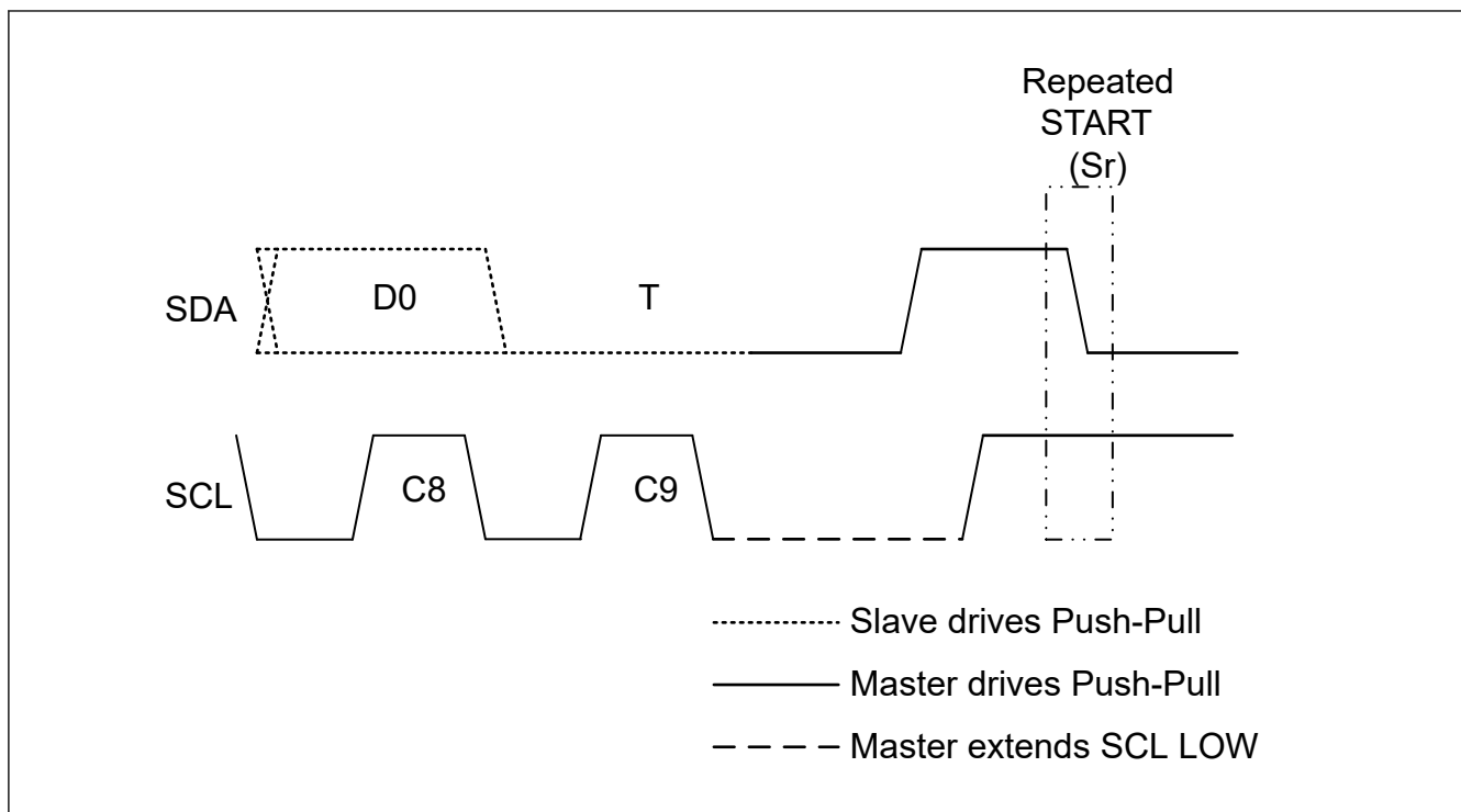
Figure 28.75 Master clock stalling in low T-bit before repeated START
