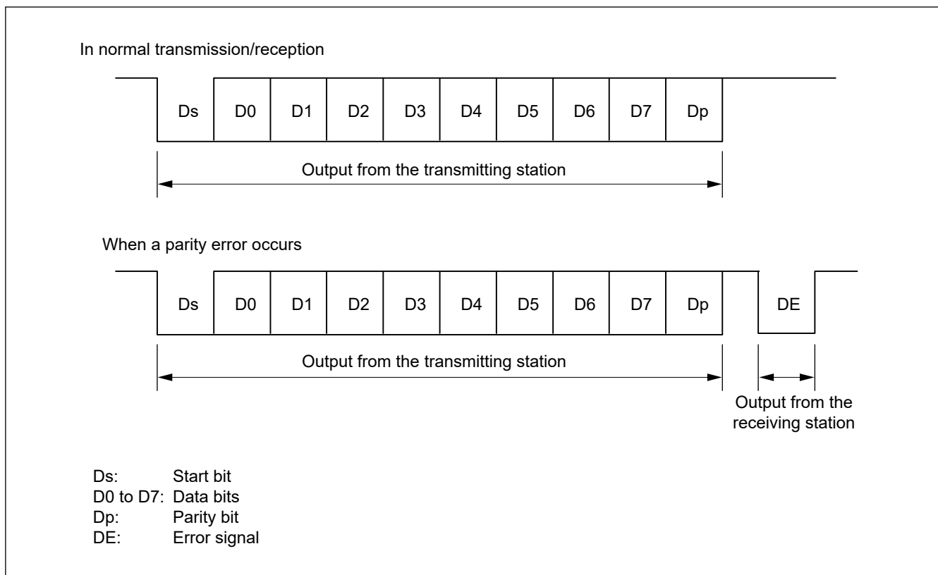
Figure 27.48 Data formats in smart card interface mode
