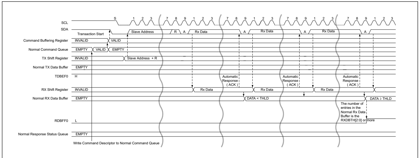
Figure 28.22 Legacy I 2 C message data read transfer timing (1/2)
