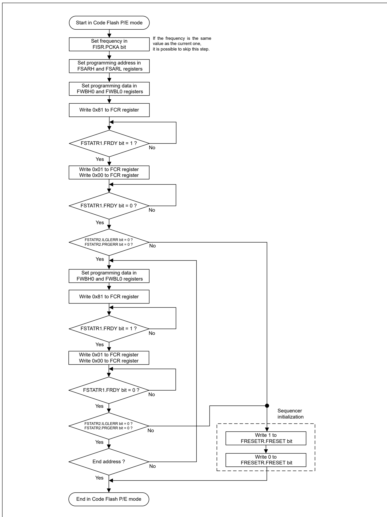
Figure 38.21 Flowchart for consecutive programming of the code flash
