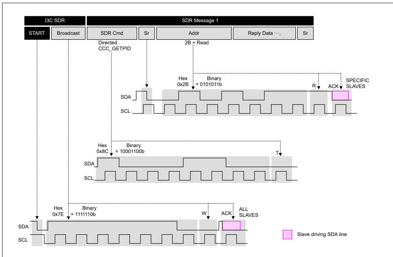
Figure 28.52 Example communication using I3C coding SDR with CCC direct addressing
