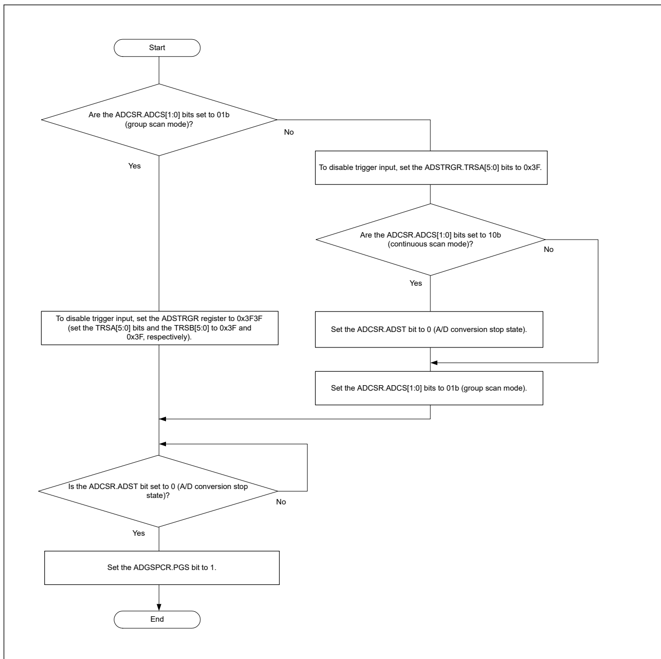
Figure 34.16 Flowchart for ADGSPCR.PGS bit setting
