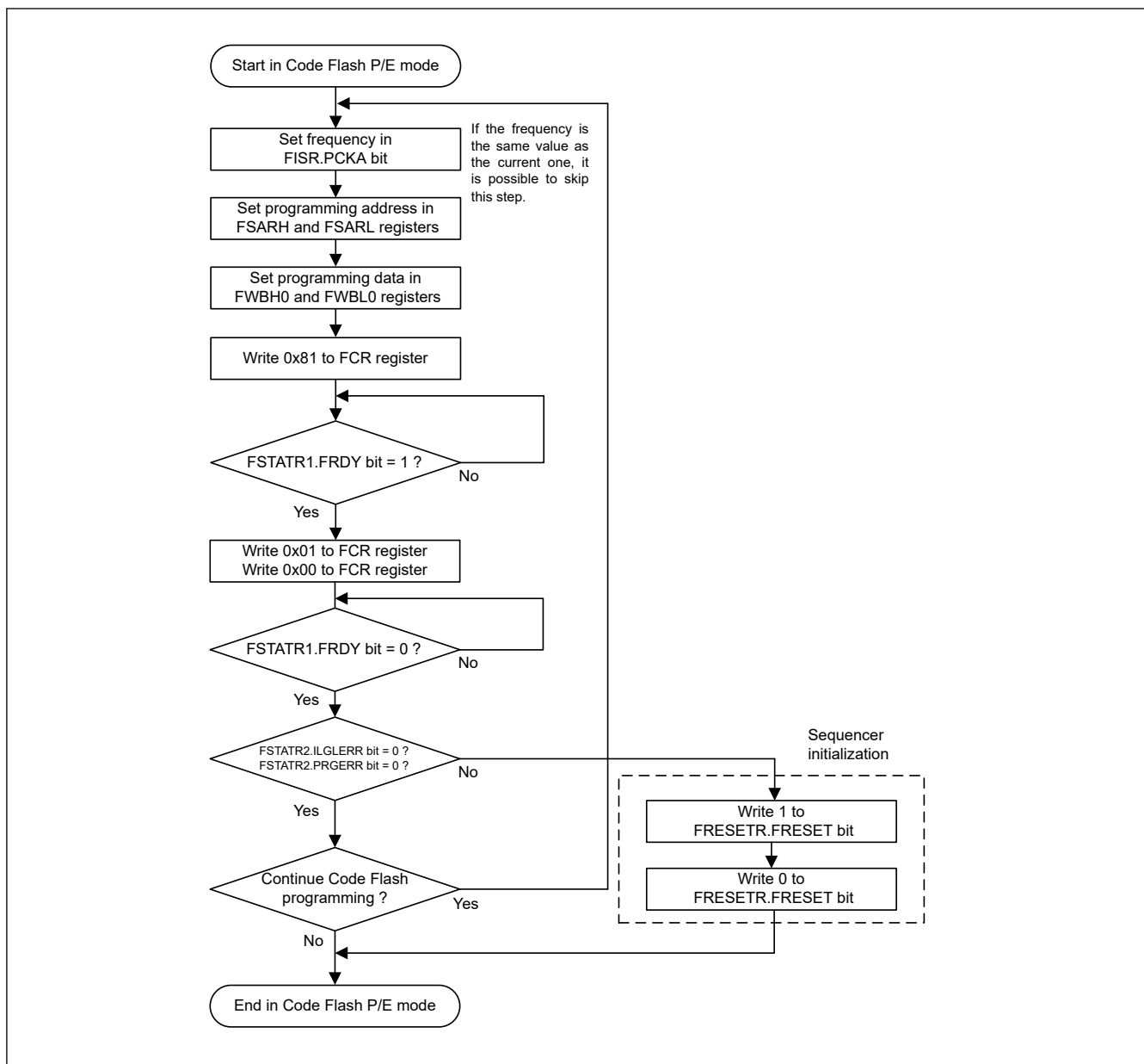
Figure 38.19 Flowchart for programming of the code flash
