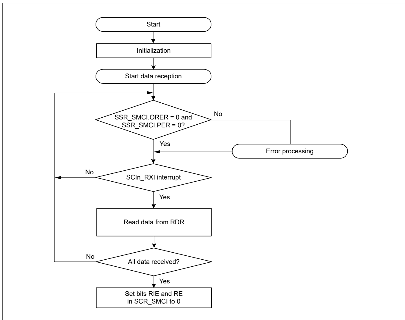
Figure 27.56 Example flow of smart card interface reception
