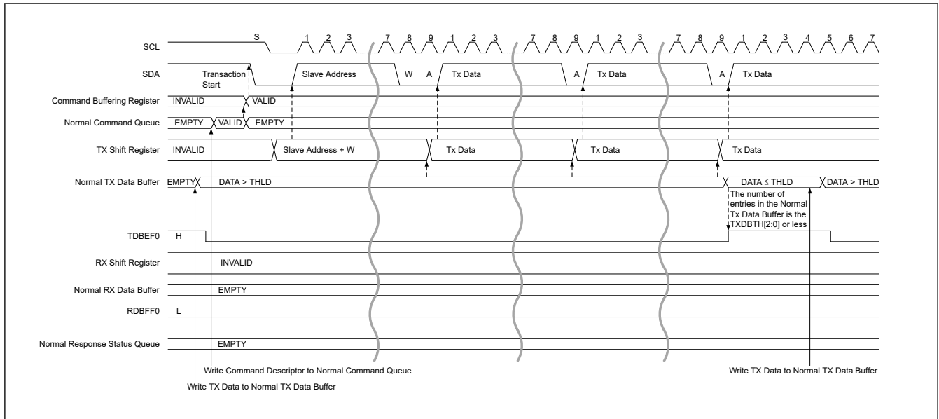
Figure 28.18 Legacy I 2 C message data write timing (1/2)
