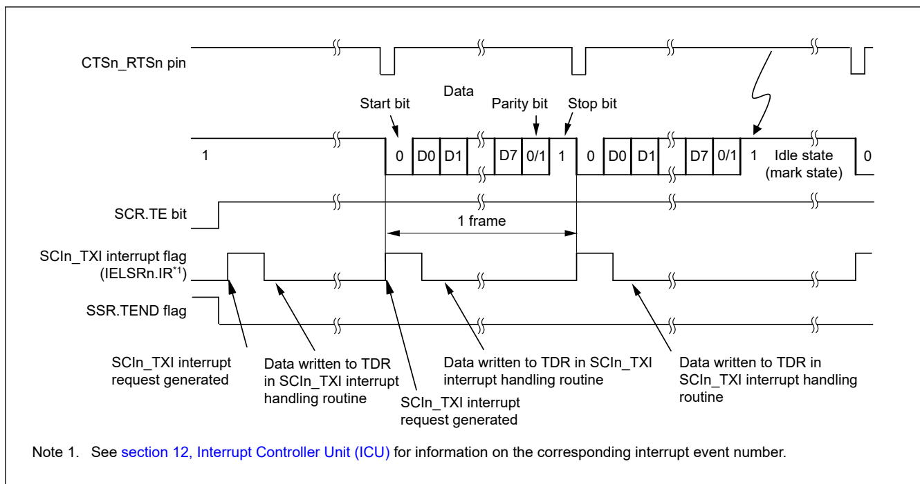
Figure 27.8 Example operation for serial transmission in asynchronous mode (2) with 8-bit data, parity bit, one stop bit, CTS function used, and at the beginning of transmission
