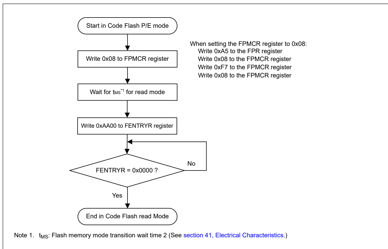
Figure 38.17 Procedure for changing from code flash P/E mode to read mode
