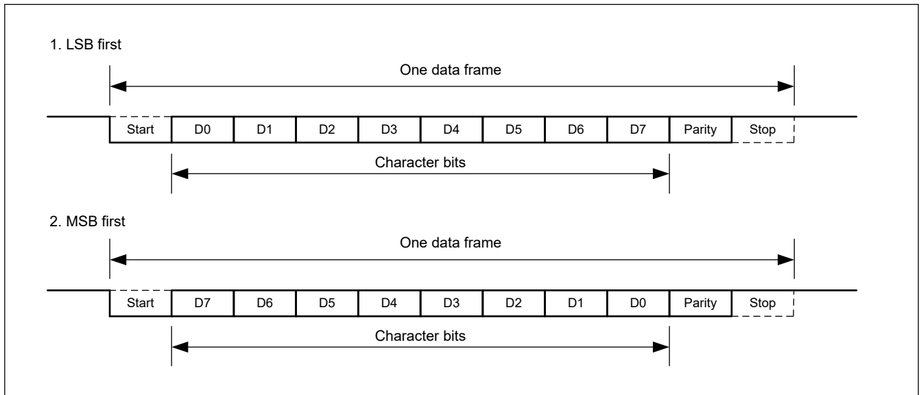
Figure 31.2 Transmit and receive data format
