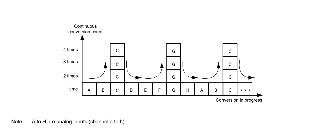
Figure 34.2 Scan conversion sequence with ADADC.ADC[2:0] = 011b, set 1 for analog inputs C and G by ADADS0/1
