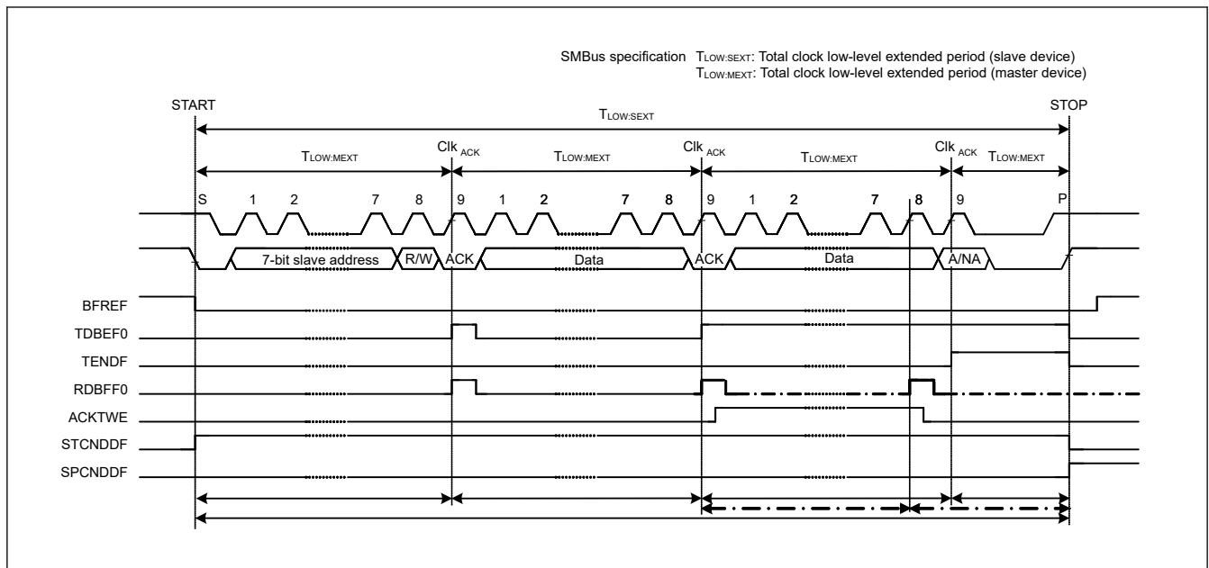
Figure 28.91 SMBus timeout measurement
