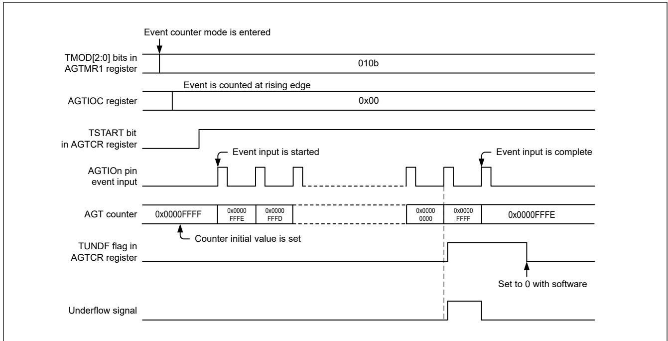
Figure 21.8 Operation in event counter mode example 1
