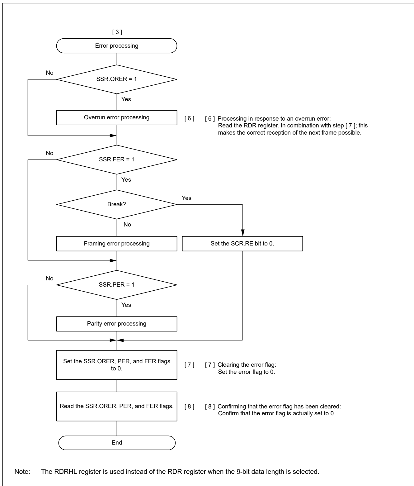
Figure 27.19 Example Flowchart of Serial Reception in Asynchronous Mode (FIFO not Selected and Address Matching Enabled) (3)
