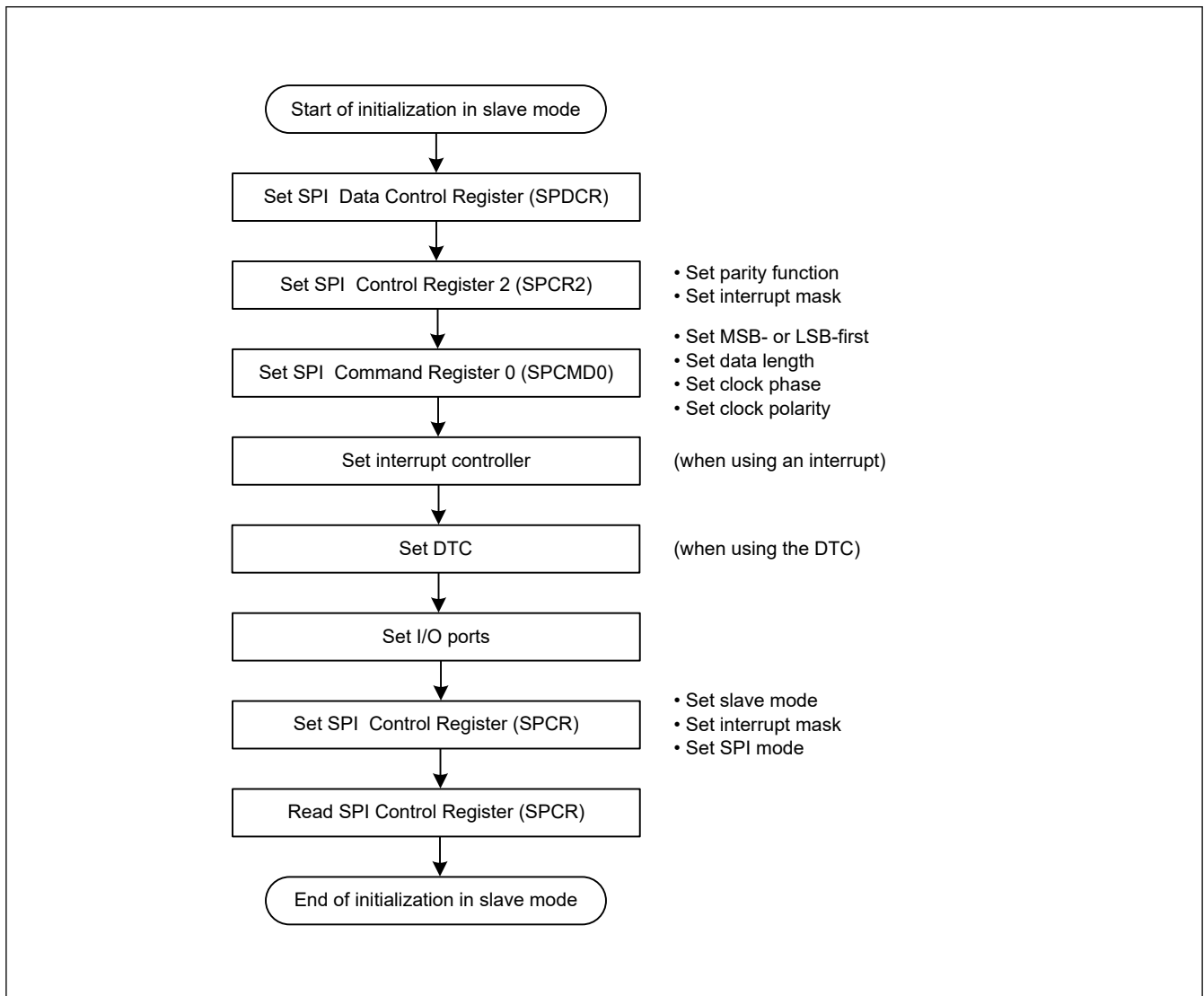
Figure 30.41 Example of initialization flow in slave mode for clock synchronous operation
