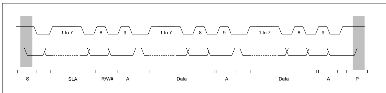
Figure 28.49 I 2 C bus timing (SLA = 7 bits)
