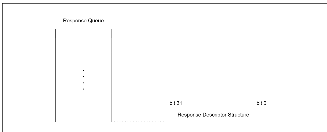
Figure 28.5 Receive status descriptor data structure
