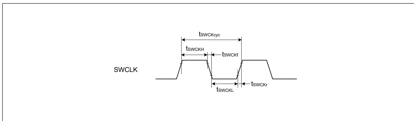
Figure 41.62 SWD SWCLK timing
