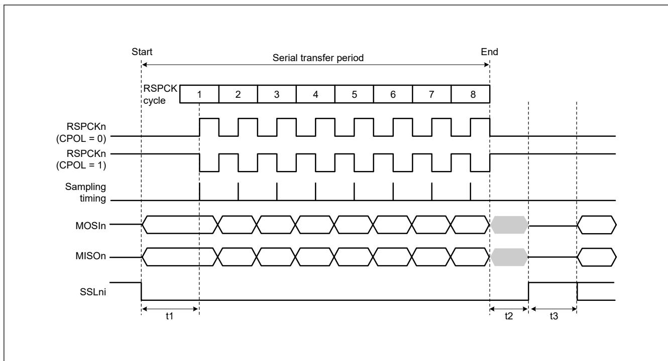
Figure 30.22 SPI transfer format when CPHA = 0
