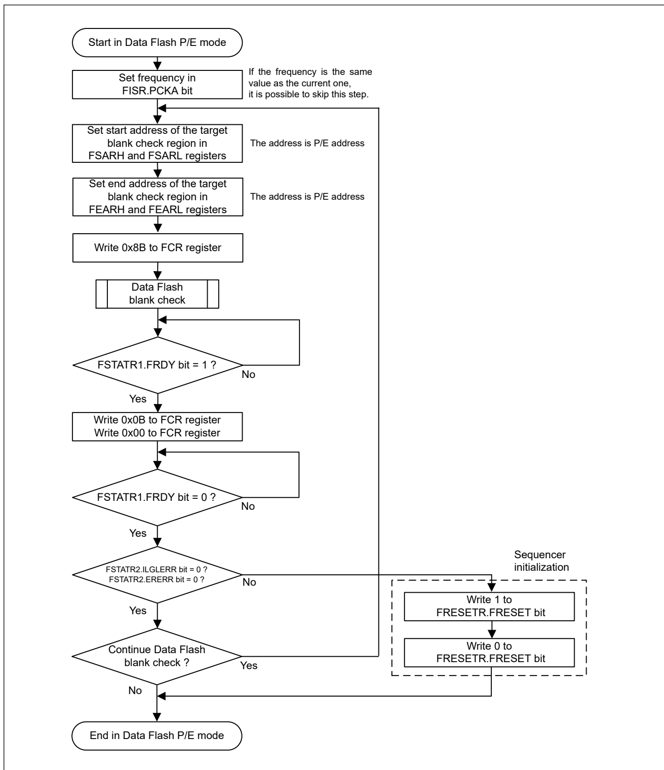
Figure 38.28 Flowchart for the data flash blank check procedure
