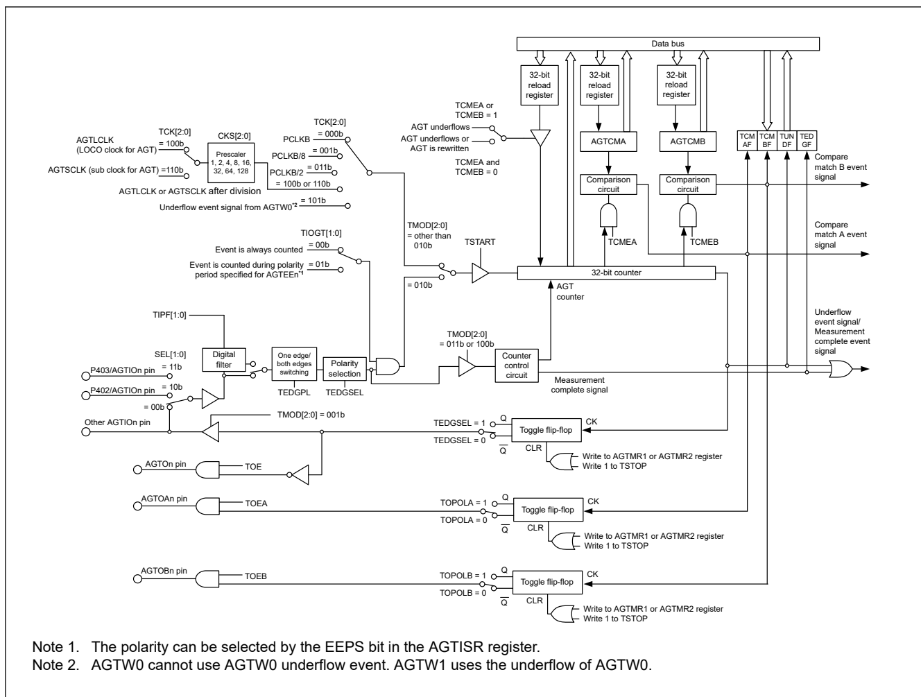
Figure 21.1 AGTW block diagram
