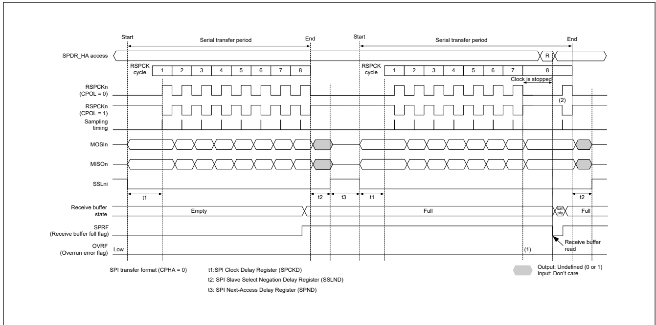
Figure 30.30 Clock stop waveform when serial transfer continues while receive buffer is full in master mode (CPHA = 0)
