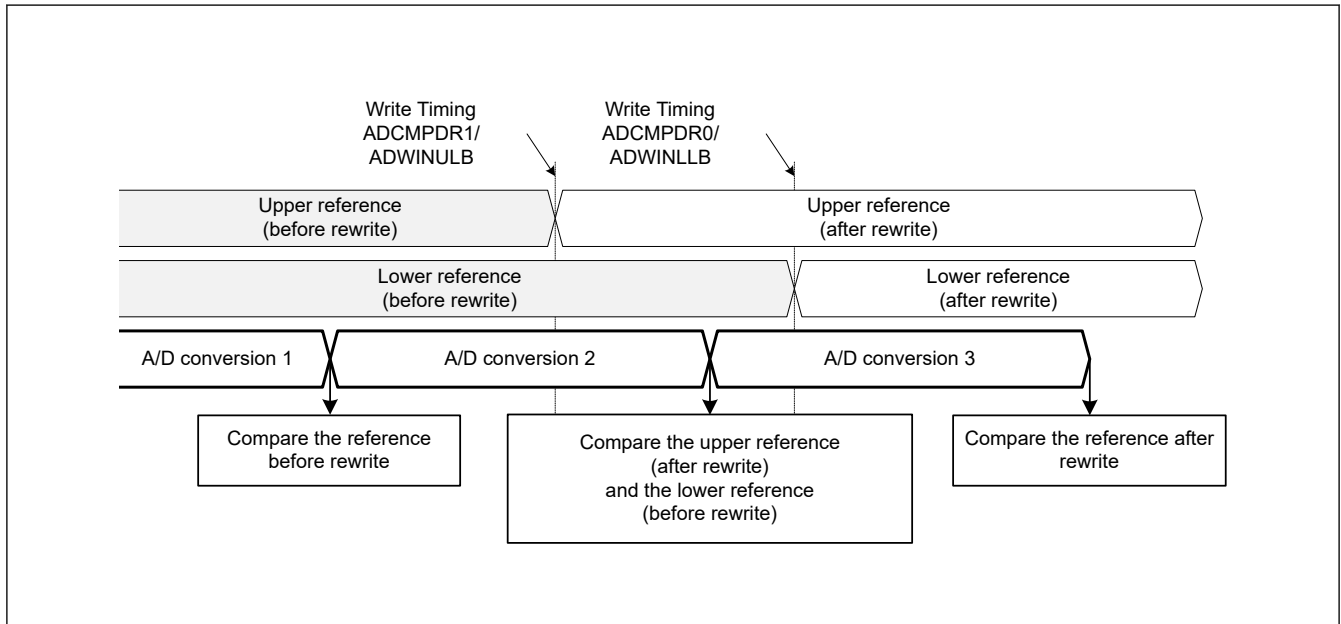
Figure 34.5 Comparison between upper and lower references before and after a rewrite
