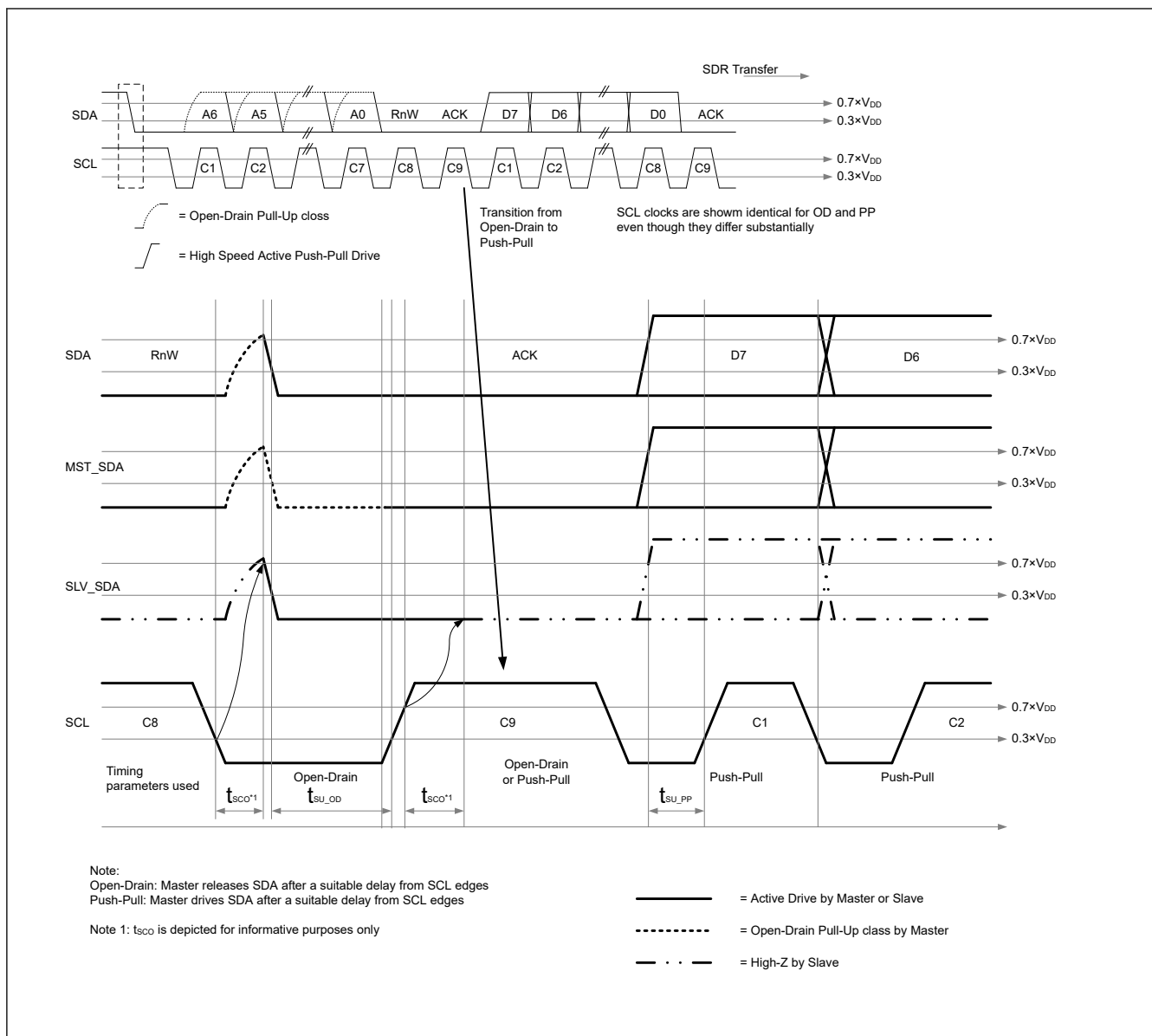
Figure 41.37 I3C Data Transfer – ACK by Slave
