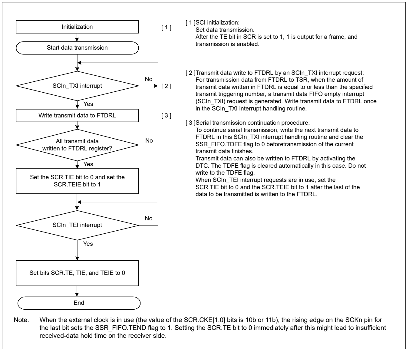
Figure 27.40 Example flow of serial transmission in clock synchronous mode with FIFO selected
