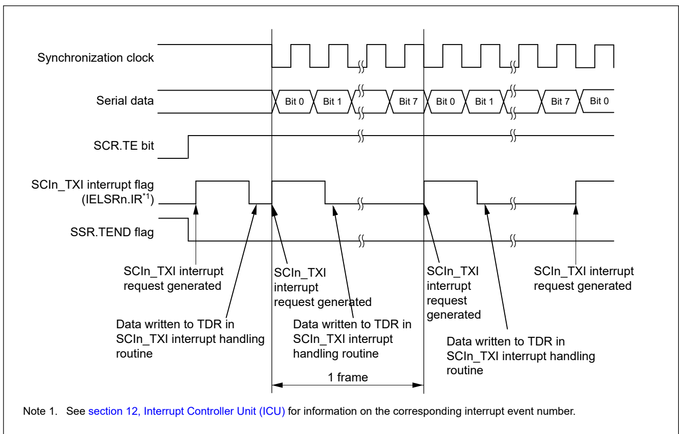
Figure 27.36 Example of serial data transmission in clock synchronous mode when the CTS function is not used at the beginning of transmission
