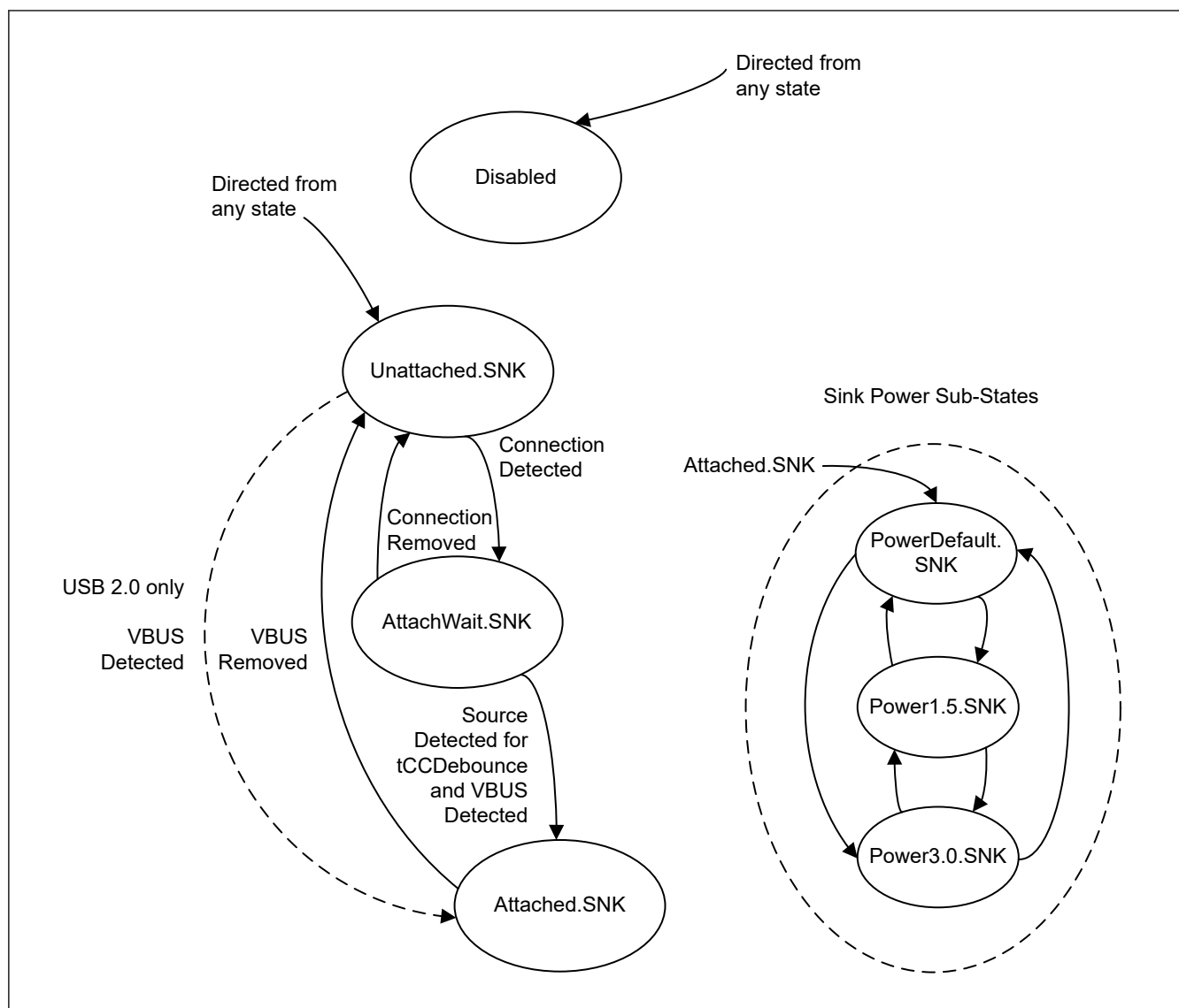
Figure 26.2 Connection state diagram for RA2L2 sink
