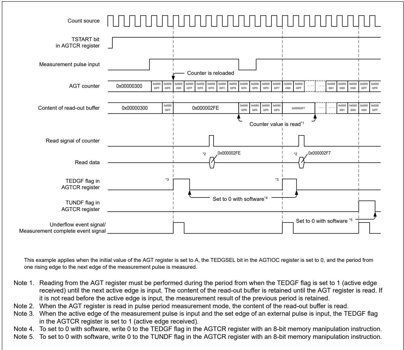
Figure 21.11 Operation example in pulse period measurement mode
