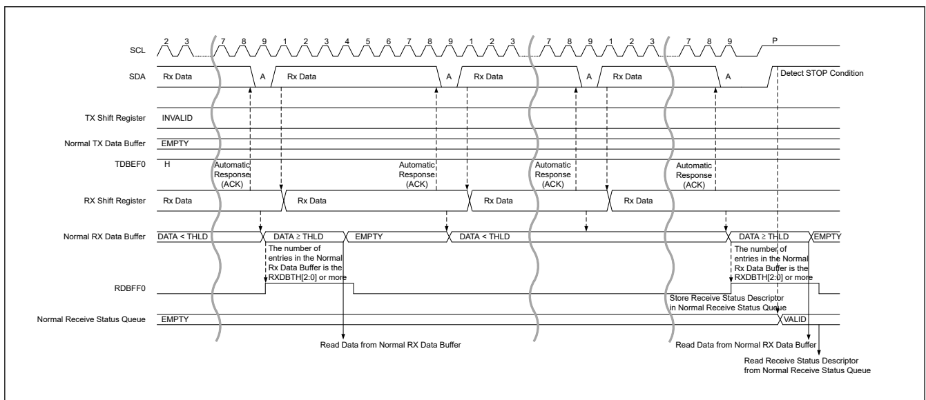
Figure 28.38 Legacy I 2 C message data write transfer timing (2/2)
