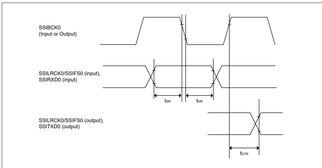
Figure 41.48 SSIE data transmit and receive timing when SSICR.BCKP = 1
