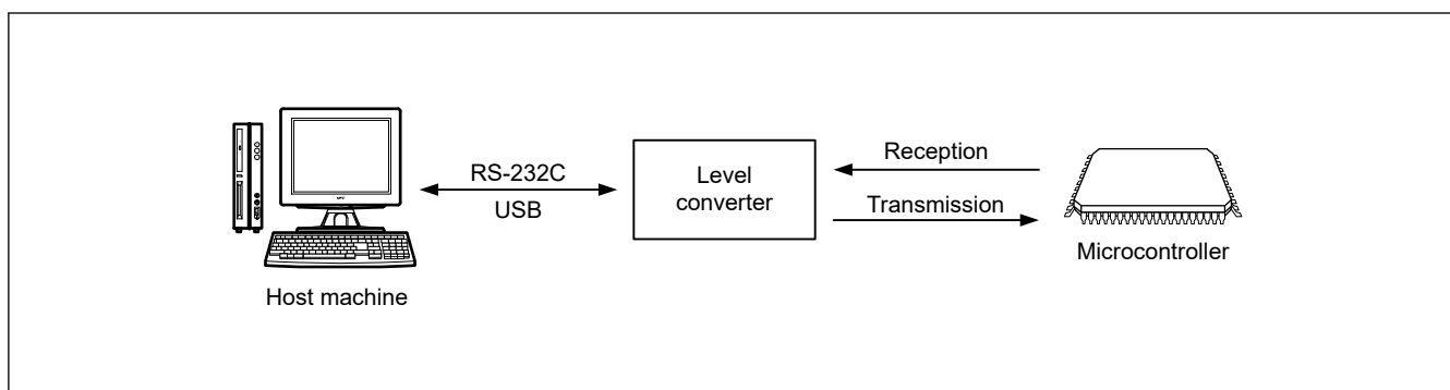
Figure 38.11 Environment for writing programs to the flash memory
