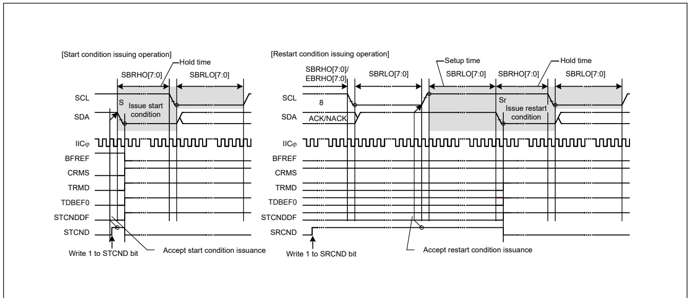
Figure 28.55 START condition / repeated START condition issue timing (STCND and SRCND bits)
