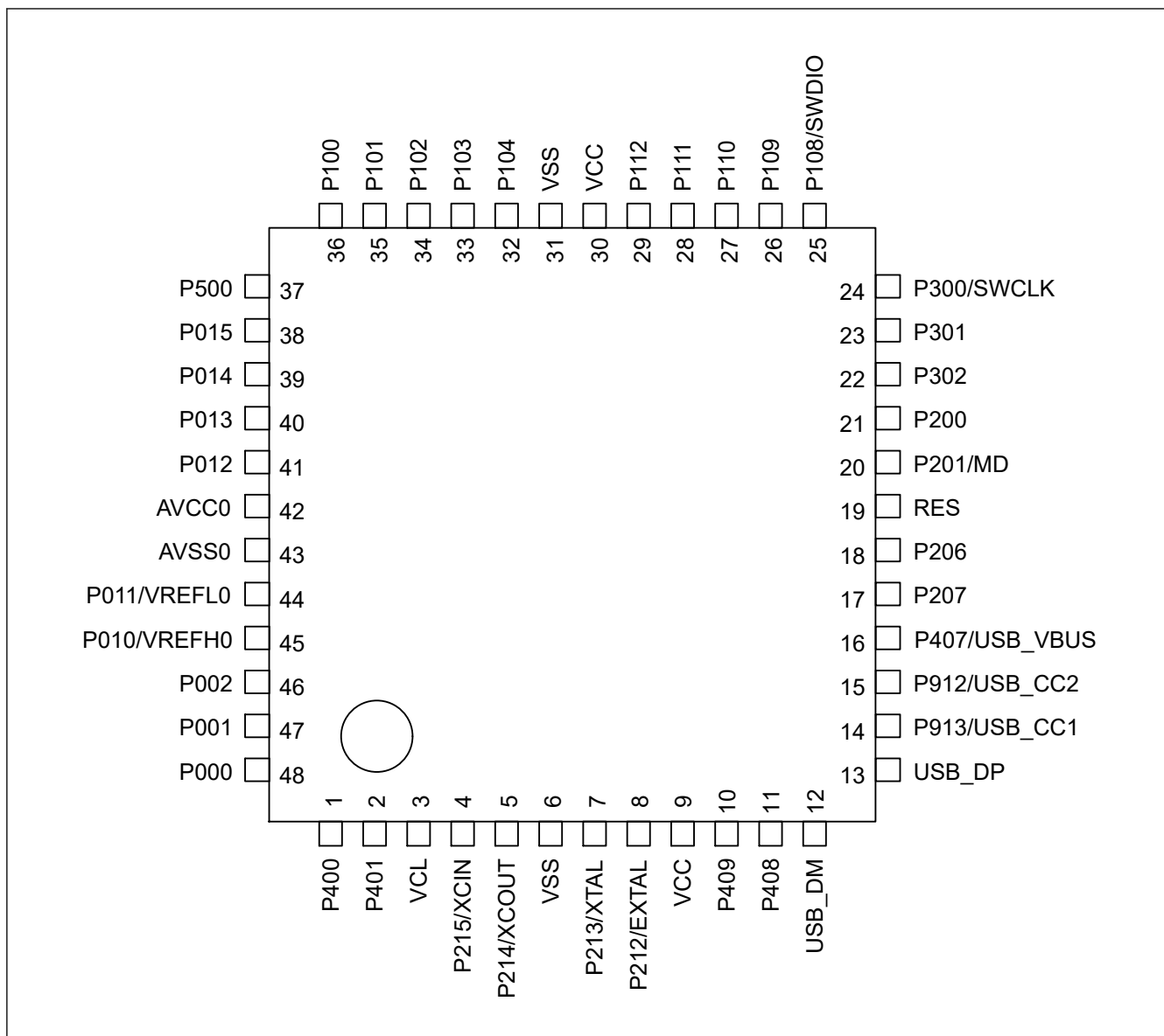
Figure 1.4 Pin assignment for LQFP/QFN 48-pin (top view)
