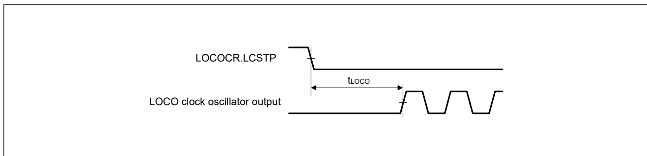
Figure 41.4 LOCO clock oscillation start timing
