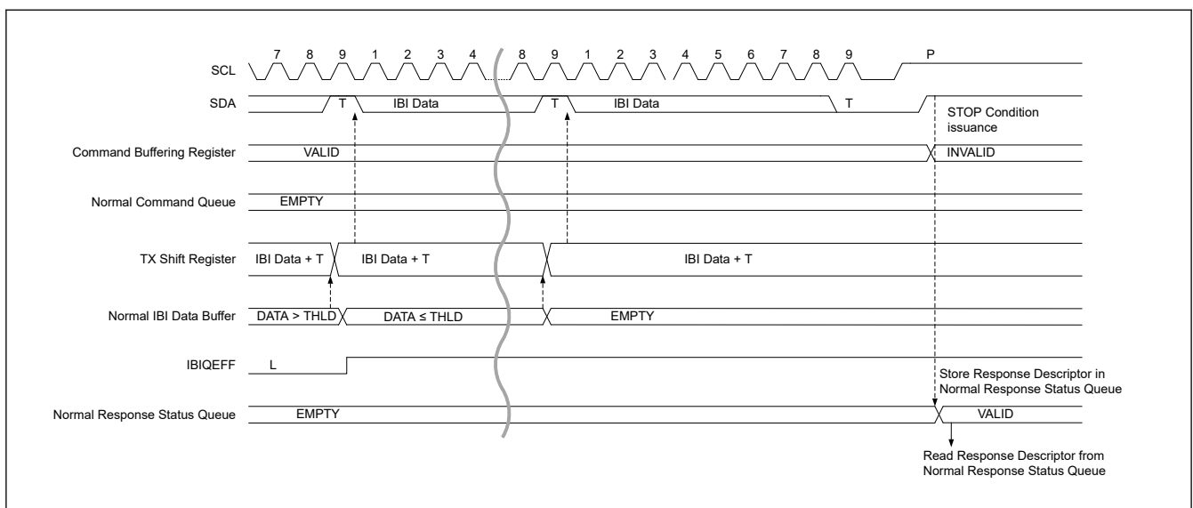
Figure 28.44 I3C slave IBI transfer timing (2/2)
