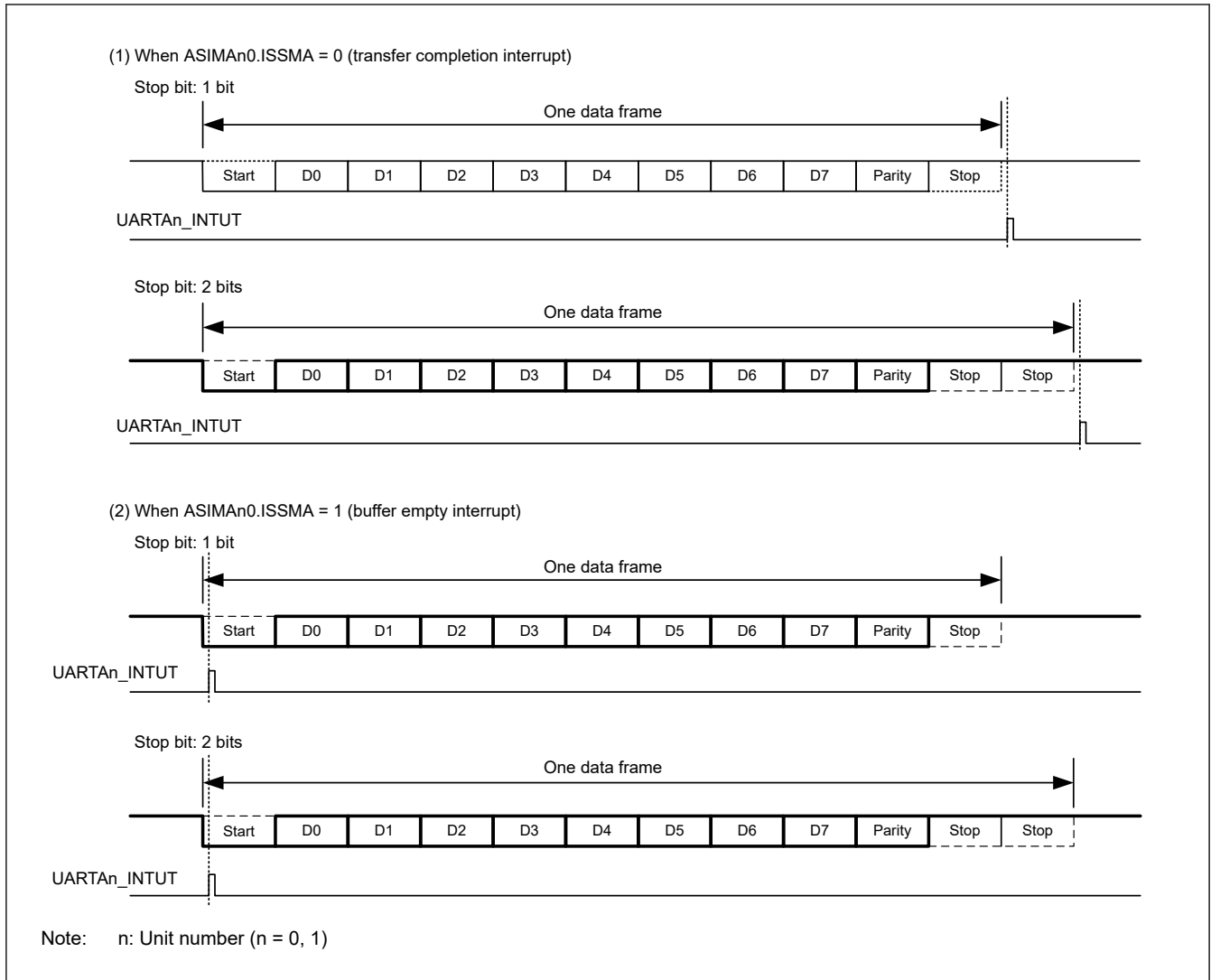
Figure 31.4 Interrupt output timing
