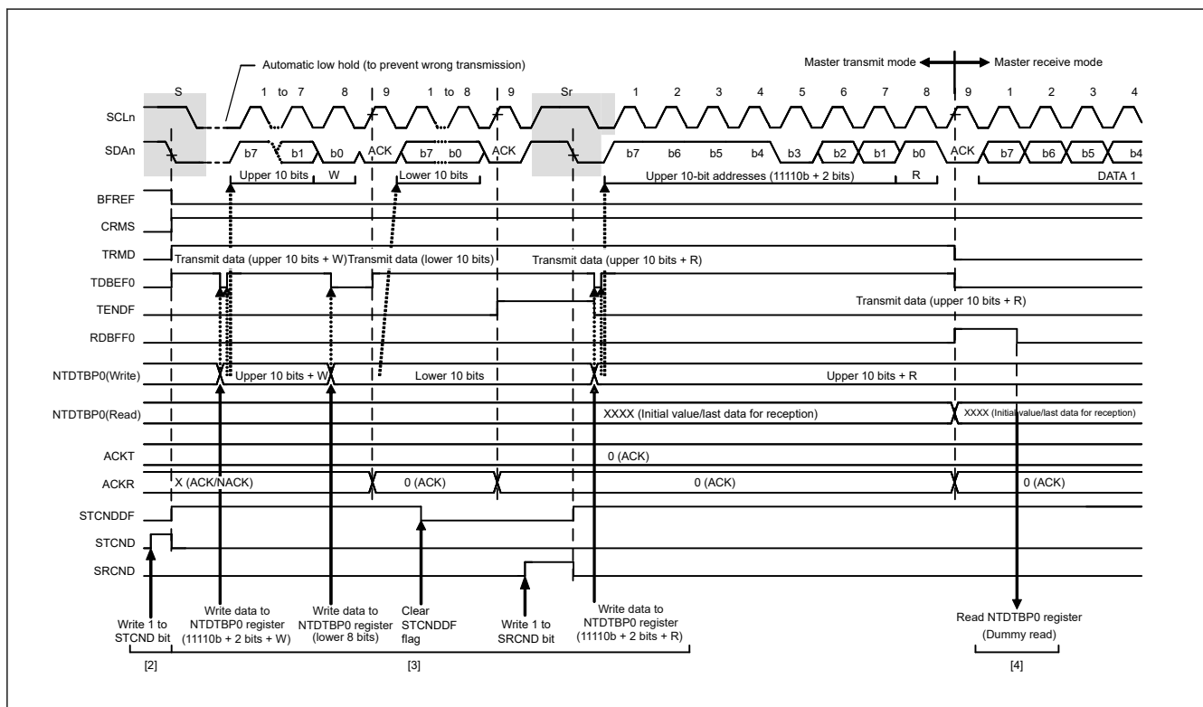
Figure 28.10 Master receive operation timing (2) (10-bit address format, when ACKTWE = 0)
