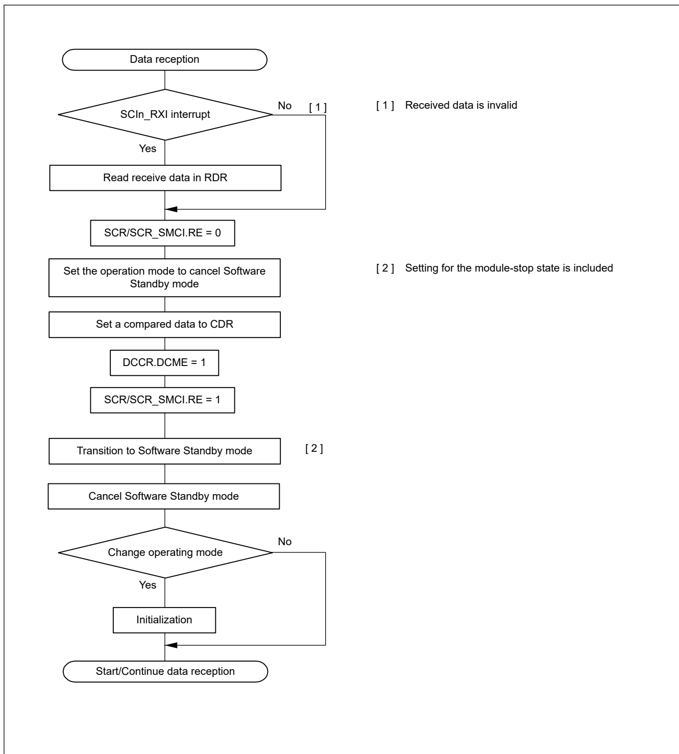
Figure 27.76 Example flow of transition to Software Standby mode during reception with address match
