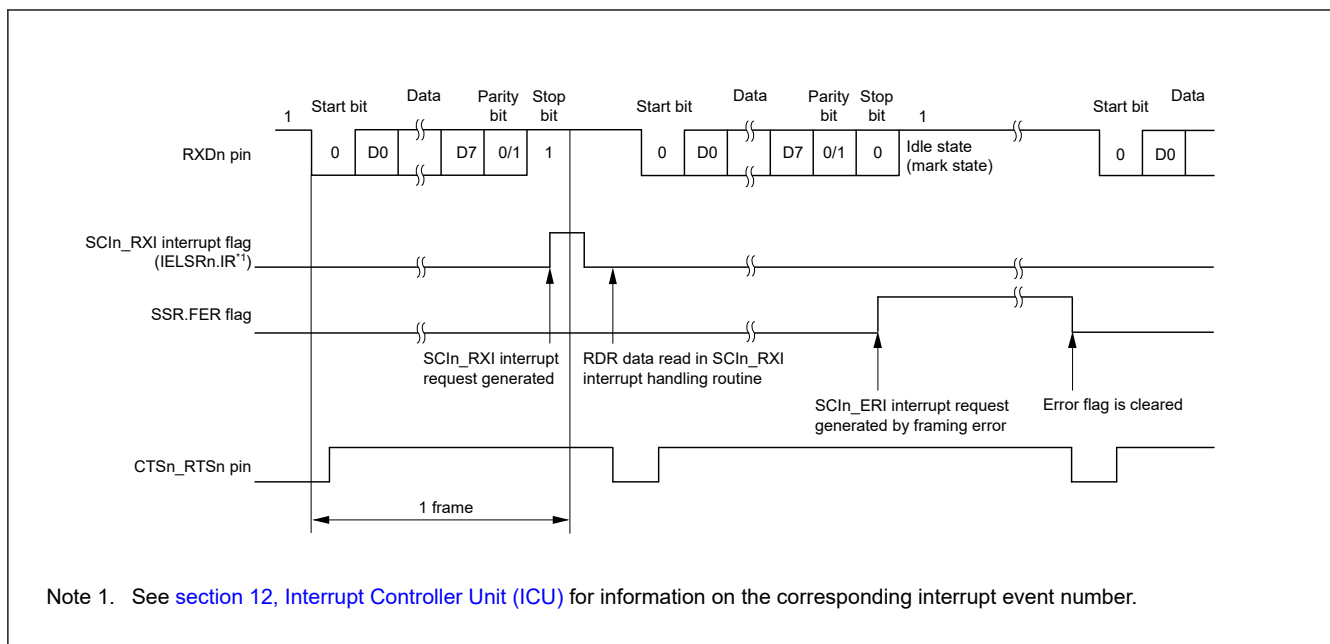
Figure 27.14 Example of SCI operation for serial reception in asynchronous mode (2) when RTS function is used, and with 8-bit data, parity bit, and 1 stop bit
