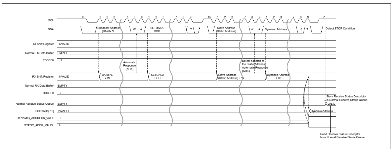
Figure 28.34 Dynamic address assign procedure (SETDASA CCC) timing
