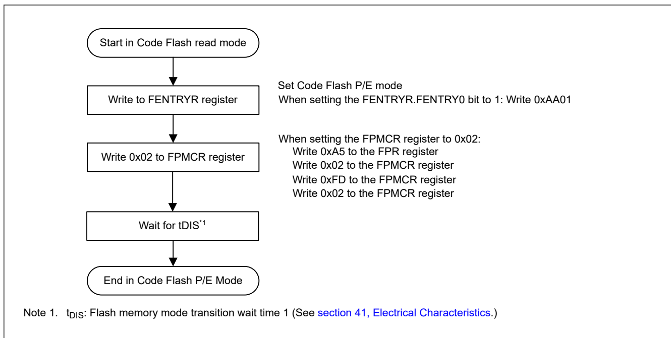
Figure 38.15 Procedure for changing from read mode to code flash P/E mode
