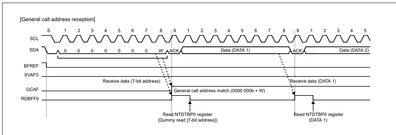
Figure 28.60 Timing of GCAF flag setting during reception of general call address
