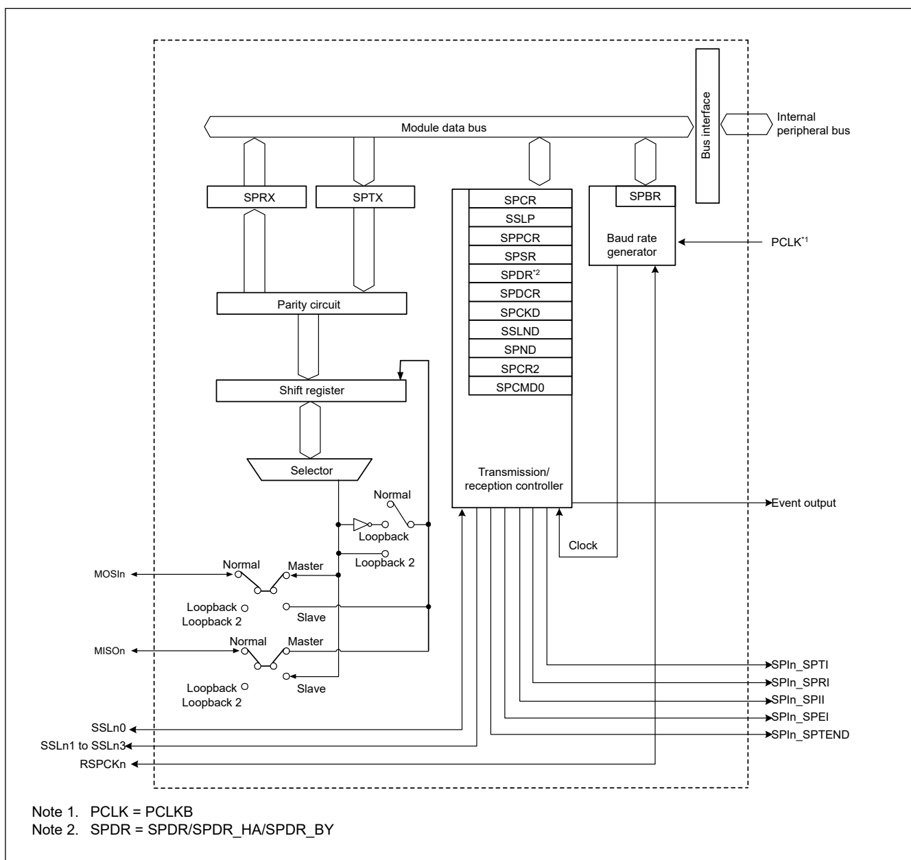
Figure 30.1 SPI block diagram
