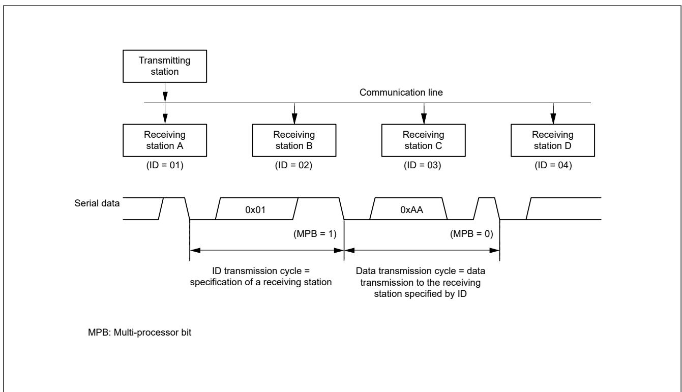
Figure 27.26 Example of communication using multi-processor format with transmission of data 0xAA to receiving station A
