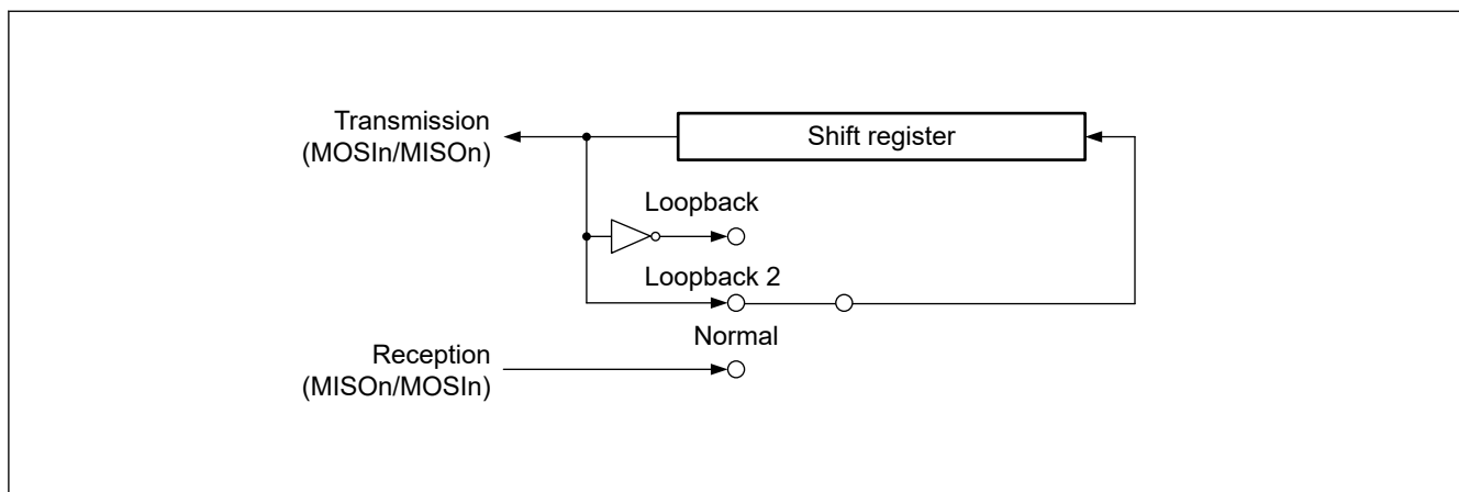
Figure 30.42 Configuration of shift register I/O paths in loopback mode for master mode
