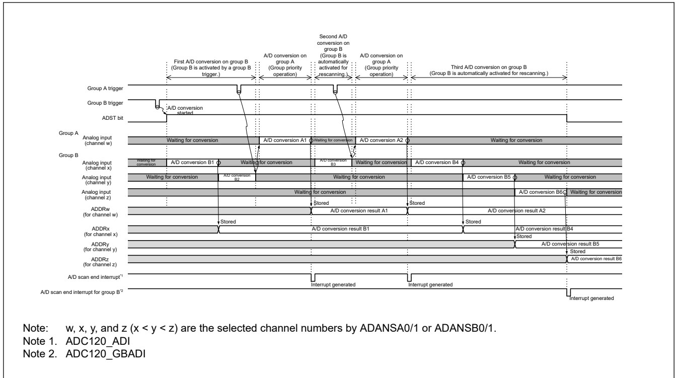
Figure 34.18 Example of group priority operation 1-2: Group A trigger input during rescanning of group B when rescanning is enabled (when ADGSPCR.GBRSCN = 1, ADGSPCR.GBRP = 0)
