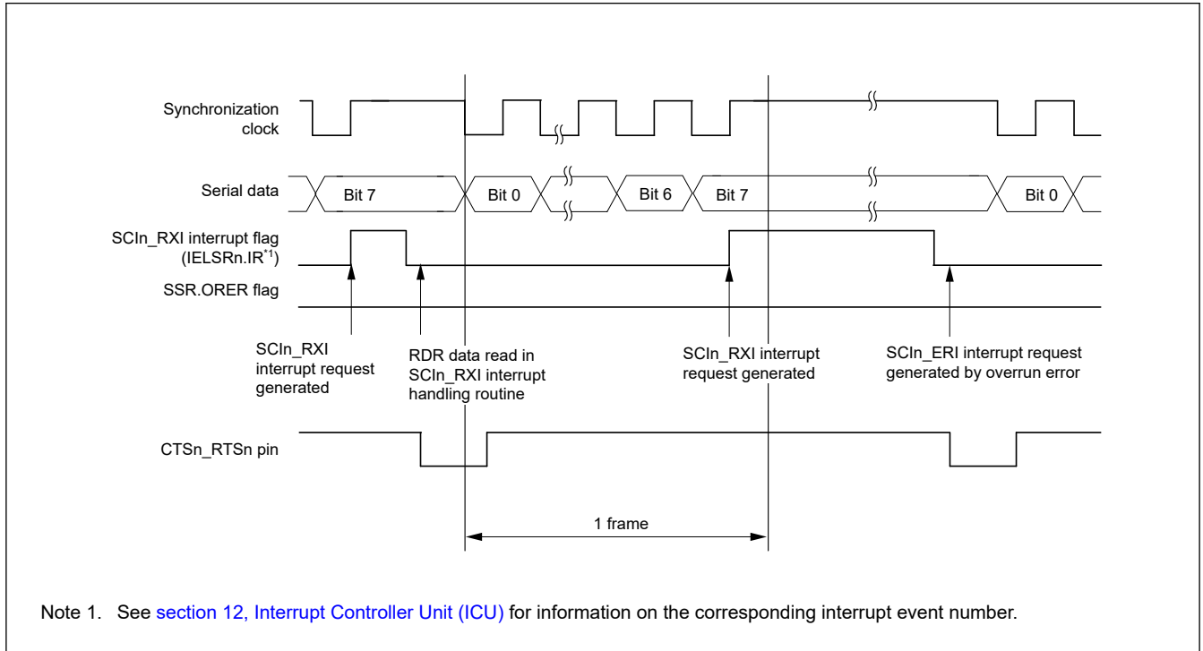
Figure 27.42 Example operation for serial reception in clock synchronous mode (2) when RTS function is used
