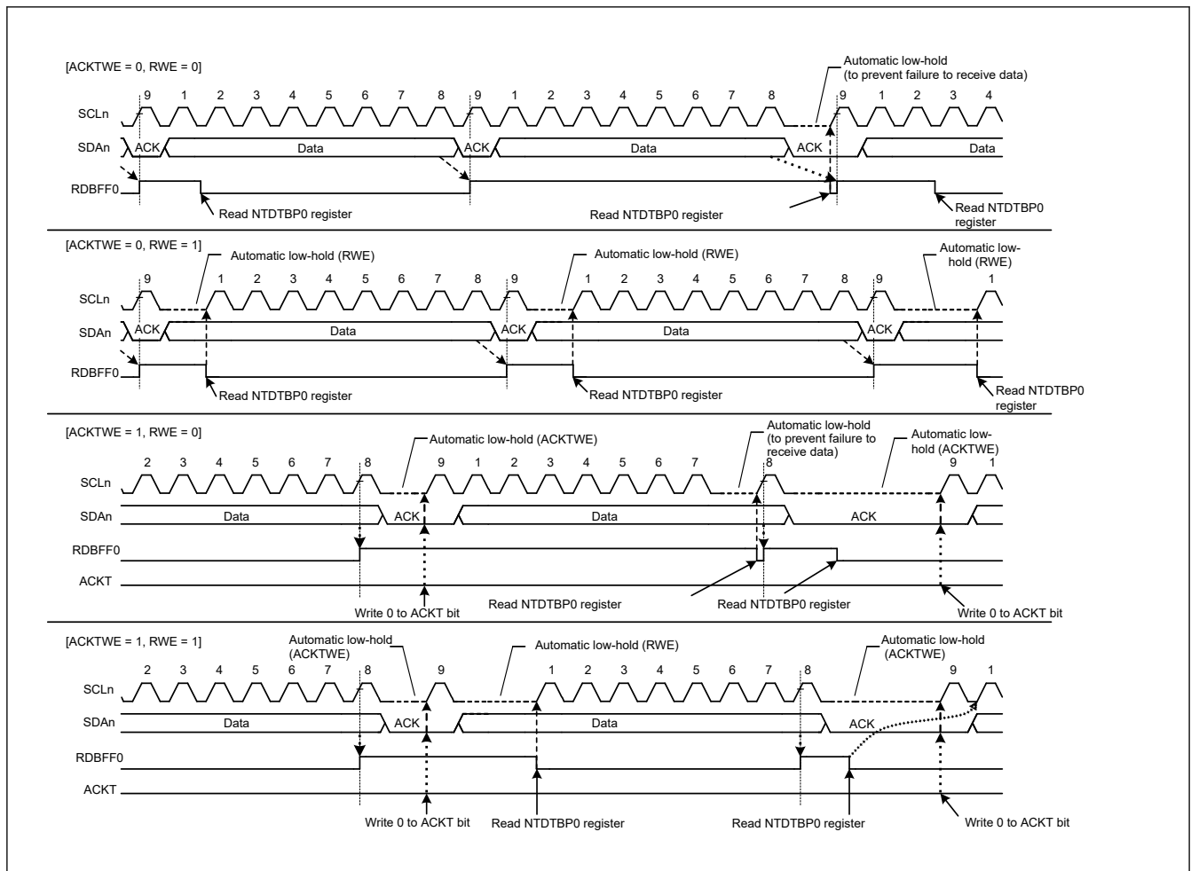
Figure 28.70 Automatic low-hold operation in receive mode (using ACKTWE and RWE bits)
