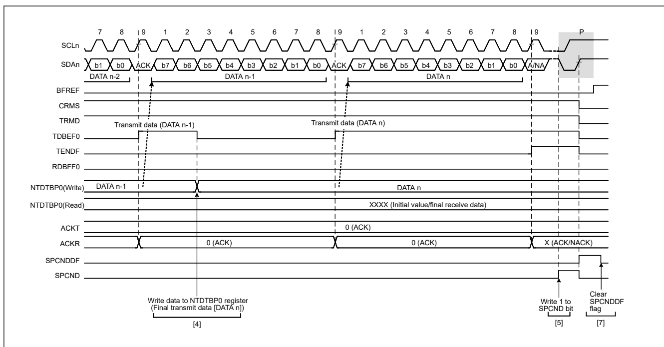
Figure 28.8 Master transmit operation timing (3)
