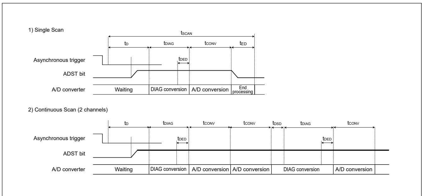
Figure 34.26 Scan conversion timing when activated by an asynchronous trigger input (ADTRG0)
