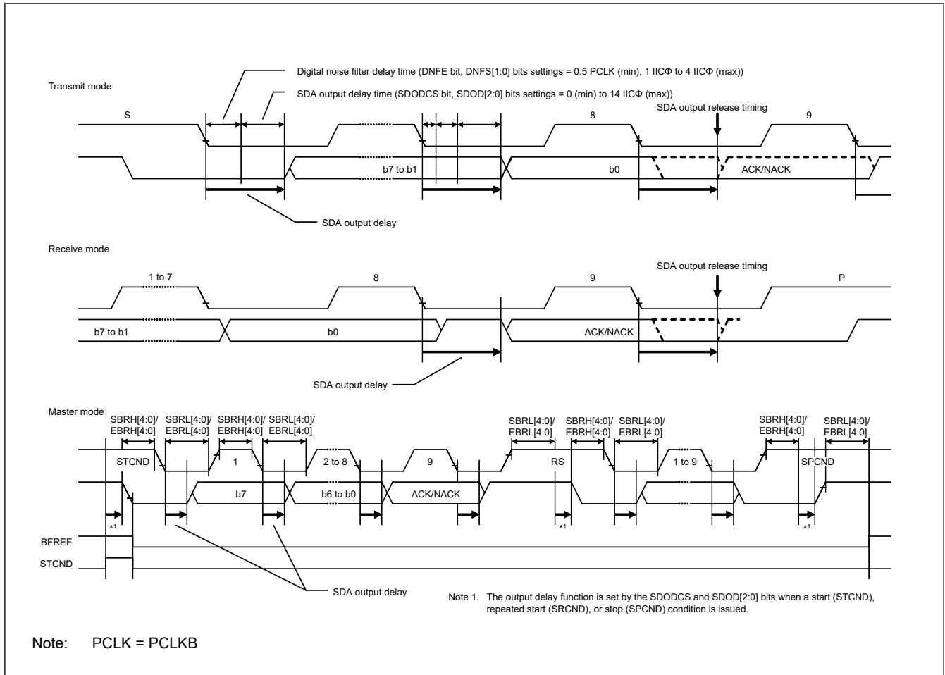
Figure 28.98 SDA output delay facility
