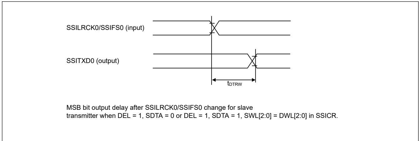
Figure 41.49 SSIE data output delay after SSILRCK0/SSIFS0 change
