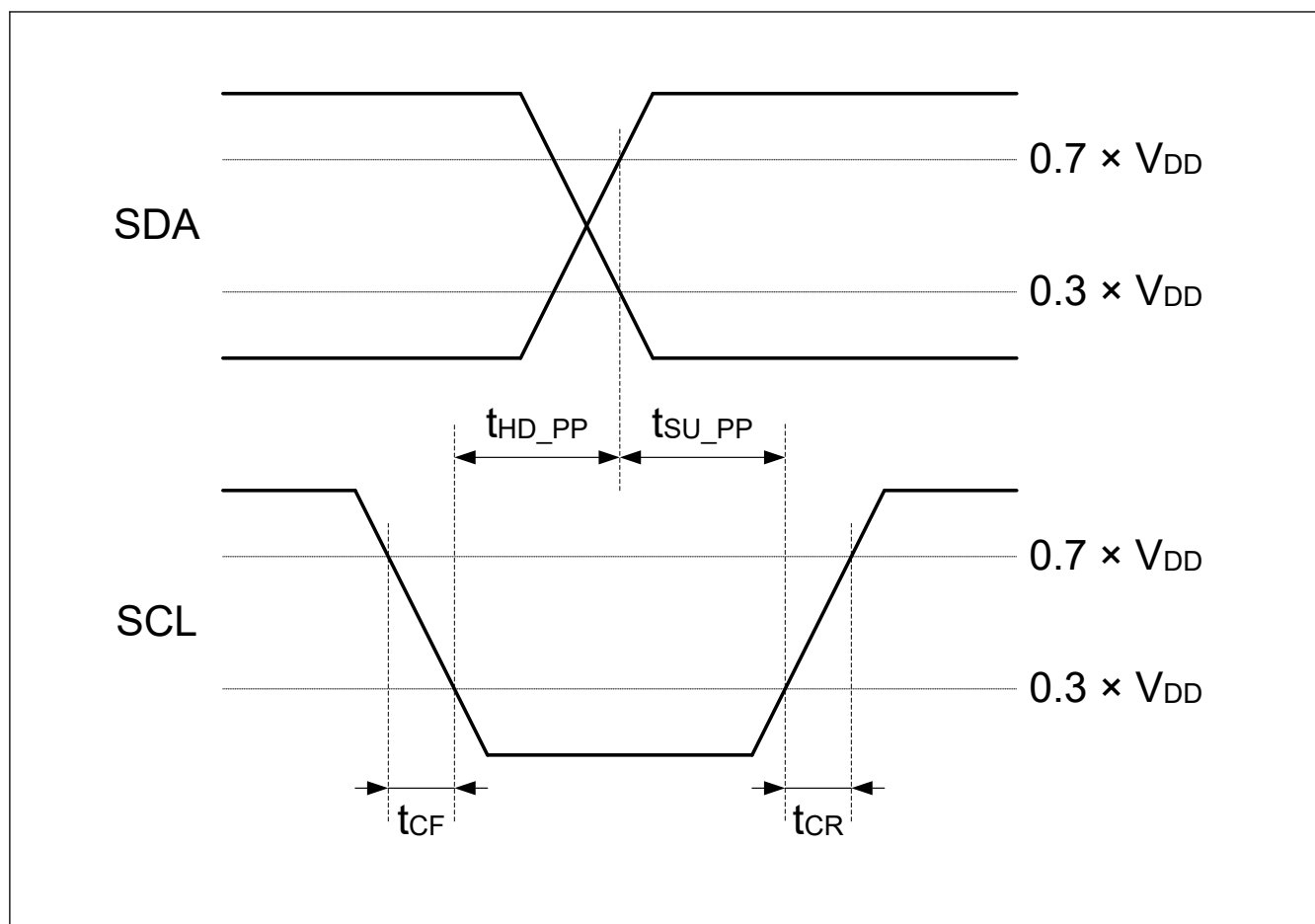
Figure 41.40 I3C Master Out Timing
