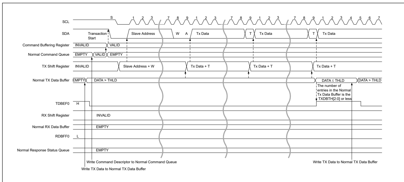
Figure 28.16 SDR data write transfer timing (1/2)
