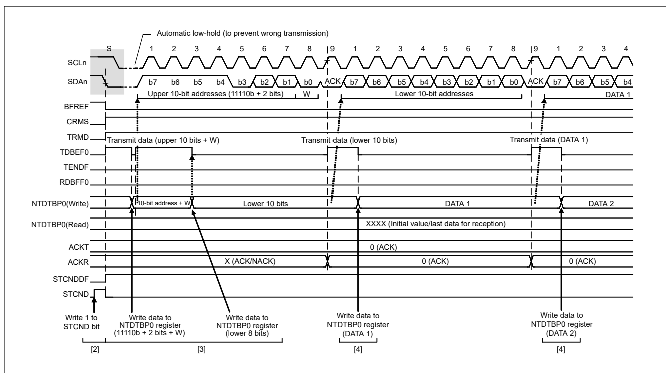
Figure 28.7 Master transmit operation timing (2) (10-bit address format)
