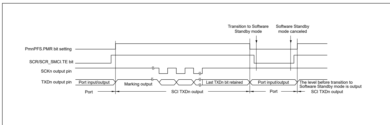
Figure 27.74 Port pin states during transition to Software Standby mode with internal clock and clock synchronous transmission
