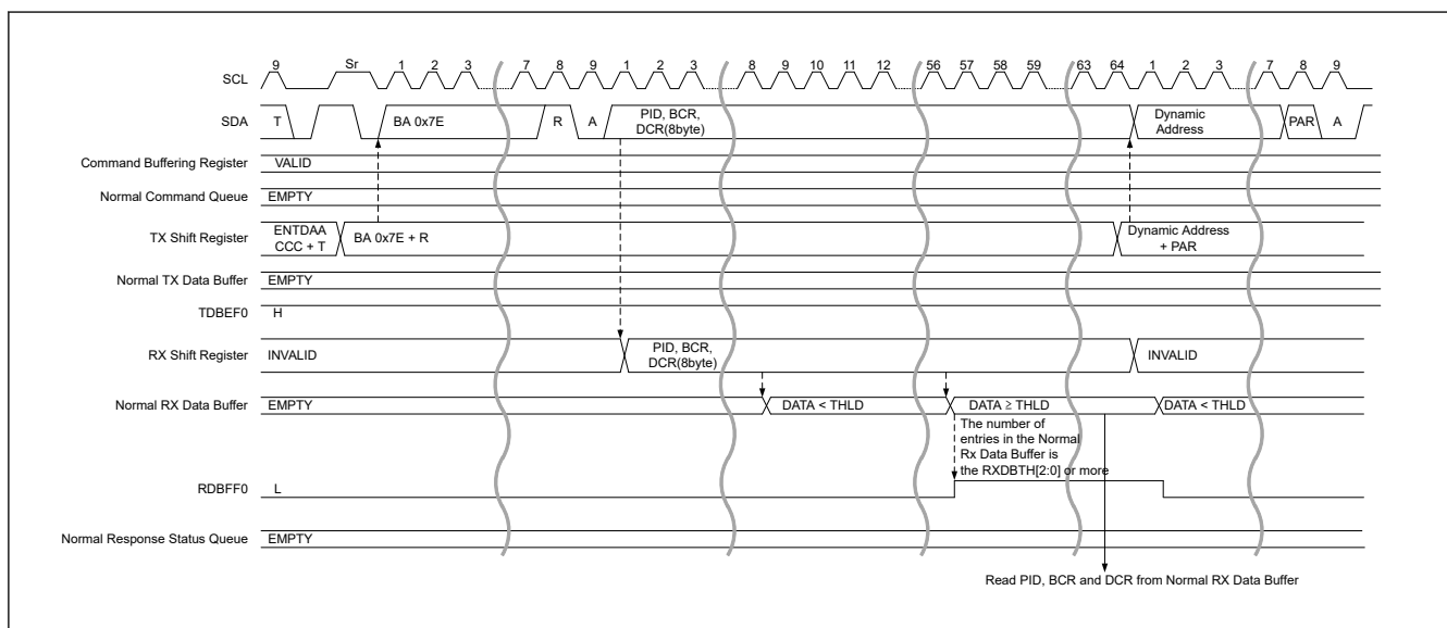
Figure 28.13 Dynamic address assign procedure (ENTDAA CCC) timing (2/3)
