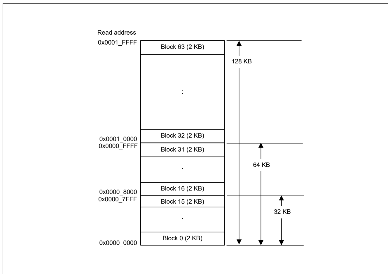
Figure 38.2 Mapping of the code flash memory
