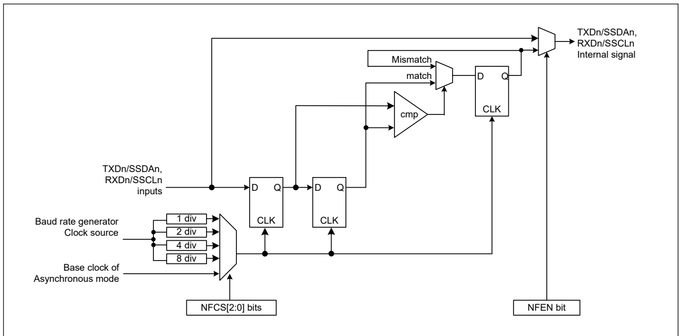
Figure 27.71 Digital noise filter circuit block diagram
