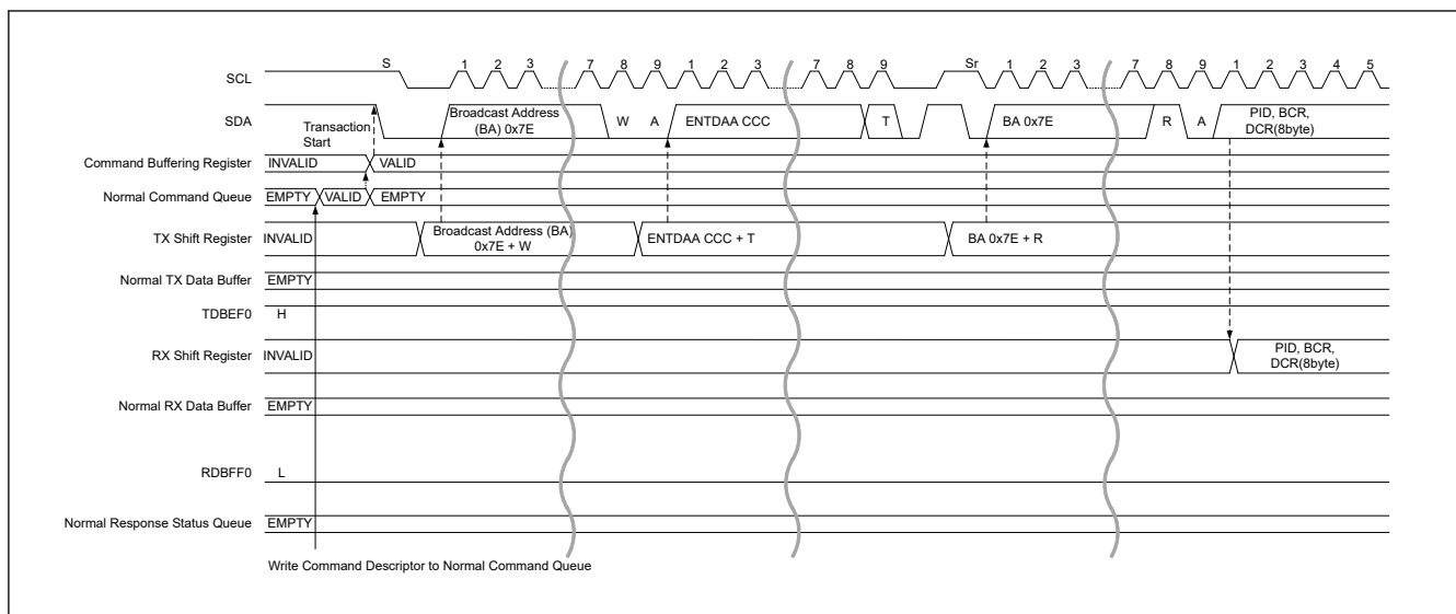
Figure 28.12 Dynamic address assign procedure (ENTDAA CCC) timing (1/3)
