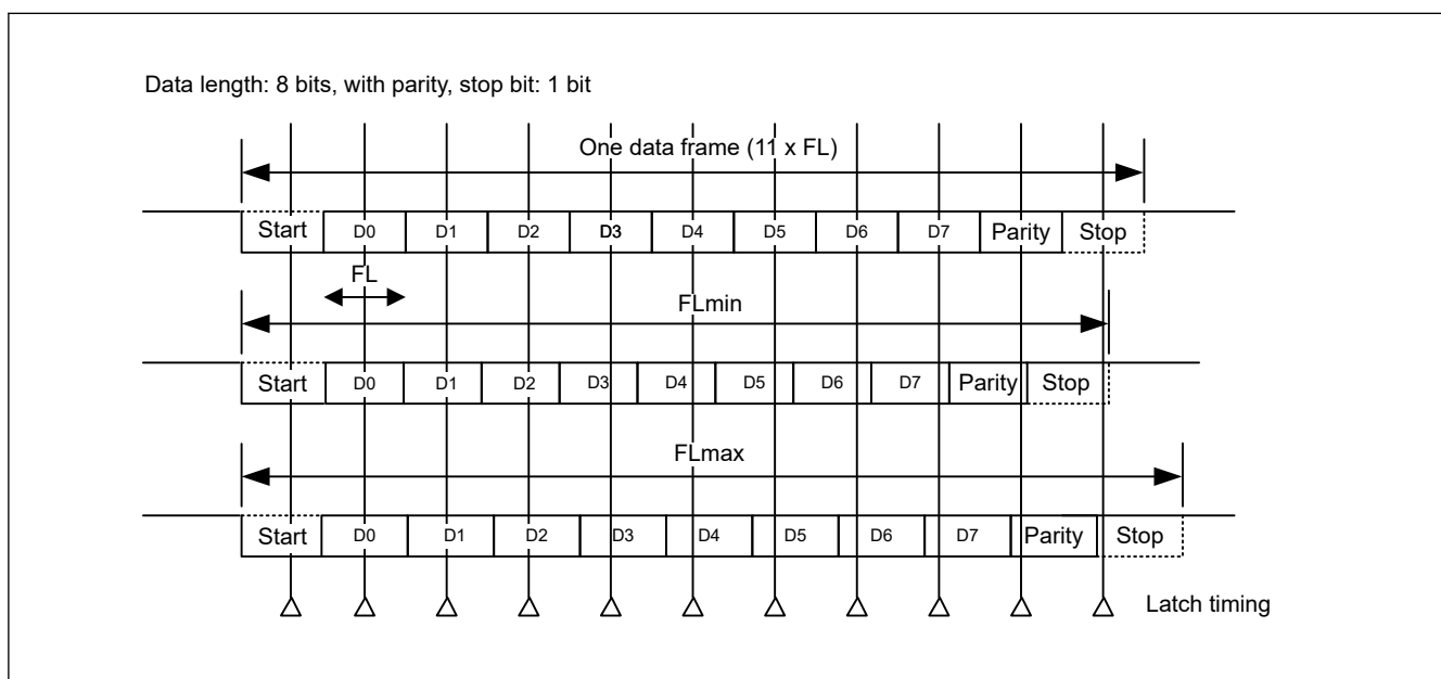
Figure 31.11 Permissible baud rate range during reception
