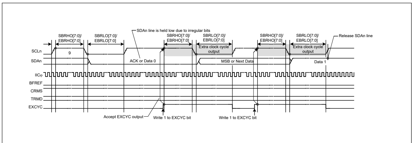
Figure 28.90 Extra SCL clock cycle output function (EXCYC bit)
