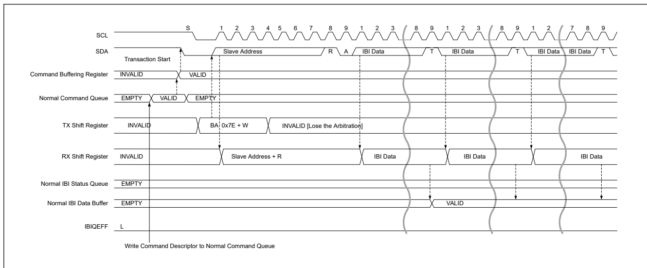
Figure 28.24 I3C master IBI transfer timing (1/2)
