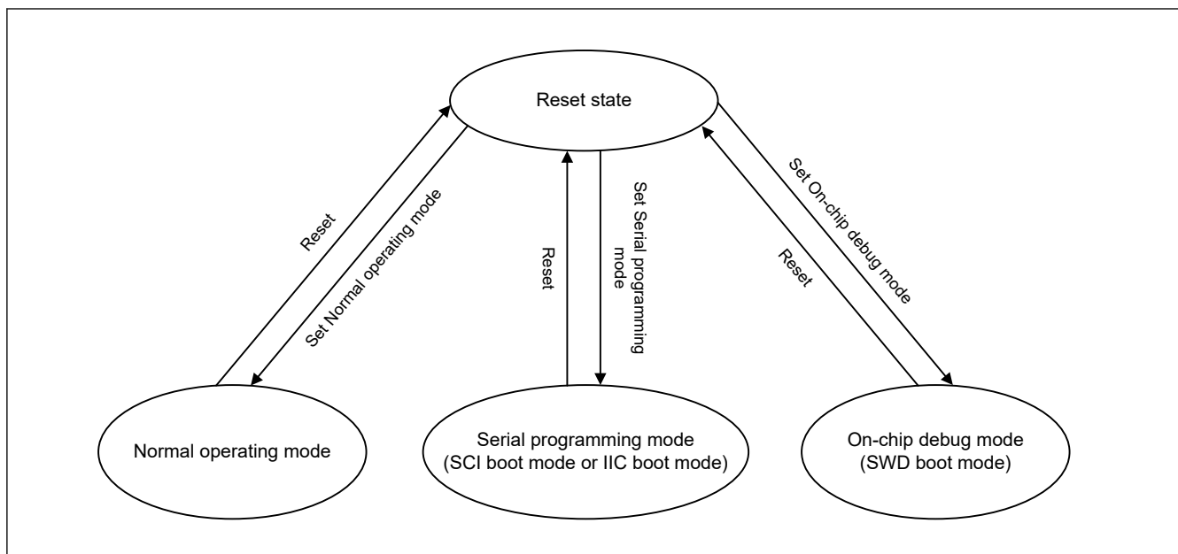
Figure 38.4 Mode transitions associated with flash memory
