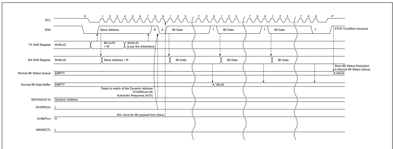
Figure 28.77 Slave interrupt request : ACK and DVIBIPL = 1
