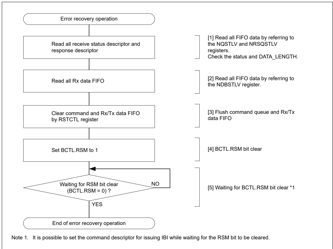
Figure 28.96 Example of error recovery operation flowchart for I3C slave
