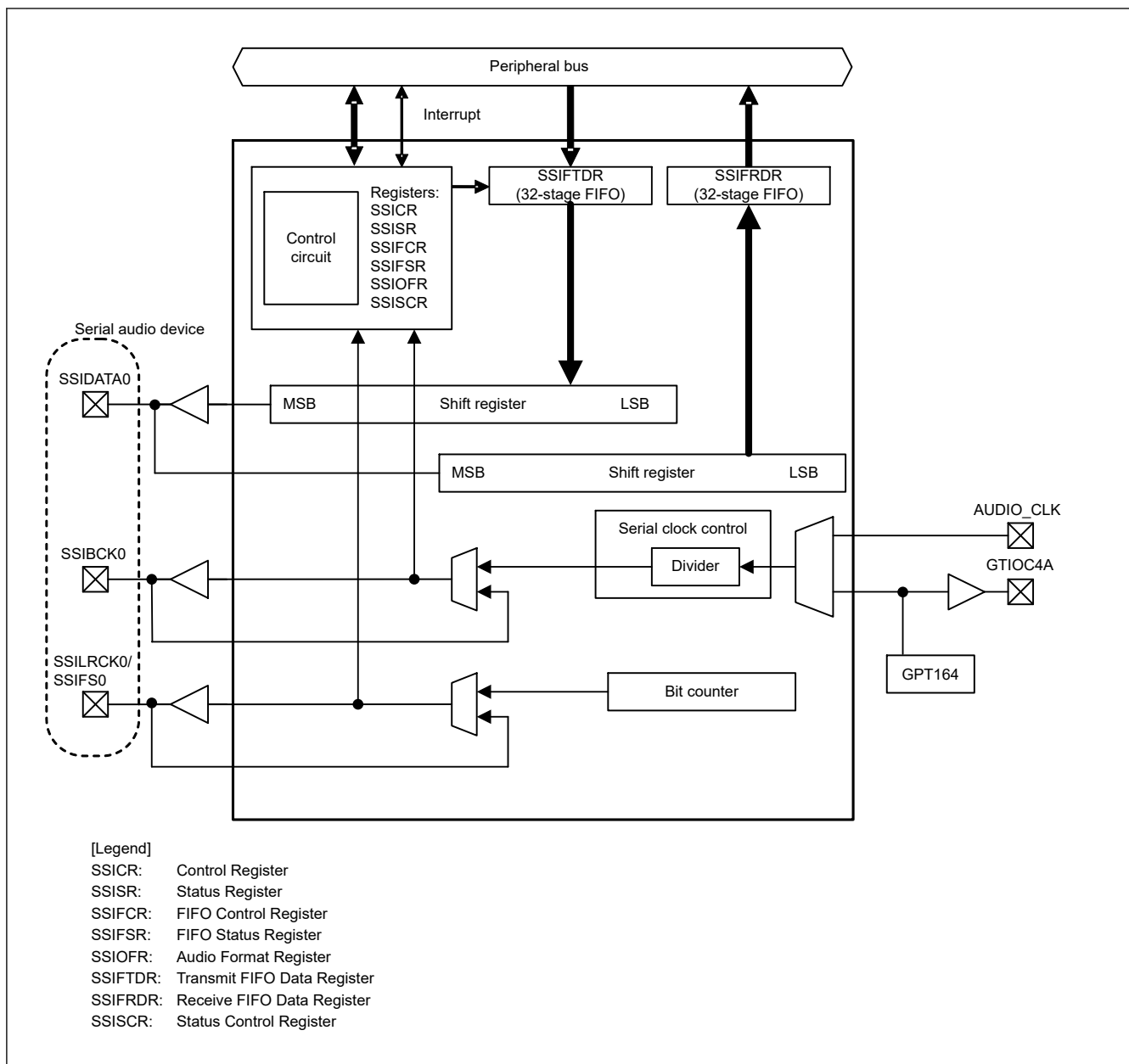
Figure 32.3 SSIE block diagram for half-duplex communication
