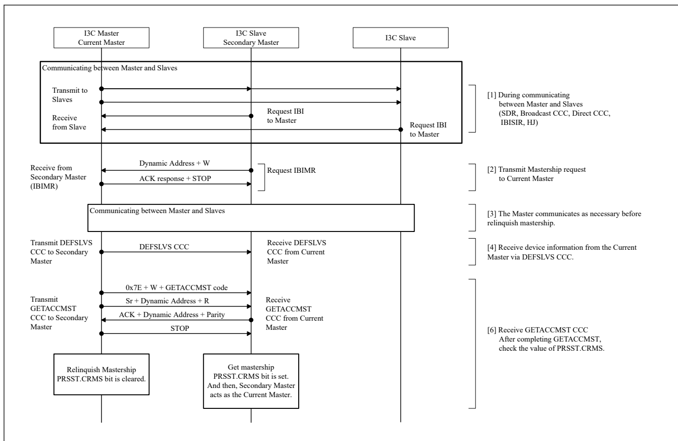
Figure 28.45 I3C slave mastership processing flow
