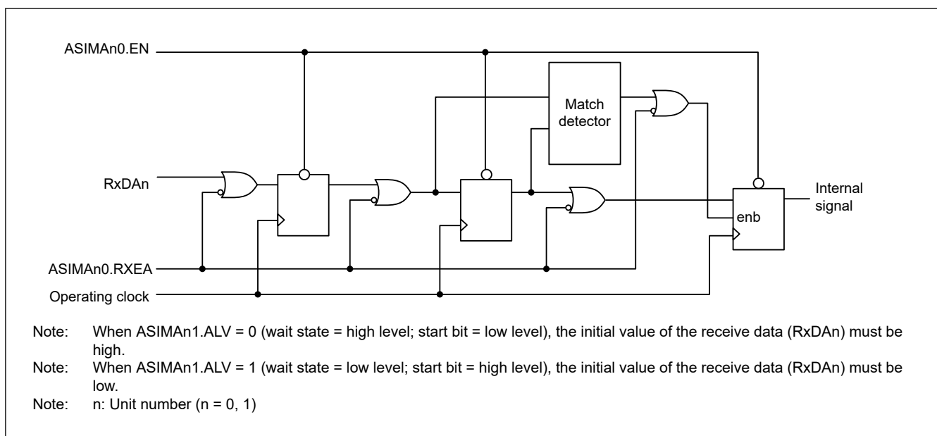
Figure 31.9 Noise filter
