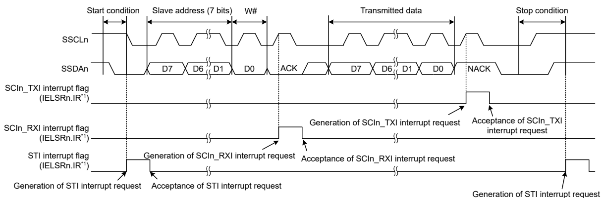
Figure 27.64 Example 2 of operations for master transmission in simple IIC mode with 7-bit slave addresses, ACK interrupts, and NACK interrupts
