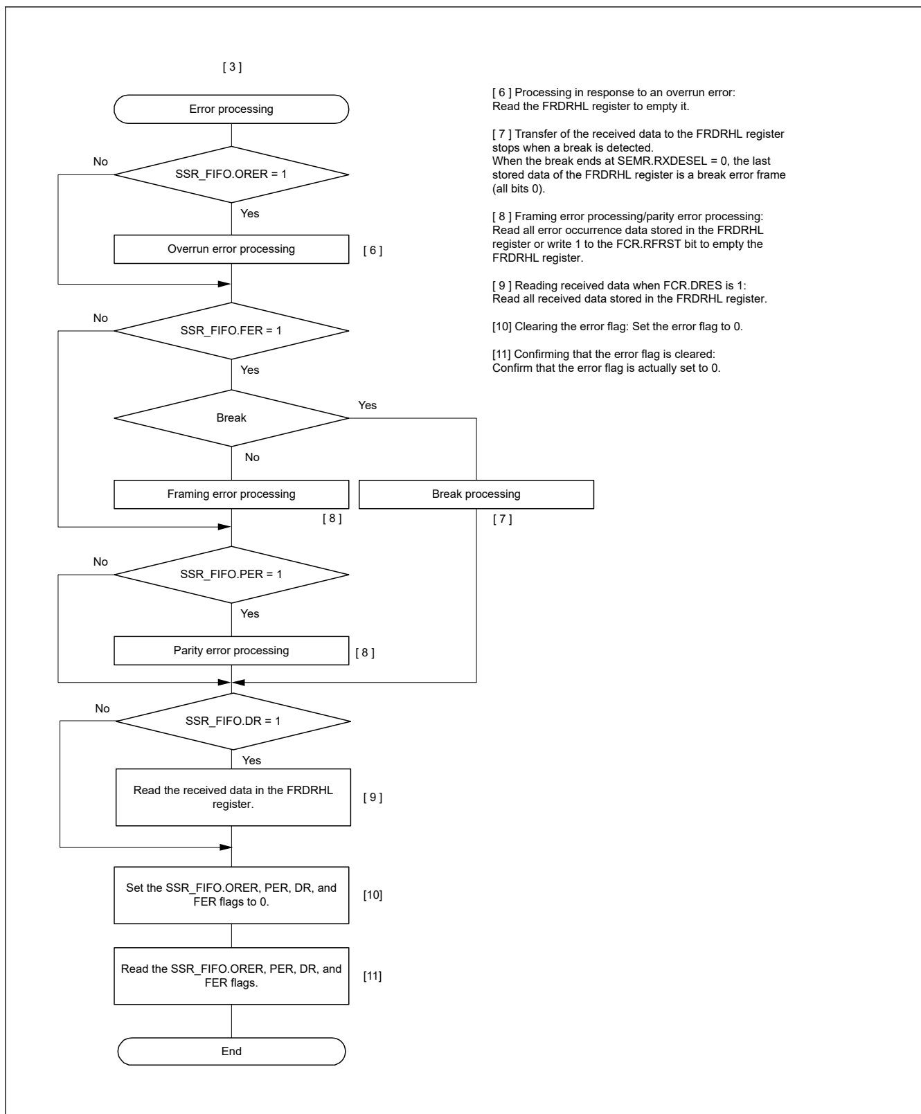
Figure 27.25 Example Flowchart of Serial Reception in Asynchronous Mode (FIFO Selected and Address Matching Enabled) (3)
