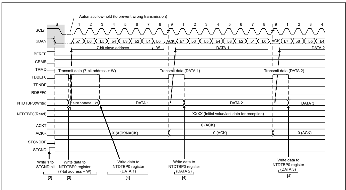
Figure 28.6 Master transmit operation timing (1) (7-bit address format)
