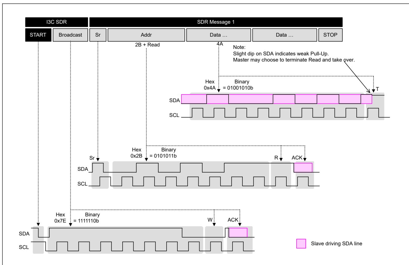
Figure 28.50 Example communication using I3C coding SDR with broadcast (0x7E)
