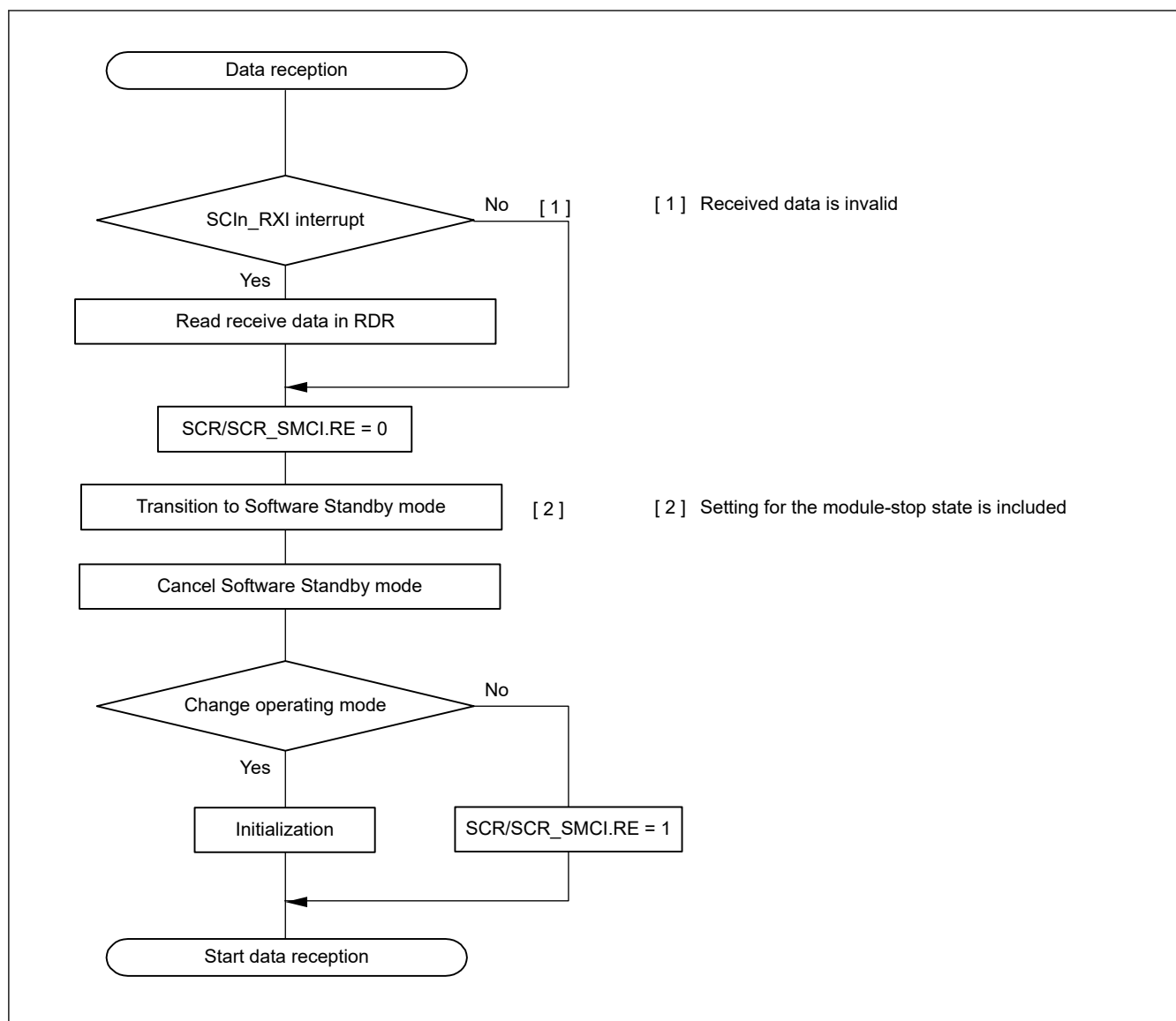
Figure 27.75 Example flow of transition to Software Standby mode during reception
