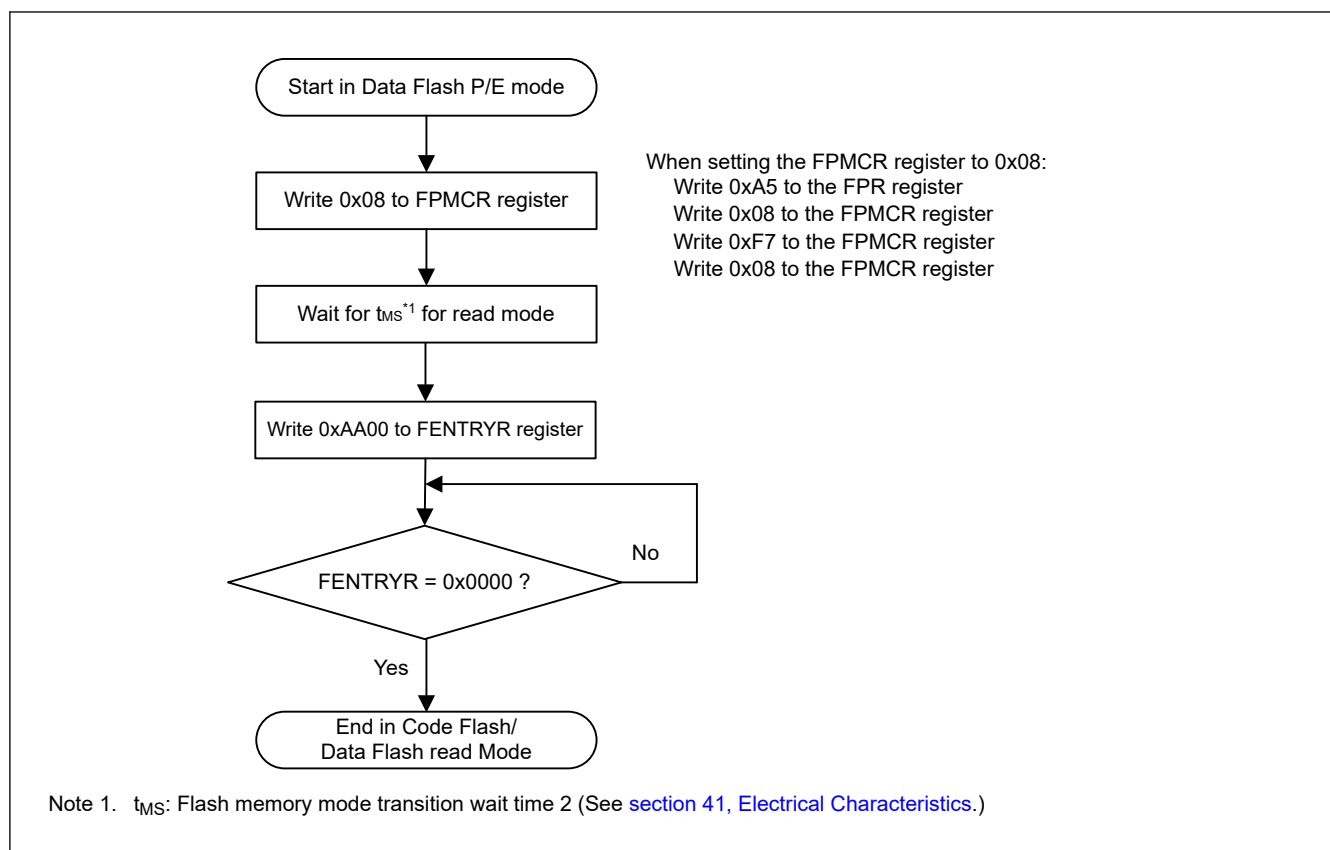
Figure 38.18 Procedure for changing from data flash P/E mode to read mode
