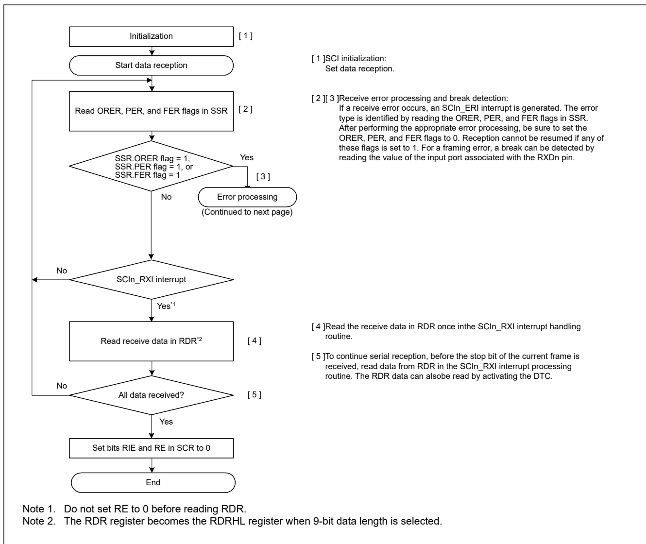
Figure 27.15 Example flow of serial reception in asynchronous mode with non-FIFO selected and Address Matching Disabled (1)
