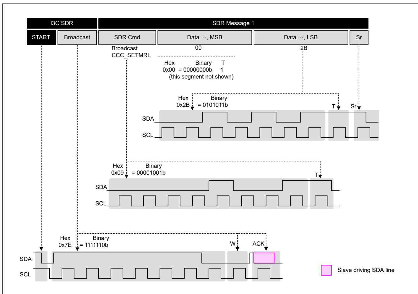
Figure 28.53 Example communication using I3C coding SDR with CCC broadcast
