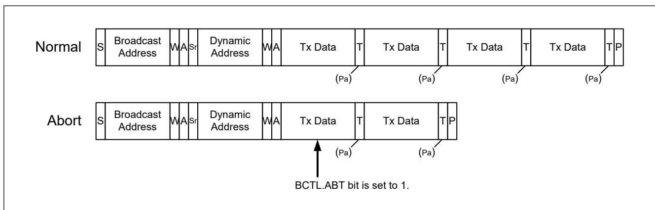
Figure 28.93 Abort operation of SDR write transfer
