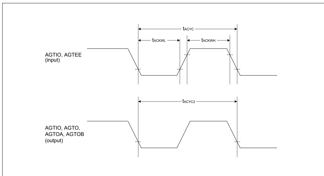
Figure 41.17 AGTW I/O timing
