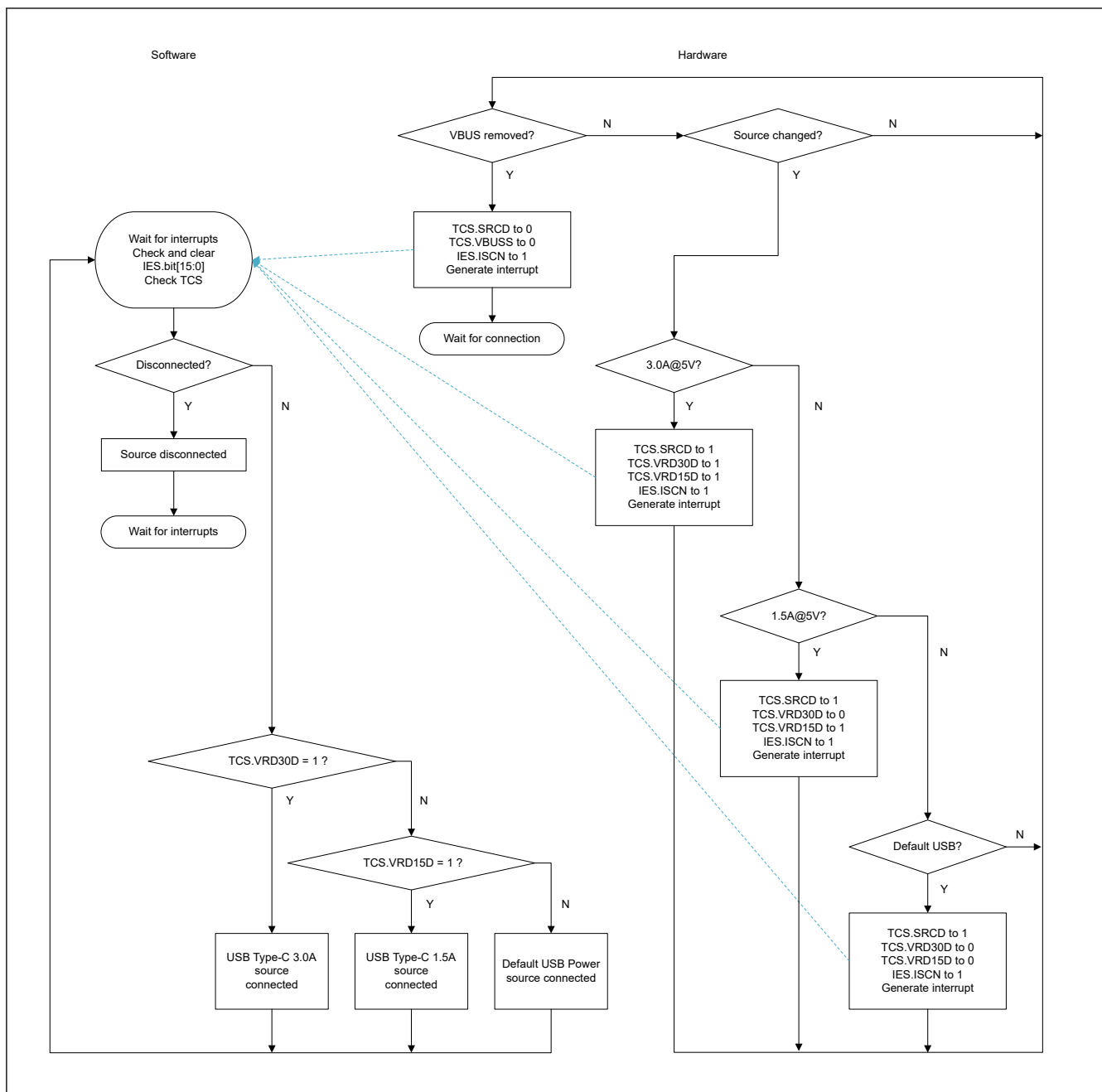
Figure 26.4 Sink-only mode 1.5A/3.0A source detection and disconnection detection flow
