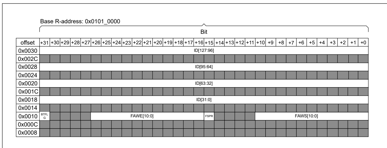
Figure 38.5 Configuration area bit map
