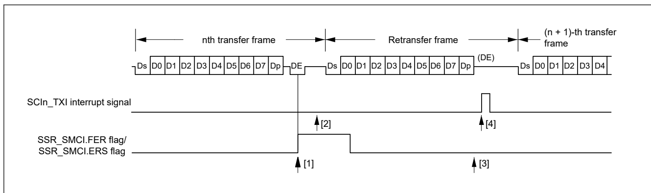
Figure 27.52 Data re-transfer operation in smart card interface transmission mode
