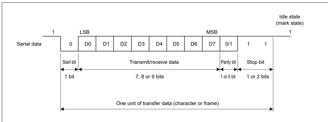
Figure 27.2 Data format in asynchronous serial communications with 8-bit data, parity bit, and 2 stop bits
