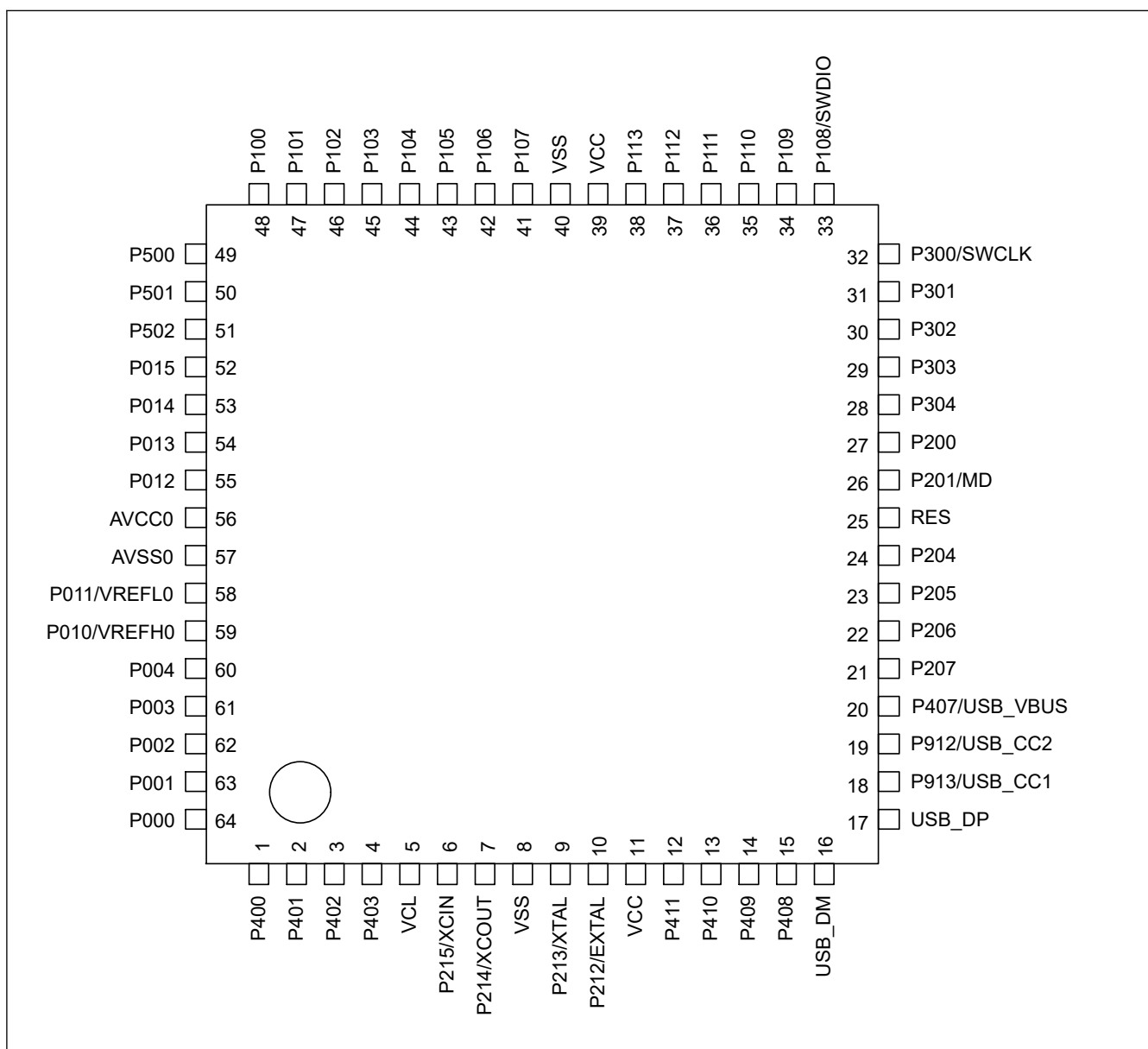
Figure 1.3 Pin assignment for LQFP 64-pin (top view)
