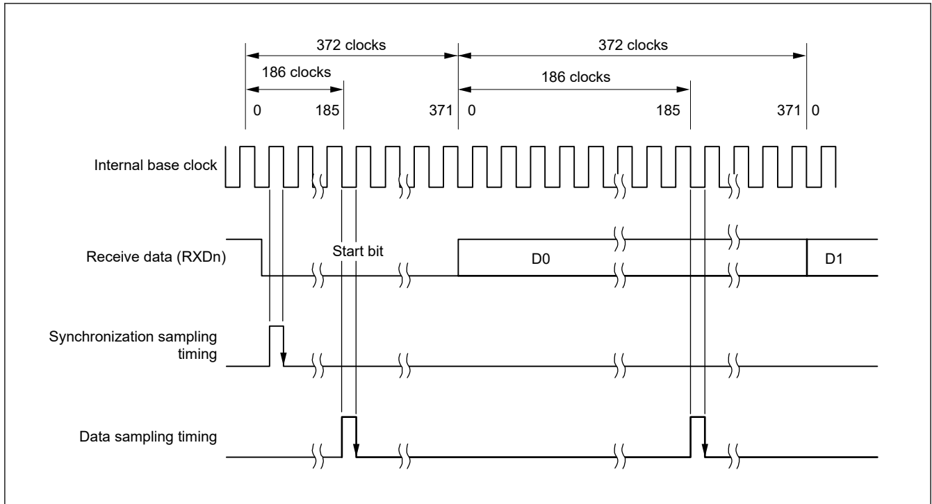
Figure 27.51 Receive data sampling timing in smart card interface mode when the clock frequency is 372 times the bit rate
