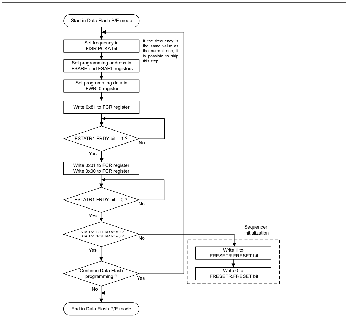
Figure 38.20 Flowchart for programming of the data flash
