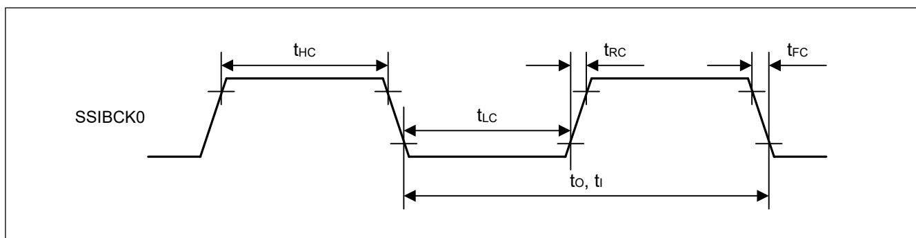
Figure 41.45 SSIE clock input/output timing
