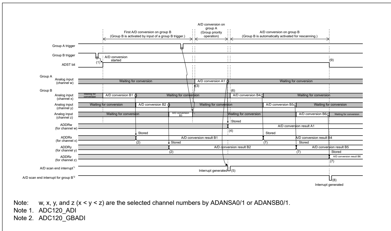
Figure 34.17 Example of group priority operation 1-1: Group A trigger input during group B scanning when rescanning is enabled (when ADGSPCR.GBRSCN = 1, ADGSPCR.GBRP = 0)
