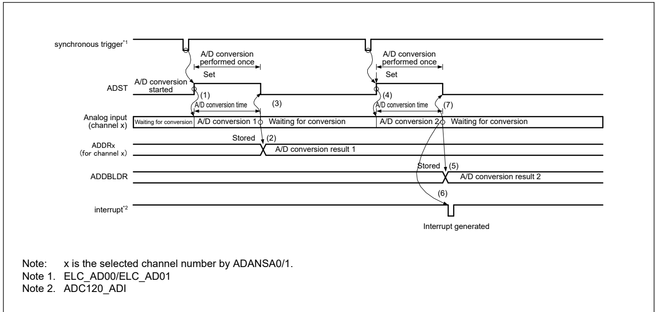
Figure 34.10 Example operation in single scan mode when double-trigger mode is selected and the analog input (channel x) is duplicated
