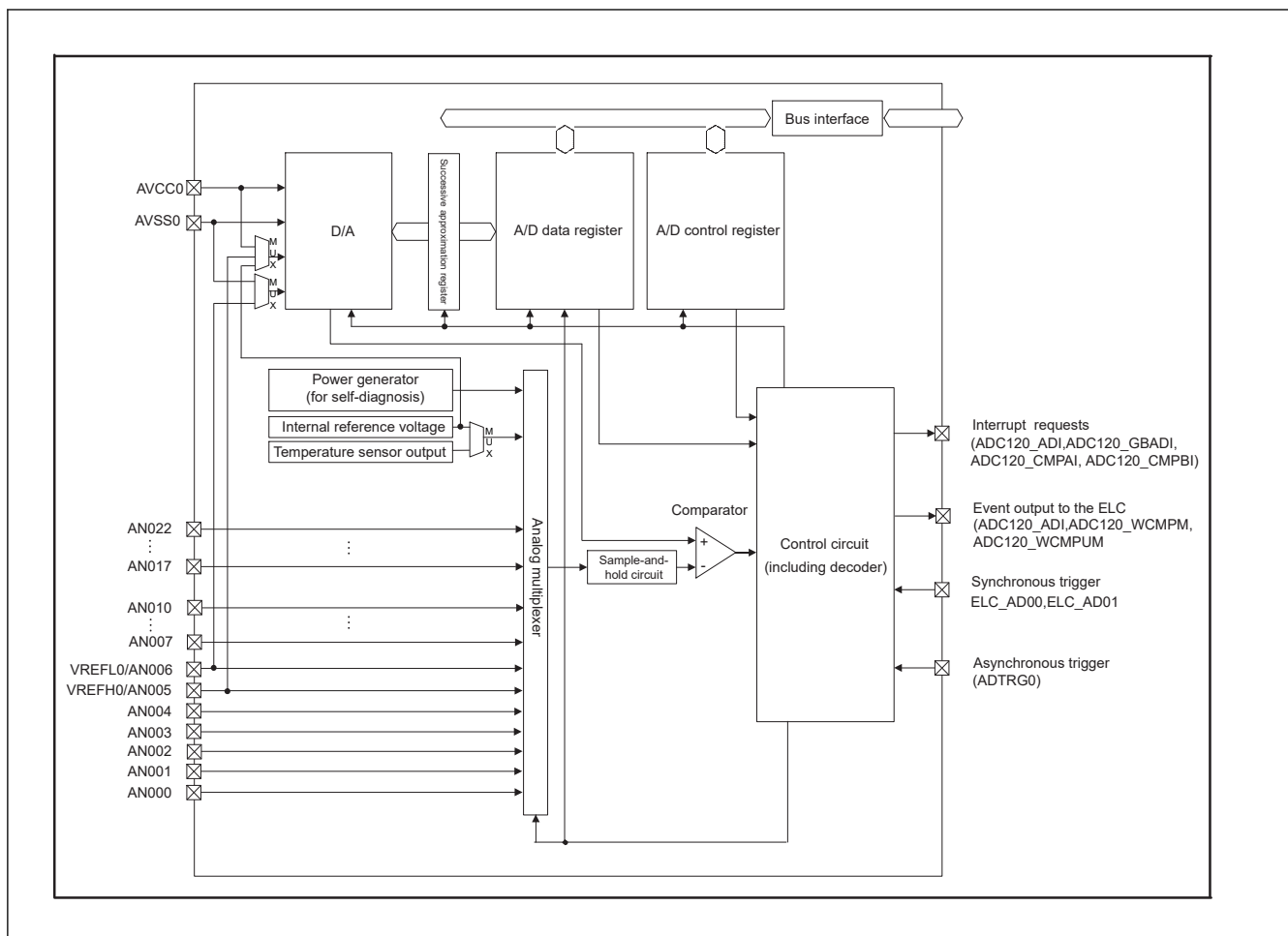
Figure 34.1 ADC12 block diagram
