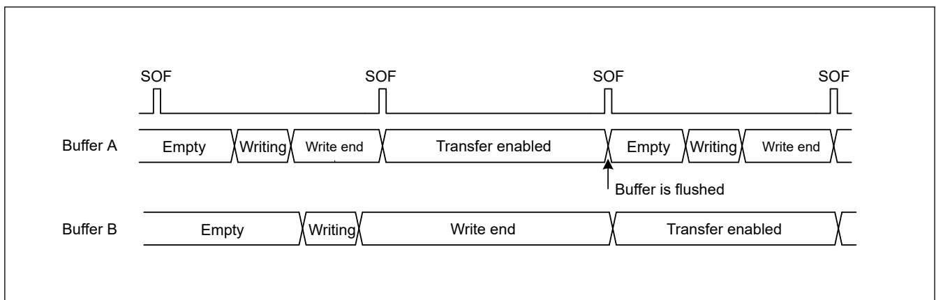
Figure 25.13 Example buffer flush operation
