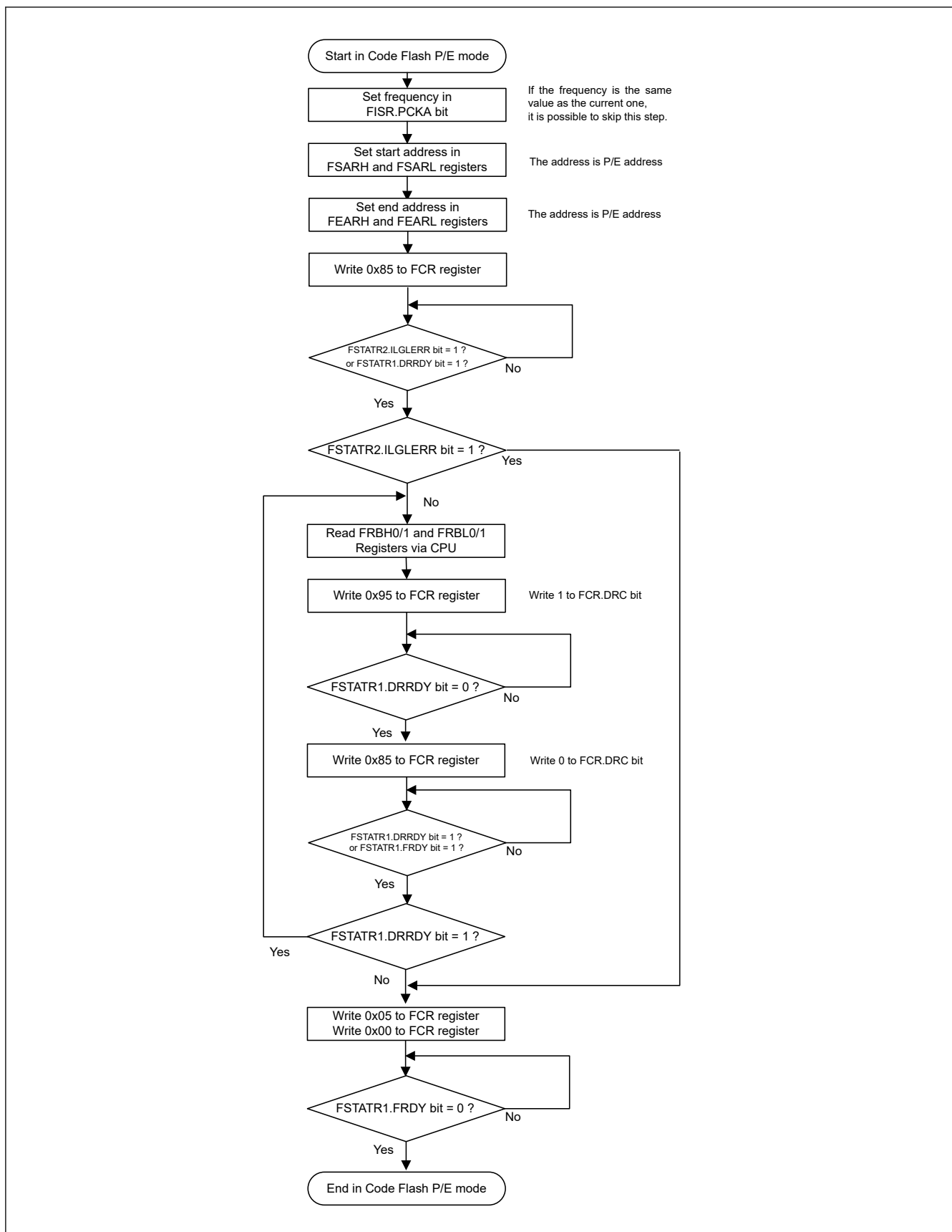
Figure 38.30 Simple flowchart for the consecutive read procedure
