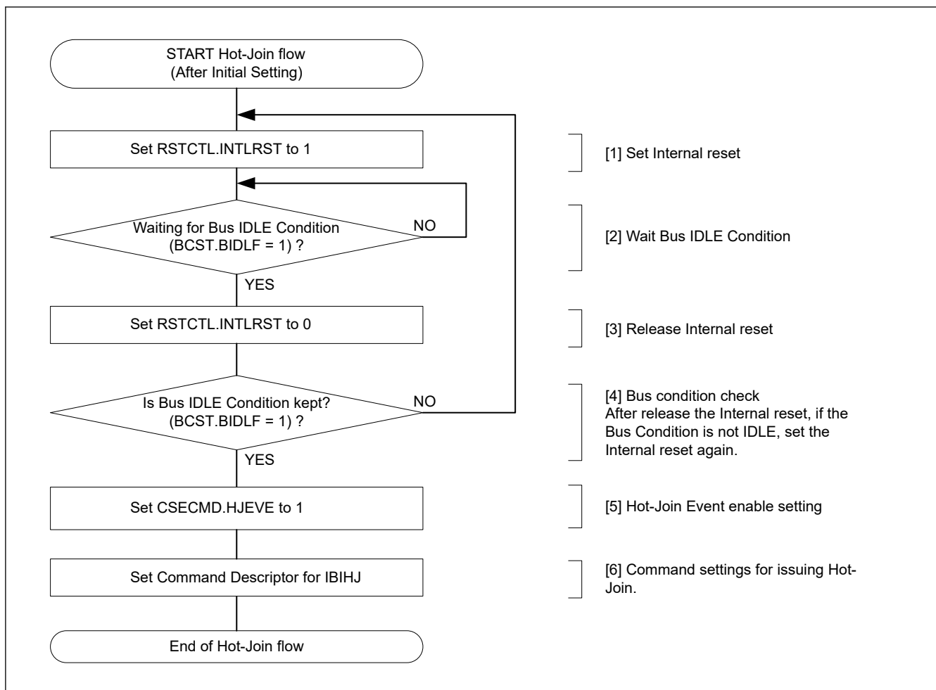
Figure 28.115 Hot-Join Flowchart after the I3C Bus has already been configured
