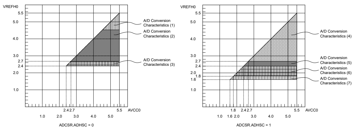
Figure 41.53 AVCC0 to VREFH0 voltage range
