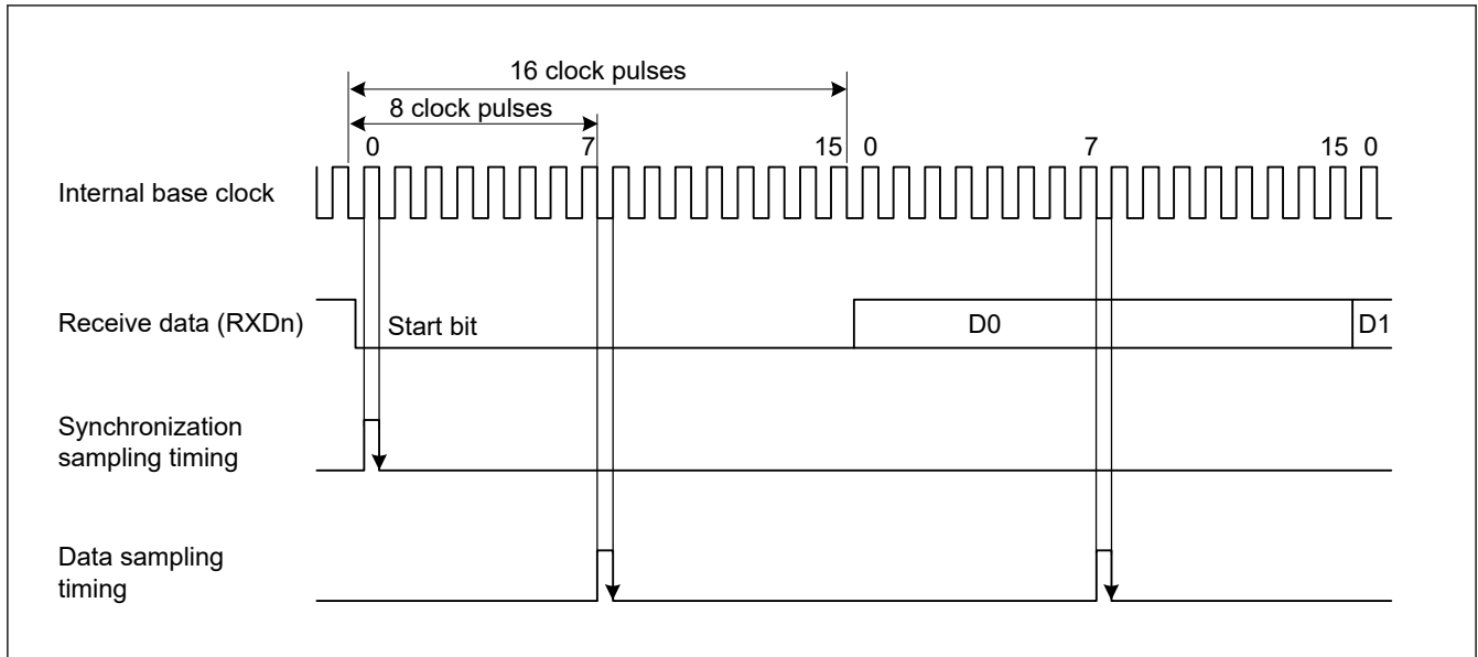
Figure 27.3 Receive data sampling timing in asynchronous mode
