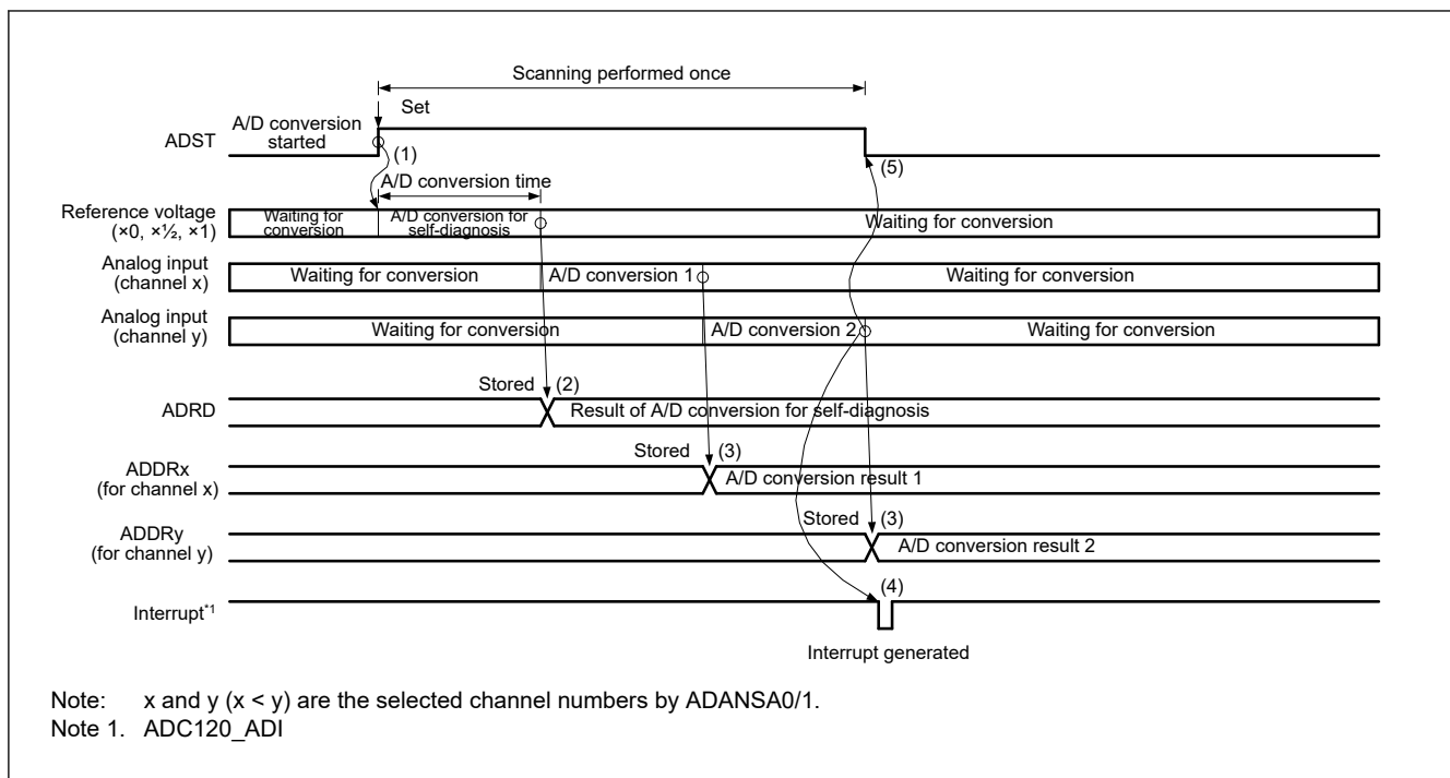
Figure 34.8 Example basic operation in single scan mode when the analog inputs (channel x and y) are selected with self- diagnosis
