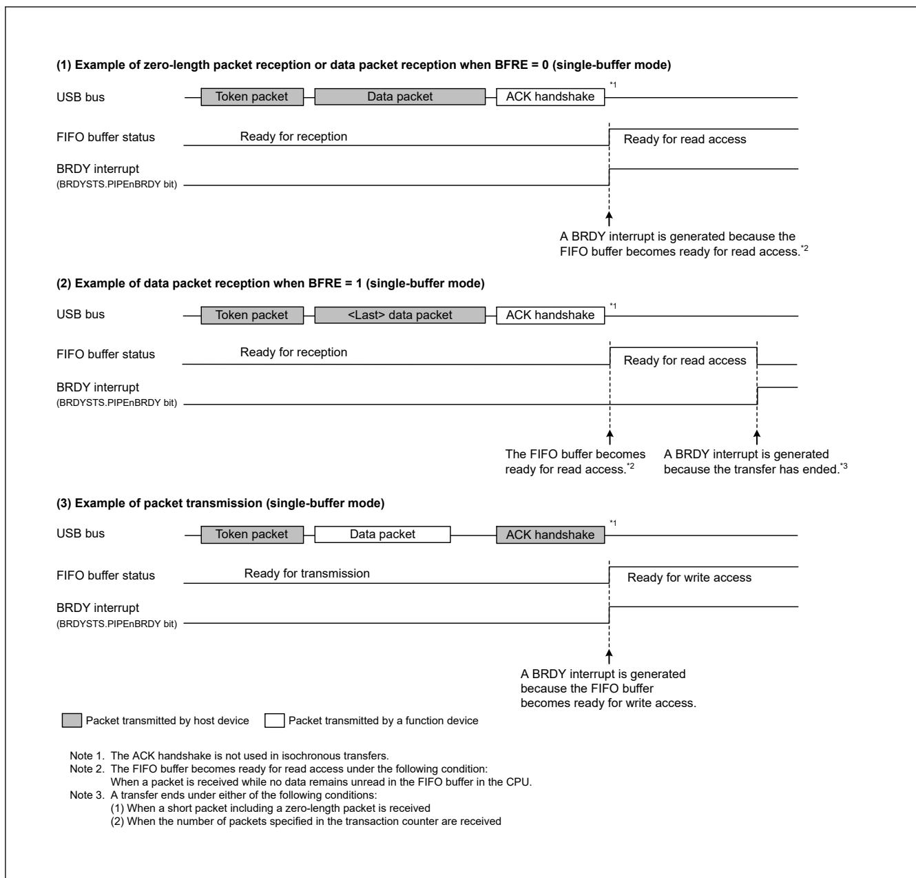
Figure 25.5 Timing of BRDY interrupt generation
