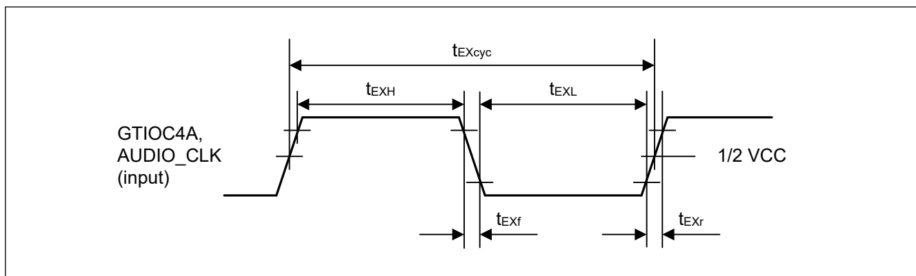
Figure 41.46 Clock input timing
