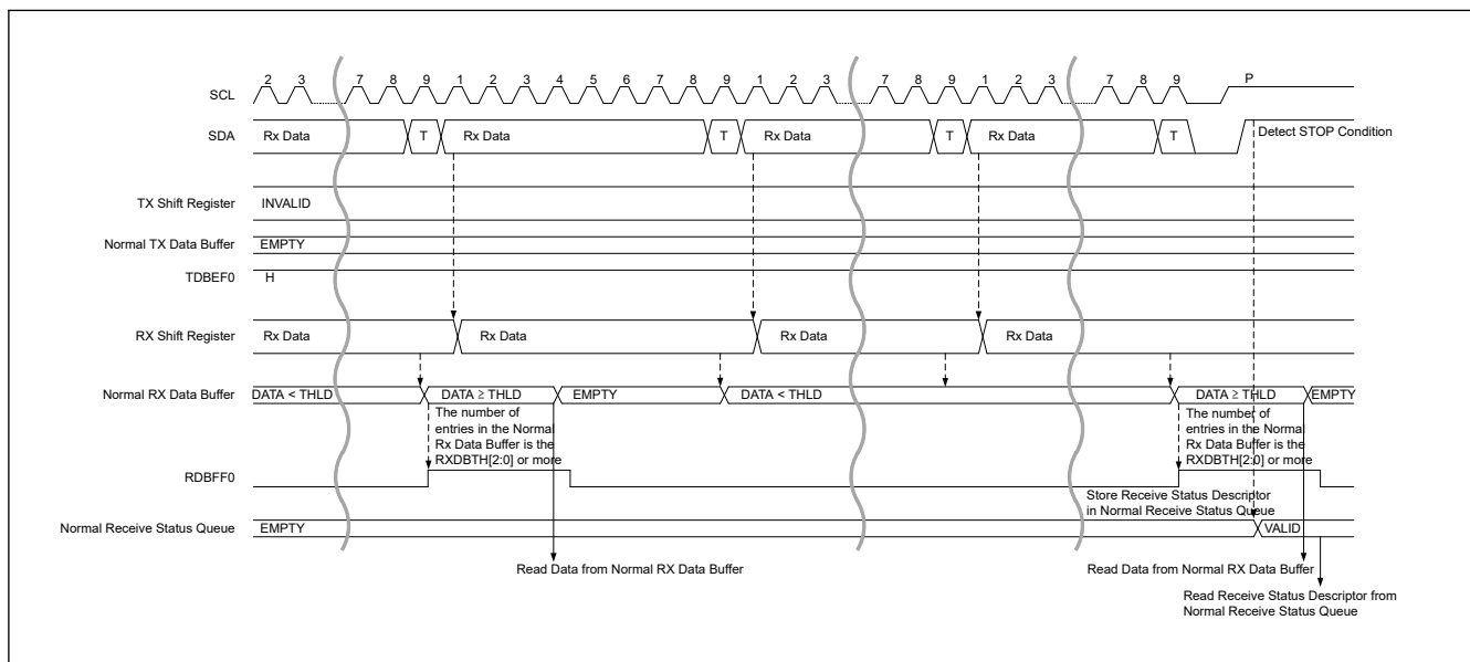
Figure 28.36 SDR data write transfer timing (2/2)
