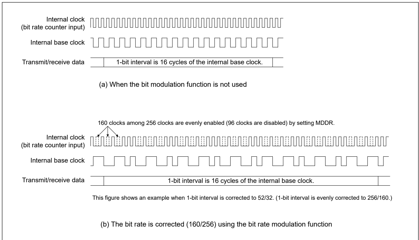
Figure 27.70 Example internal base clock when bit rate modulation function is used
