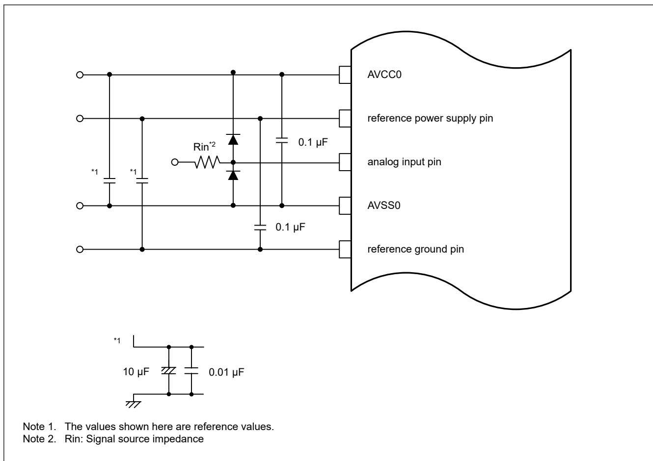
Figure 34.33 Example protection circuit for analog inputs
