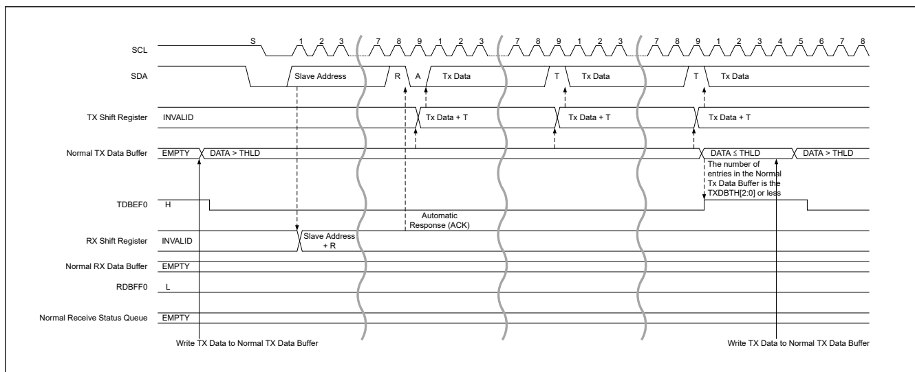
Figure 28.39 SDR data read transfer timing (1/2)
