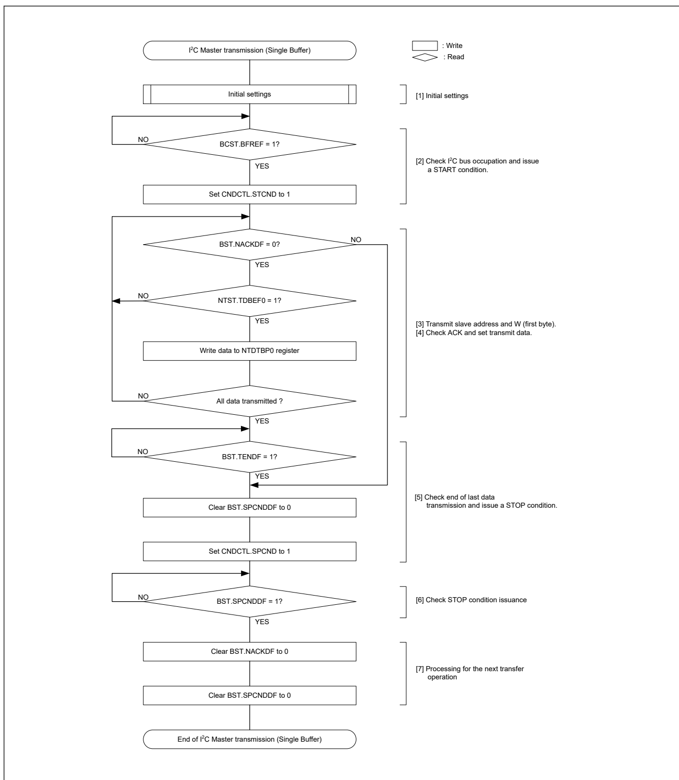
Figure 28.103 Example of I 2 C master transmission flowchart (single buffer transfer)
