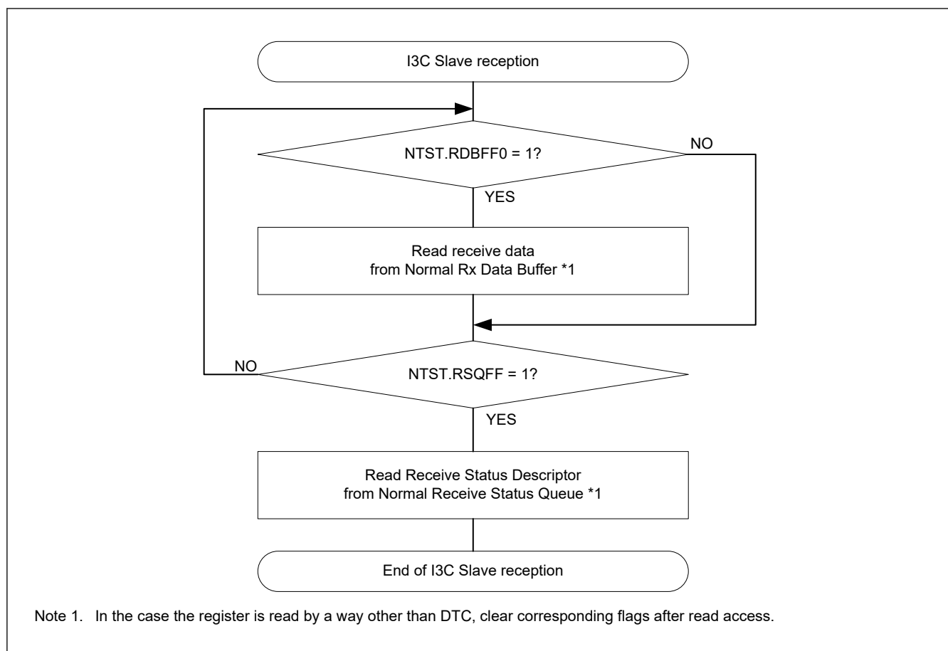
Figure 28.113 Example of I3C slave reception flowchart (normal FIFO buffer transfer)
