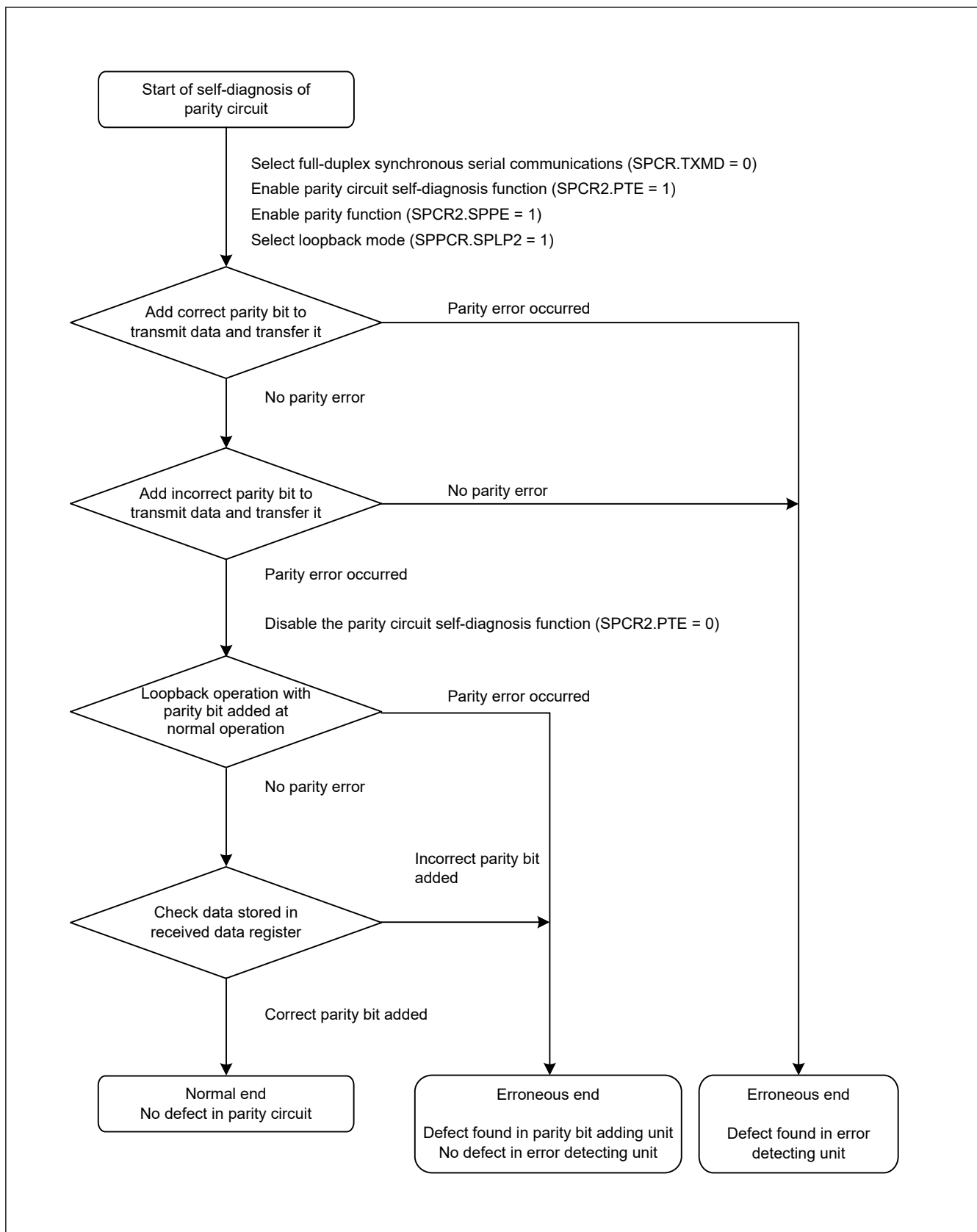
Figure 30.43 Self-diagnosis flow for parity circuit
