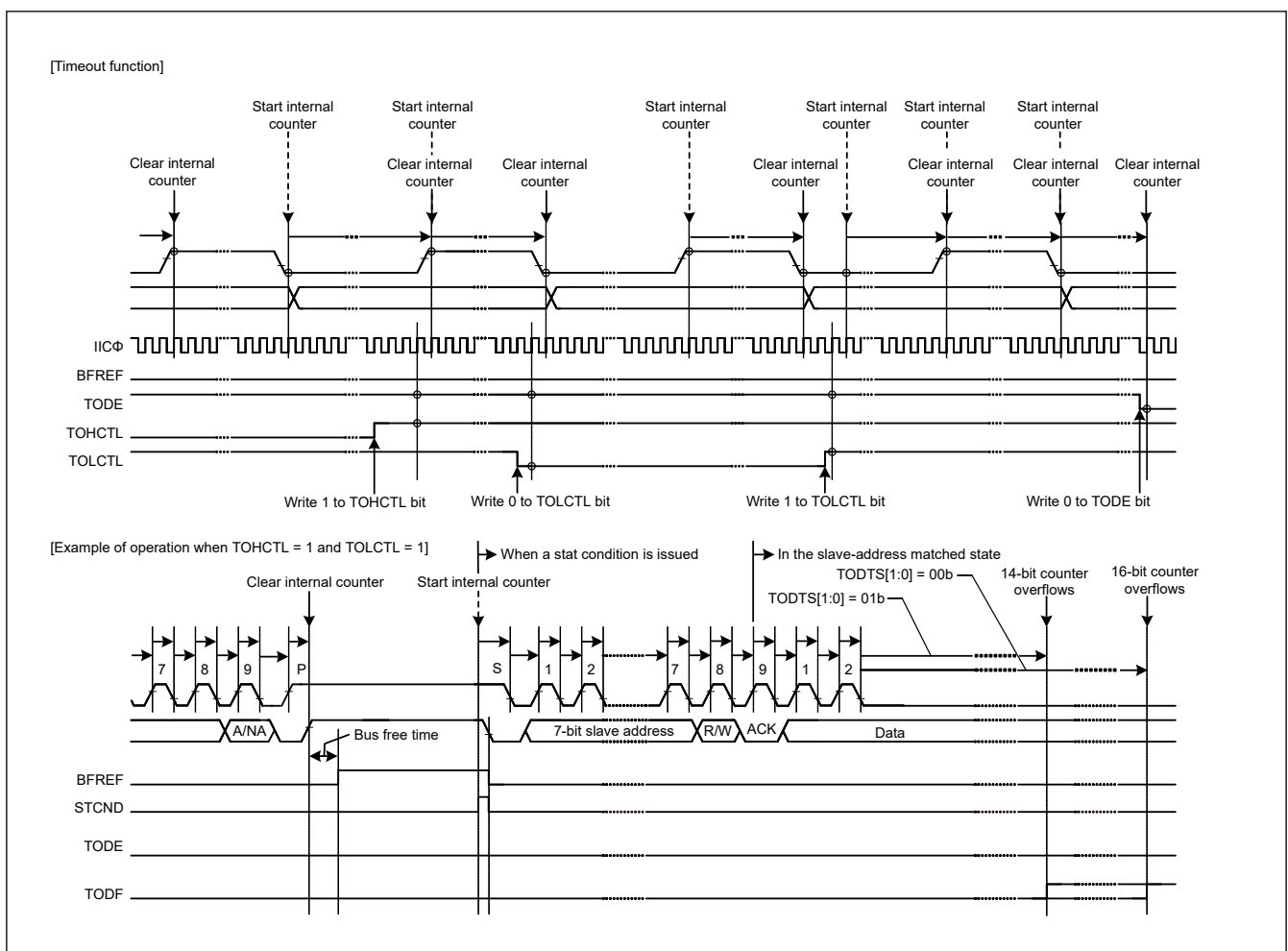
Figure 28.92 Timeout error detection (TODE, TODTS[1:0], TOHCTL, and TOLCTL bits)
