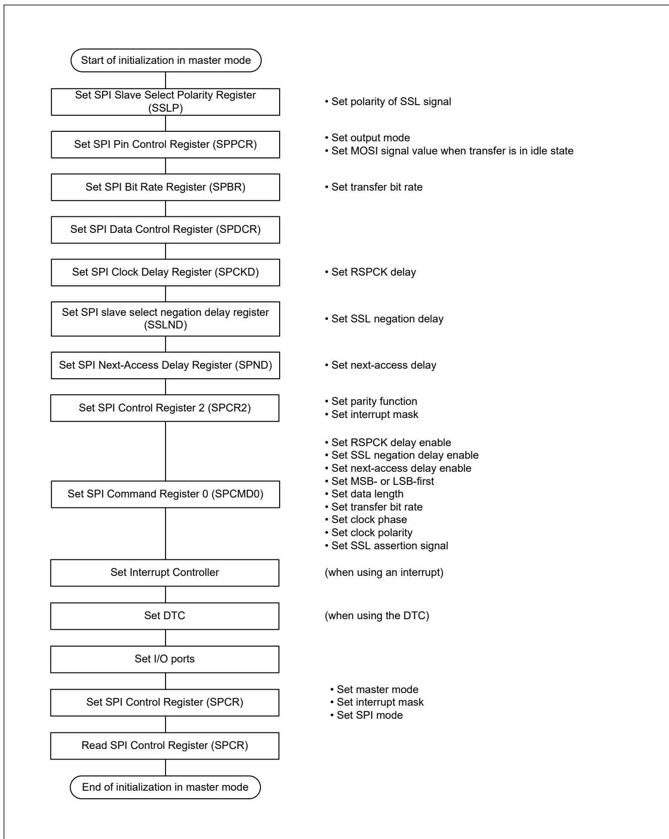
Figure 30.32 Example of initialization flow in master mode for SPI operation
