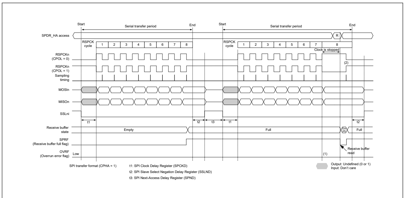
Figure 30.29 Clock stop waveform when serial transfer continues while receive buffer is full in master mode (CPHA = 1)
