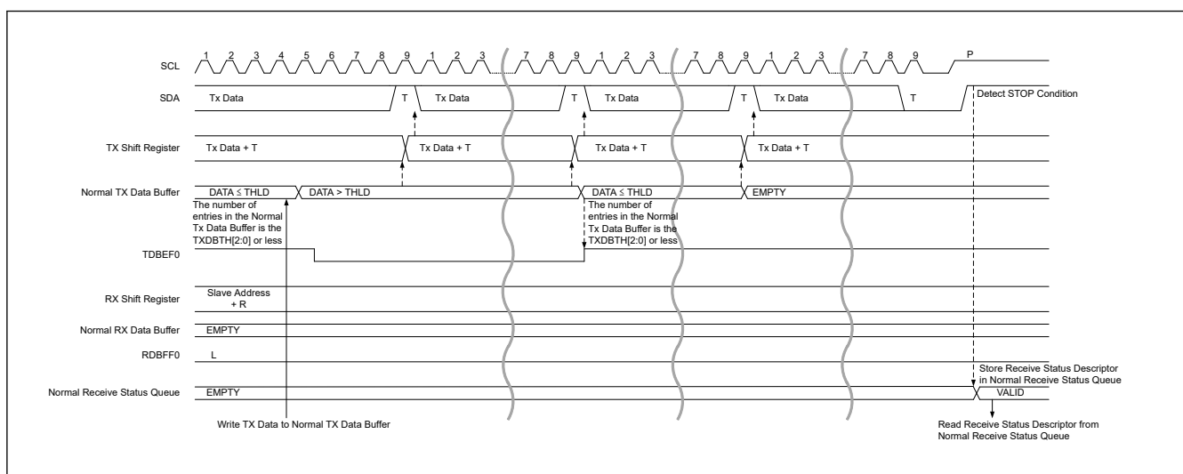
Figure 28.40 SDR data read transfer timing (2/2)
