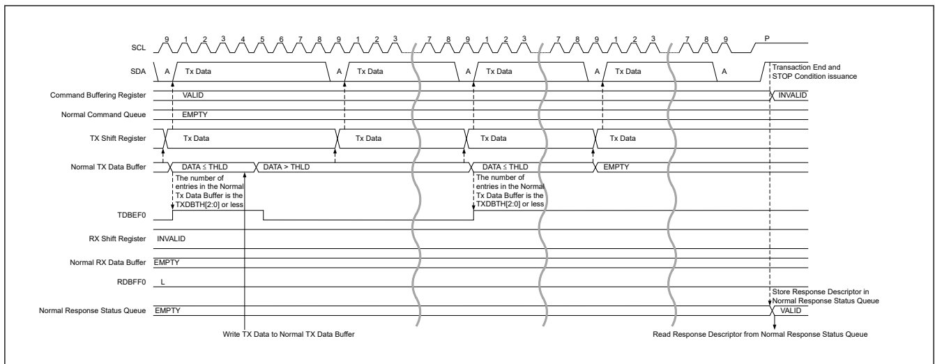
Figure 28.19 Legacy I 2 C message data write timing (2/2)
