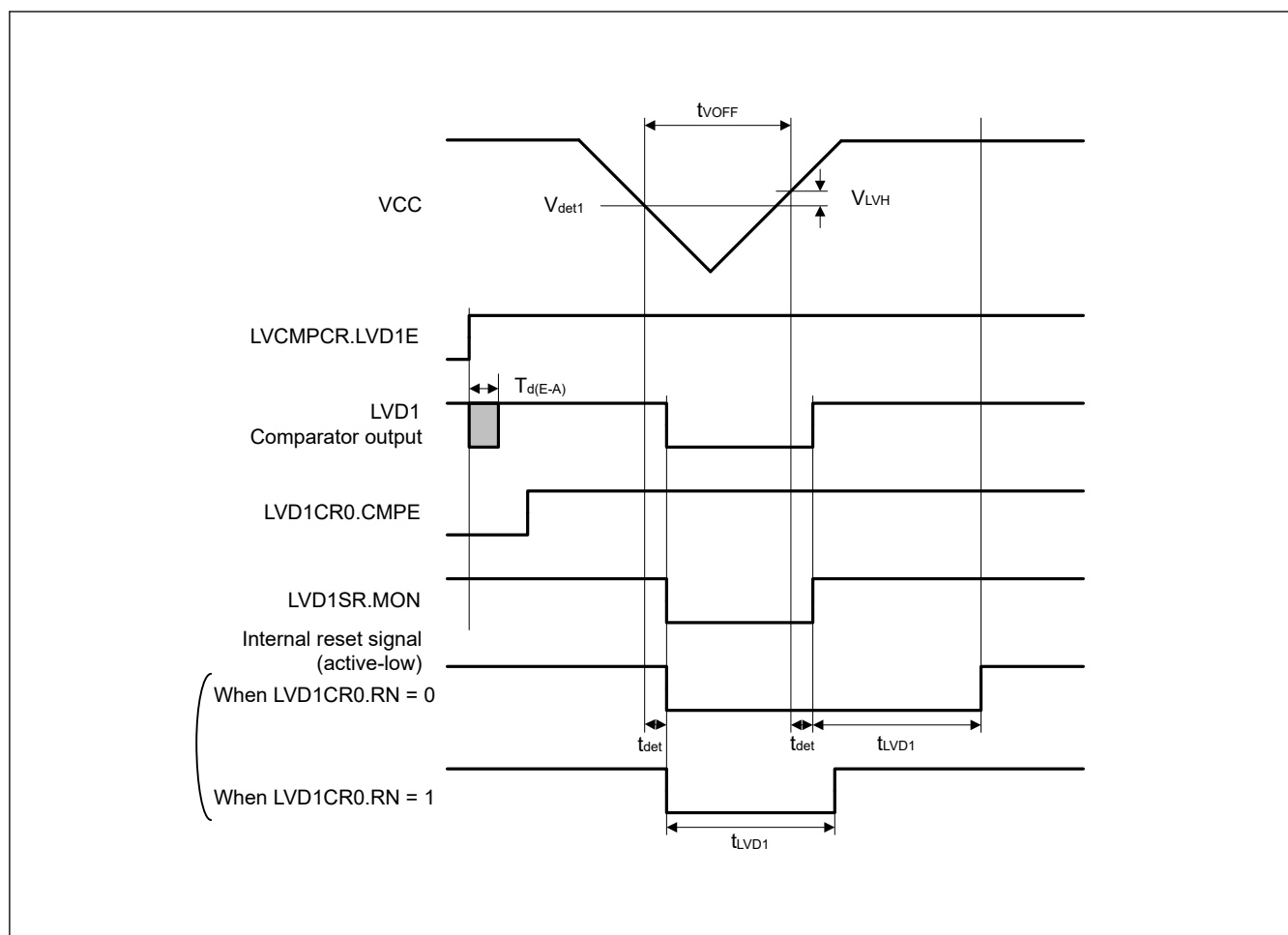
Figure 41.60 Voltage detection circuit timing ( V_{det1} )
