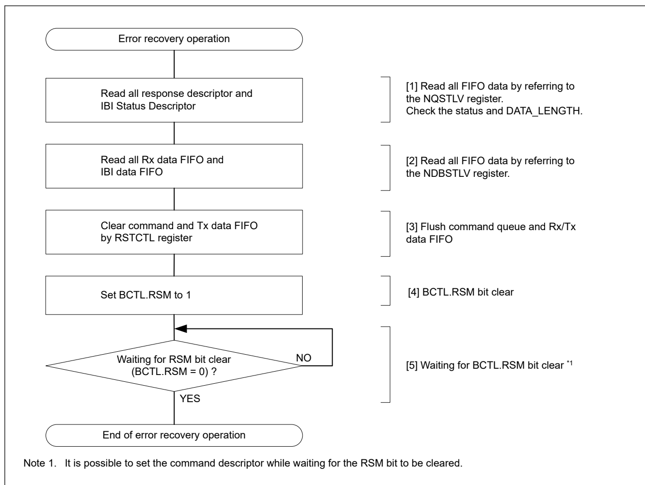
Figure 28.95 Example of error recovery operation flowchart for I3C master
