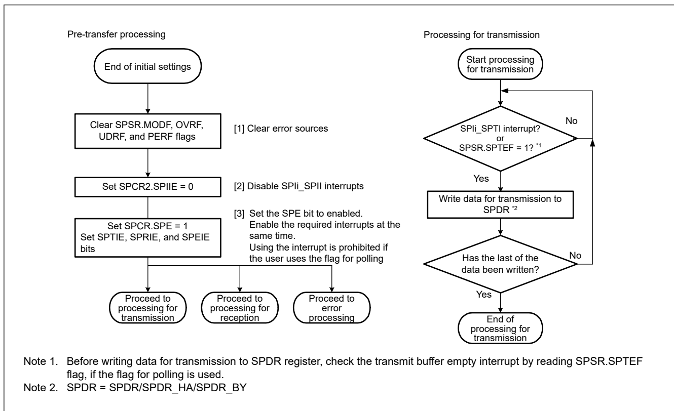
Figure 30.37 Transmission flow in slave mode
