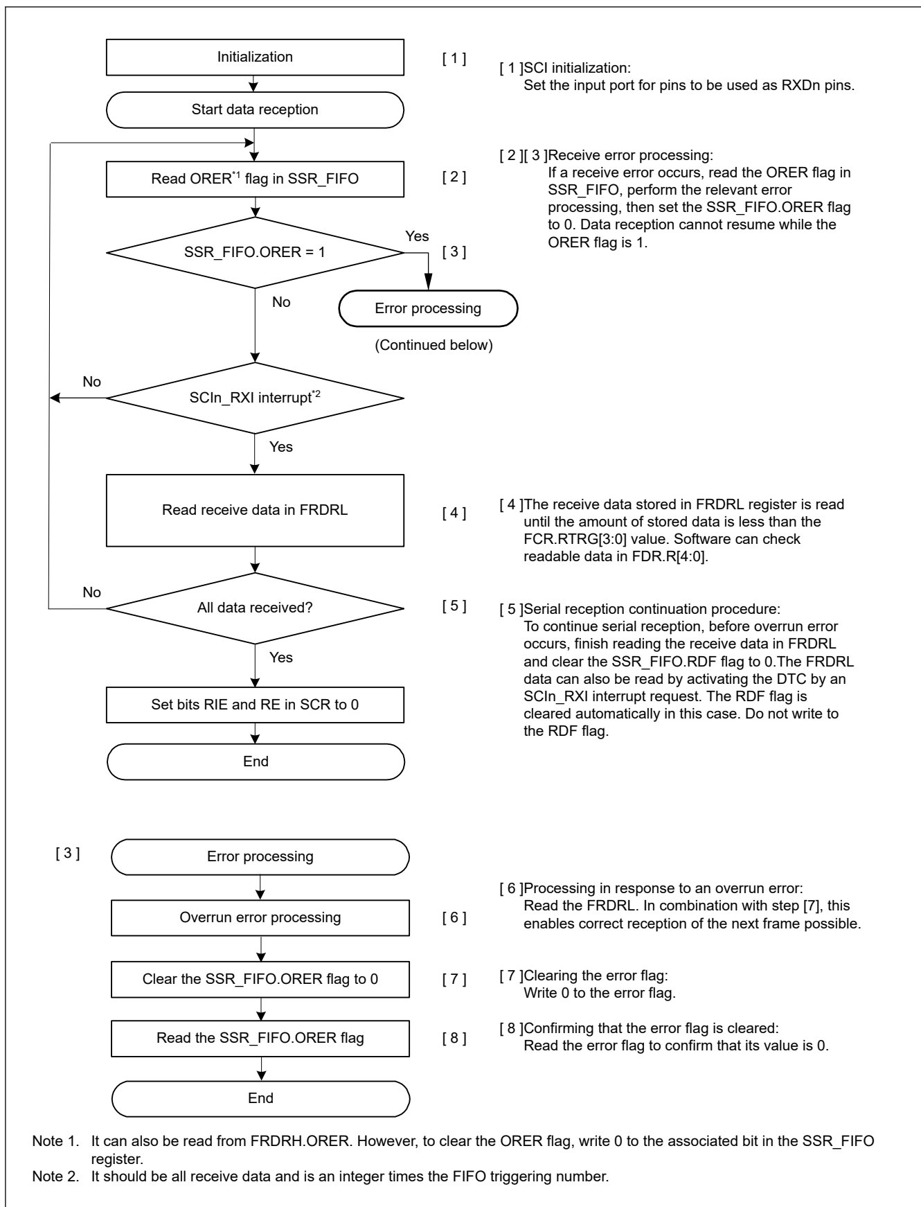
Figure 27.44 Example flow of serial reception in clock synchronous mode with FIFO selected
