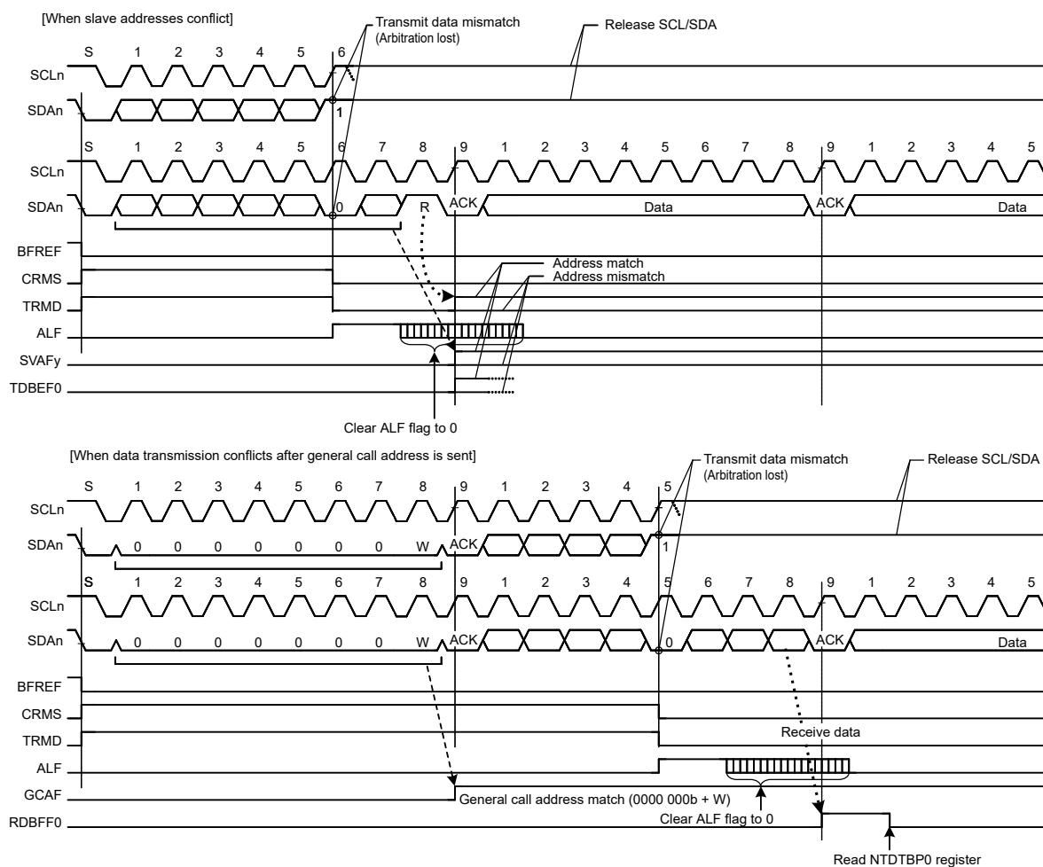
Figure 28.64 Examples of master arbitration-lost detection (MALE = 1)
