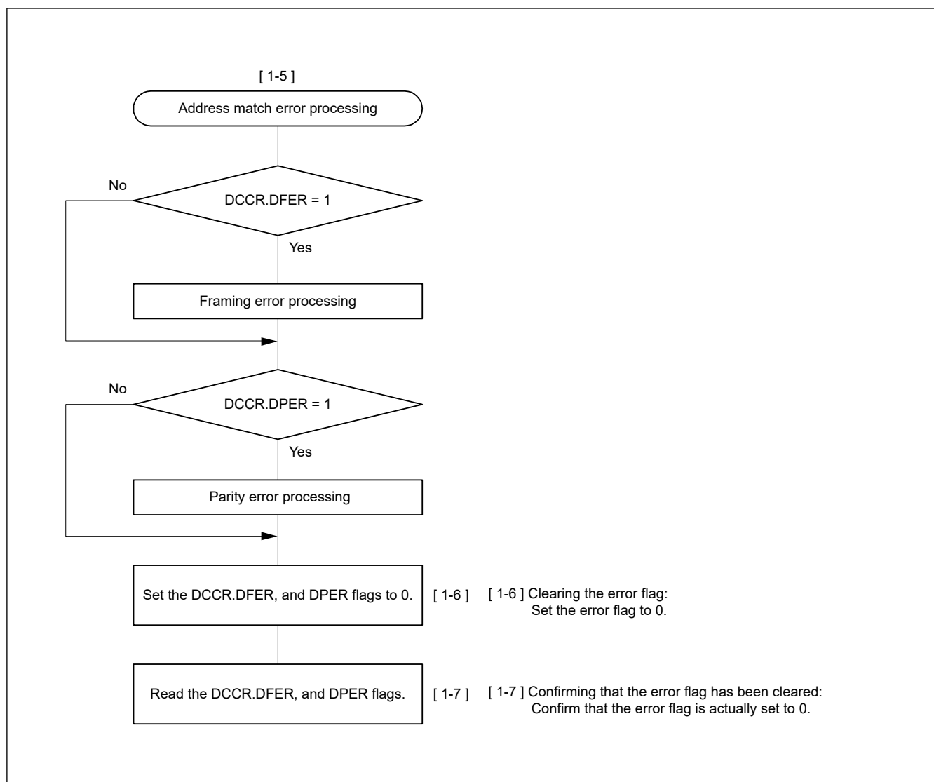
Figure 27.24 Example Flowchart of Serial Reception in Asynchronous Mode (FIFO Selected and Address Matching Enabled) (2)
