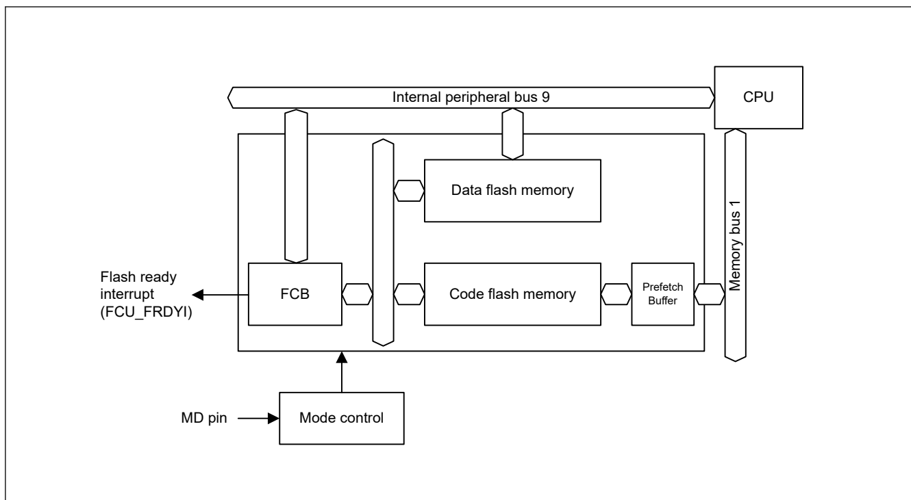
Figure 38.1 Flash memory-related modules block diagram
