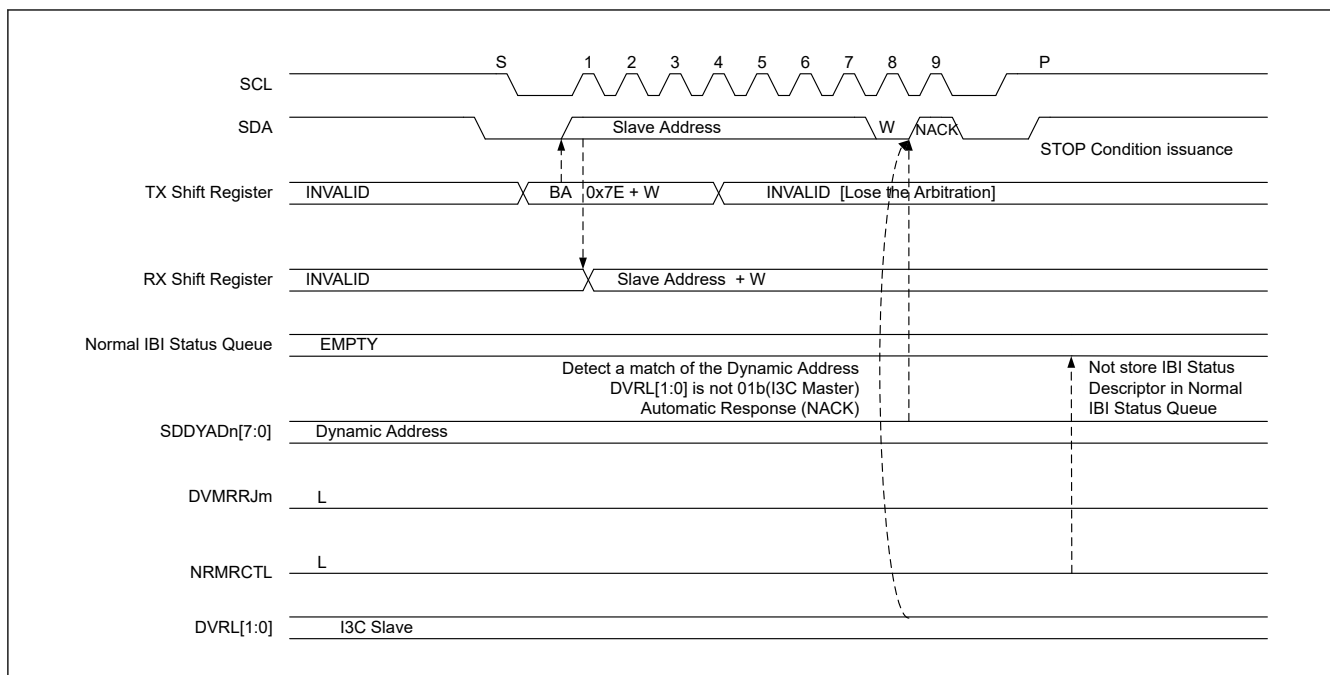
Figure 28.84 Mastership request : NACK (Device Role[1:0] is not 01 (I3C master)) and NRMRCTL = 0
