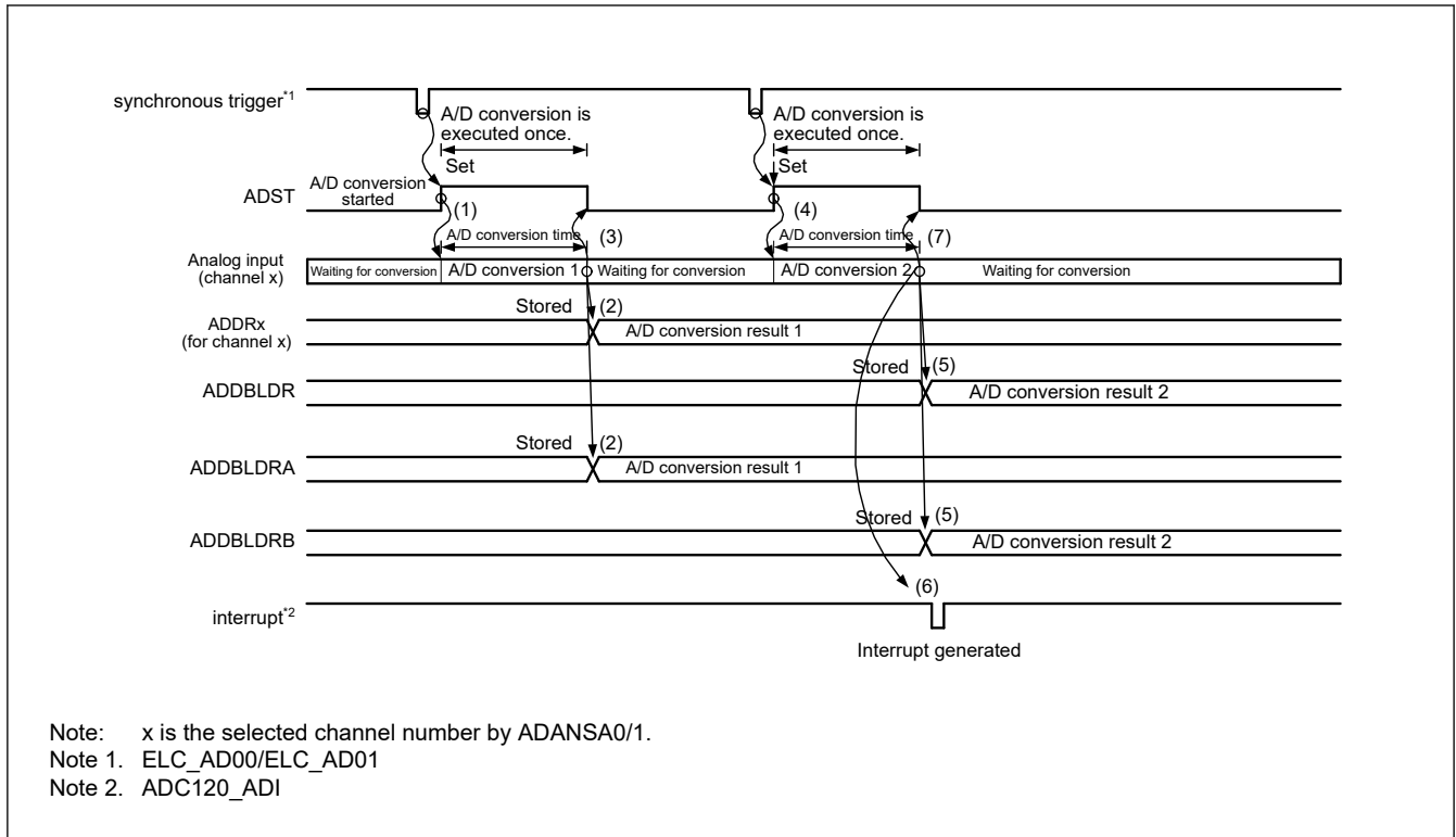
Figure 34.11 Example extended operation in double trigger mode with duplication selected for the analog input (channel x) and ELC_AD00/ELC_AD01
