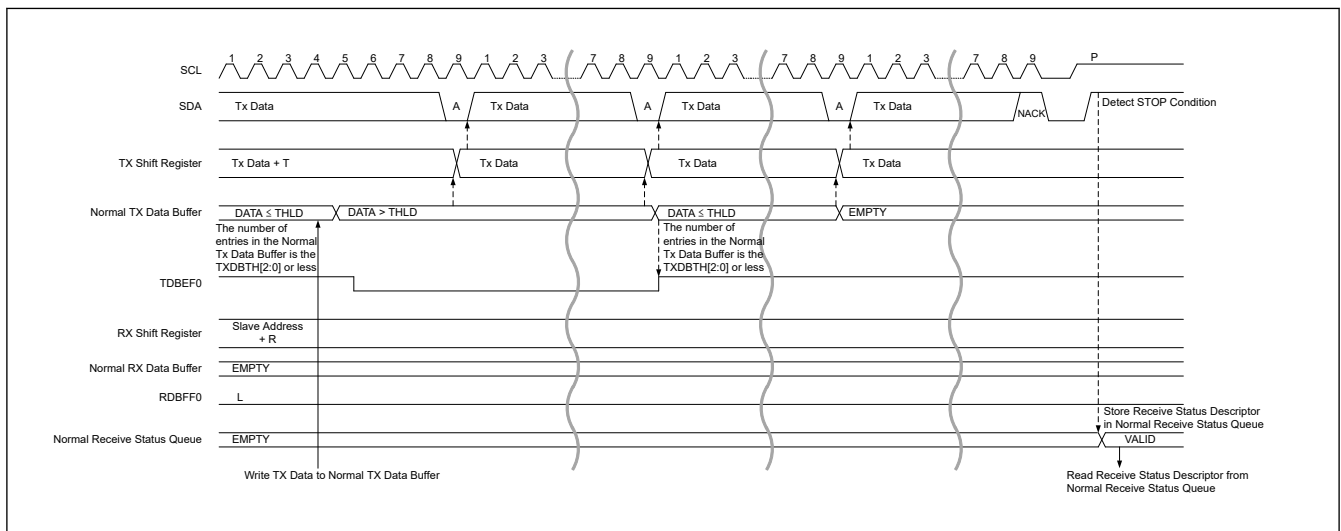
Figure 28.42 Legacy I 2 C message data read transfer timing (2/2)
