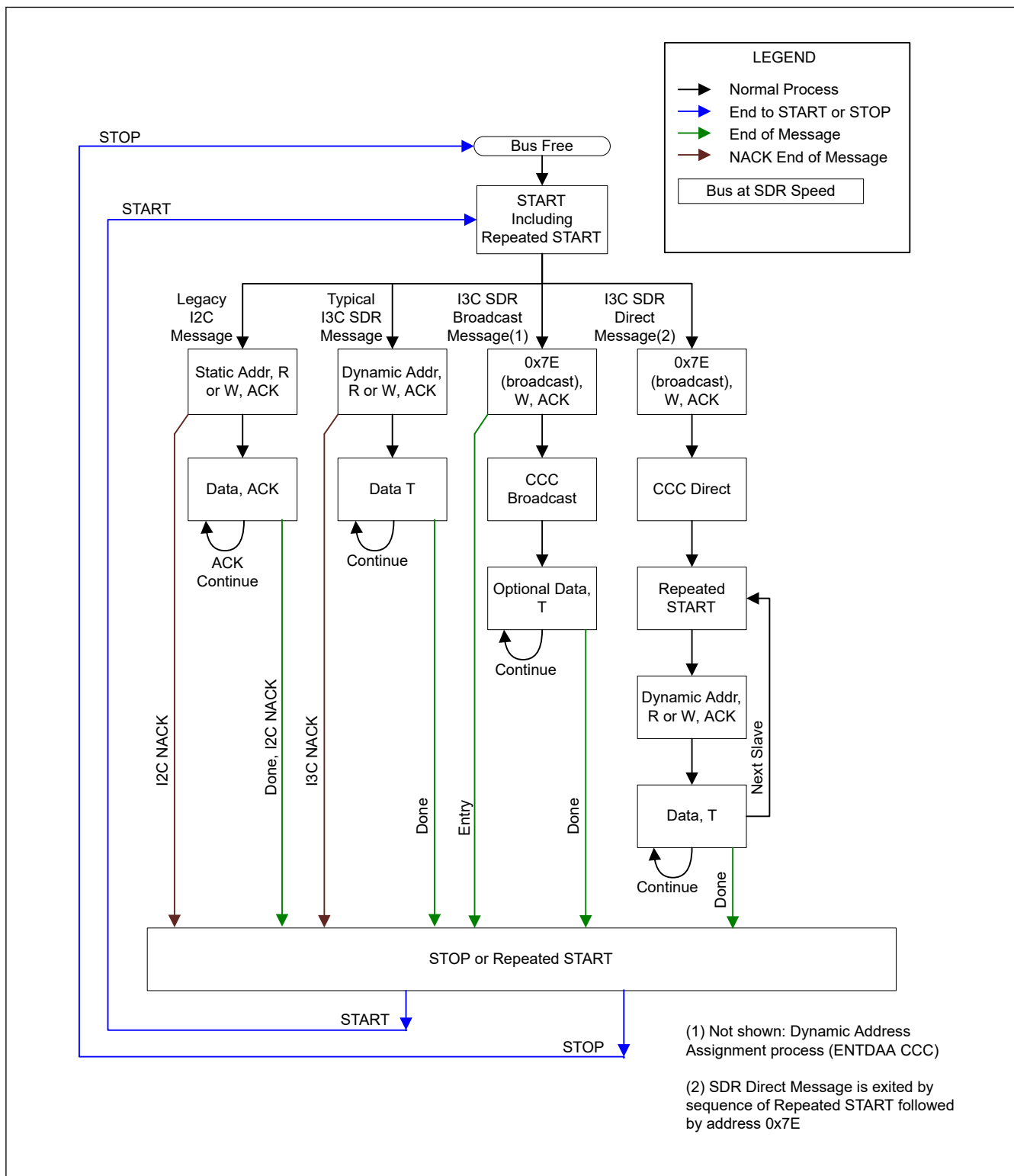
Figure 28.102 I3C communication flow
