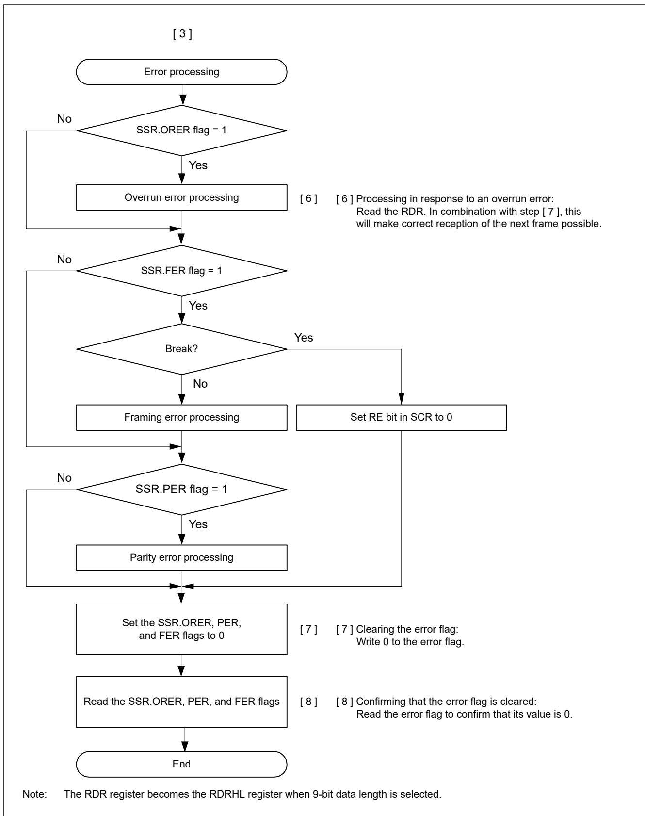
Figure 27.16 Example flow of serial reception in asynchronous mode with non-FIFO selected and Address Matching Disabled (2)
