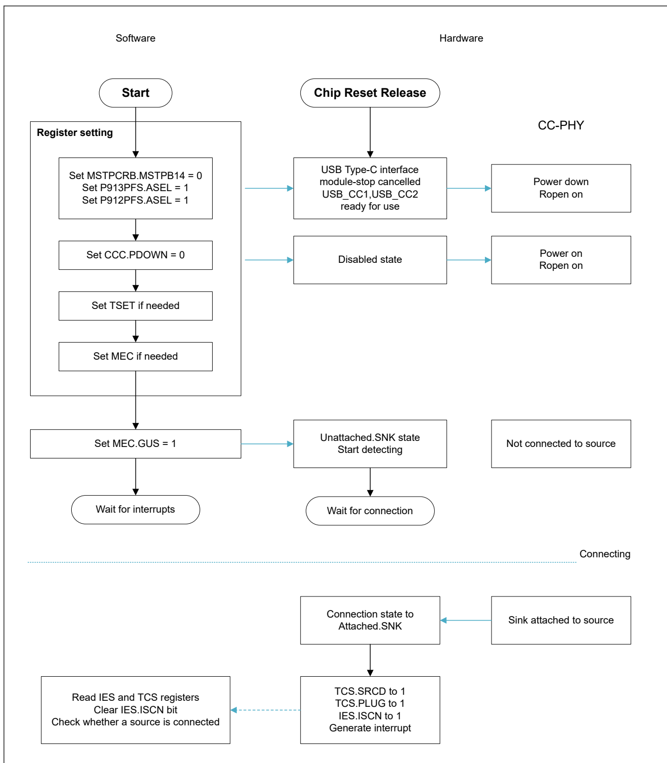
Figure 26.3 Sink-only mode initialization and connection detection flow
