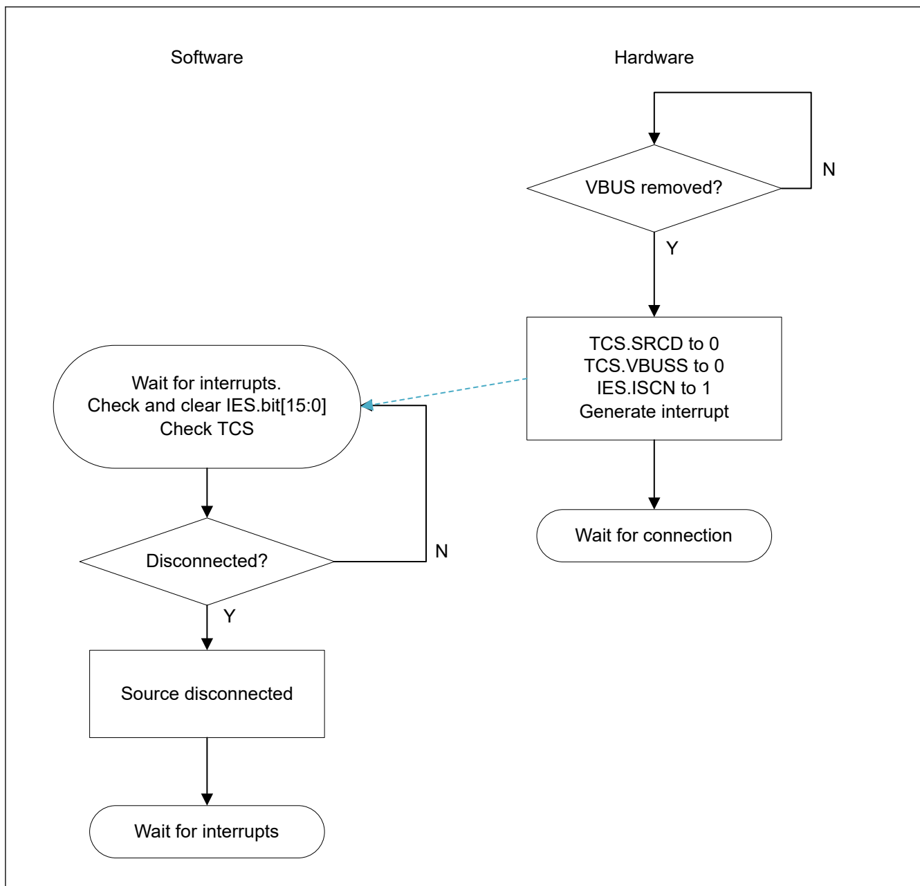
Figure 26.8 USB 2.0-only Sink mode disconnection detection flow
