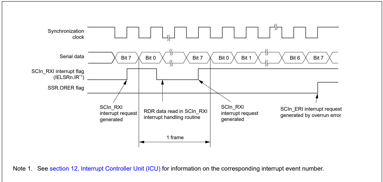
Figure 27.41 Example operation for serial reception in clock synchronous mode (1) when the RTS function is not used
