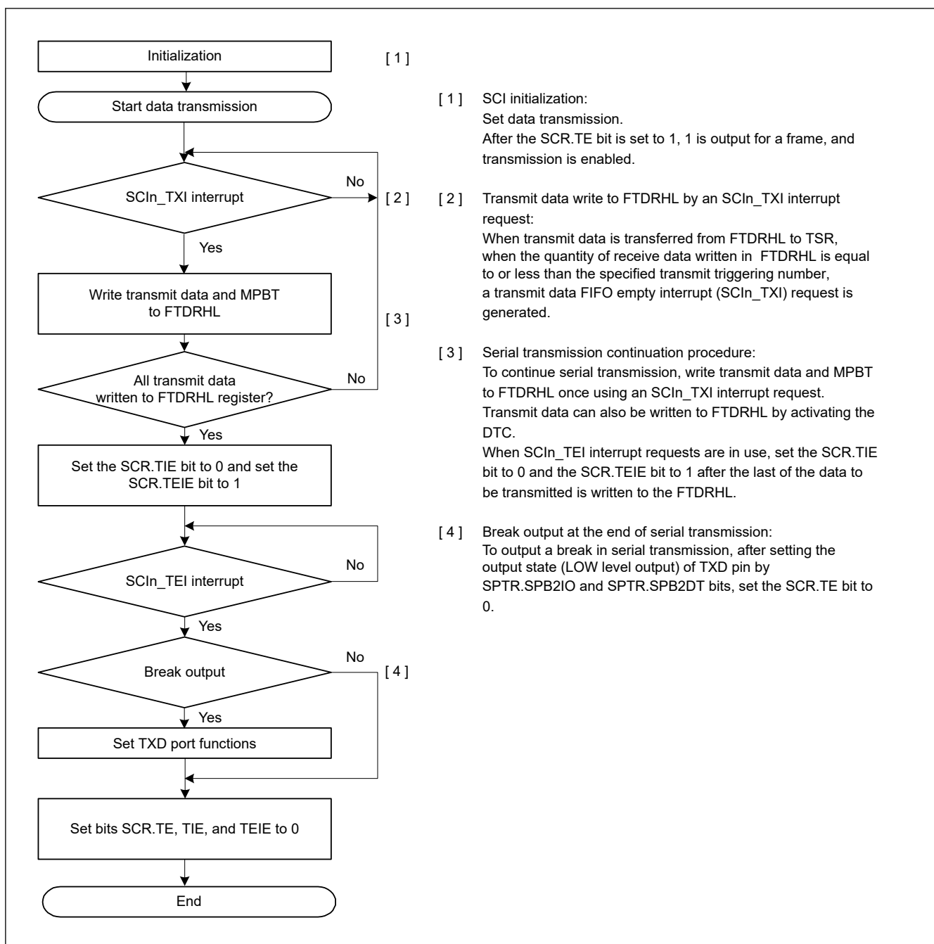
Figure 27.29 Example flow of serial transmission in multi-processor mode with FIFO selected
