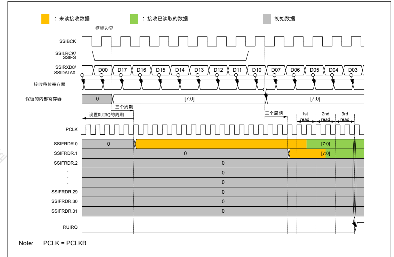
Figure 32.17 RUIRQ设置时序
