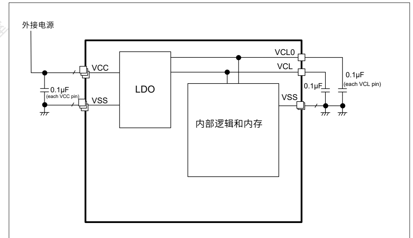
Figure 45.1 LDO模式设置
