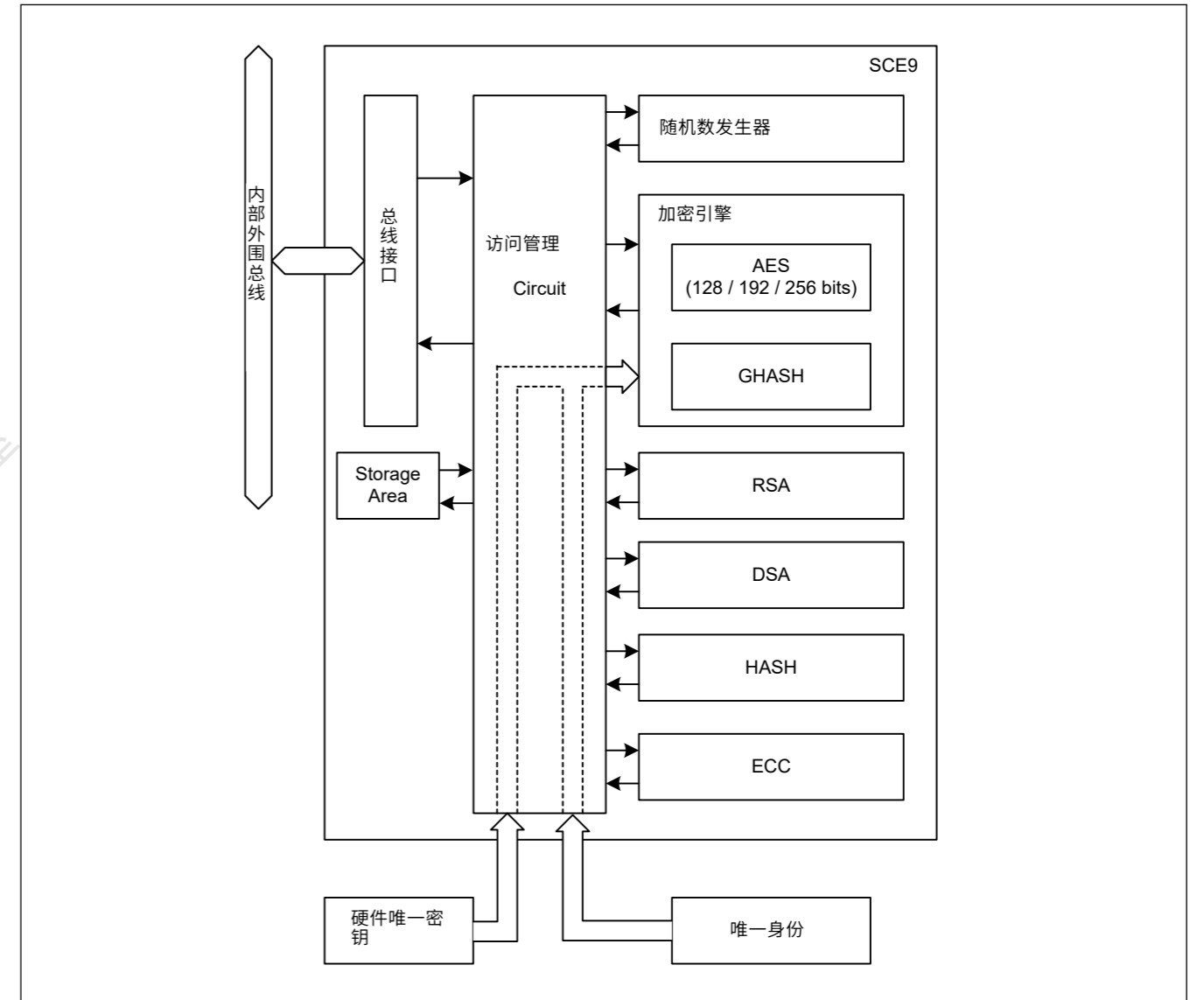
Figure 36.1 SCE9框图
