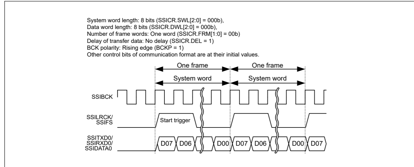
Figure 32.40 Long frame in mono format (without padding)
