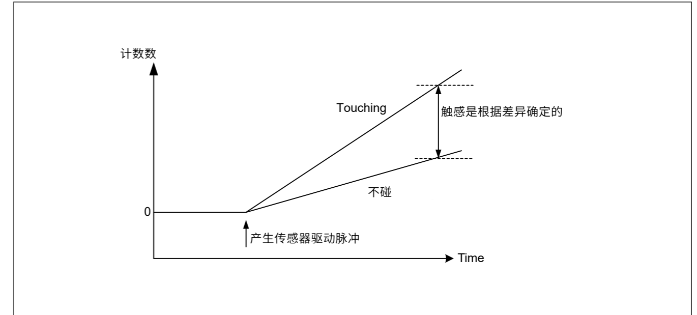
Figure 40.7 手指接触和不接触时测量值的变化
