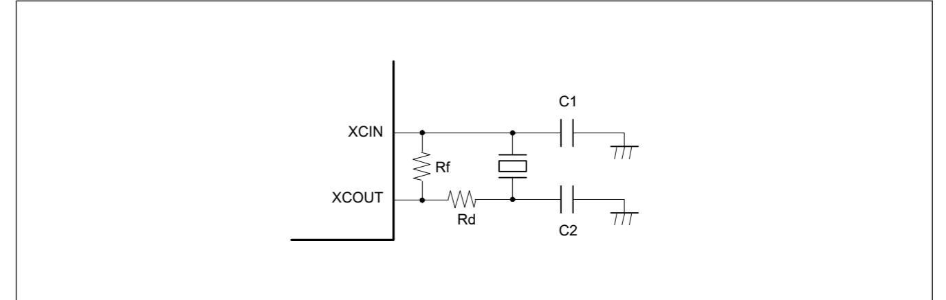
Figure 8.5 32.768-kHz晶体谐振器的连接示例
