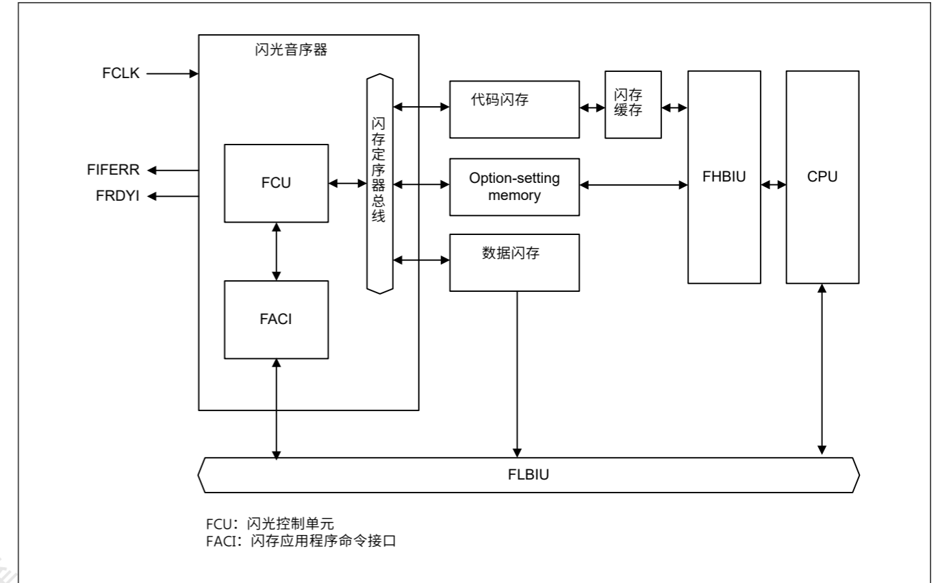
Figure 44.1 闪存相关模块框图
