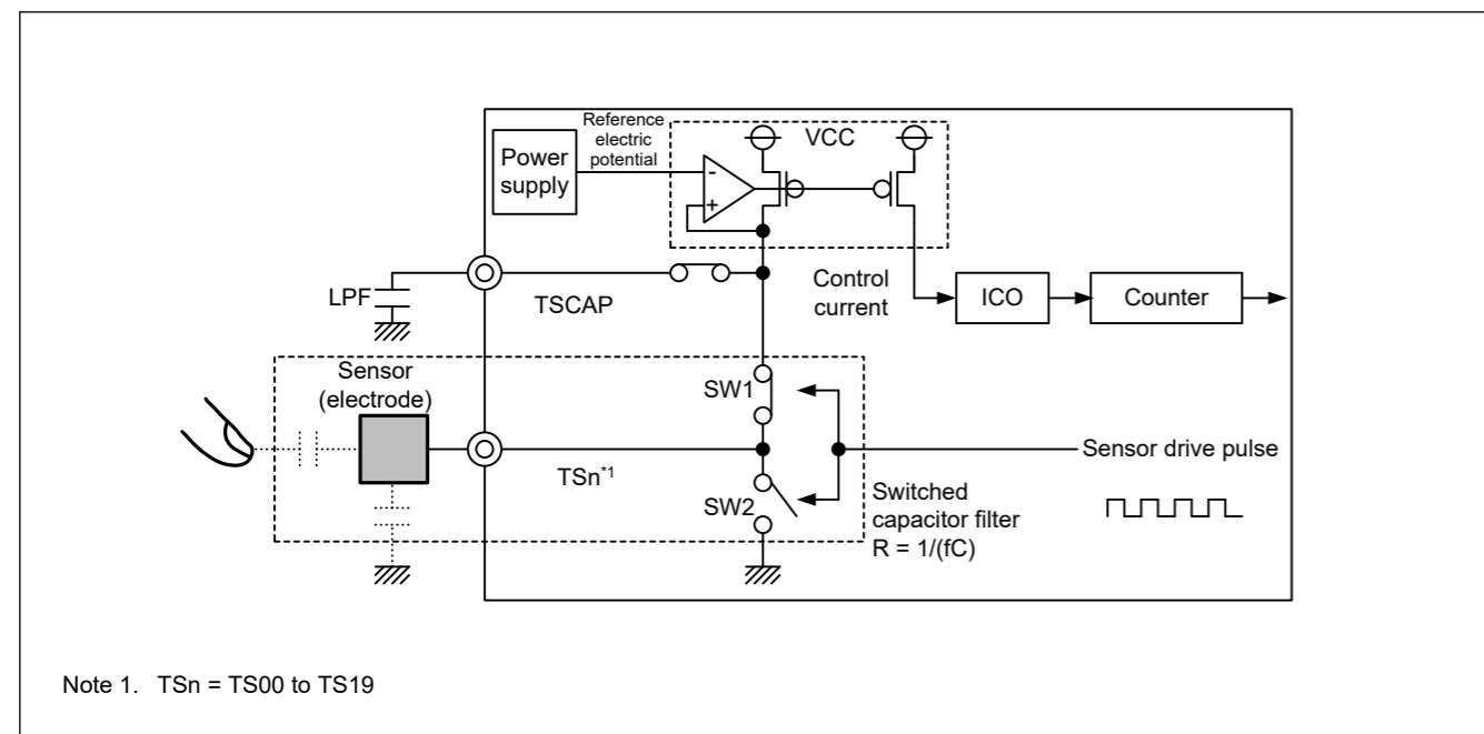
Figure 40.4 Measurement circuit
