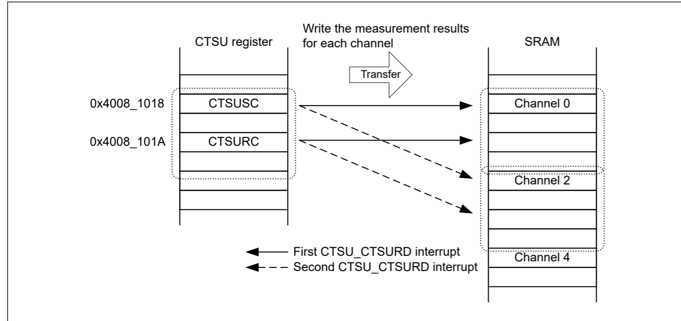
Figure 40.20 Example of DTC transfer operation using the CTSUS_CTSURD interrupt
