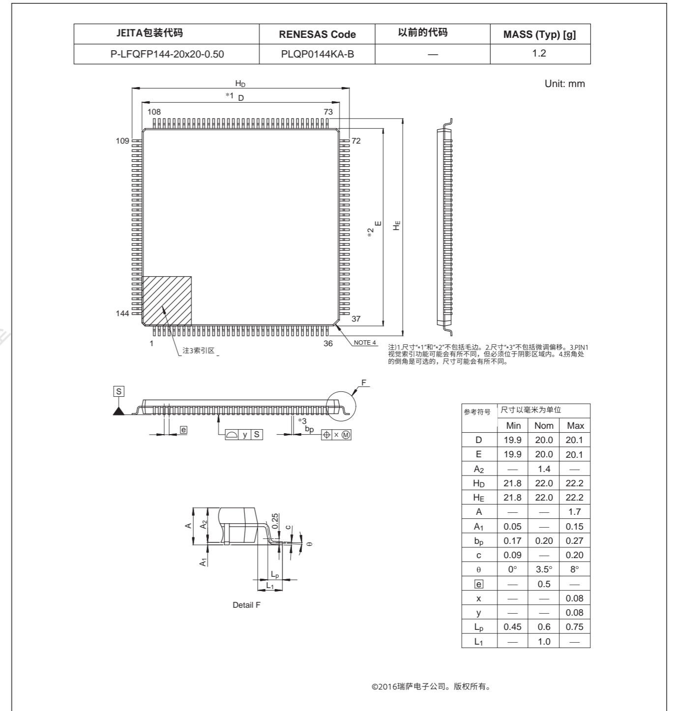
Figure 2.1 LQFP 144-pin
