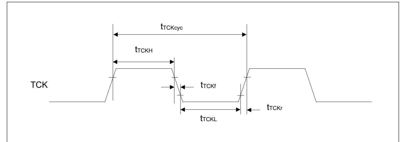
Figure 47.66 JTAG TCK timing
