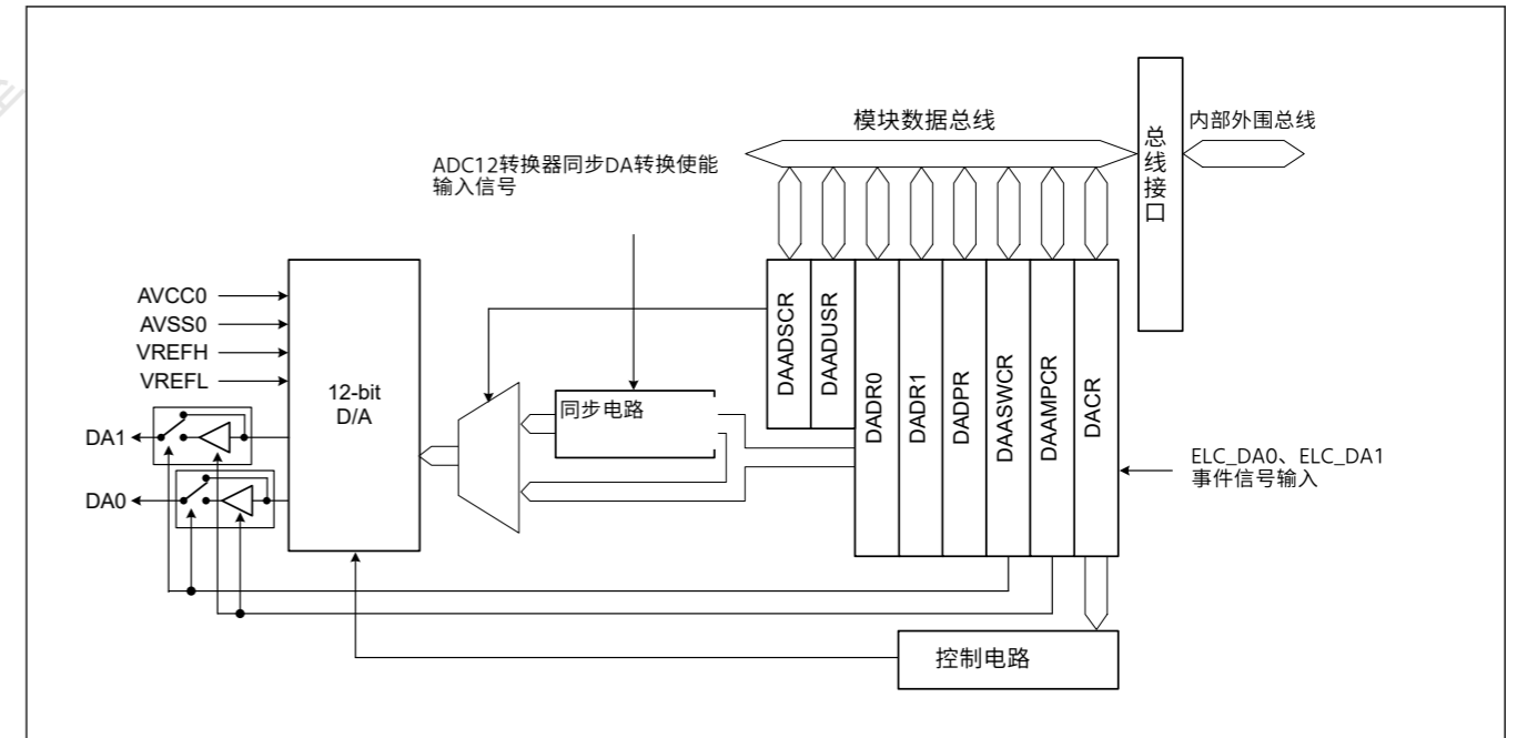
Figure 38.1 DAC12框图
