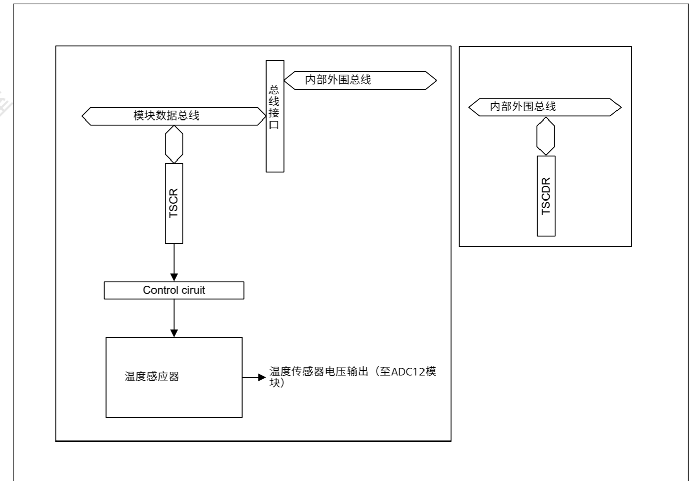
Figure 39.1 TSN框图
