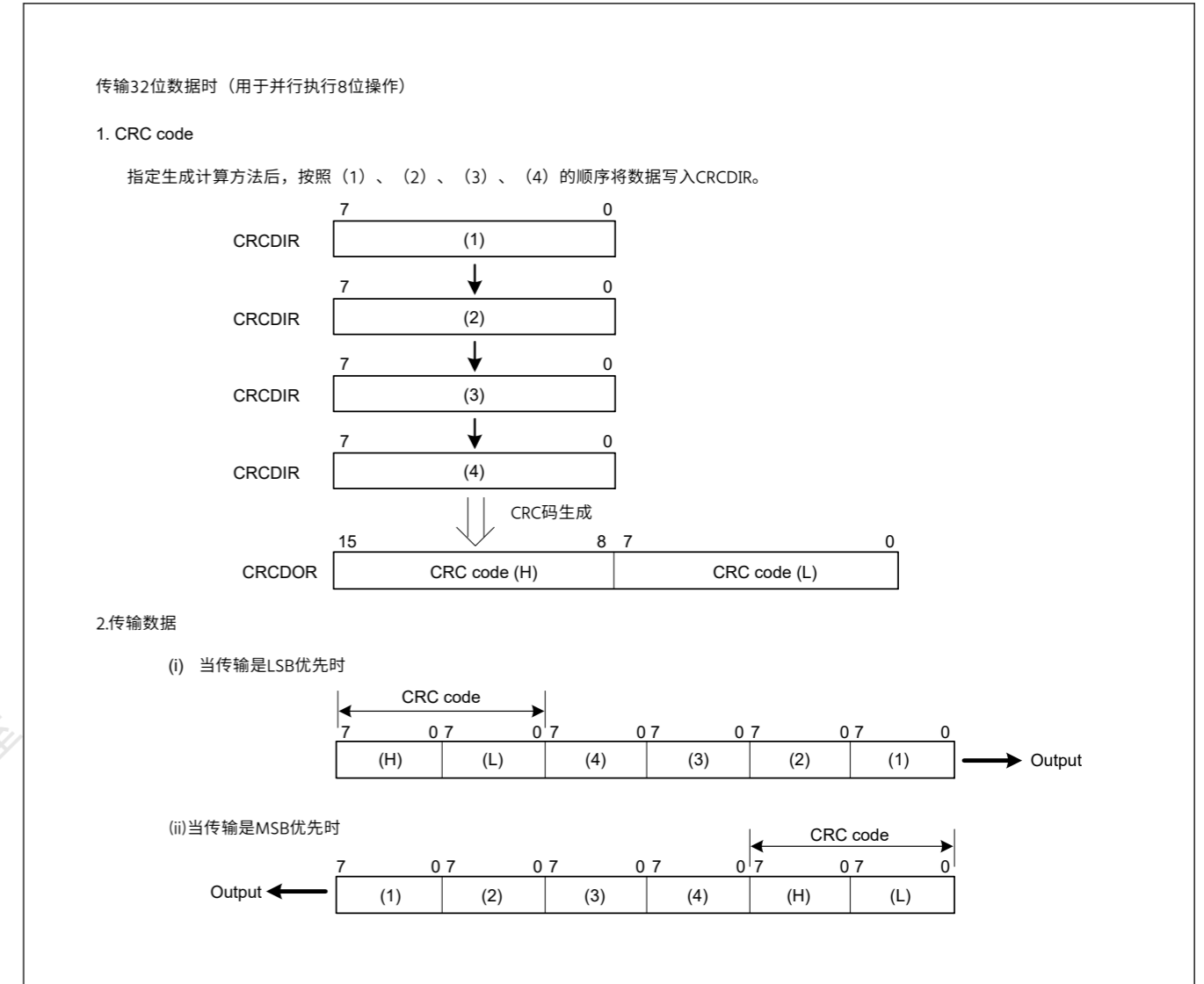
Figure 34.6 LSB-first和MSB-first数据传输
