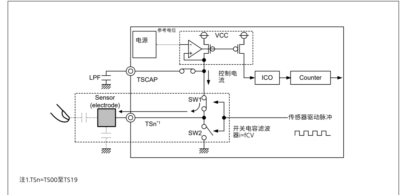
Figure 40.5 充电操作
