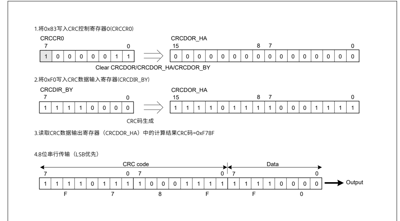
Figure 34.2 LSB-first数据传输
