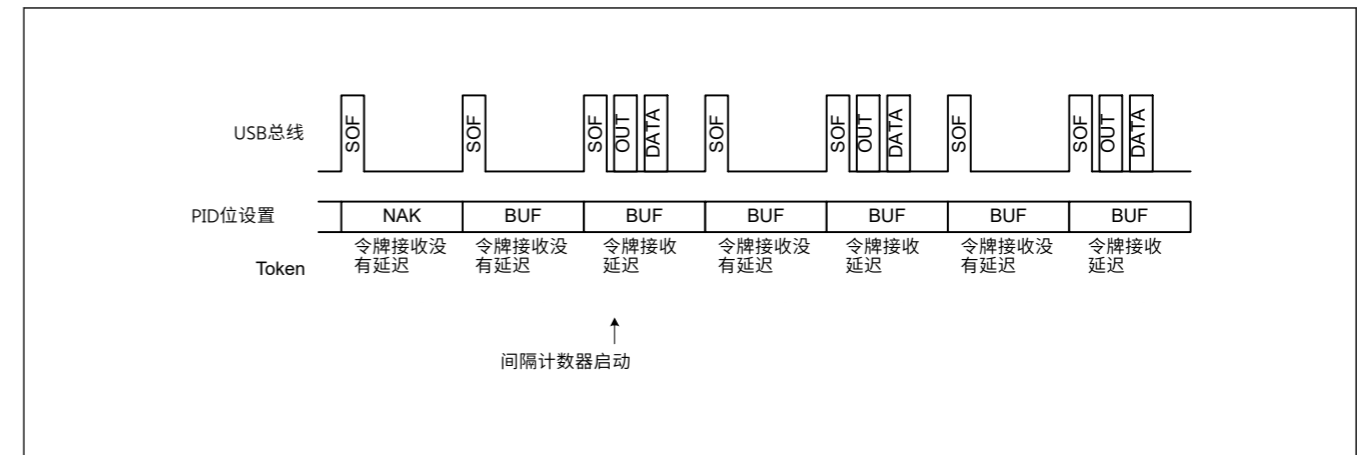
Figure 26.20 IITV[2:0]≠0时帧与预期令牌接收的关系
