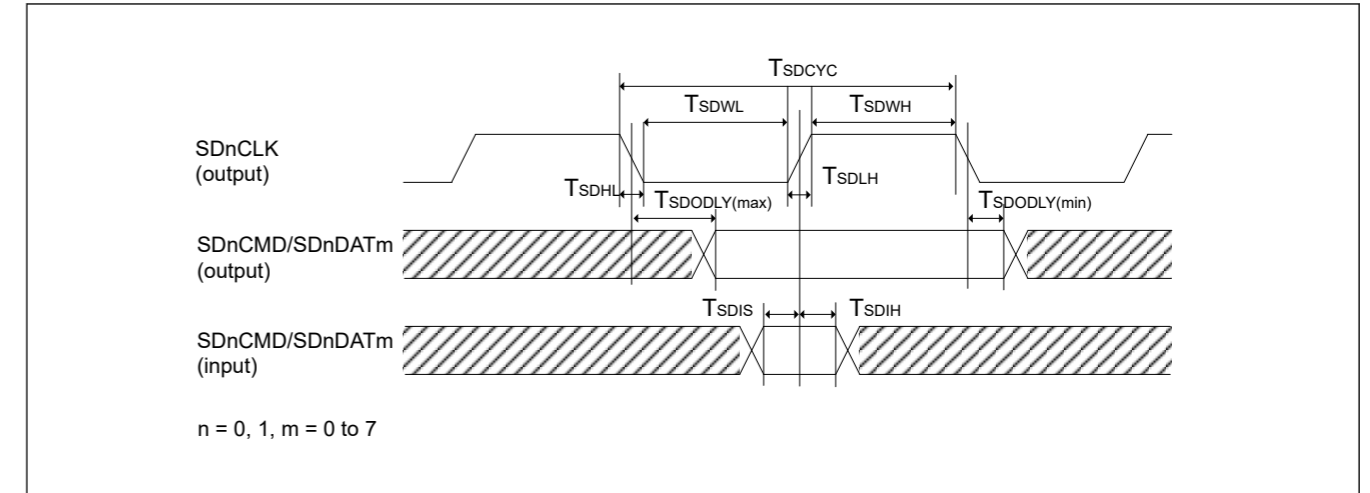
Figure 47.49 SDMMC主机接口信号时序
