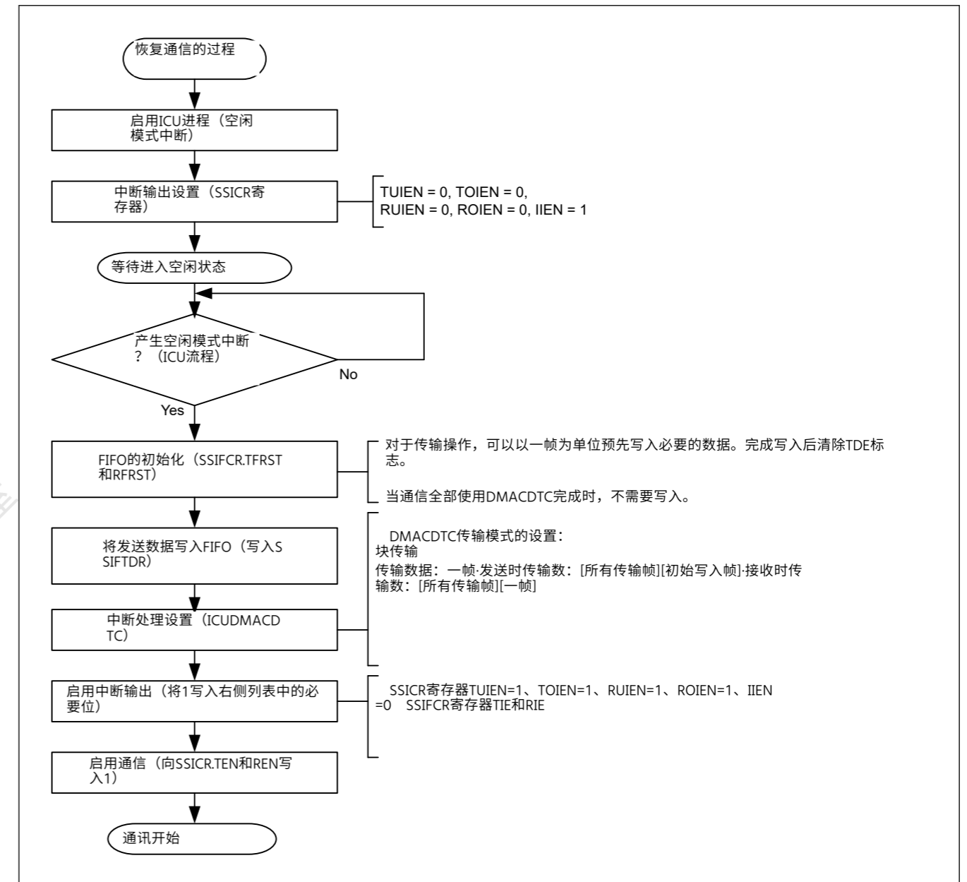
Figure 32.58 恢复通信的步骤 (CPU操作步骤)
