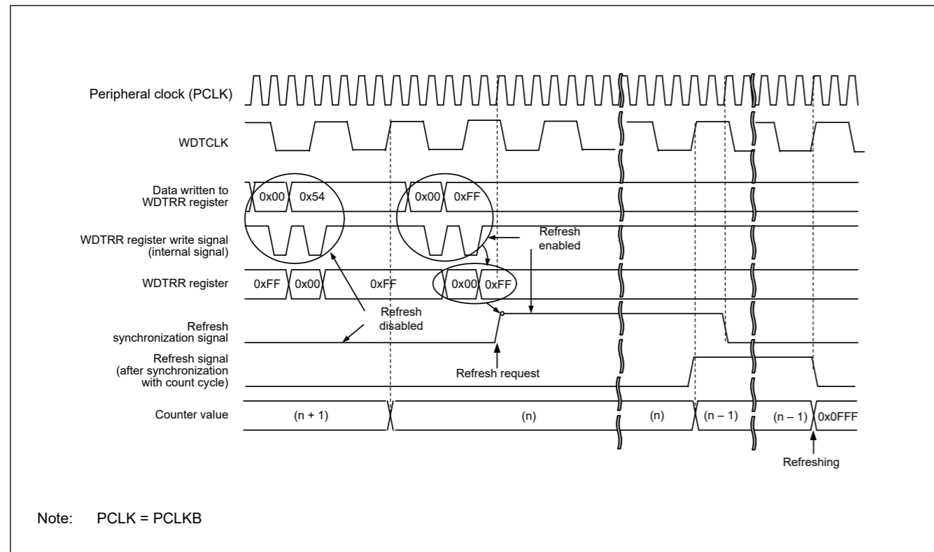
Figure 24.6 WDT refresh operation waveforms when WDTCSR.CKS[3:0] = 0x4 and WDTCSR.TOPS[1:0] = 01b
