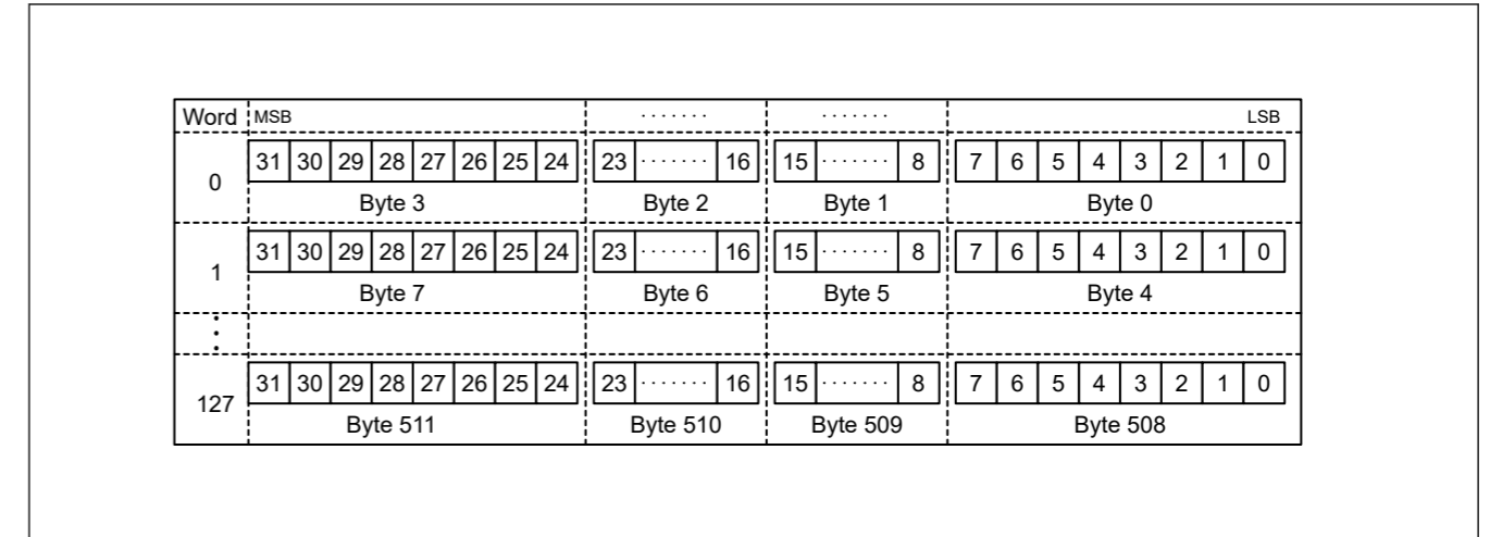
Figure 33.5 SD_BUF存储数据
