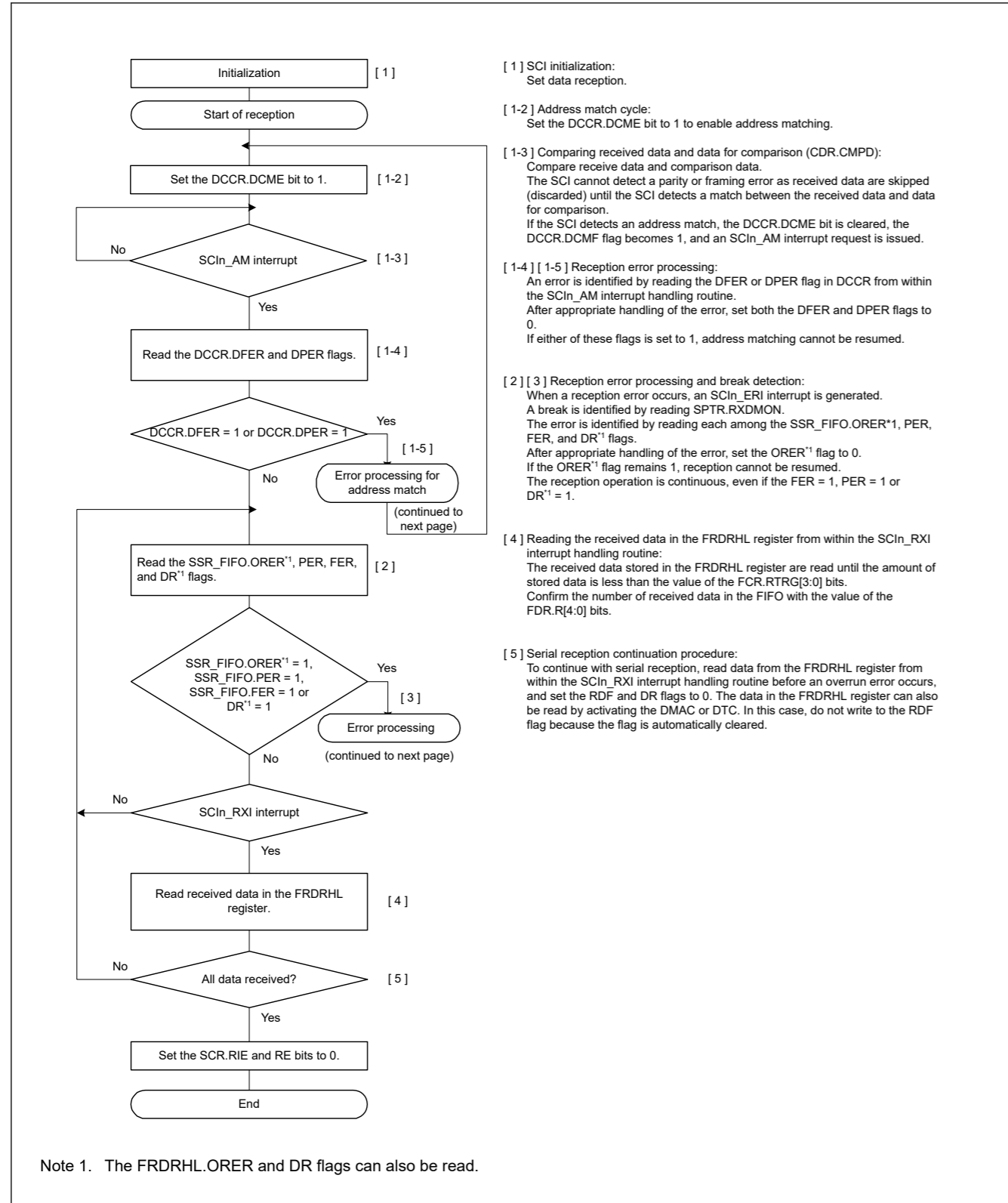
Figure 27.28 Example Flowchart of Serial Reception in Asynchronous Mode (FIFO Selected and Address Matching Enabled) (1)
