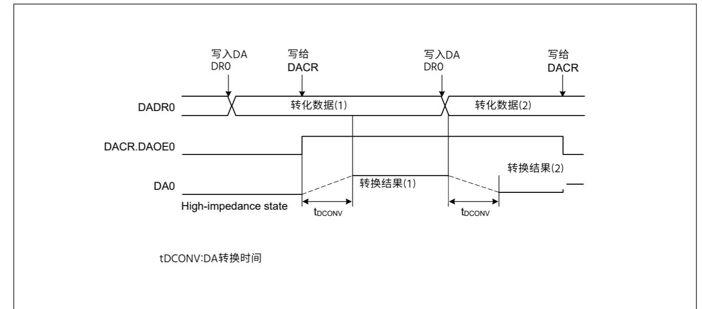
Figure 38.2 DAC12操作示例
