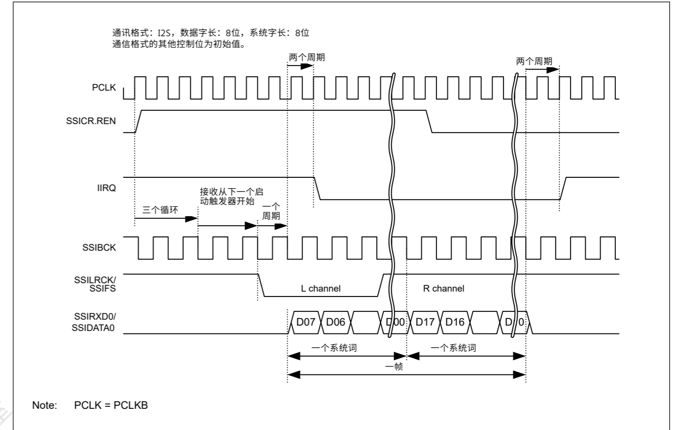
Figure 32.15 IIRQ设置时序 (接收)
