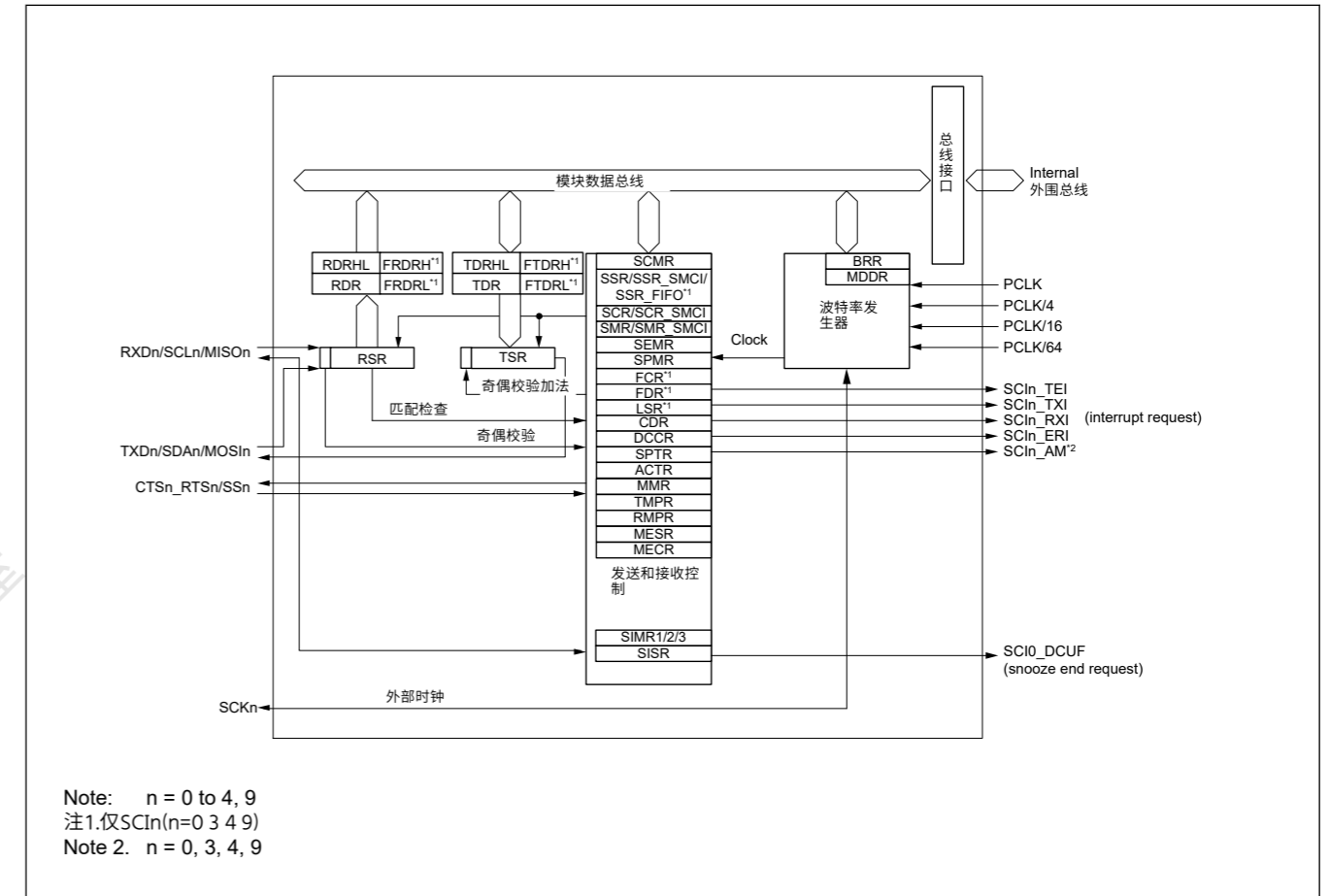
Figure 27.1 SCI框图
