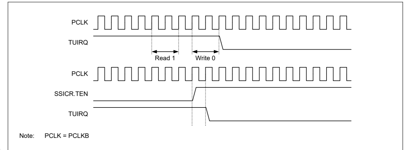
Figure 32.19 TUIRQ清零时机
