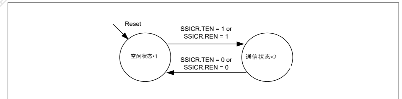
Figure 32.43 SSIE状态转换
