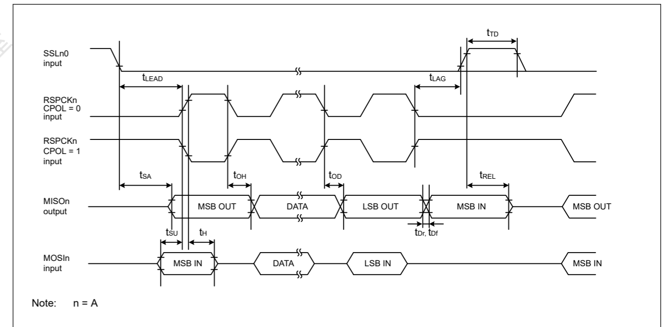
Figure 47.39 CPHA=0时从机的SPI时序
