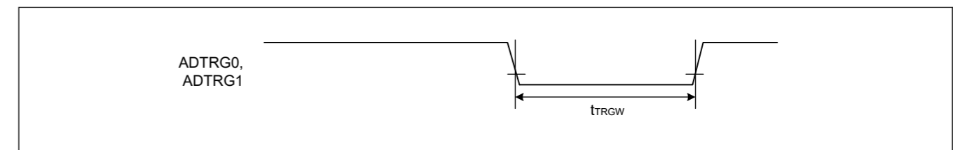
Figure 47.25 ADC12触发输入时序
