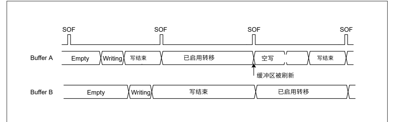
Figure 26.22 缓冲区刷新操作示例
