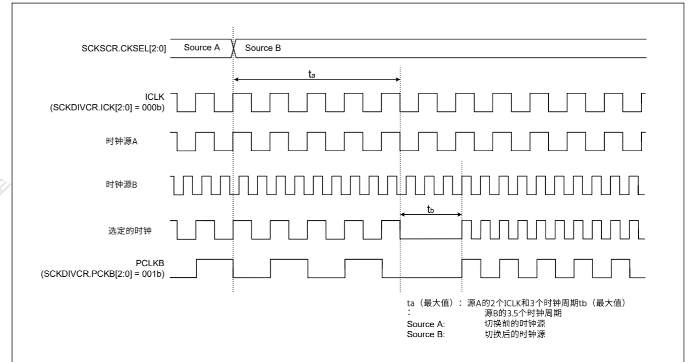
Figure 8.10 时钟源切换时序
