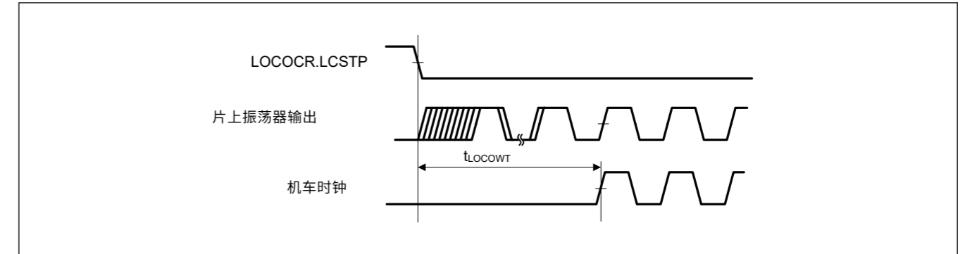
Figure 47.9 LOCO时钟振荡开始时序
