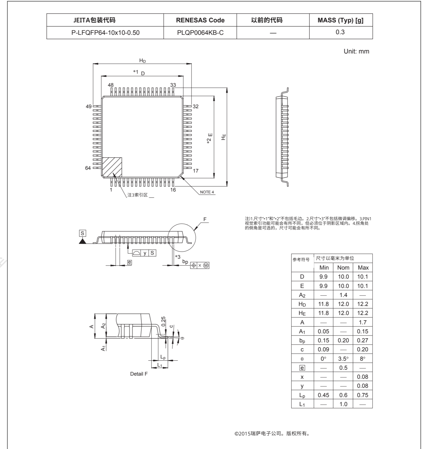
Figure 2.3 LQFP 64-pin
