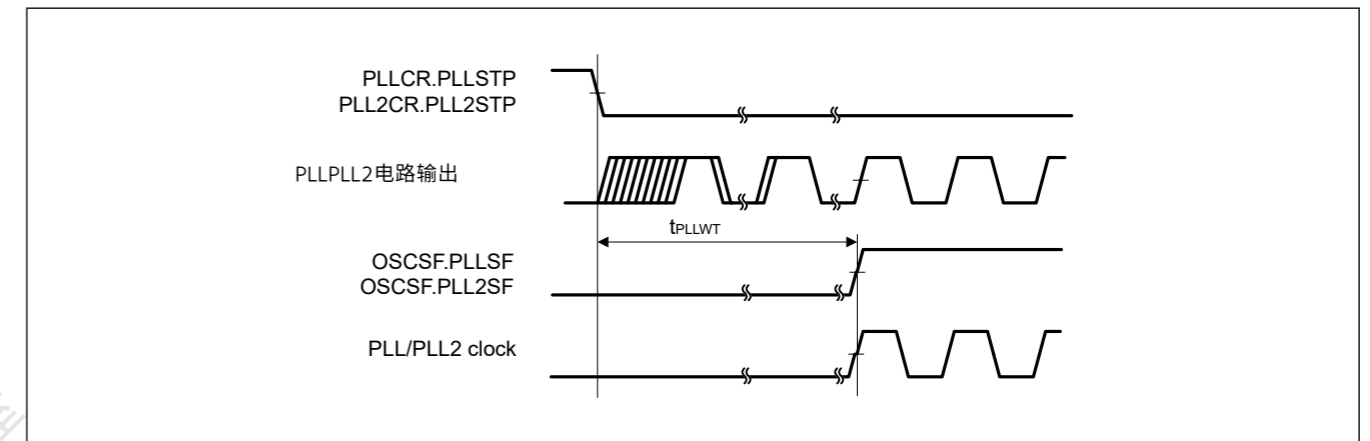
Figure 47.10 PLL/PLL2时钟振荡开始时序
