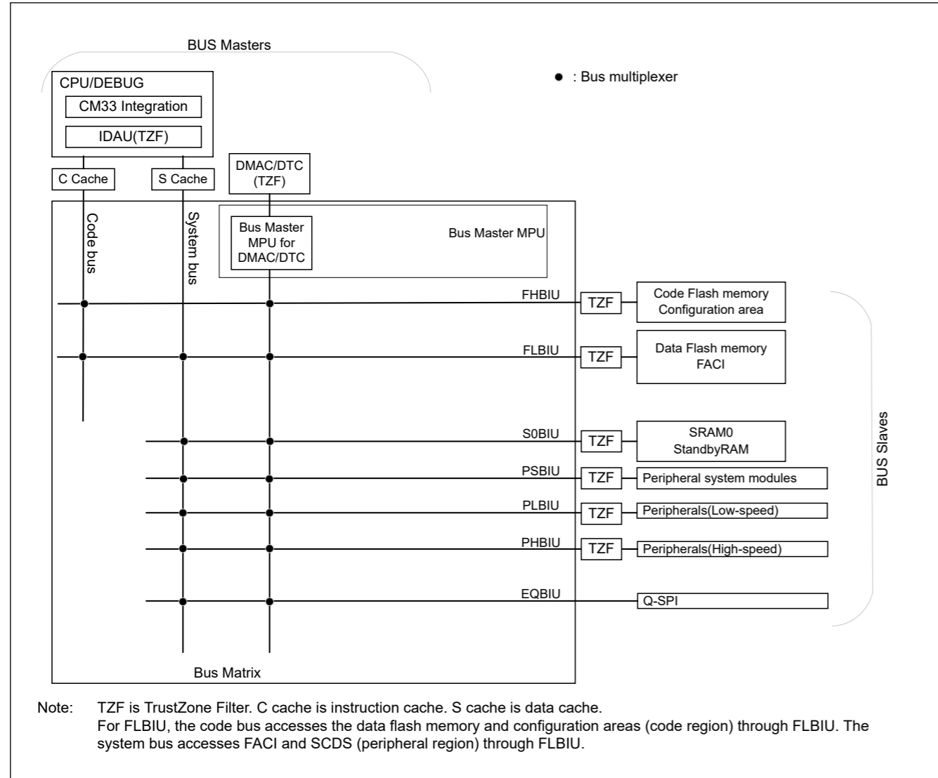
Figure 14.1 Bus Connection
