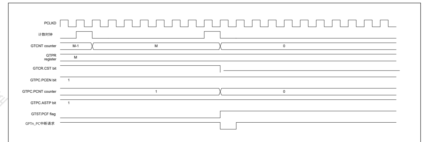
Figure 21.46 PWM周期计数功能的操作时序示例 (Saw-WaveOne-Shot脉冲模式, 递增计数)
