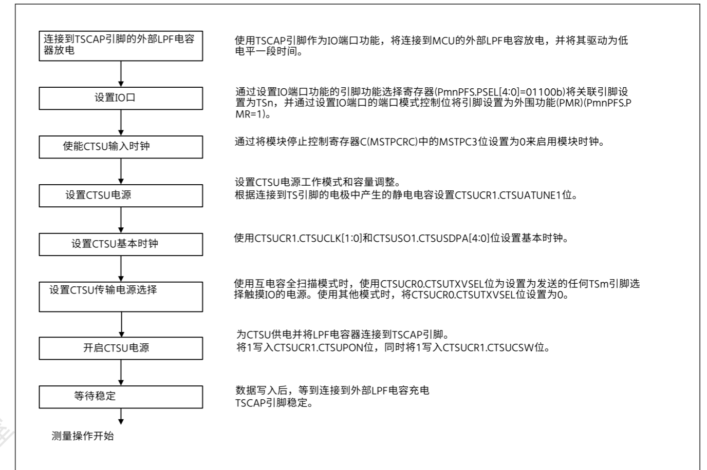
Figure 40.9 CTSU初始设置流程
