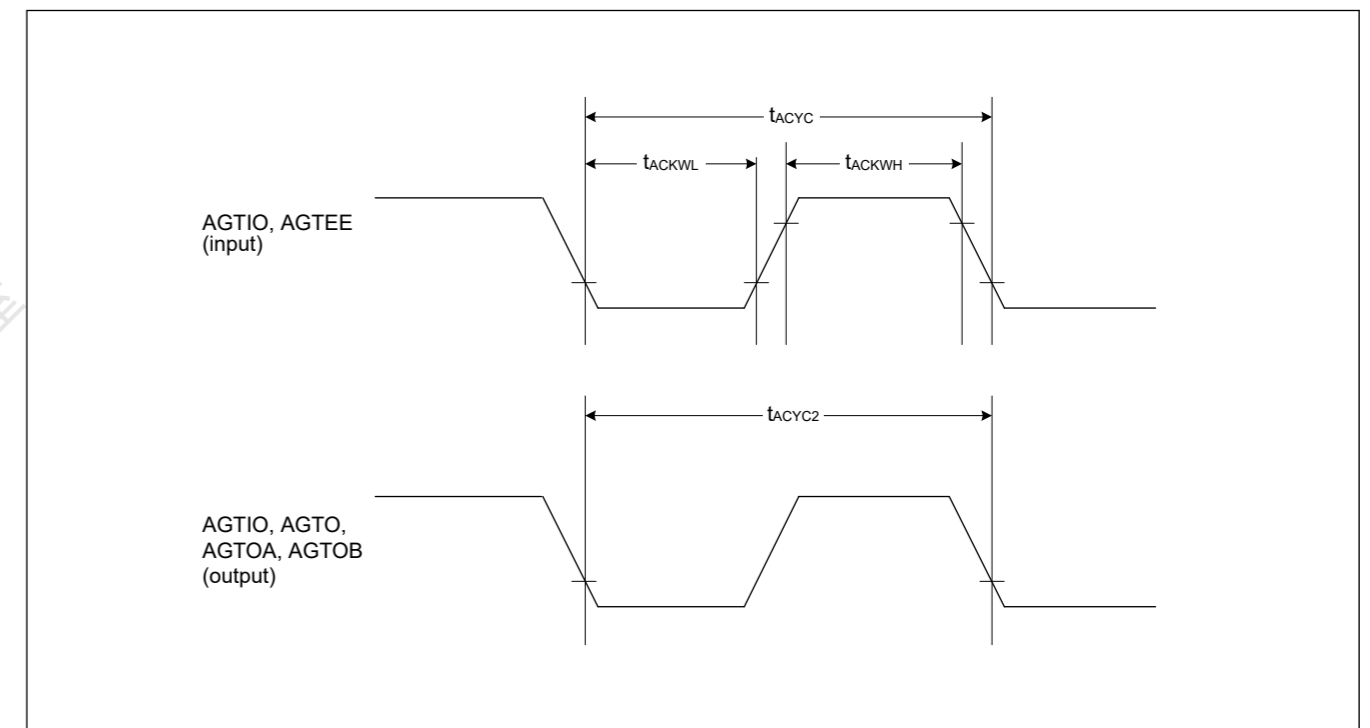
Figure 47.24 AGT input/output timing
