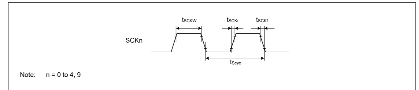
Figure 47.26 SCK时钟输入输出时序
