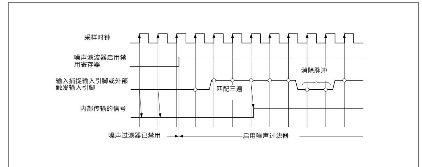
Figure 21.63 噪声过滤的时序
