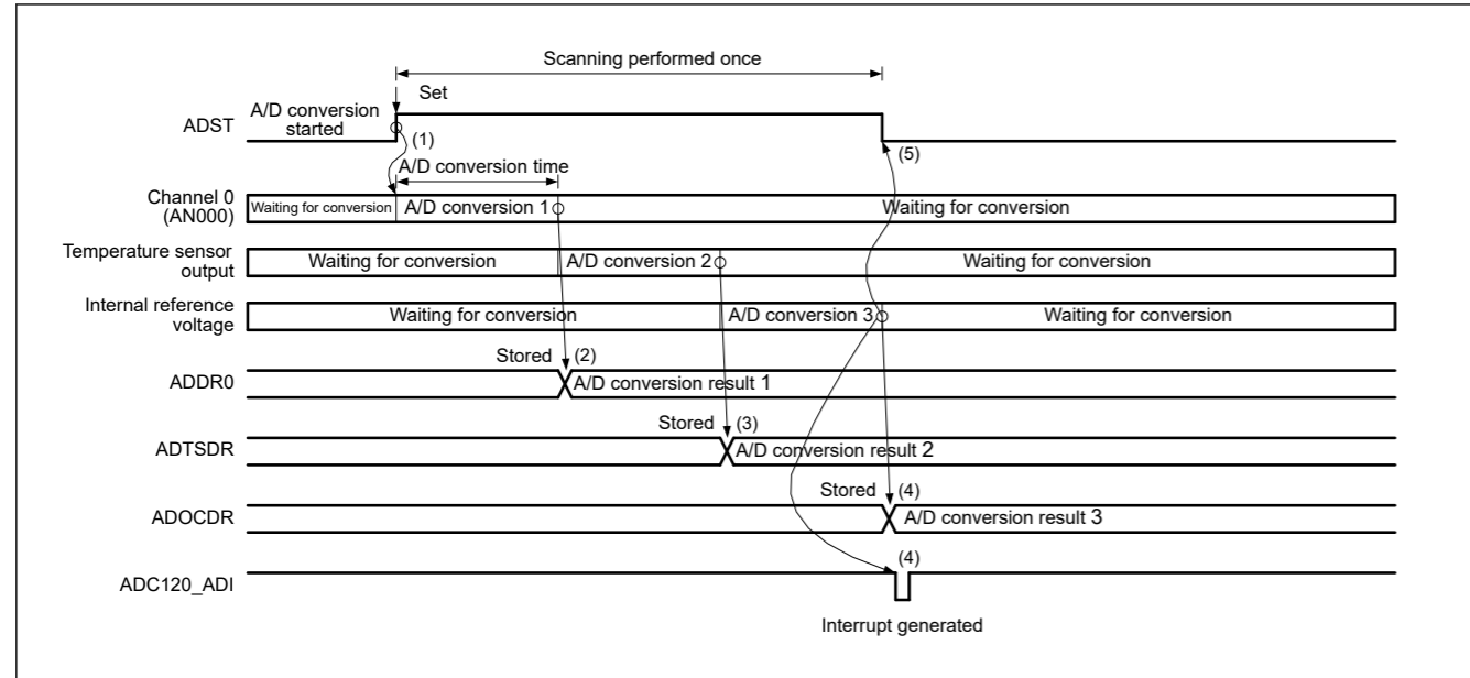
Figure 37.10 Example basic operation in single scan mode when AN000 and temperature sensor output or internal reference voltage are selected
