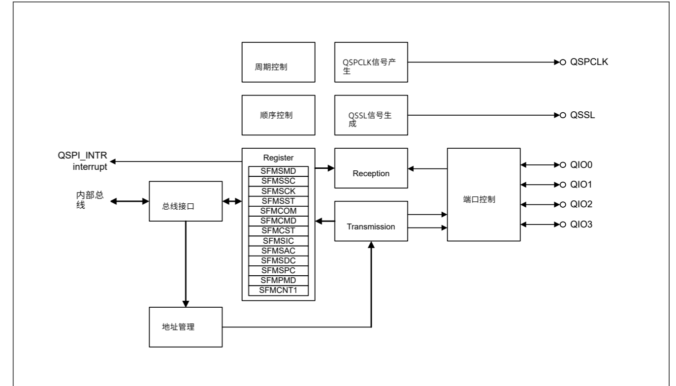
Figure 31.1 QSPI框图
