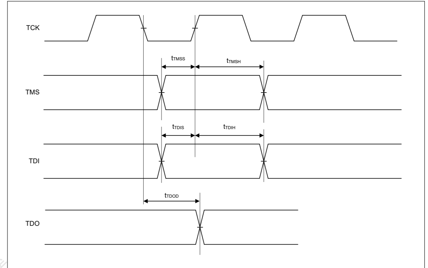
Figure 47.67 JTAG input/output timing
