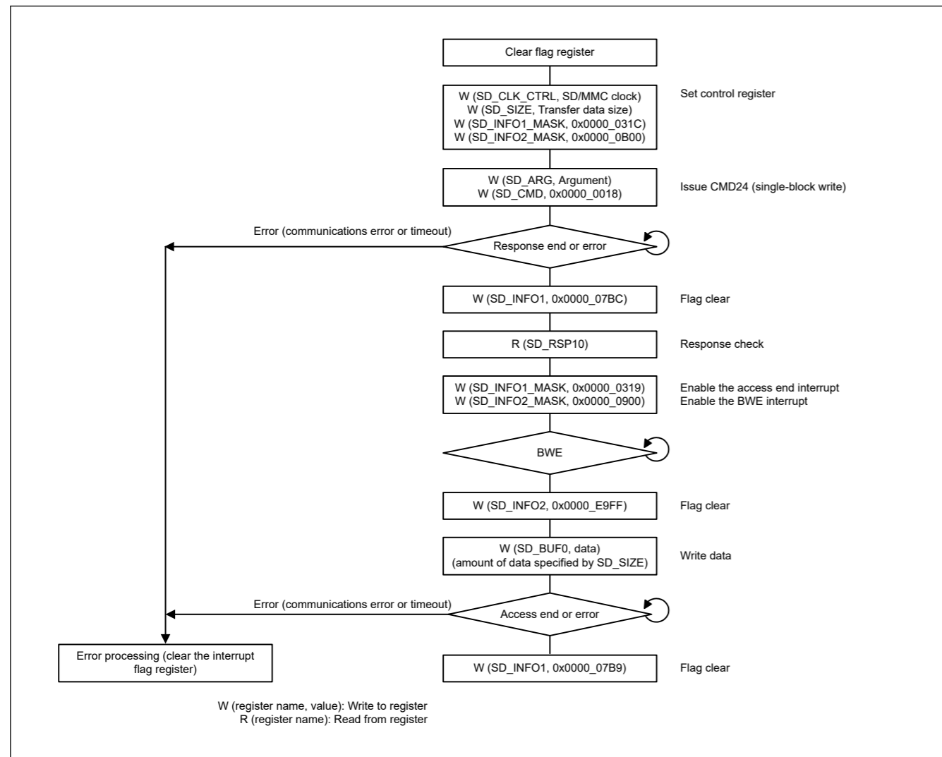
Figure 33.12 Example of single block write operation
