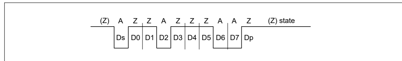
Figure 27.79 Direct convention with SDIR in SCMR = 0, SINV in SCMR = 0, and PM in SMR_SMCI = 0
