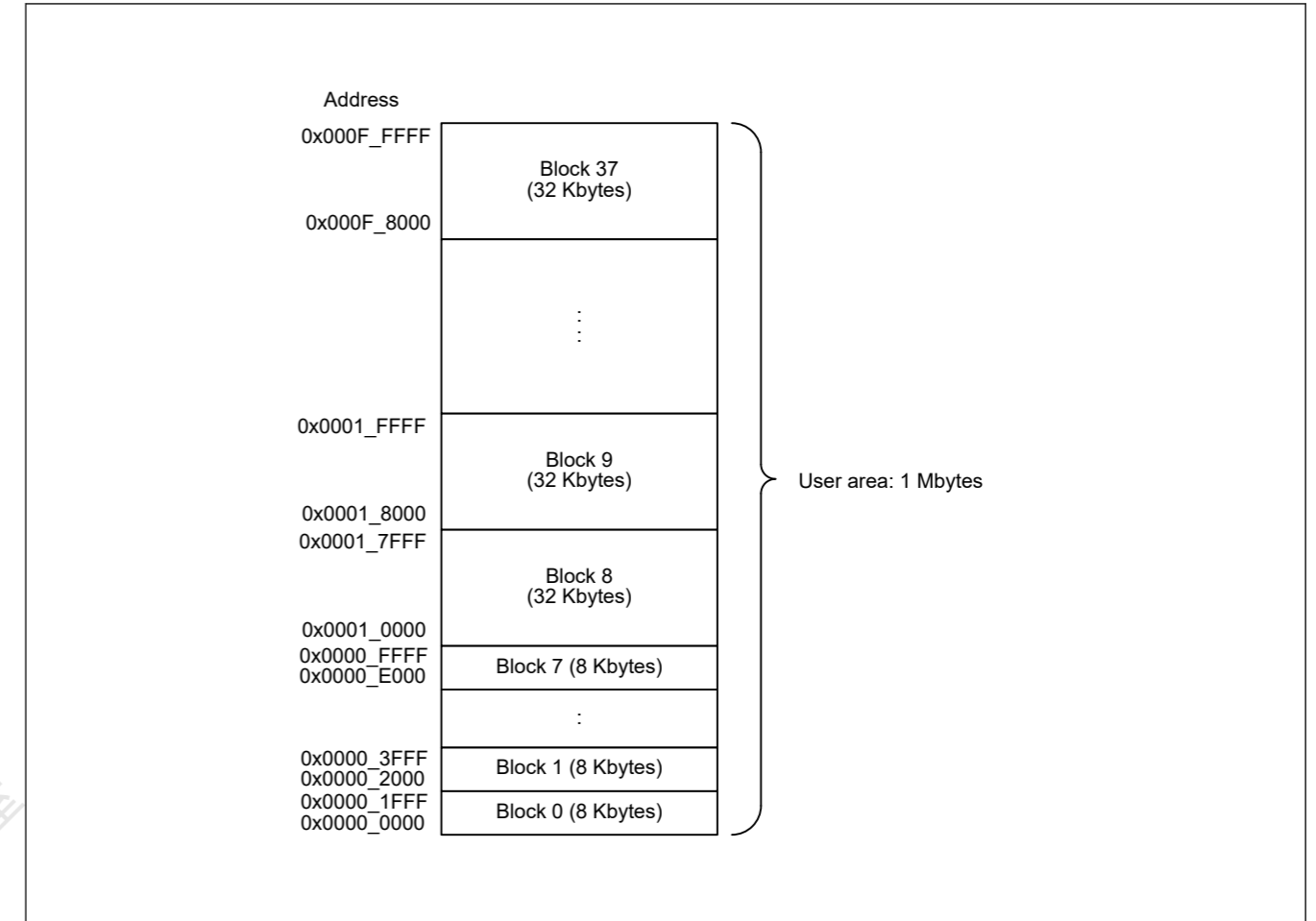
Figure 44.2 代码闪存映射
