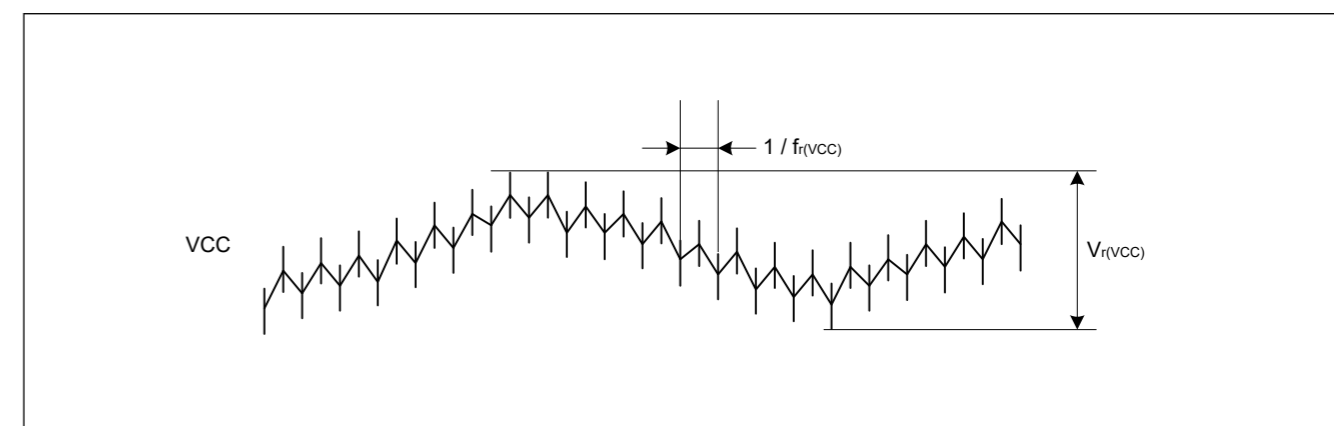
Figure 47.6 纹波波形
