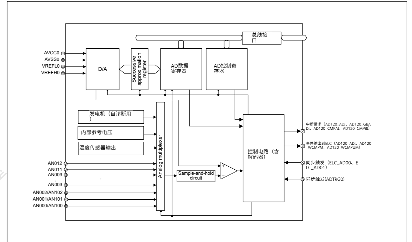
Figure 37.1 ADC12框图 (单元0)
