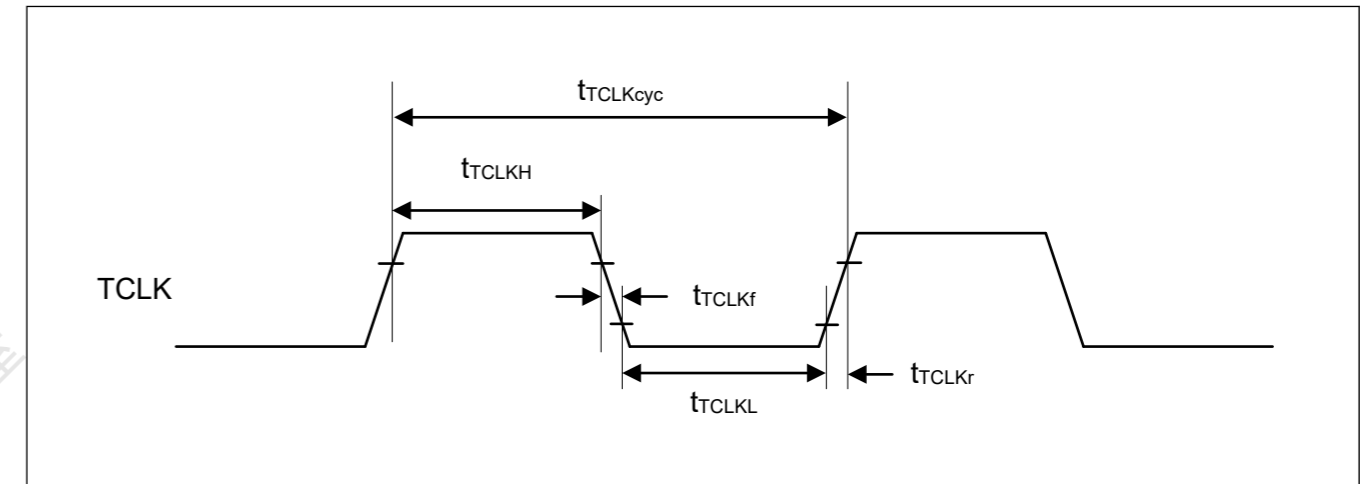
Figure 47.70 ETM TCLK timing
