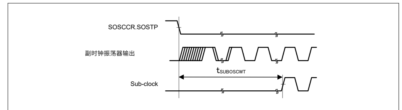
Figure 47.11 副时钟振荡开始时序
