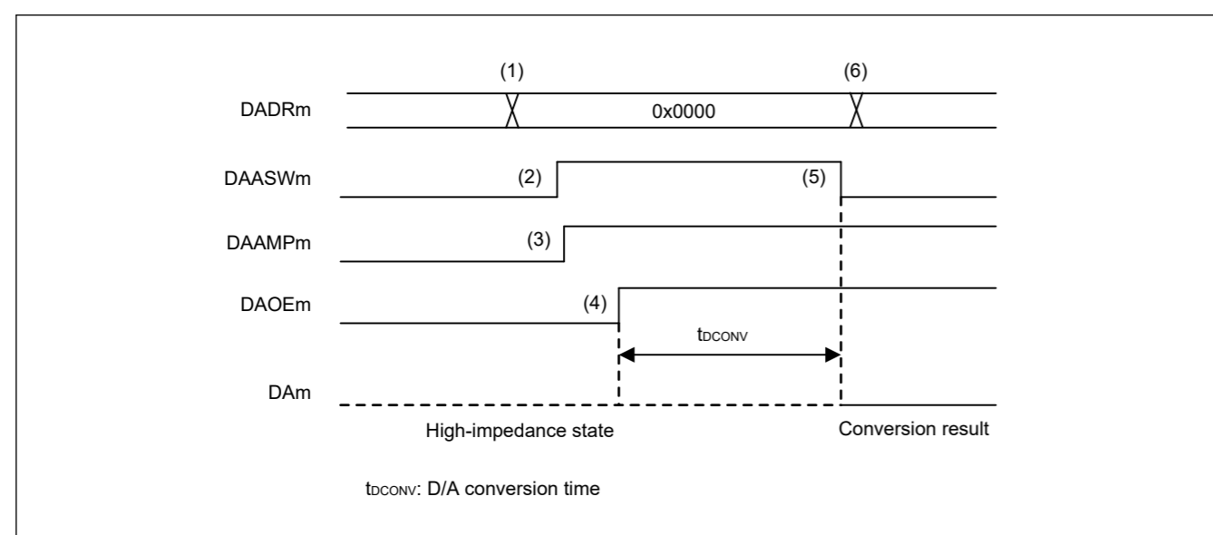
Figure 38.5 Example of the initial flow with the output amplifier in DAC12
