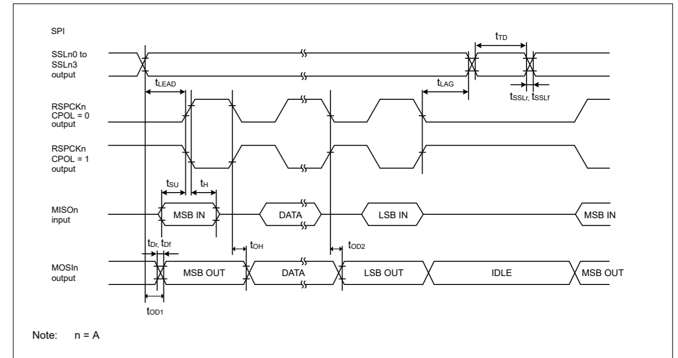
Figure 47.35 CPHA=0时主机的SPI时序
