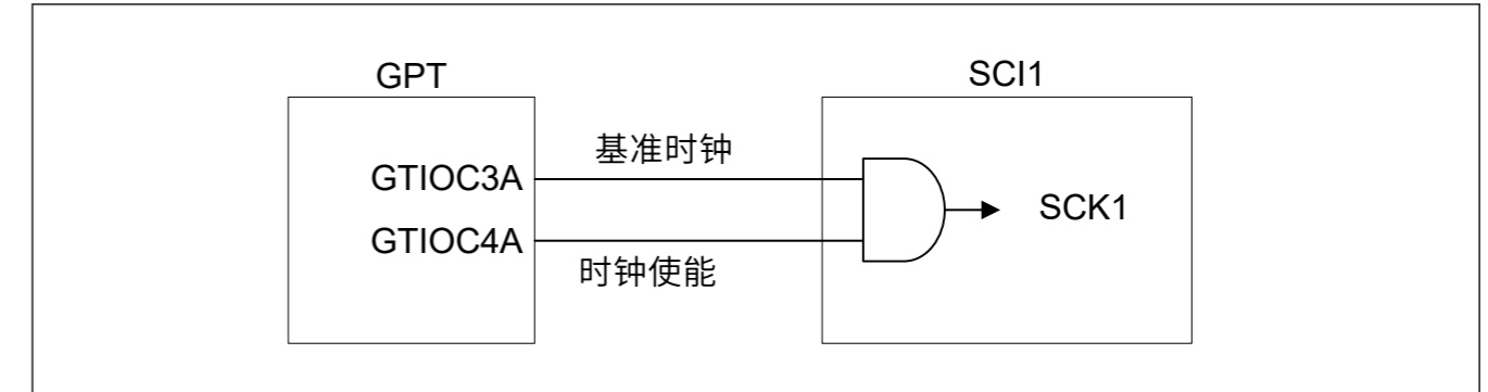
Figure 27.3 GPT和SCI连接示例
