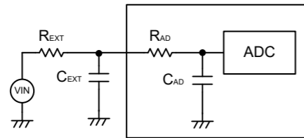
Figure 37.40 Sample and hold circuit simplified diagram
