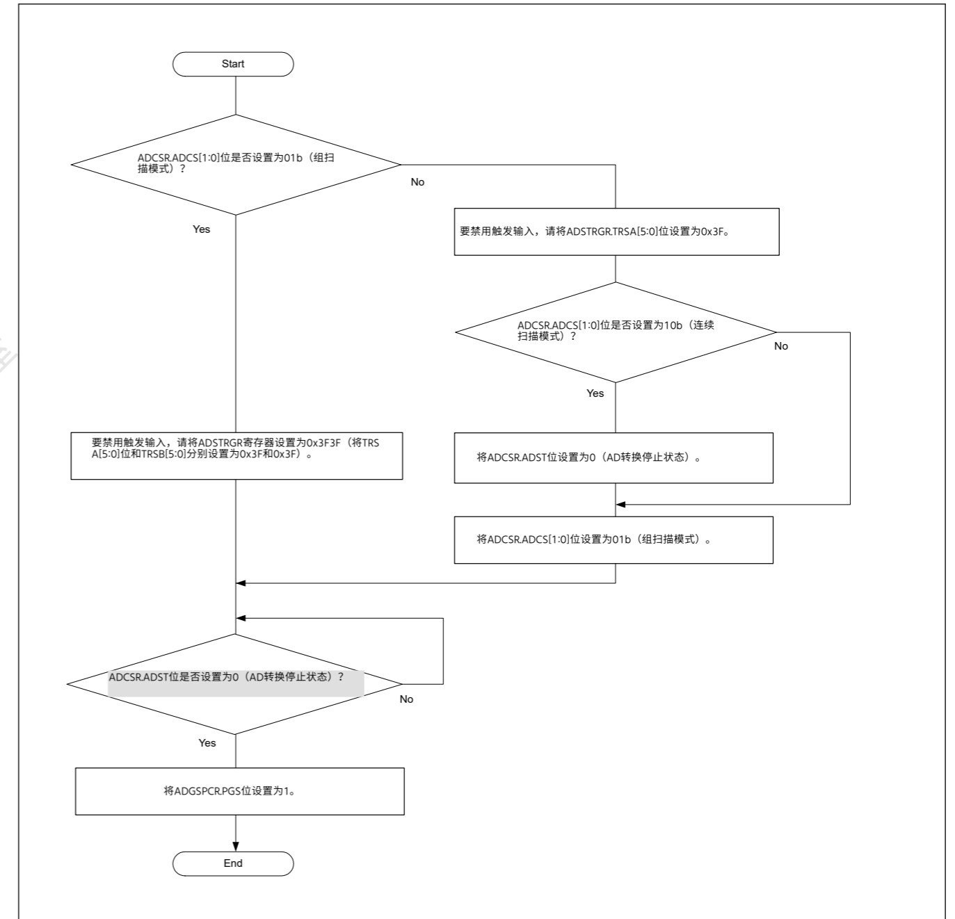
Figure 37.18 ADGSPCR.PGS位设置流程图
