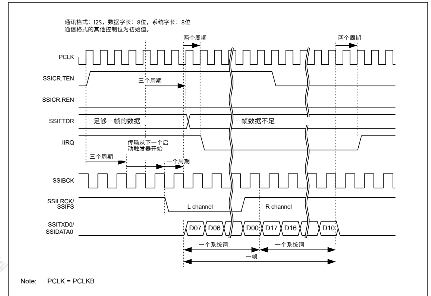
Figure 32.14 IIRQ设置时序 (传输)
