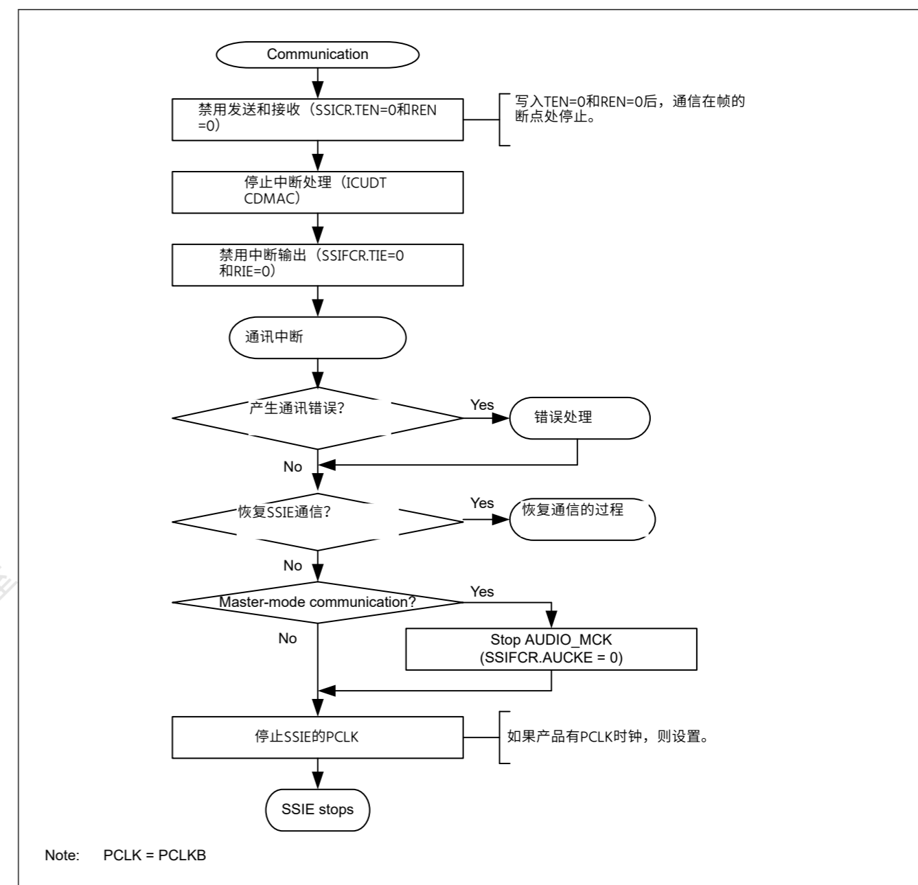
Figure 32.56 停止通信的步骤 (CPU操作步骤)
