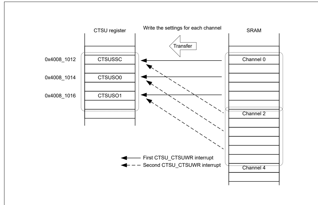
Figure 40.19 Example of DTC transfer operation using the CTSUSUWR interrupt
