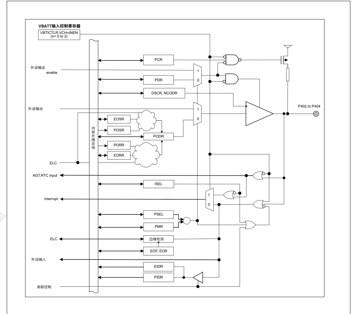
Figure 19.5 P402, P403, P404 diagram
