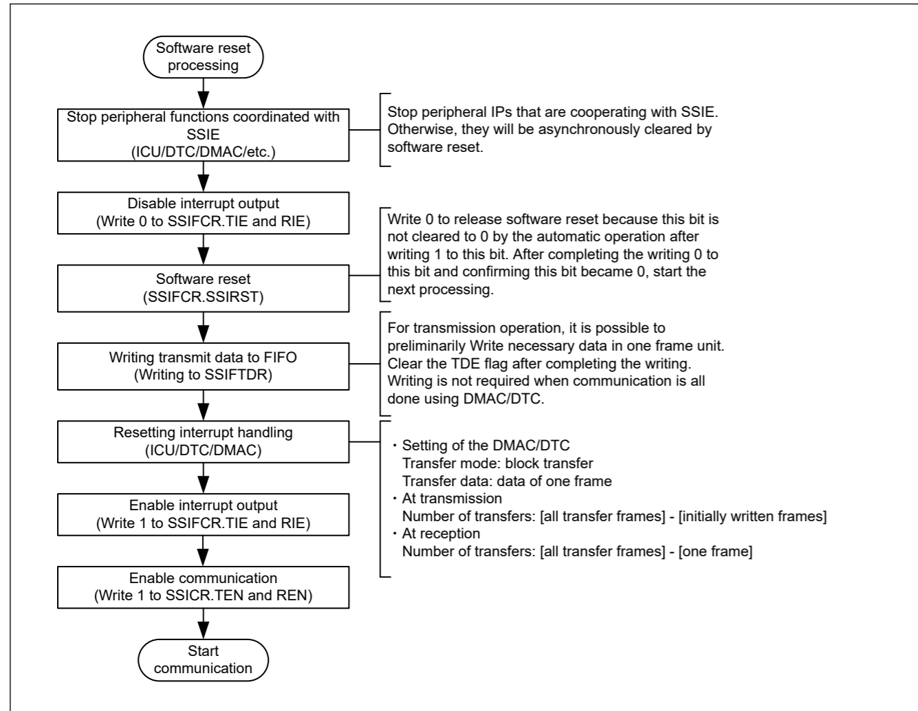
Figure 32.61 Software reset procedure (CPU operation procedure)
