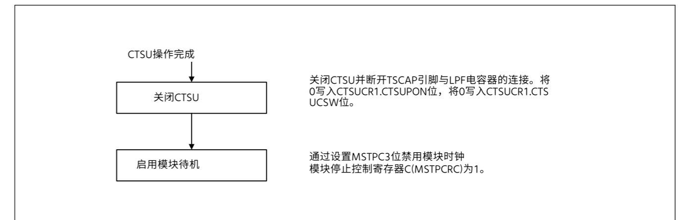
Figure 40.10 CTSUS停止流程
