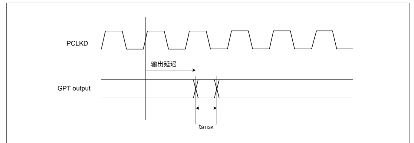
Figure 47.22 GPT输出延迟偏差
