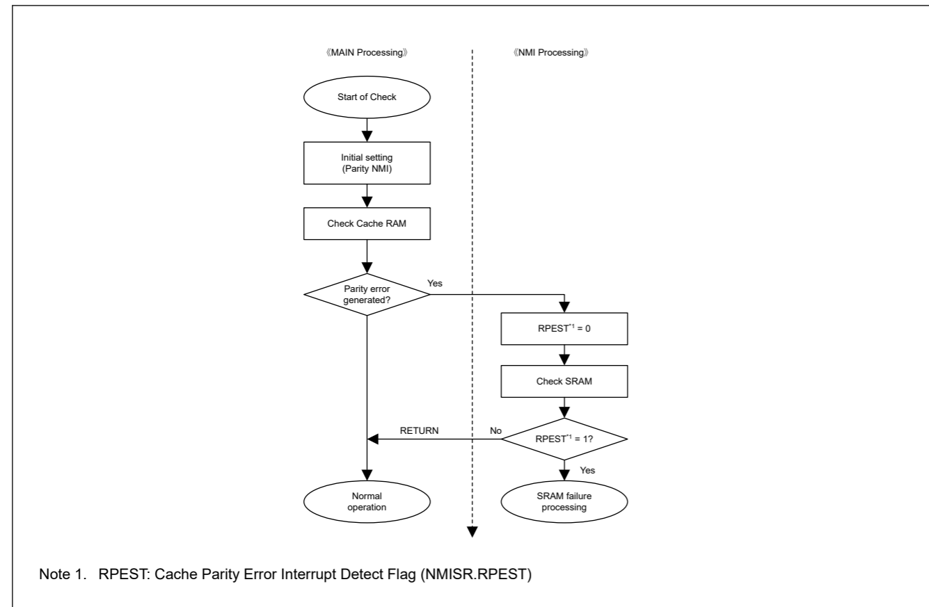
Figure 14.9 Flow of cache parity check when parity interrupt is enabled
