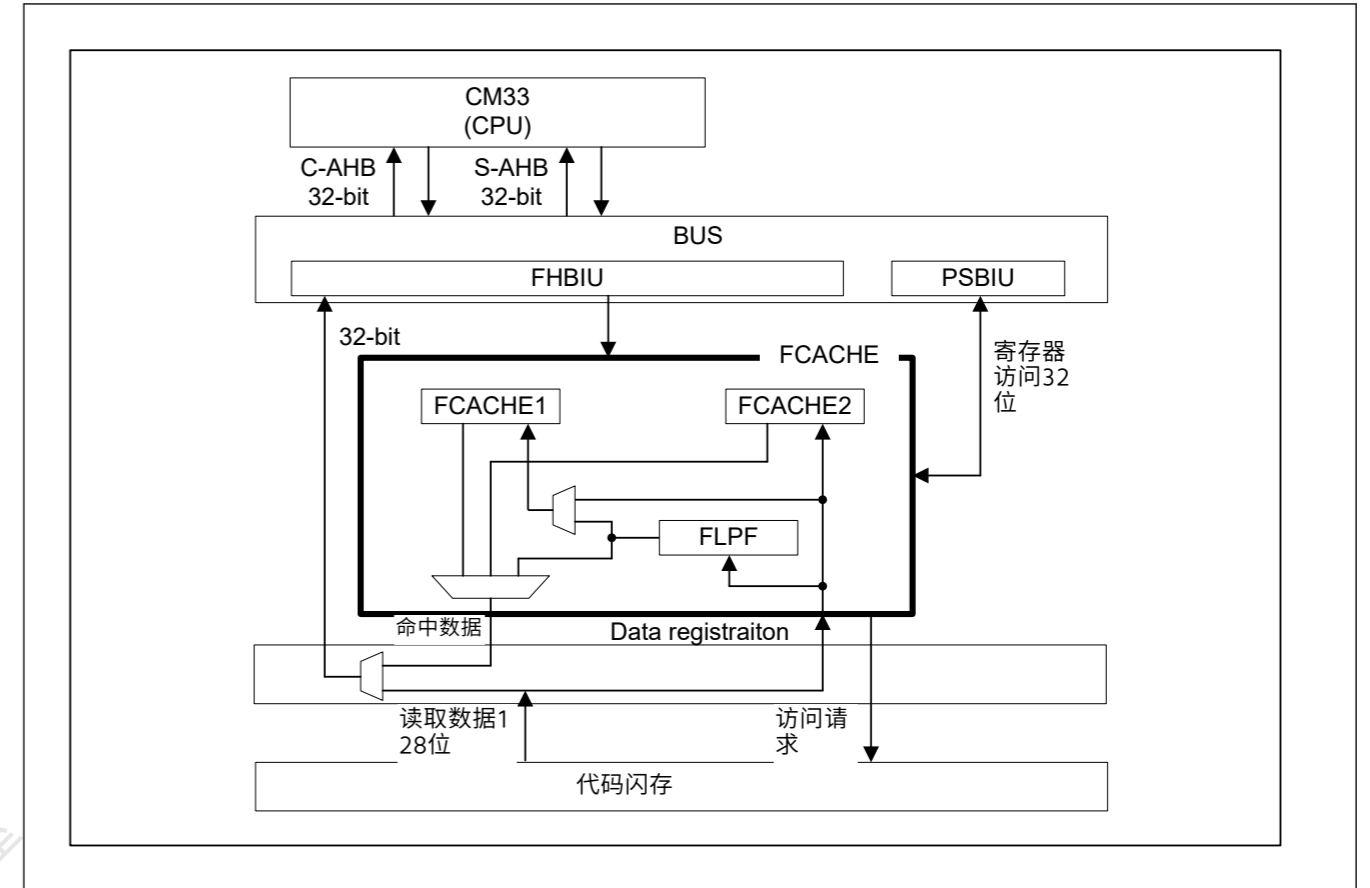
Figure 44.4 FCACHE的框图
