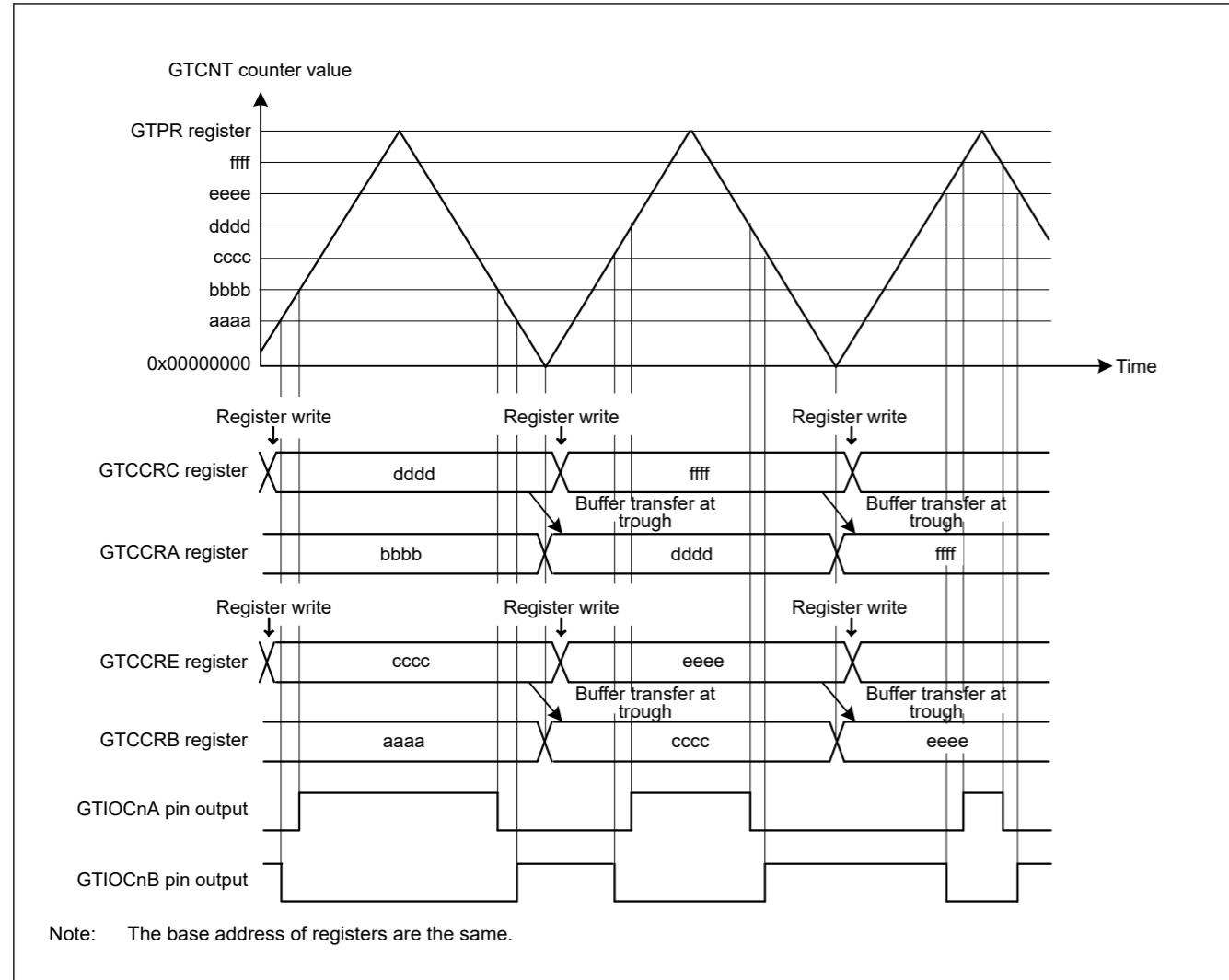
Figure 21.21 Example of triangle-wave PWM mode 1 operation with buffer operation, low output from the GTIOCnA pin and high output from the GTIOCnB pin at count start, output toggled at GTCCRA/GTCCRB register compare match, and output retained at cycle end
