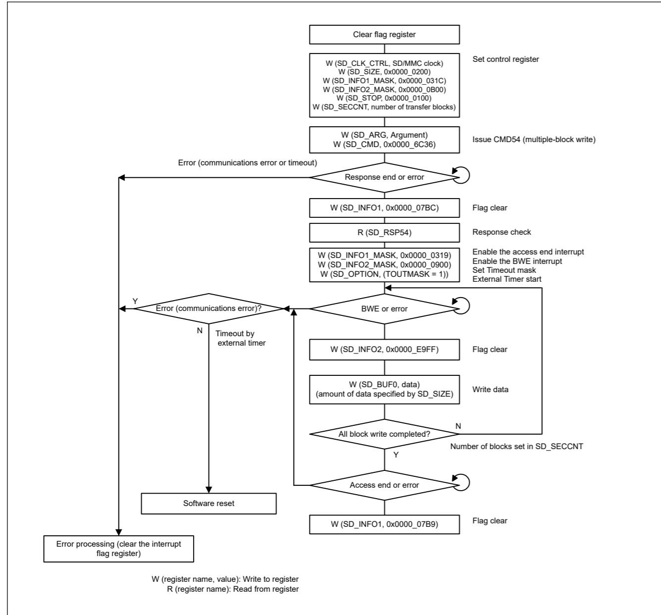
Figure 33.15 Example of multiple block write operation using external timer
