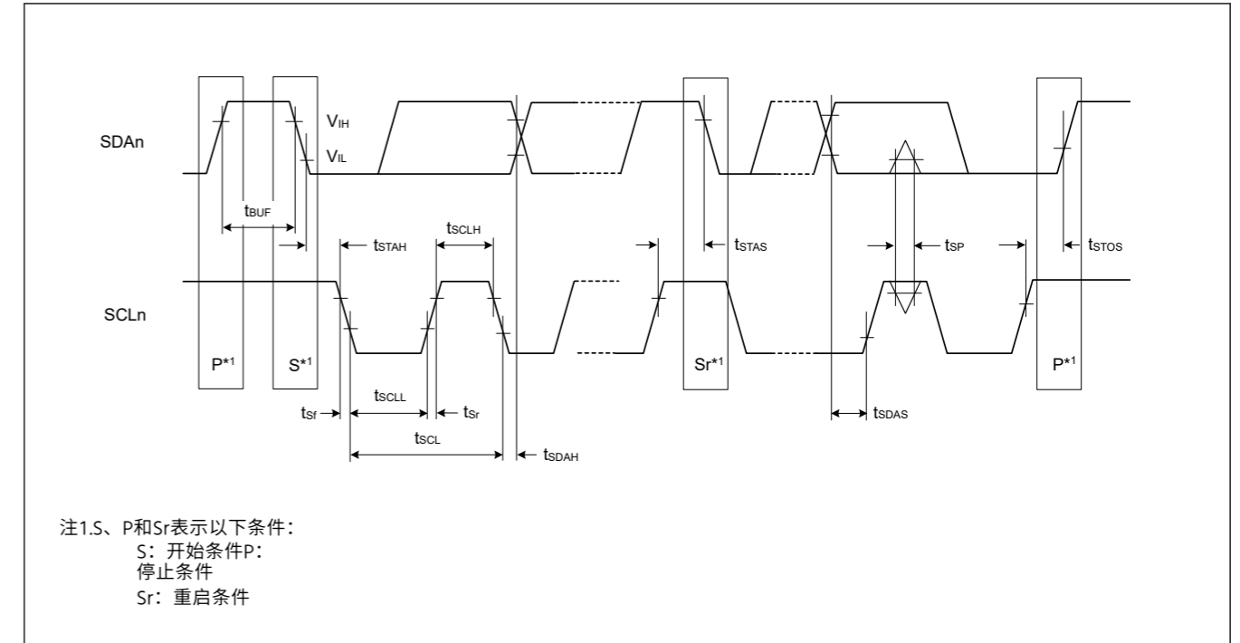
Figure 47.43 I 2 C总线接口输入输出时序
