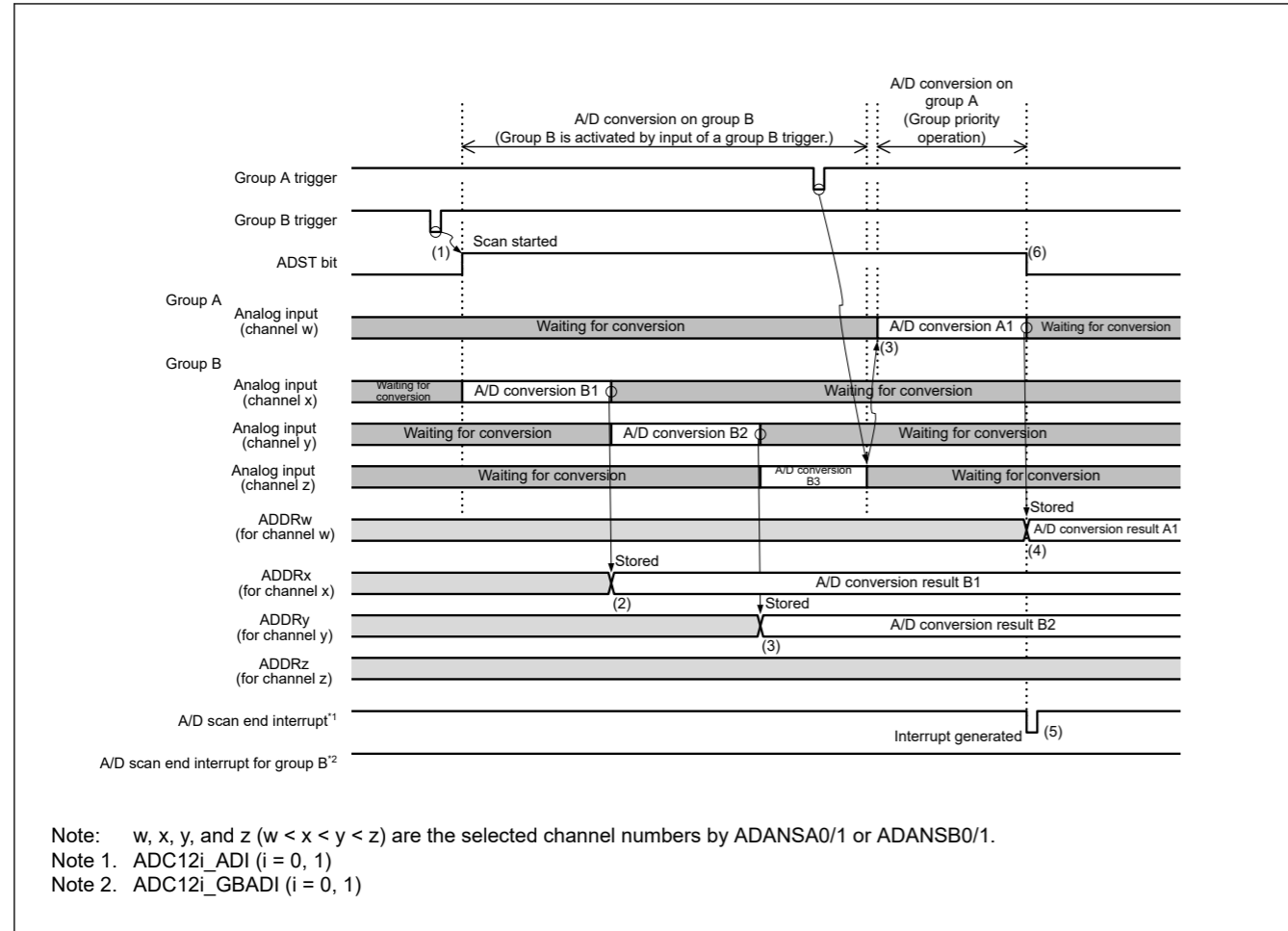
Figure 37.22 Group priority operation example 1-4: “Group A trigger is input during group B scan” when rescanning is disabled (when ADGSPCR.GBRSCN = 0, ADGSPCR.GBRP = 0, and ADGSPCR.LGRRS = 0)
