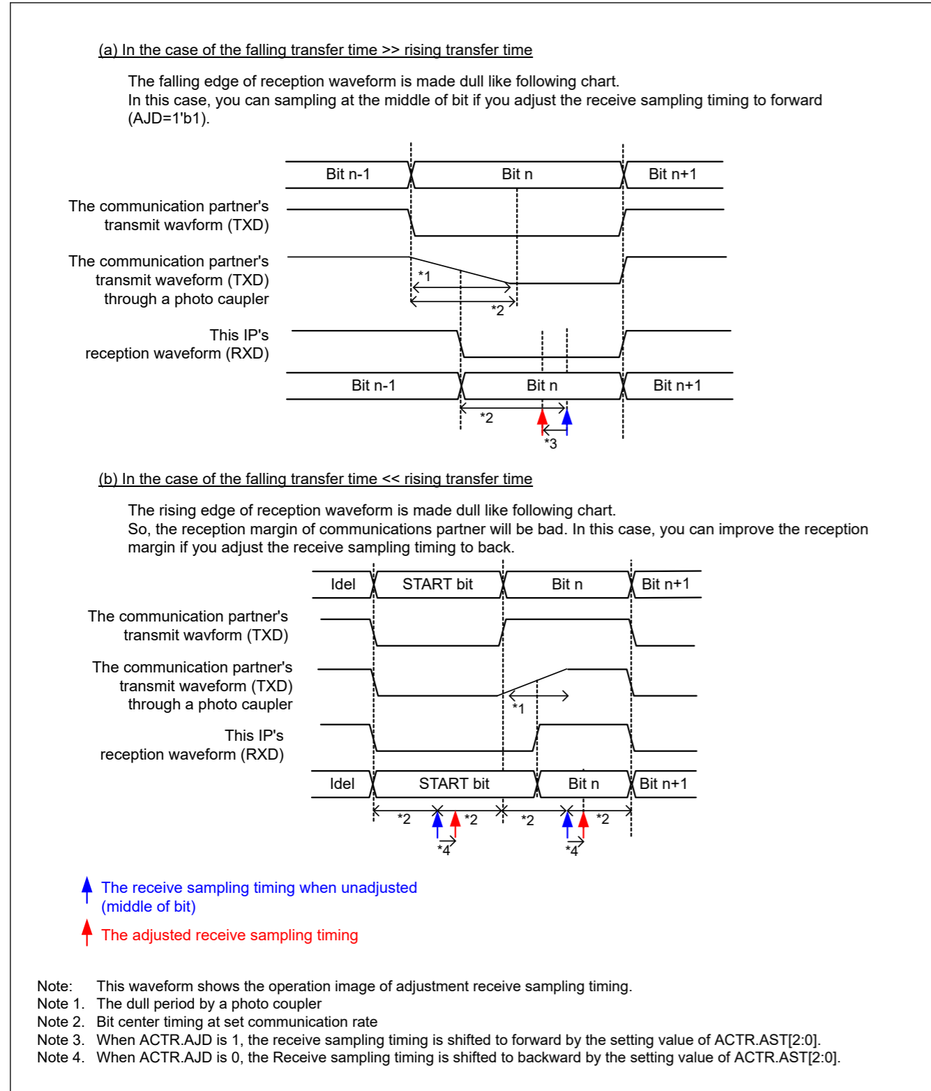
Figure 27.32 The reception movement image figure of the communication through a photo coupler
