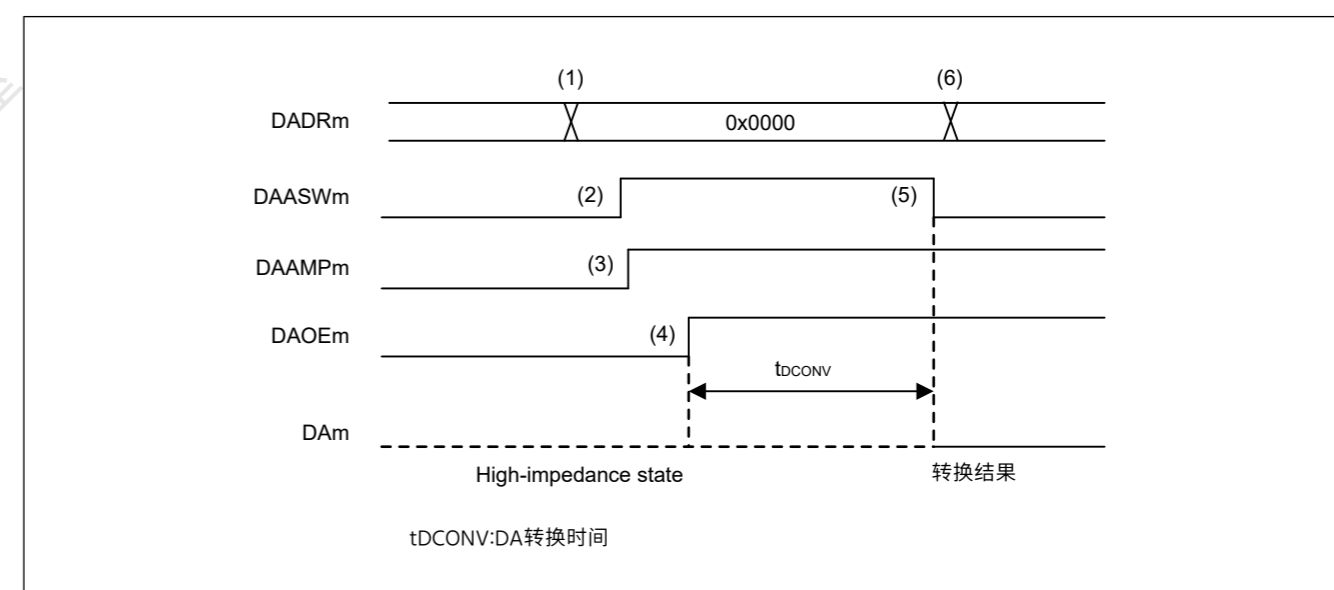
Figure 38.5 DAC12中输出放大器的初始流程示例
