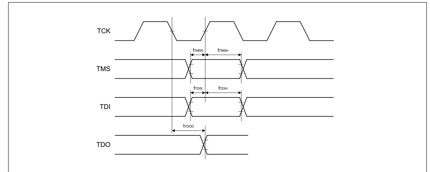
Figure 47.64 边界扫描输入输出时序
