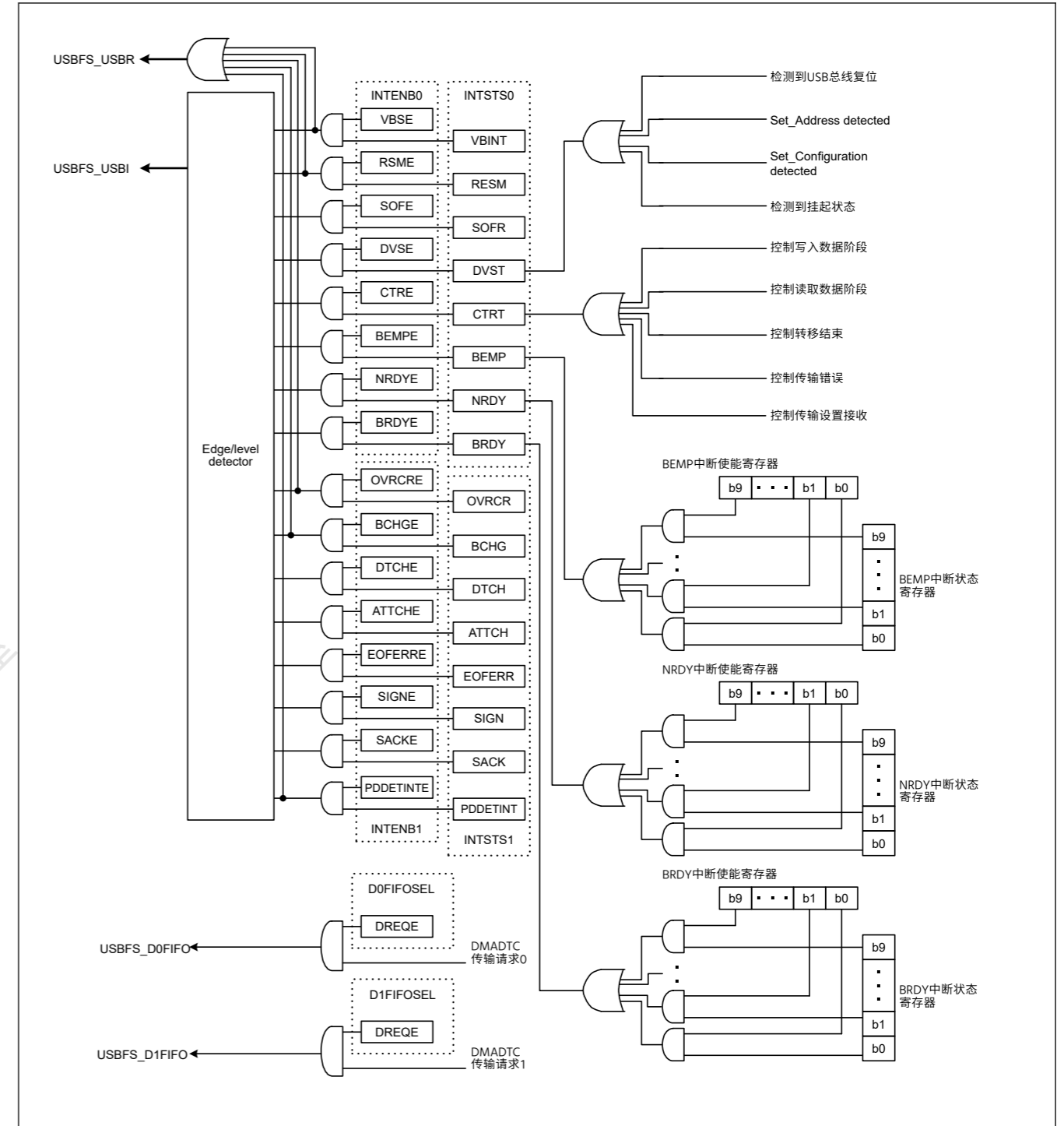
Figure 26.11 USBFS interrupt-related circuits
