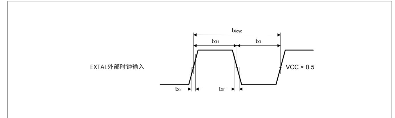
Figure 47.7 EXTAL外部时钟输入时序
