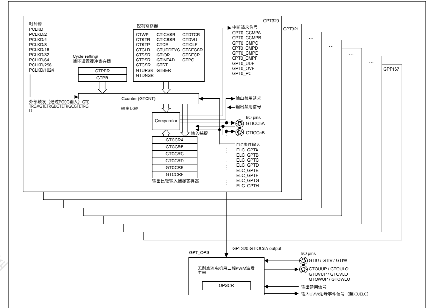
Figure 21.1 GPT框图
