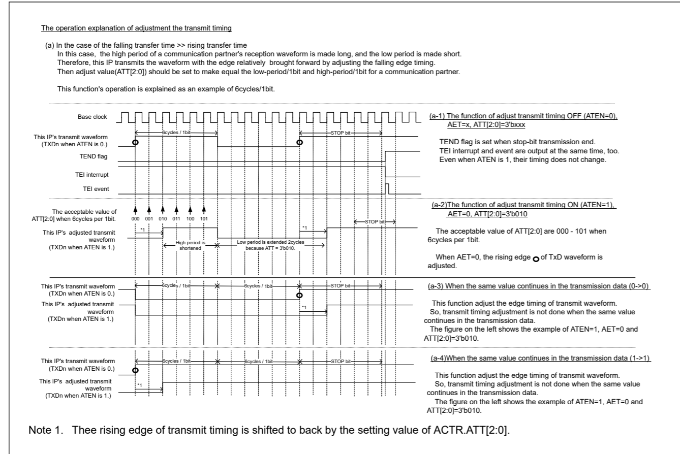
Figure 27.38 The adjustment operation explanation for the transmit timing when AET is 0
