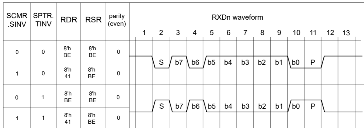
Figure 27.5 Example of the receive/transmit data control
