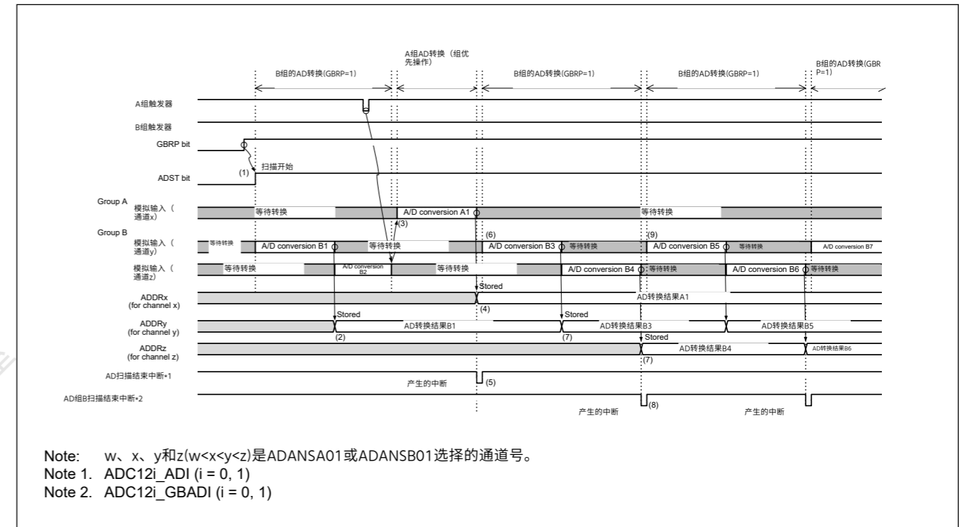
Figure 37.23 组优先操作示例1-5: B组连续激活单次扫描 (当 ADGSPCR.GBRP = 1, ADGSPCR.LGRRS = 0)
