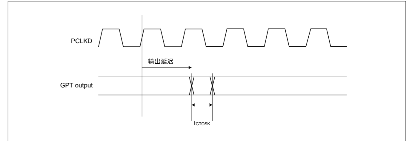
Figure 47.23 OPS的GPT输出延迟偏差
