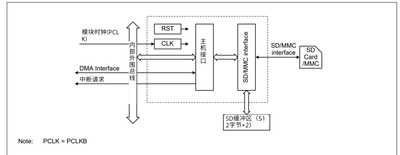
Figure 33.1 SDMMC主机接口框图
