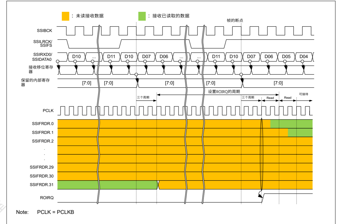
Figure 32.16 ROIRQ设置时序
