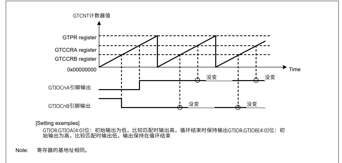
Figure 21.7 低输出和高输出操作示例
