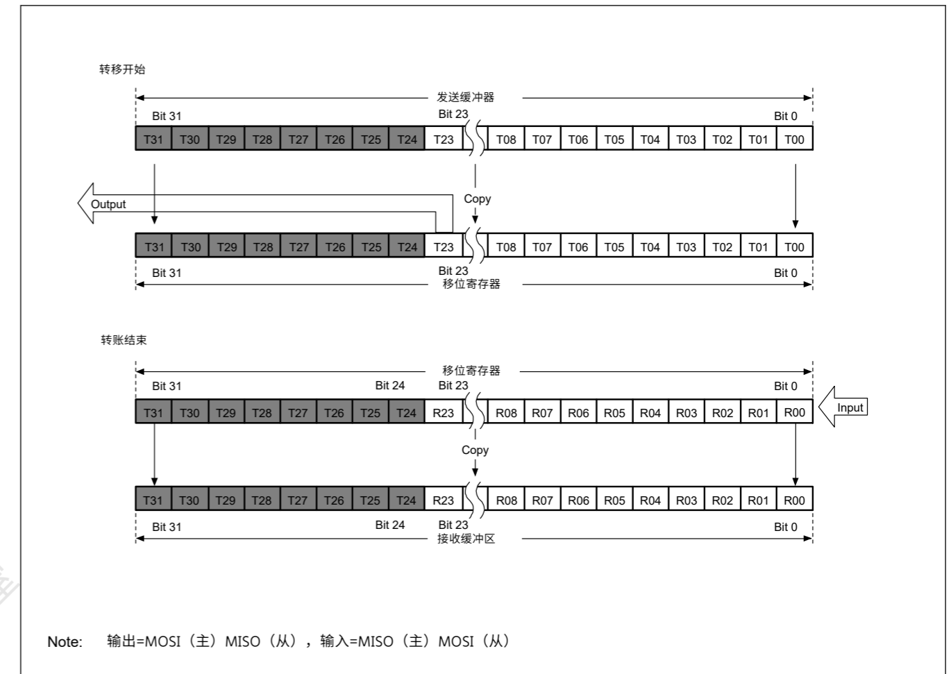
Figure 30.15 禁用24位数据和奇偶校验的MSB优先传输
