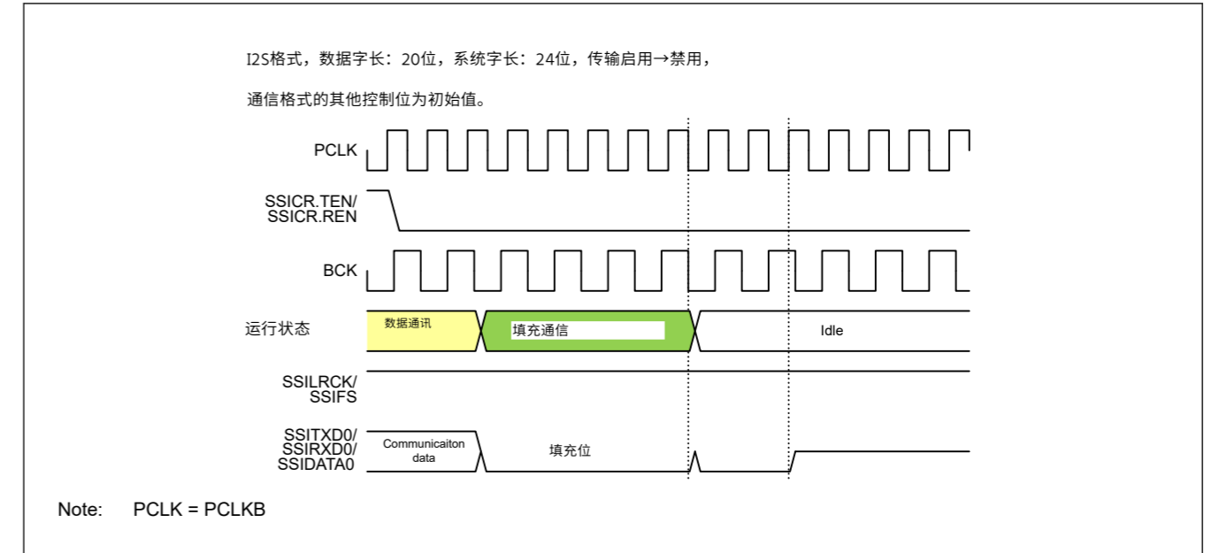
Figure 32.51 从填充通信中停止
