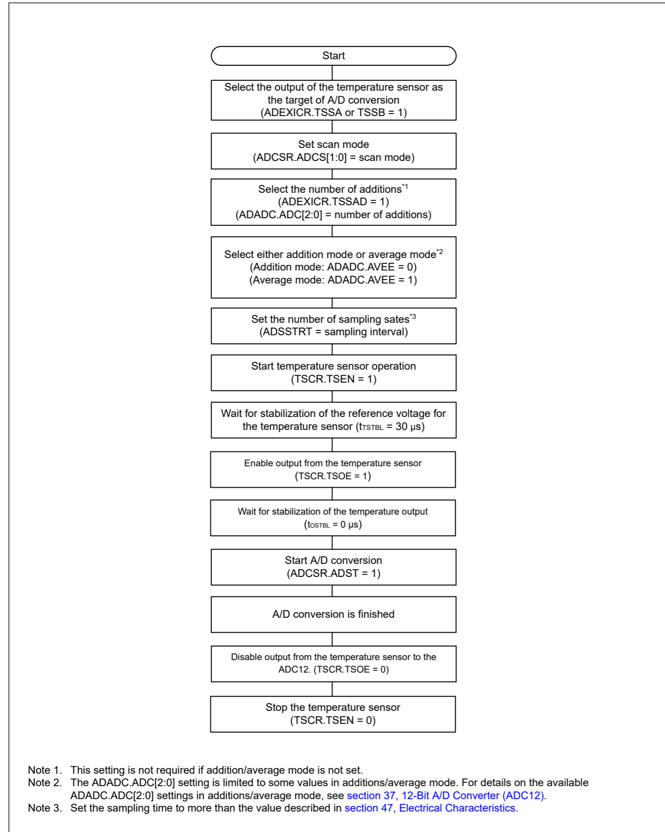
Figure 39.2 Procedure example for using the TSN
