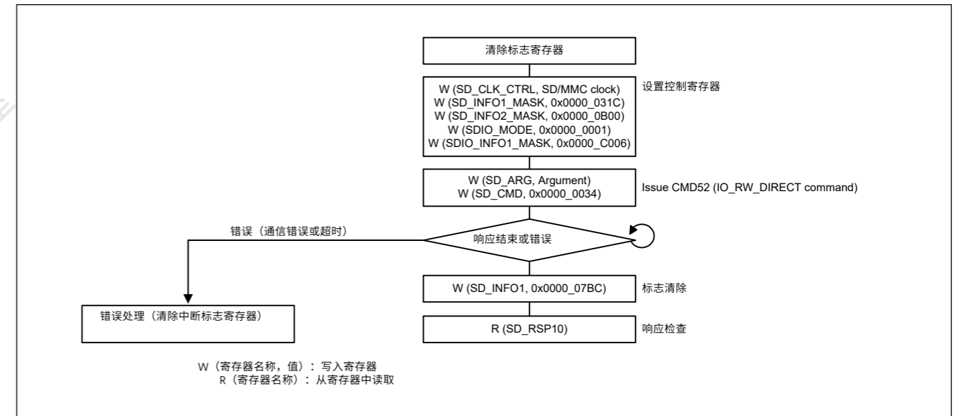
Figure 33.16 IO_RW_DIRECT命令(CMD52)操作示例
