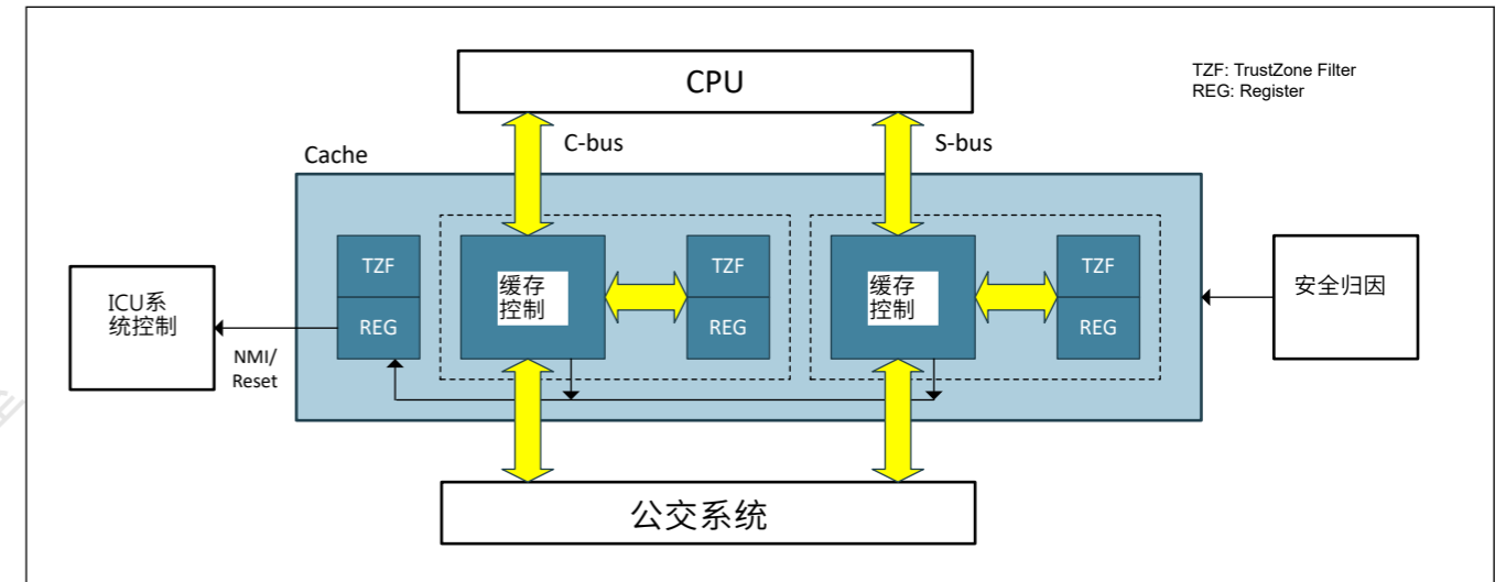
Figure 14.4 缓存框图
