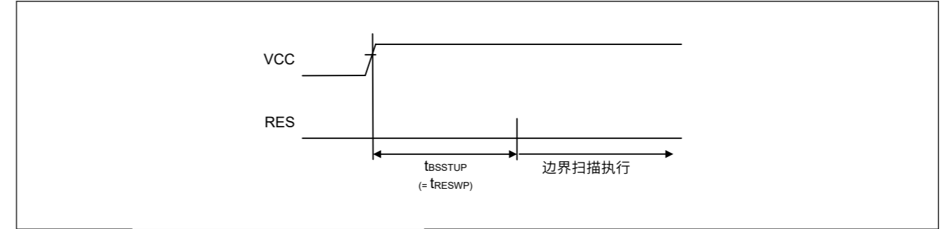
Figure 47.65 边界扫描电路启动时序
