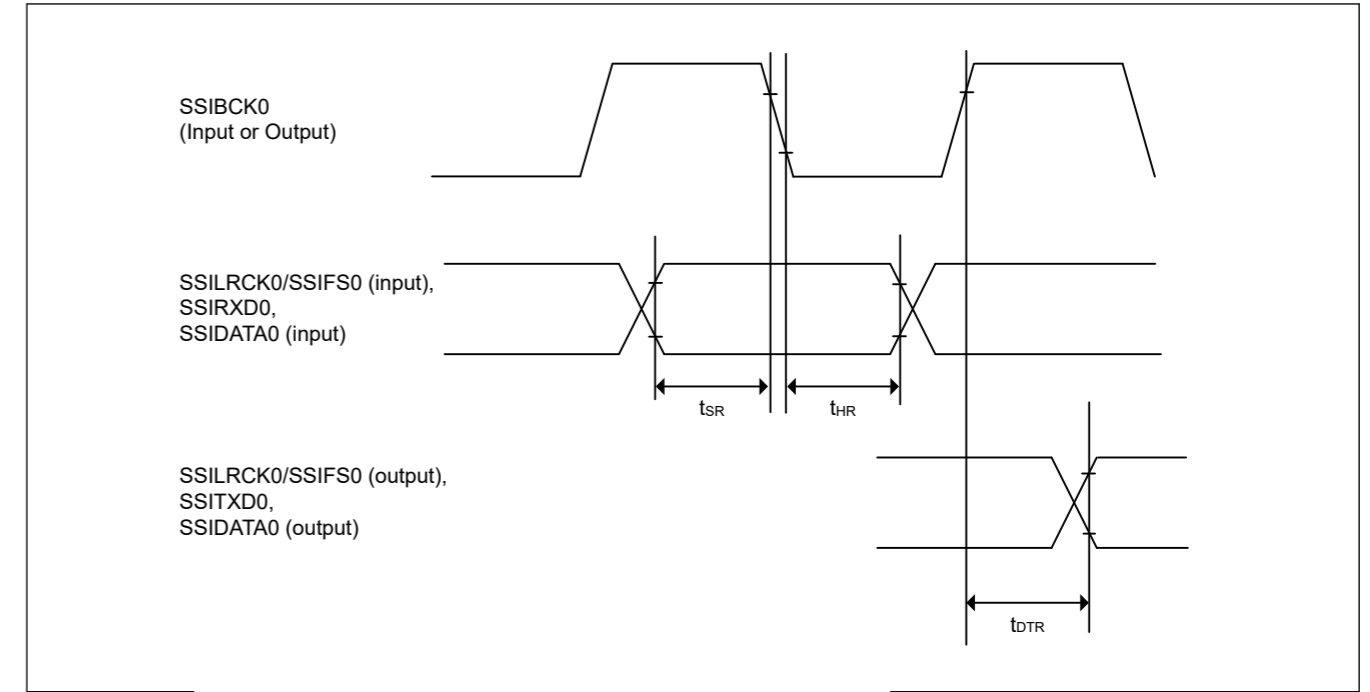
Figure 47.47 SSICR.BCKP=1时的SSIE数据发送和接收时序
