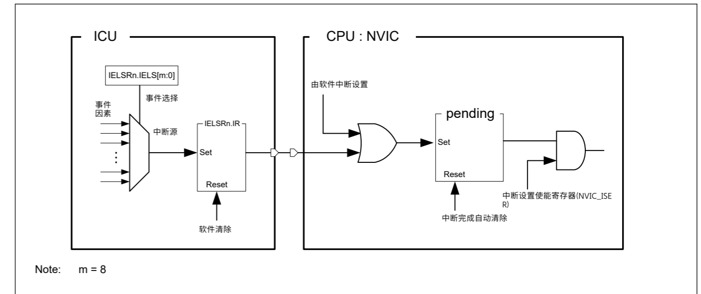
Figure 13.2 ICU和CPU(NVIC)的中断路径
