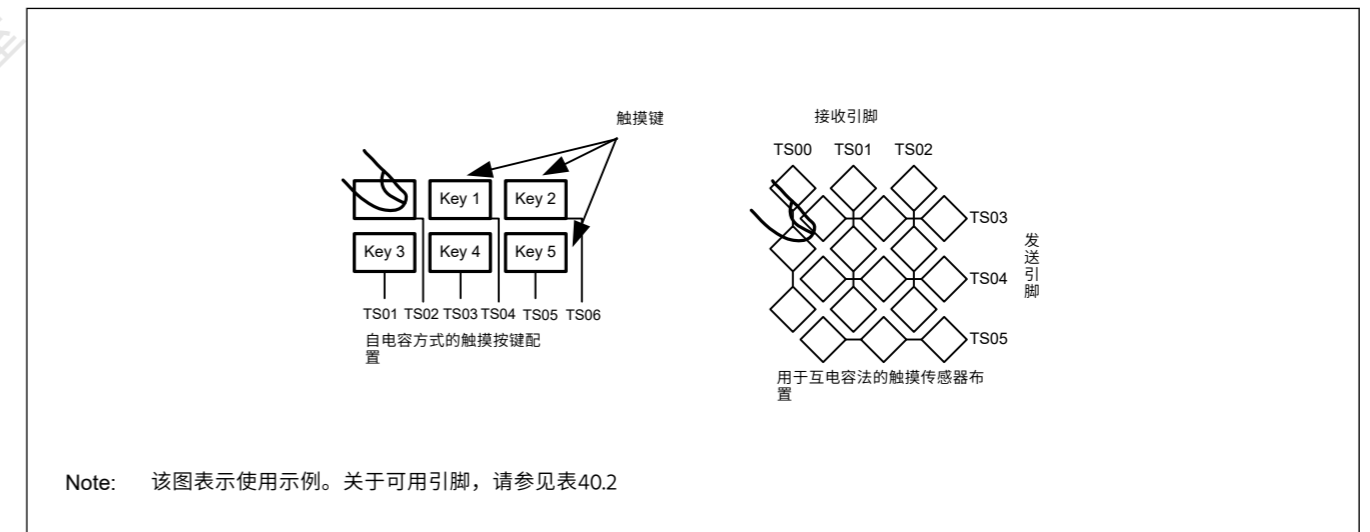
Figure 40.8 自电容法和互电容法概述
