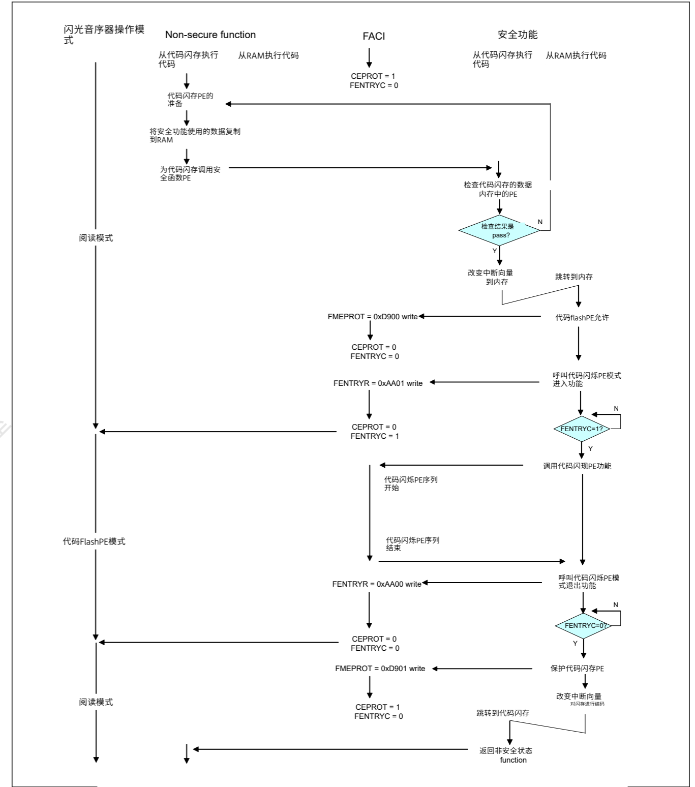
Figure 44.39 CodeFlashPESequenceExamplebynon-securefunction(UsingsecurefunctionforcodeflashPE)
