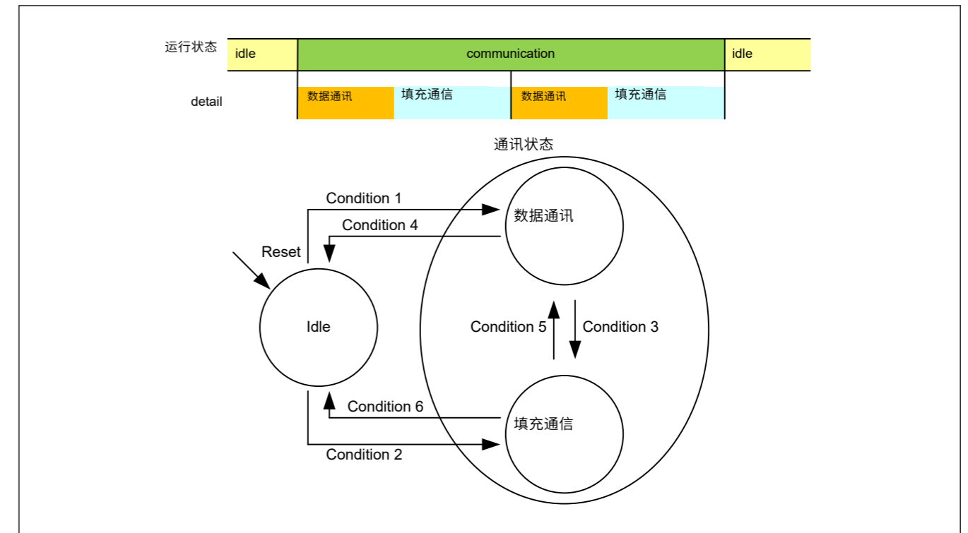
Figure 32.46 通信状态转换
