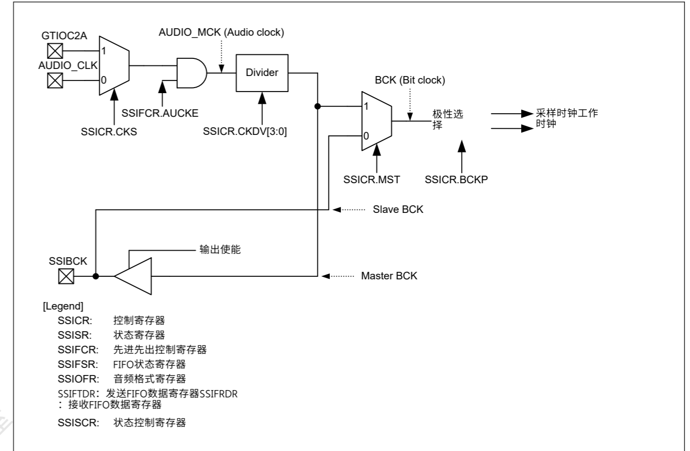
Figure 32.4 SSIE时钟配置
