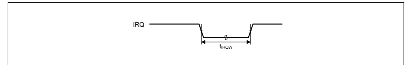
Figure 47.18 IRQ中断输入时序
