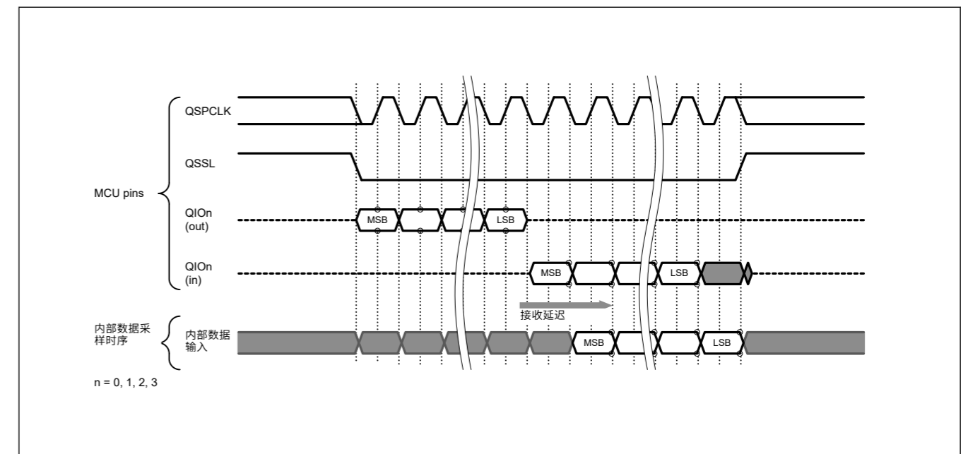
Figure 31.17 接收延迟
