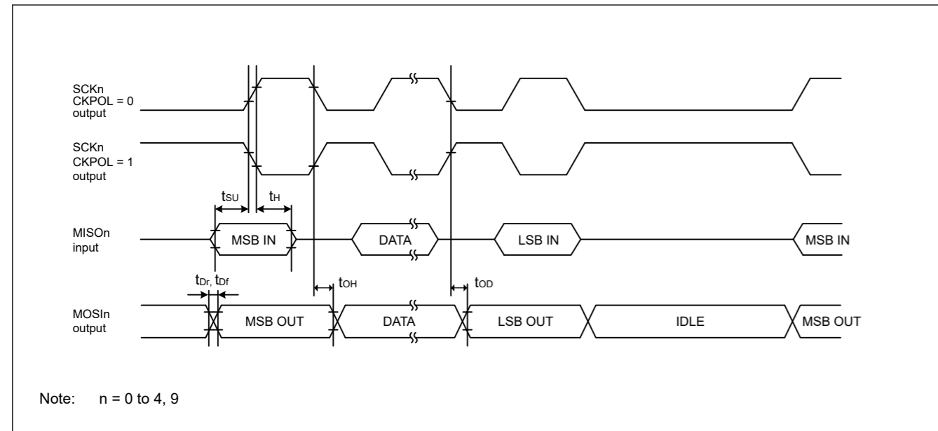
Figure 47.29 SCI simple SPI mode timing for master when CKPH = 1
