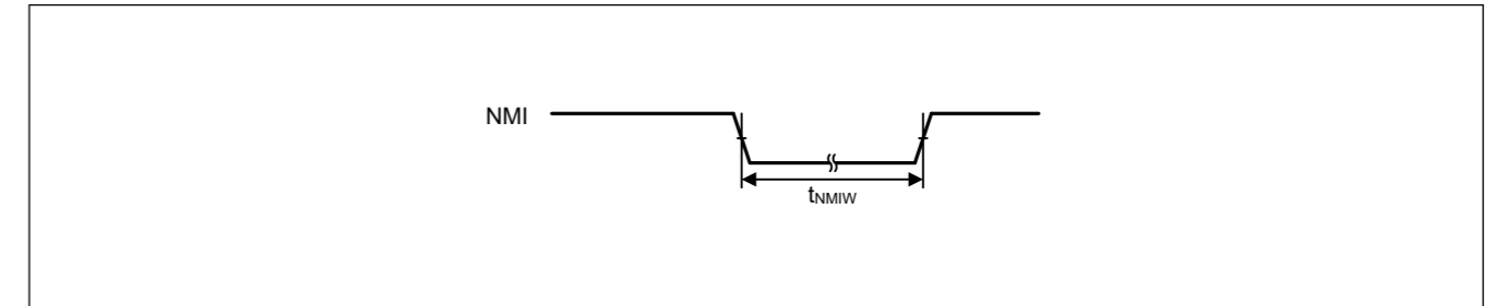
Figure 47.17 NMI中断输入时序
