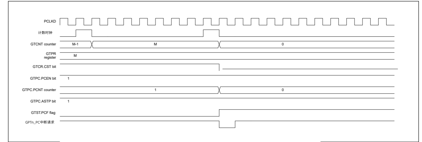
Figure 21.45 PWM周期计数功能示例 (Saw-WaveOne-Shot脉冲模式)
