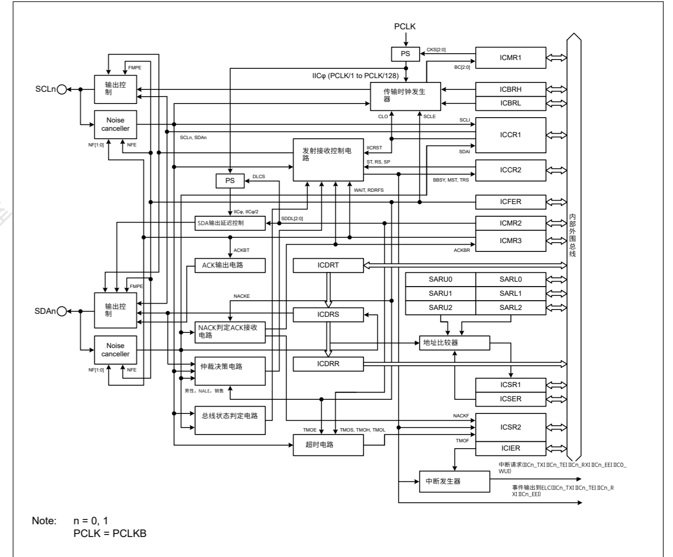
Figure 28.1 IIC框图
