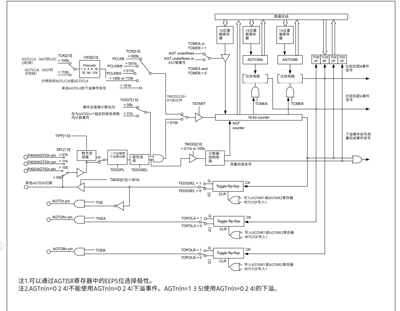
Figure 22.1 AGT框图
