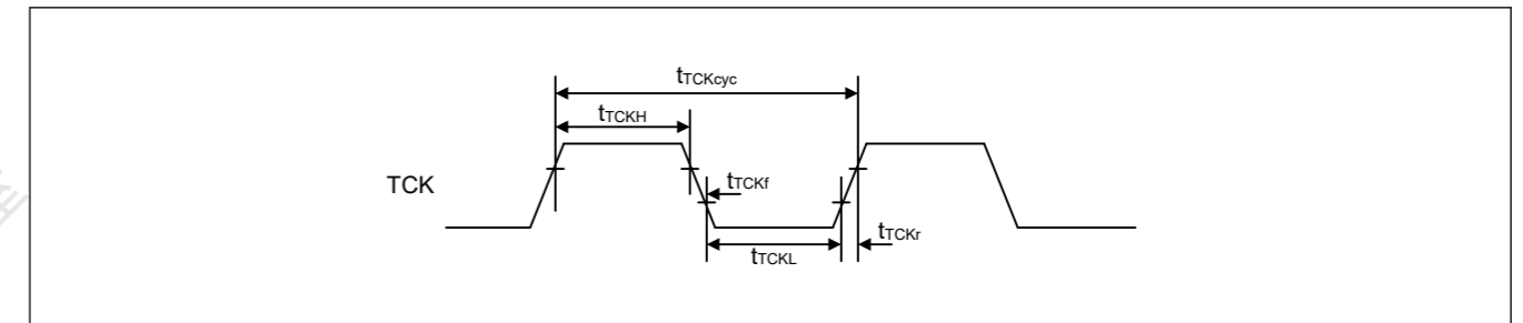
Figure 47.63 边界扫描TCK时序
