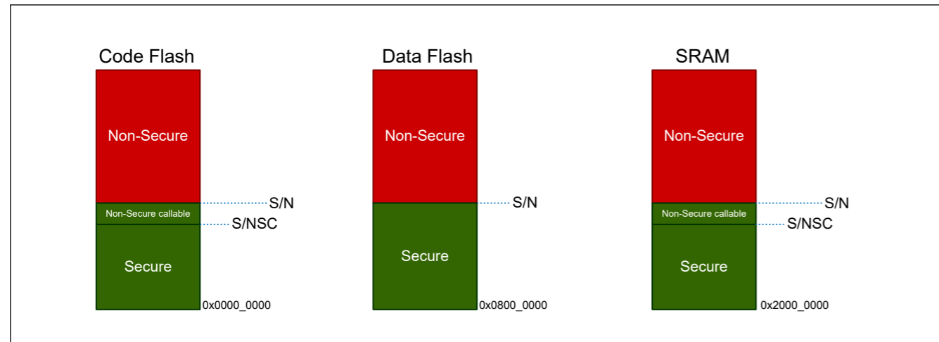
Figure 2.2 Memory partitioning
