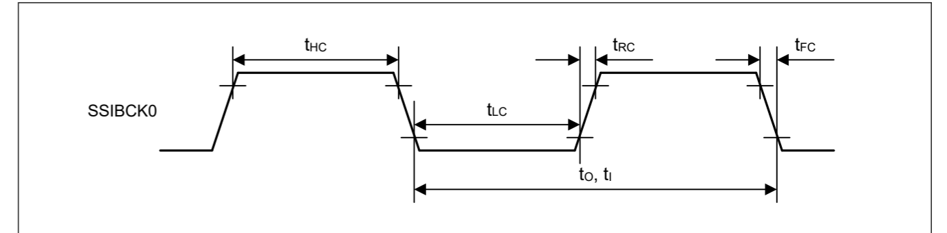
Figure 47.44 SSIE时钟输入输出时序
