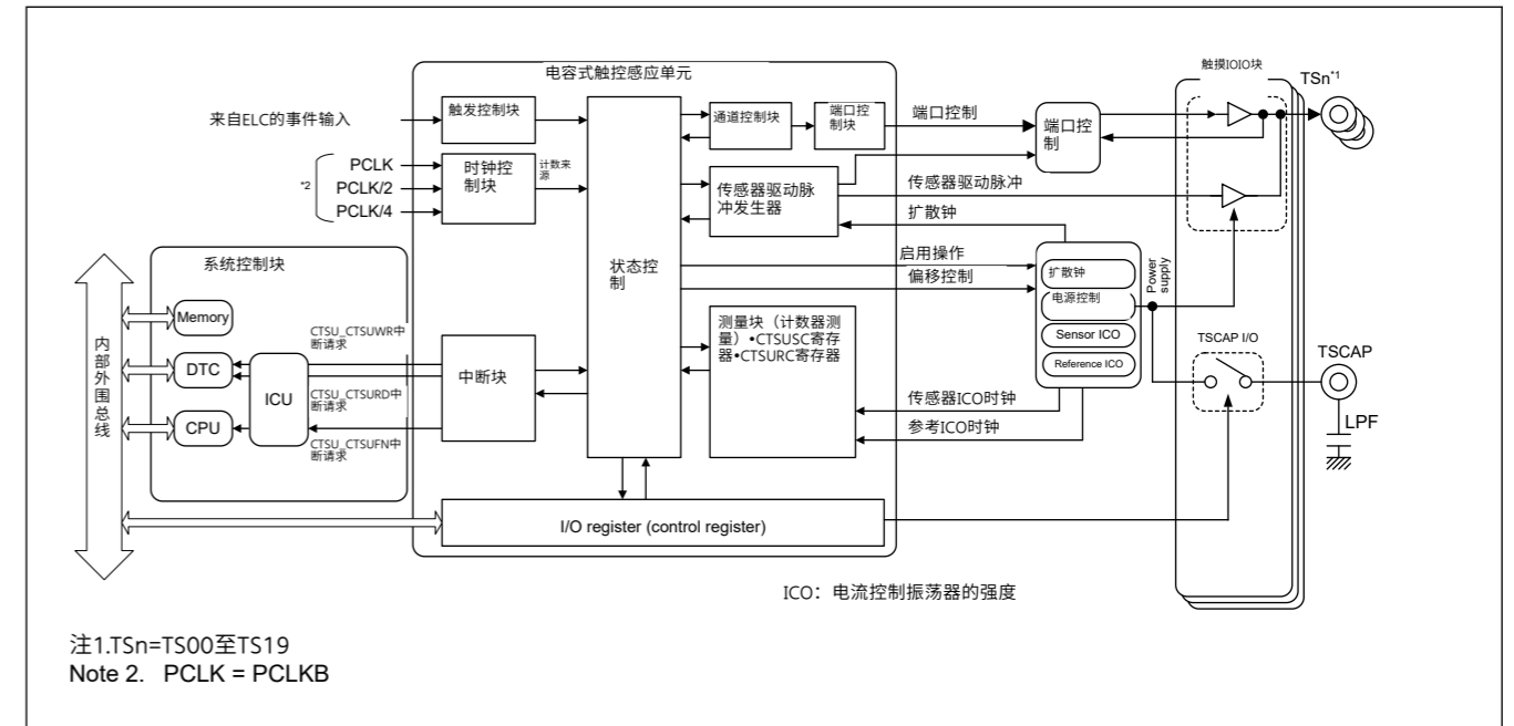
Figure 40.3 CTSU框图
