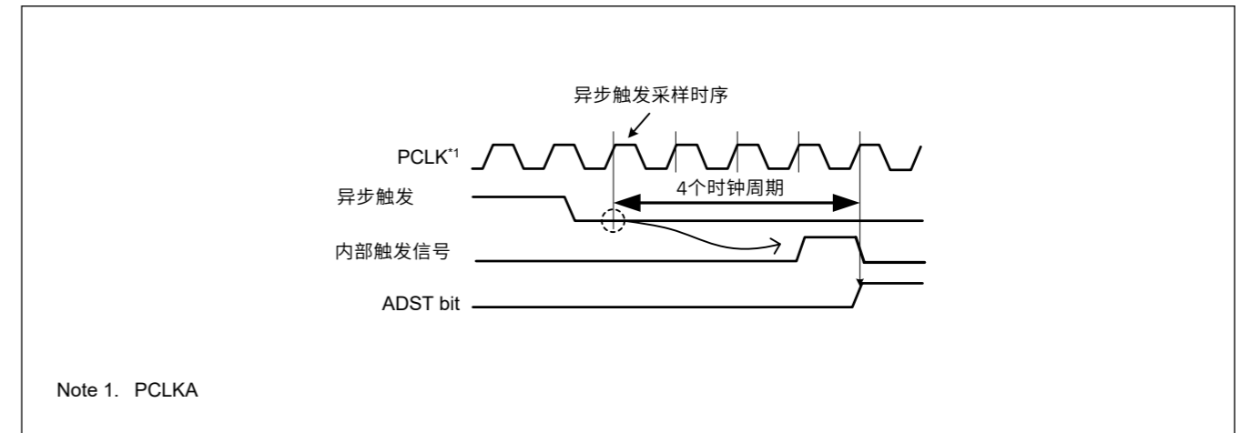
Figure 37.36 异步触发输入时序
