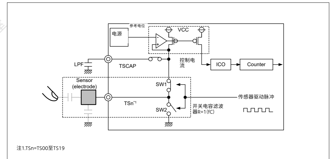
Figure 40.4 测量电路
