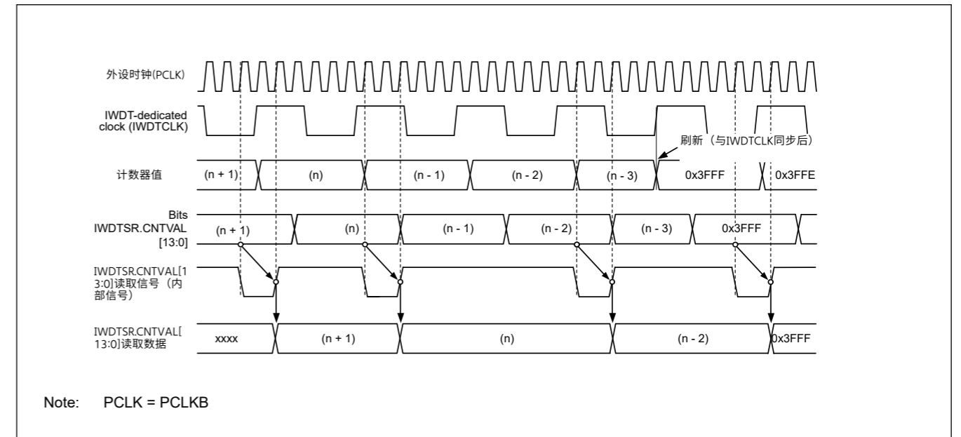
Figure 25.5 OFS0.IWDTCCKS[3:0]=0000b时读取IWDT计数器值的处理, OFS0.IWDTTOPS[1:0] = 11b
