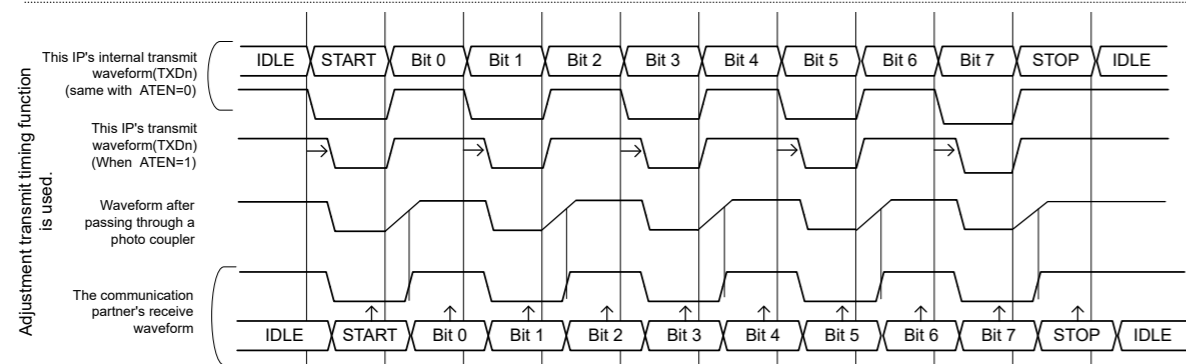
Figure 27.37 The explanation for the transmit waveform through a photo coupler
