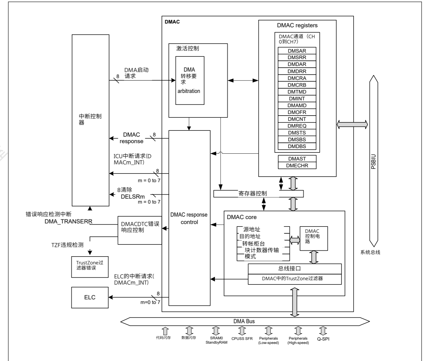
Figure 16.1 DMAC框图
