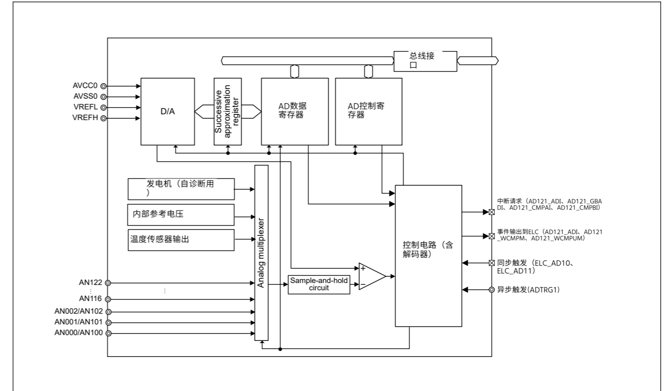
Figure 37.2 ADC12框图 (单元1)
