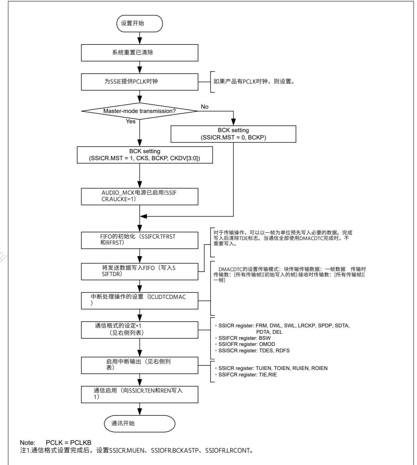
Figure 32.53 开始通信的步骤 (CPU操作步骤)
