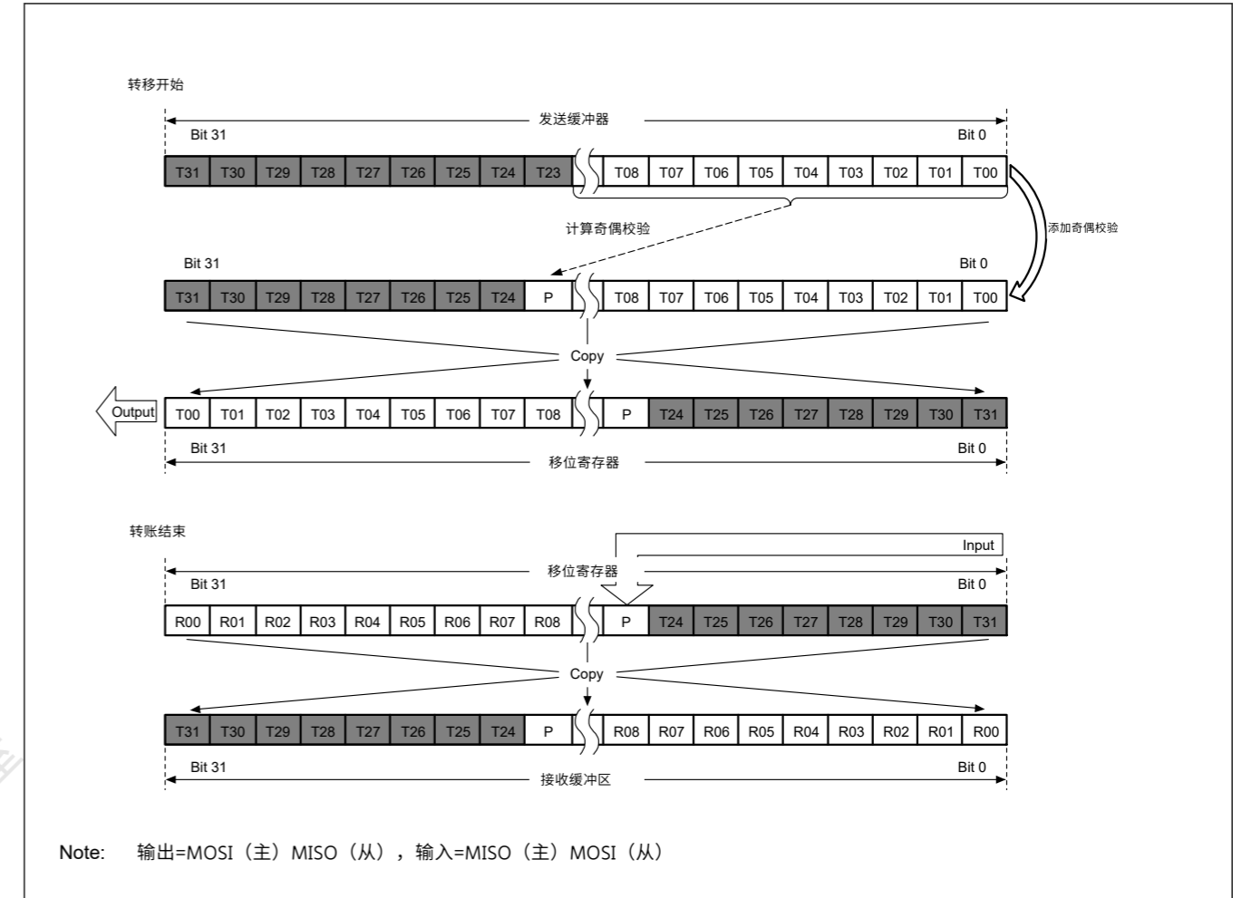
Figure 30.21 启用24位数据和奇偶校验的LSB优先传输
