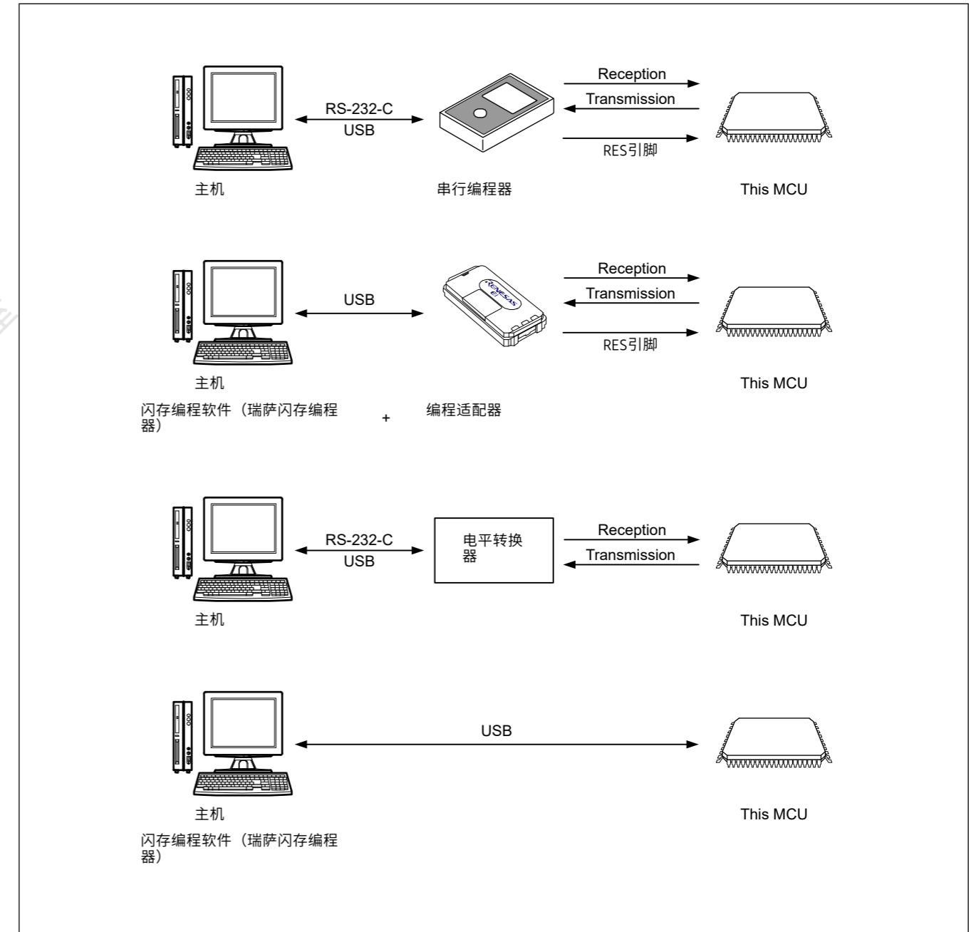
Figure 44.42 重写闪存的环境
