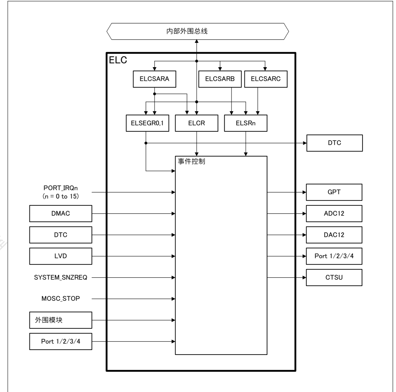
Figure 18.1 ELC框图
