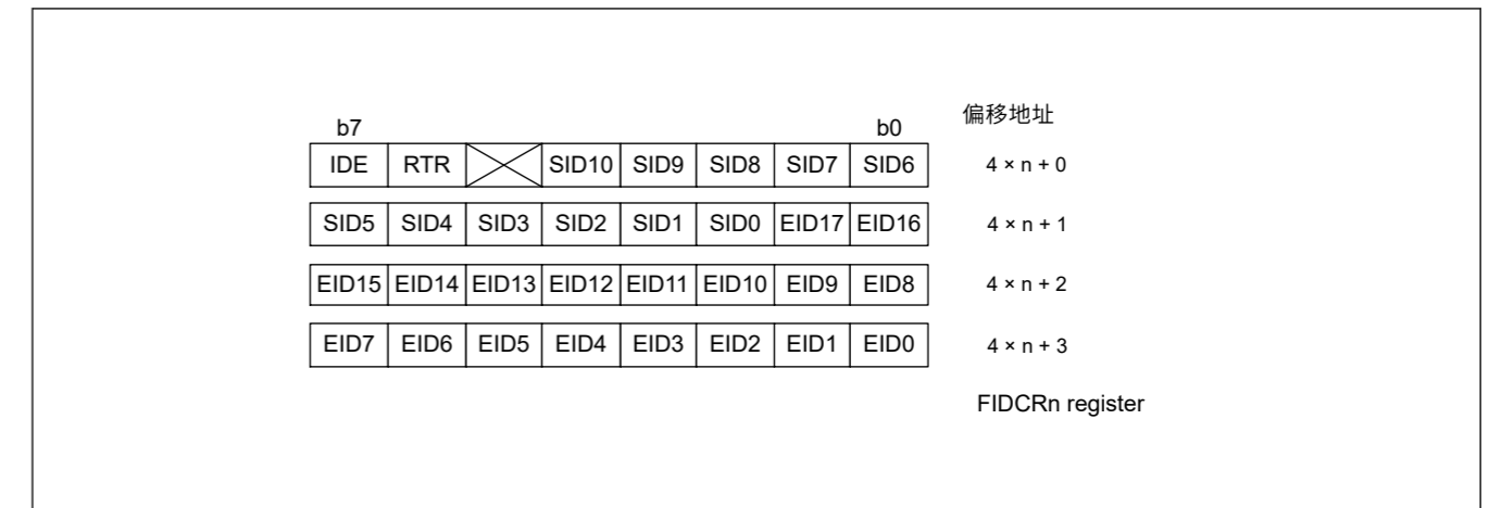
Figure 29.15 FIDCRn寄存器的结构(n=0 1)
