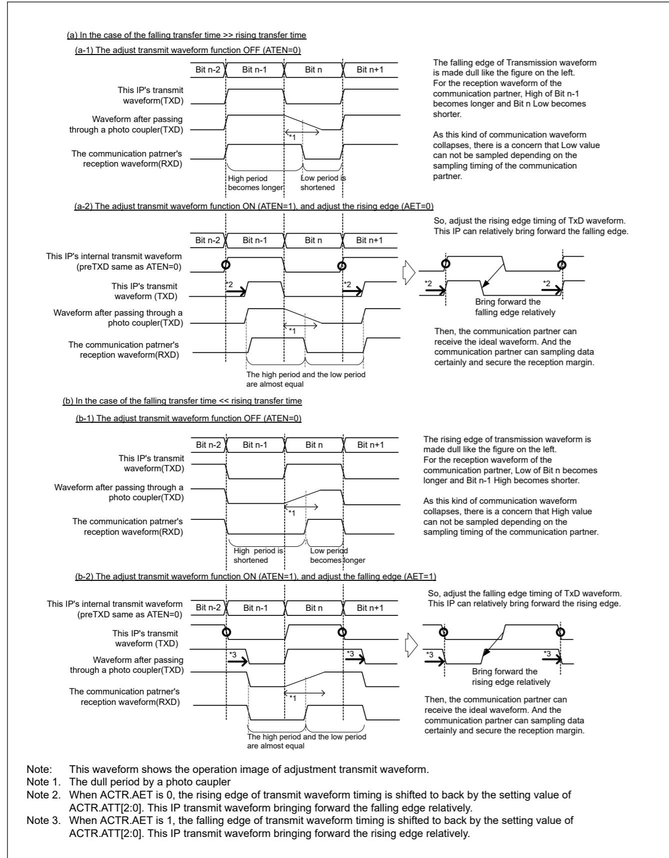
Figure 27.36 The transmission movement image figure of the communication through a photo coupler
