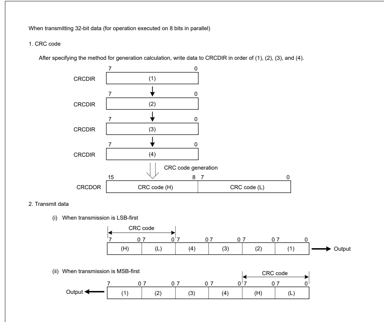
Figure 34.6 LSB-first and MSB-first data transmission
