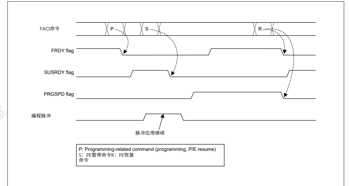
Figure 44.17 编程期间暂停
