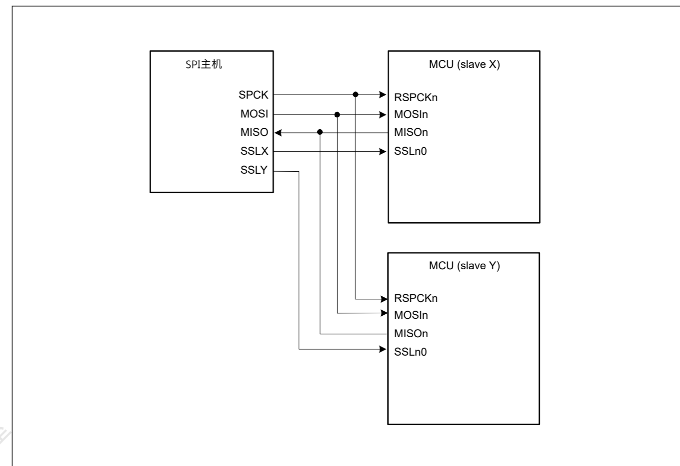
Figure 30.9 MCU作为从机的单主多从配置示例
