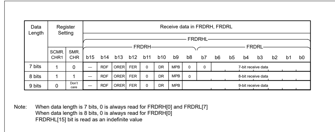
Figure 27.47 Data format stored in FRDRH and FRDRL in multi-processor mode with FIFO selected
