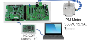
RX26T MCK(Motor Control Kit)
